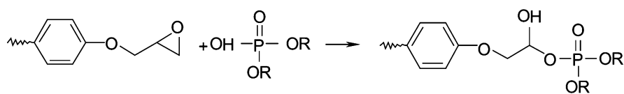
Scheme 4 Dialkyl (or diaryl) phosphate modified epoxy resin, where R is methyl, ethyl, butyl, or phenyl. (Redrawn from Ref. [221] )
