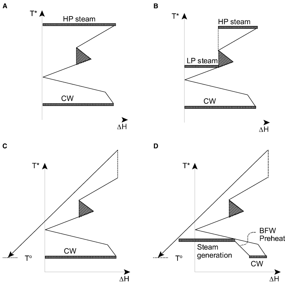
Fig. 21 Examples of the use of the grand composite curve. (A) High pressure steam and cooling water; (B) two steam levels and cooling water; (C) fuel gas and cooling water; (D) fuel gas, steam generation, and cooling water.
