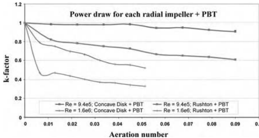
Fig. 6 k -Factor vs. aeration number for the two dual agitation systems. (View this art in color at www.dekker.com .)
