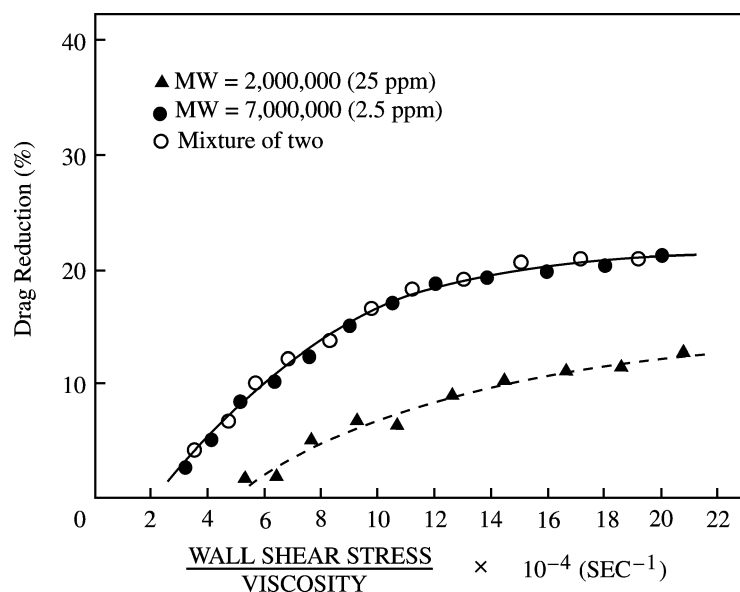
Fig. 3 Molecular weight effects on DR. (From Ref. [18] .)
