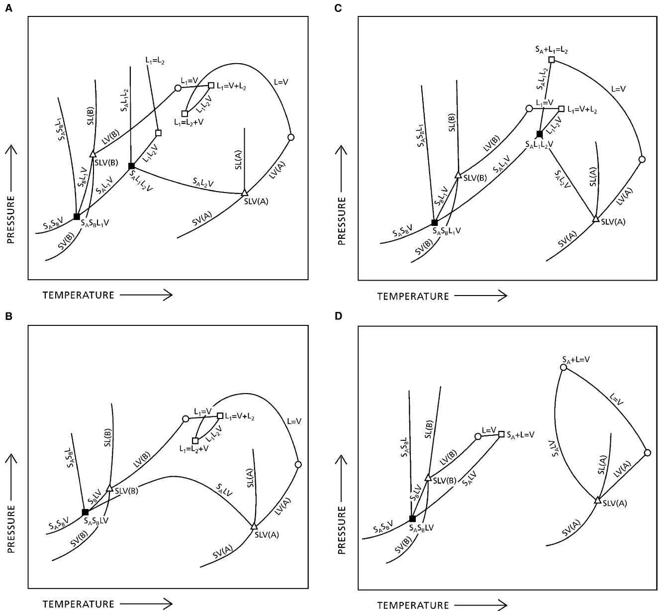
Fig. 5 Possible pressure–temperature projections for Type IV binaries including solids where the melting point of component A increases from A to D.
