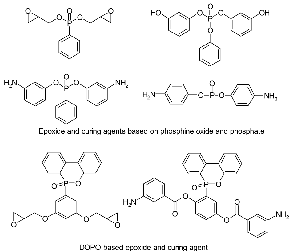
Fig. 9 Selected phosphine oxide-, phosphate-, and DOPO-based epoxides and curing agents. (Redrawn from Ref. [221] .)
