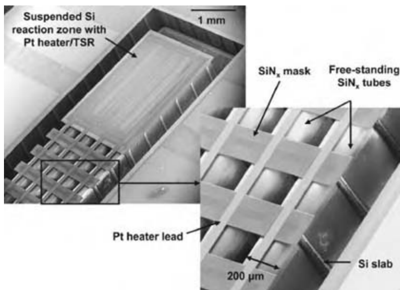
Fig. 11 Scanning electron microscopy photos of microreactor produced by Jensen et al. for reforming of ammonia showing four free-standing \text{SiN}_x tubes, a suspended Si reaction zone with integrated thin-film platinum heater and temperature sensing resistor (TSR), and Si slabs wrapped around the four tubes. (From Ref. [27] .)
