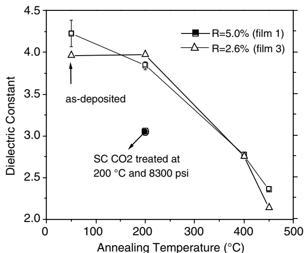
Fig. 11 Effect annealing temperature and SCCO 2 treatments on the dielectric constant of Films 1 and 3. R stands for gas flow ratio given by \{[\text{C}_4\text{H}_{12}\text{Si}]/[(\text{C}_4\text{H}_{12}\text{Si}) + (\text{CH}_4)]\} \times 100\% .
