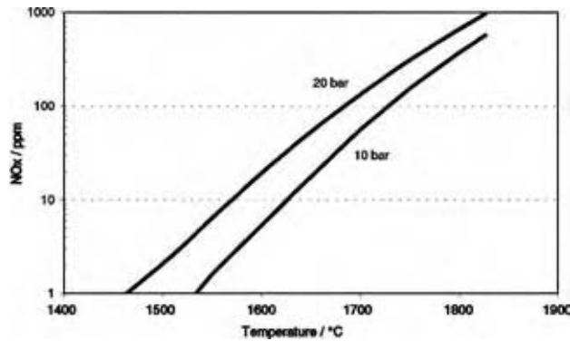
Fig. 2 Calculated NO x levels vs. temperature for the pressures indicated. Curves were calculated using the GRI-Mech combustion kinetics database for an isothermal combustor with 20 msec residence time and an inlet composition showed in Table 1. (From Ref. [1] ) (View this art in color at www.dekker.com .)
