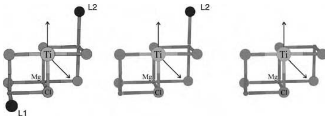
Fig. 6 Model of possible active species for highly isotactic, isotactoid and syndiotactic propagation. (From Ref. [53] ) (View this art in color at www.dekker.com .)
