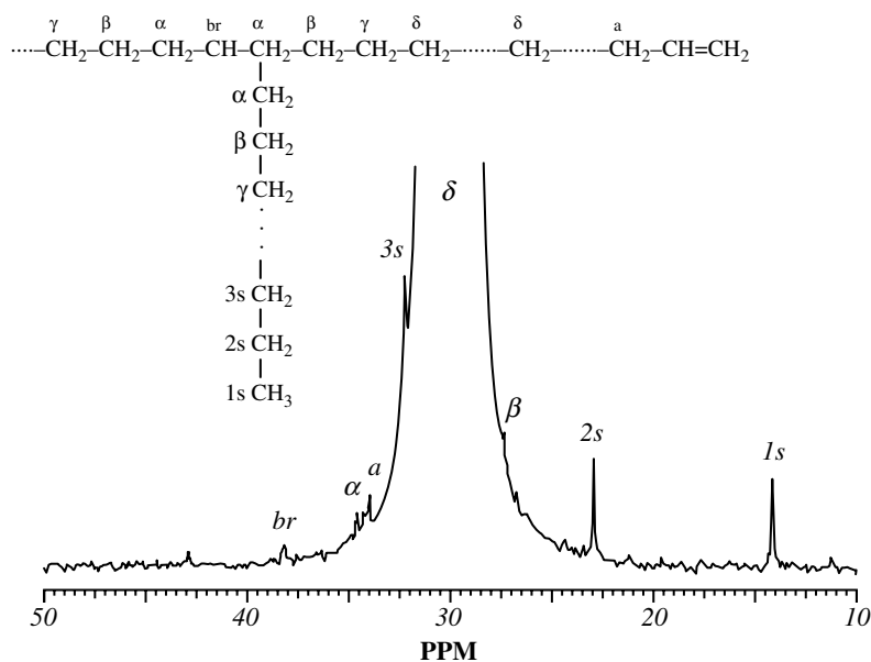
Fig. 4 ^{13}\text{C} -NMR spectrum of polyethylene sample measured at 120^\circ\text{C} using deuterium o -dichlorobenzene and 1,2,4-trichlorobenzene as solvents. (From Ref. [62] .)
