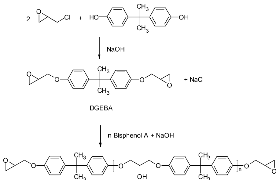
Scheme 1 Commercial preparation of the diglycidyl ether of bisphenol A, DGEBA, and higher oligomers.
