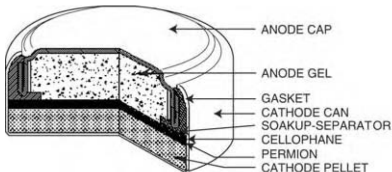
Fig. 3 Typical cell construction of the button alkaline cell. (From Ref. [14] .)
