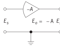
Fig. 5. Symbol for a high-gain direct-current amplifier, with one inverting input referenced to ground.
