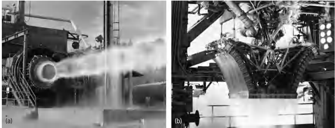
Fig. 1. Static firing tests of (a) aerospike engine with 250,000 pounds (1,112,000 newtons) of thrust, and (b) linear aerospike engine with 125,000 pounds (556,000 newtons) of thrust. Both engines use hydrogen/oxygen propellants. (Boeing Company, Rocketdyne Division)
