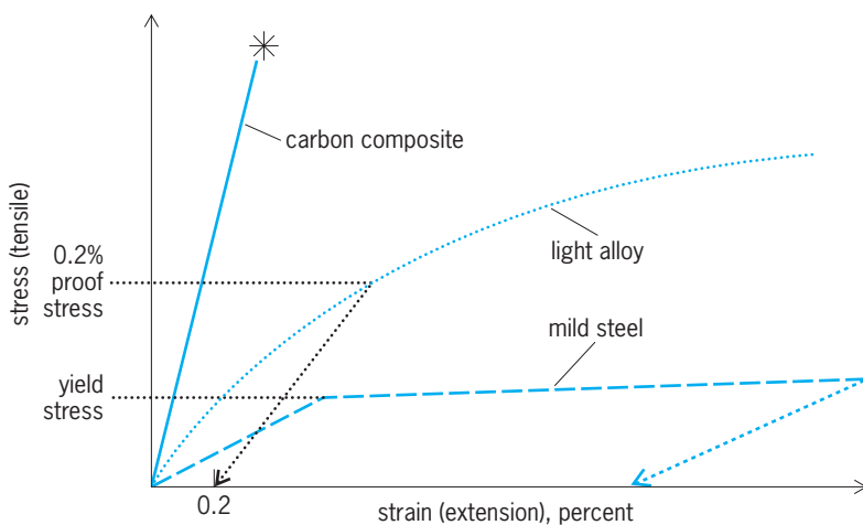
Fig. 2. Stress/strain curves for various types of material.
