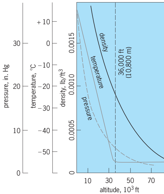
Fig. 4. Variation of ambient pressure, temperature, and density as functions of altitude. 1 in. Hg = 3.4 kPa; ^{\circ}\text{F} = (^{\circ}\text{C} \times 1.8) + 32 ; 1 \text{ lb/ft}^3 = 16.0 \text{ kg/m}^3 ; 10 \text{ M ft} = 10,000 \text{ ft} = 3000 \text{ m} . (After I. E. Treager, Aircraft Gas Turbine Technology , 2d ed., McGraw-Hill, 1979)
