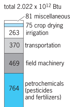
Fig. 3. Energy use in United States agricultural production. (USDA)
