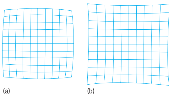
Fig. 3. Distortion. (a) Barrel distortion. (b) Pincushion distortion.
