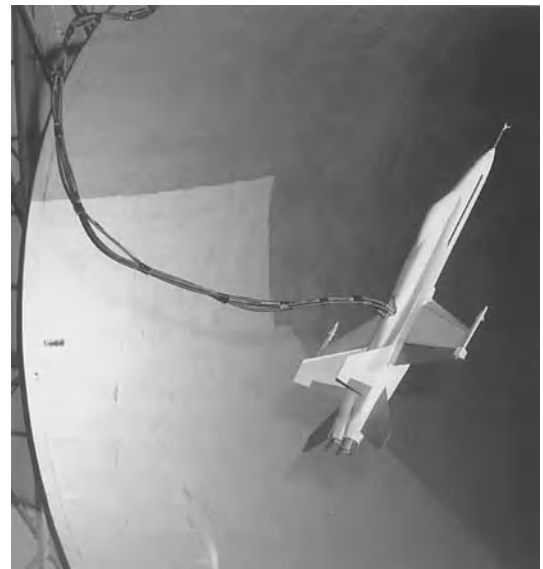
Fig. 2. Free-flying scale model aircraft in wind tunnel; attached cable contains sensors and other measurement instruments. (NASA)
