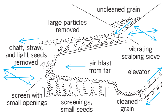
Fig. 21. Fanning mill operation.
