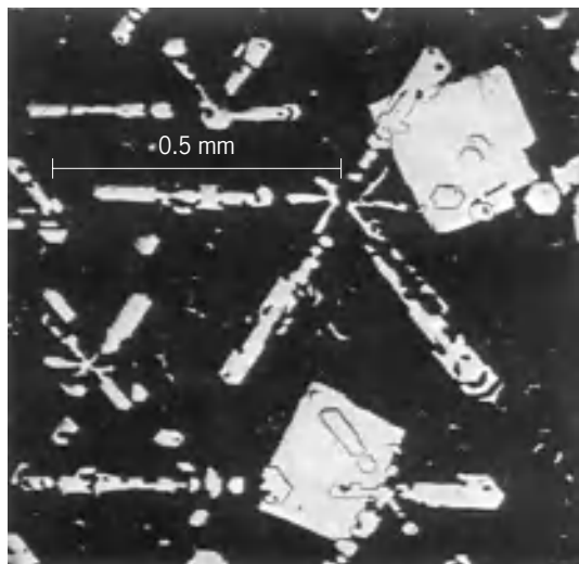
Fig. 1. Babbitt metal (84% Sn–7% Cu–9% Sb). The white areas are crystals of CuSn (star dendrites) and SbSn (nearly square); these resist wear. The dark matrix is a soft, tin-rich alloy, which adjusts to the hard particles to give uniform loading. (From R. M. Brick et al., Structure and Properties of Alloys , 3d ed., McGraw-Hill, 1965)
