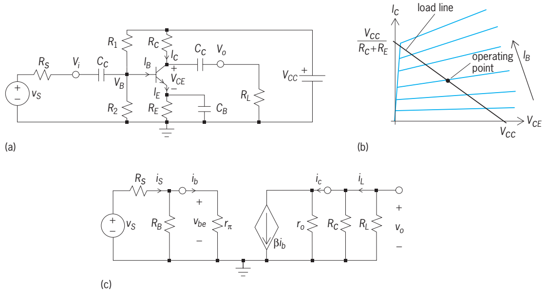
Fig. 5. Bipolar junction transistor common-emitter amplifier. (a) Circuit diagram. (b) Transistor dc characteristics and load line, showing placement of operating point. Arrow indicates increasing values of I_B . (c) Small-signal model of amplifier.
