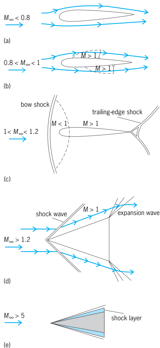
Fig. 1. Regimes for aerodynamic flows; M_\infty = Mach number for flow far upstream of the airfoil: (a) subsonic flow; (b) transonic flow with M_\infty < 1 ; (c) transonic flow with M_\infty > 1 ; (d) supersonic flow; and (e) hypersonic flow, where the thin, hot shock layer has viscous interaction and chemical reactions.
