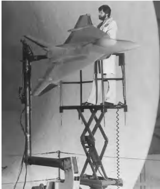
Fig. 1. Scale model of fighter aircraft being mounted inside test section of large wind tunnel. (NASA)
