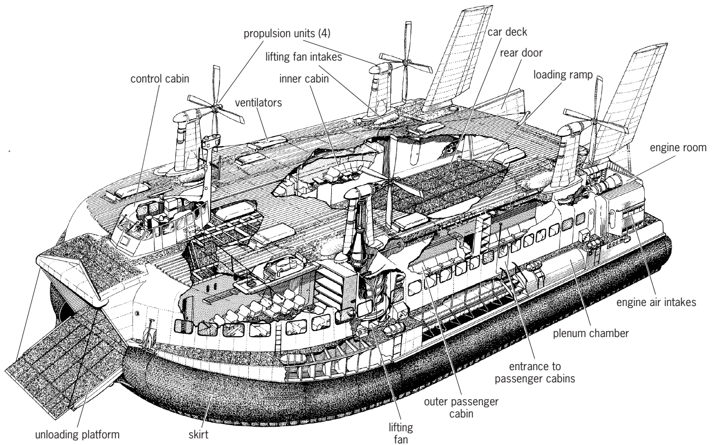
Fig. 2. Air-cushion vehicle used to transport cars and passengers across the English Channel. (British Hovercraft Corp.)
