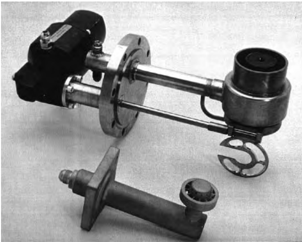
Figure 3-13. Courtesy of Solar Turbines Incorporated. Comparison of the low \text{NO}_x and standard fuel injectors for the Centaur 50 gas turbine. SoLo \text{NO}_x ™ is Solar's designation for its low \text{NO}_x emission engine configuration.
