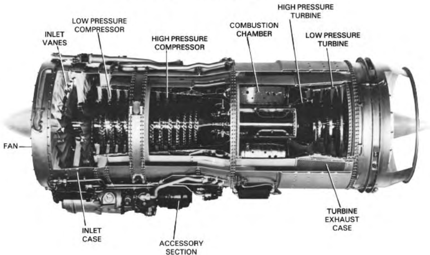
Figure 2-1. Courtesy of United Technologies Corporation, Pratt & Whitney Aircraft. The JT8D turbofan engine was one of the early “bypass” engines (BPR 1.7:1). The JT8D-200 series produces over 20,000 pounds “take-off” thrust and powers the McDonnell Douglas MD-80. The FT8 is the industrial, aero-derivative, version of this engine.
