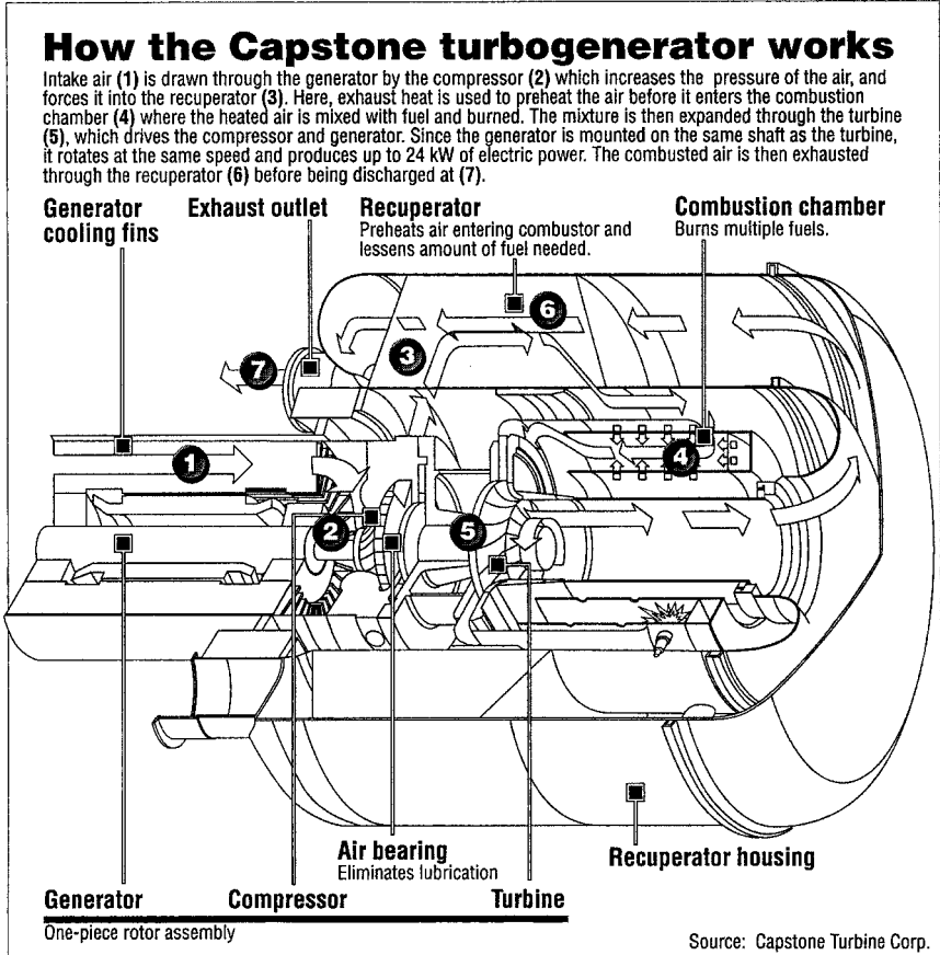
Figure 18-3. Courtesy of Capstone Turbine Corp. Schematic cross-section of the ISO base load 24 kilowatt turbogenerator. This unit, configured with the centrifugal compressor and turbine wheels mounted on the same shaft as the electric generator, weighs 165 pounds.
