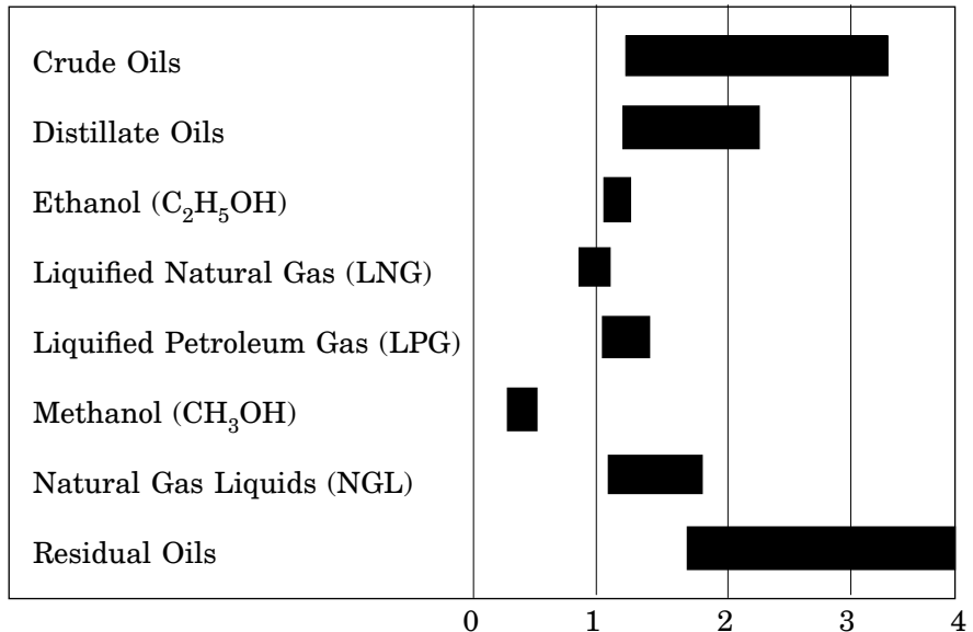
Figure 9-2. Courtesy of Solar Turbines Incorporated. Comparison to methane of the relative Thermal NO x produced by various liquid fuels.
