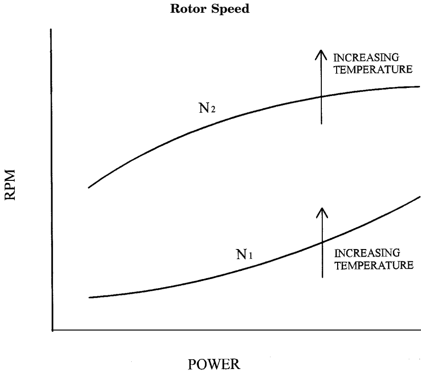
Figure 7-4. Rotor speed is a control function biased by temperature.
