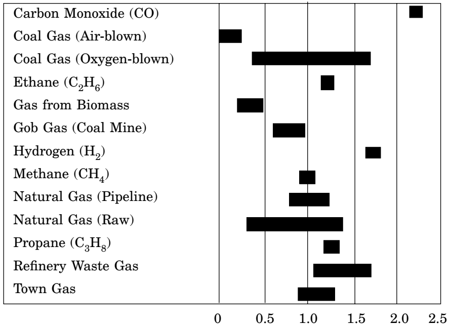
Figure 9-1. Courtesy of Solar Turbines Incorporated. Comparison to methane of the relative Thermal \text{NO}_x produced by various fuel gases.
