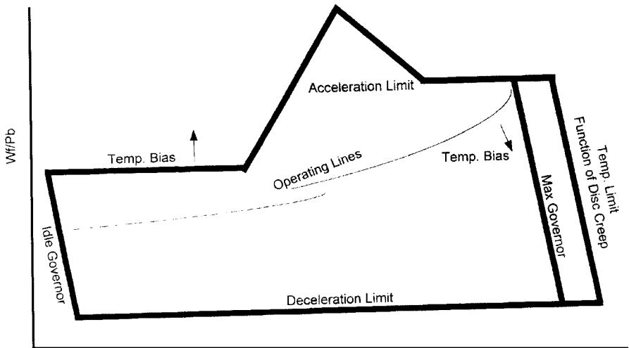
Figure 5-7 Control map.
