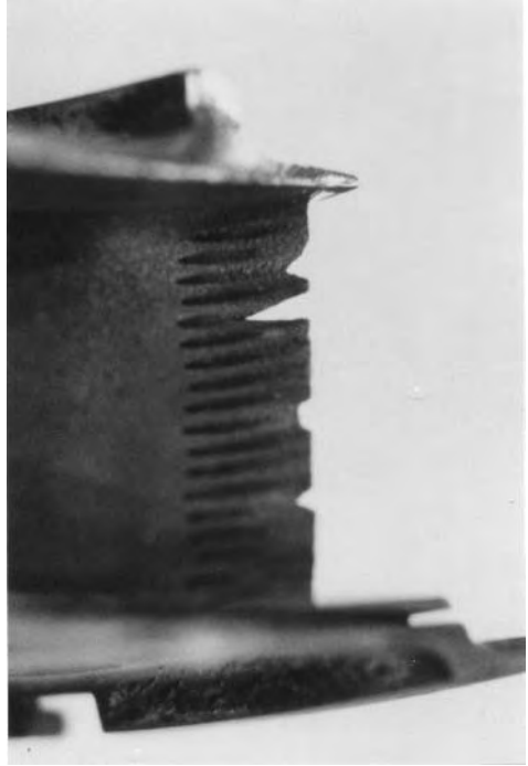
Figure 13-18. Cracked, burnt, eroded, and corroded first stage turbine nozzle concave trailing edge surface. This 4,500 horsepower gas turbine-generator unit operated for 17,000 hours with undersized water injection nozzle orifices in half the distribution ring.
