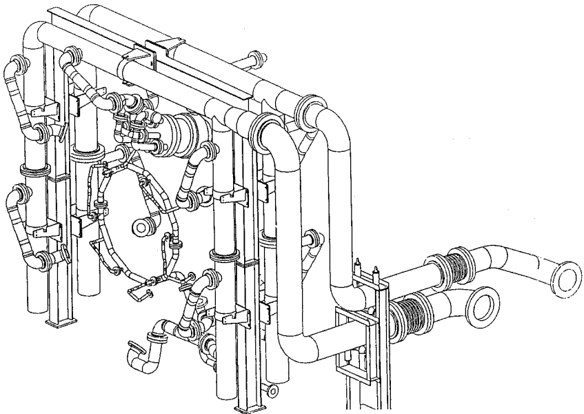
Figure 14-7. View of MS6001FA Combustor Case Extraction Manifold.
