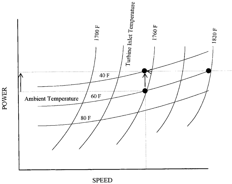
Figure 5-2. Temperature-power-speed interrelationships.
