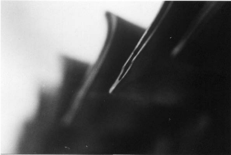
Figure 13-27. First stage turbine blade trailing edge tip rub. 5,000 horsepower gas turbine-compressor drive unit with 8,000 hours operation.
