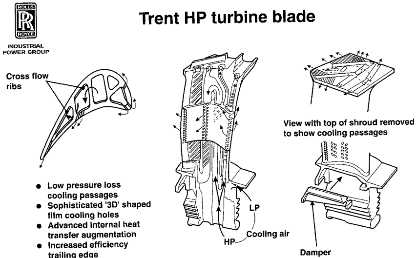
Figure 3-6. Courtesy of Rolls-Royce Industrial & Marine Gas Turbines Limited. Composite view of the Trent high pressure turbine blade showing its internal cooling scheme. The Trent is a growth version of the RB211 aero and industrial engine. The industrial Trent gas turbine is a 70,000 shaft horsepower engine.
