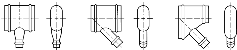
90° conical tee
