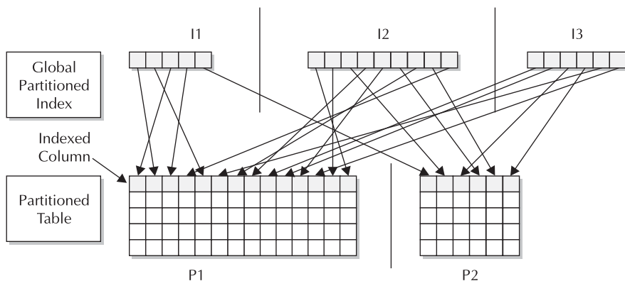
FIGURE 16-2 Global partitioned index on a partitioned table
