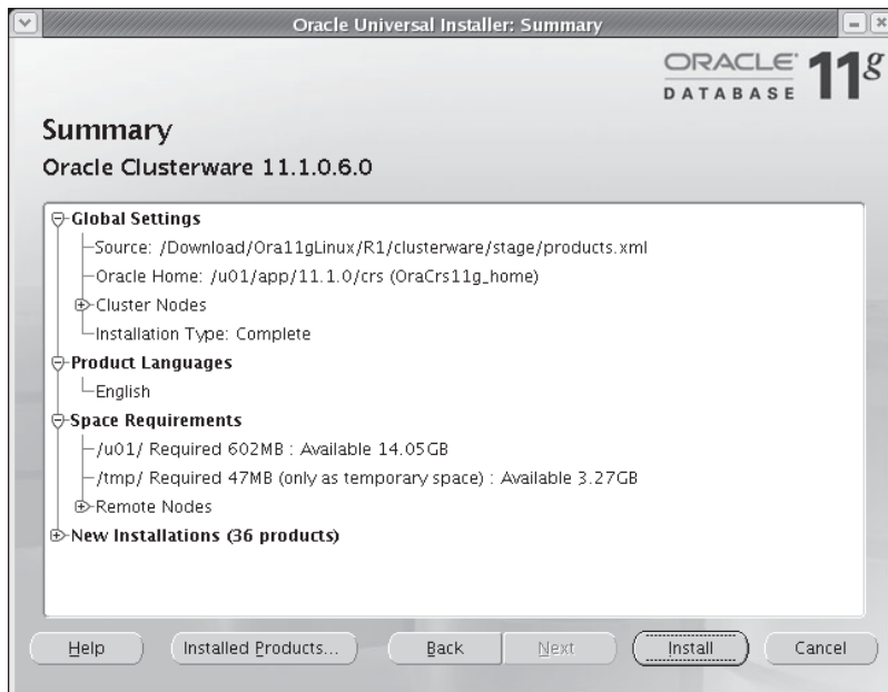
FIGURE 10-7 Pre-installation summary
