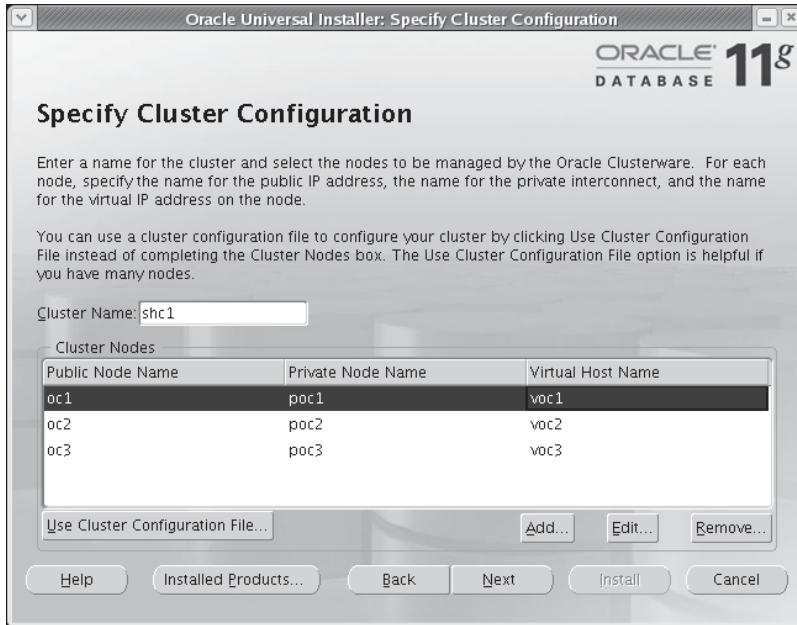
FIGURE 10-3 Cluster configuration
