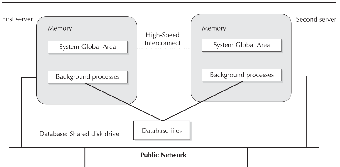
FIGURE 10-1 RAC network configuration
