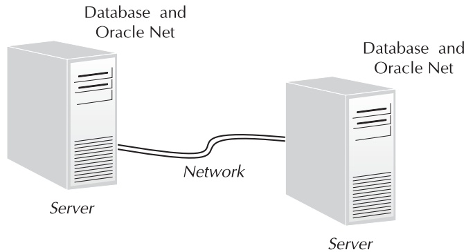
FIGURE 15-3 Server/server architecture
