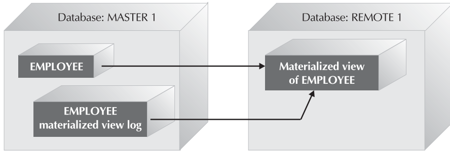
(a) A simple materialized view; materialized view logs can be used.
