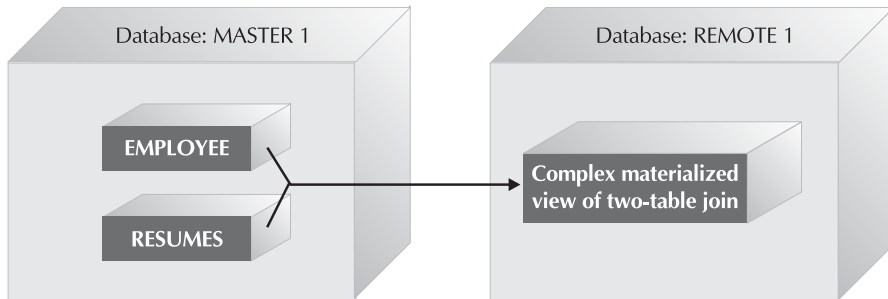
(b) A complex materialized view; the result of the join is replicated.
