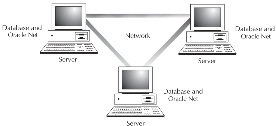
FIGURE 17-1 Server/Server architecture
