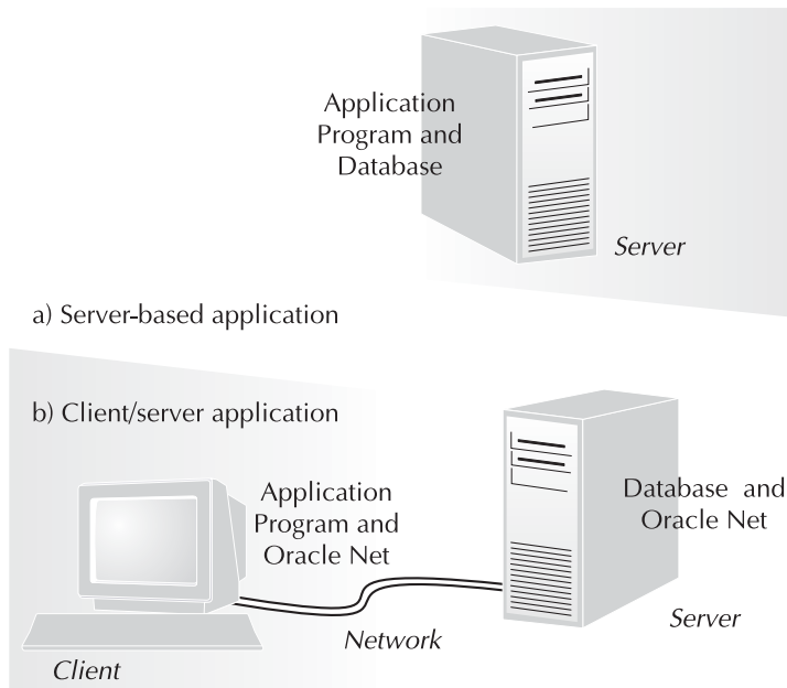
FIGURE 15-1 Client/server architecture
