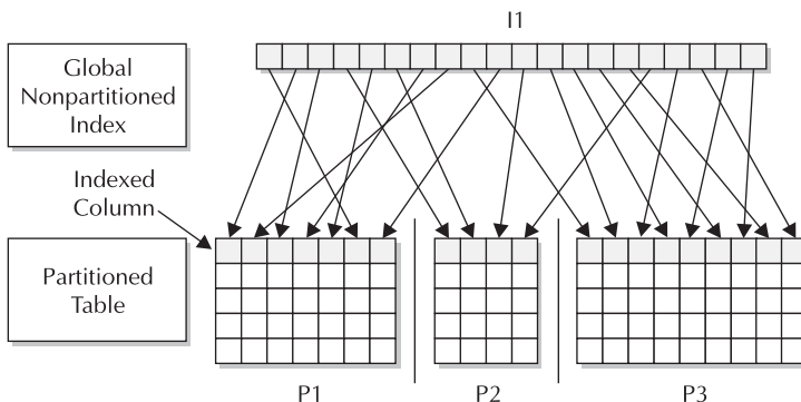
FIGURE 16-3 Global nonpartitioned index on a partitioned table
