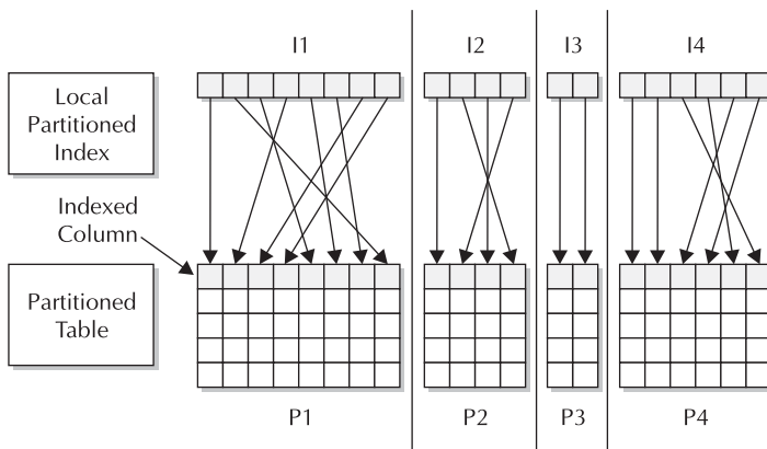
FIGURE 16-1 Local partitioned index on a partitioned table
