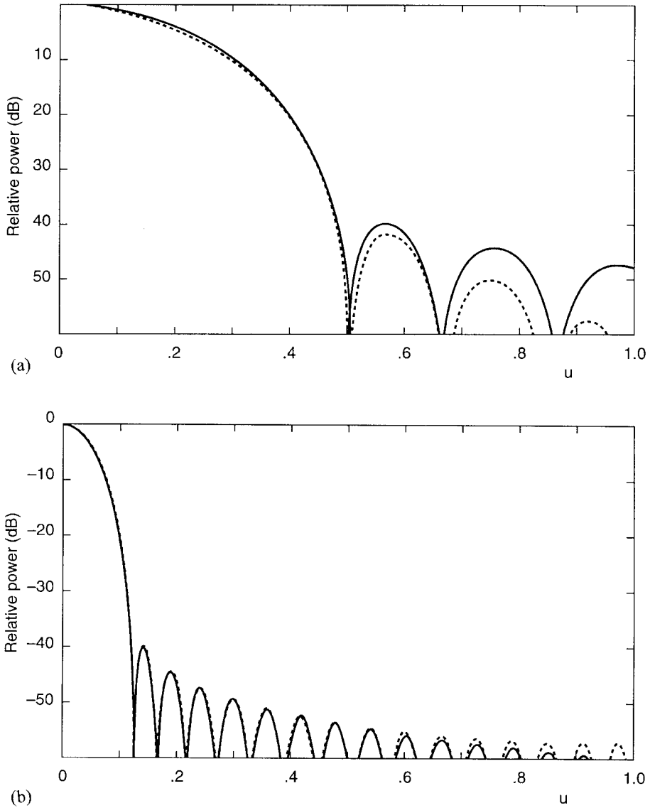
Figure 3.7 Modified \sin(\pi z)/(\pi z) line source and array patterns ( -40 -dB sidelobes) (solid curves from function, dashed curve from array currents): (a) four-wavelength line sources (solid) and 8-element array patterns (dashed); and (b) 16-wavelength line source (solid) and 32-element array patterns (dashed).
