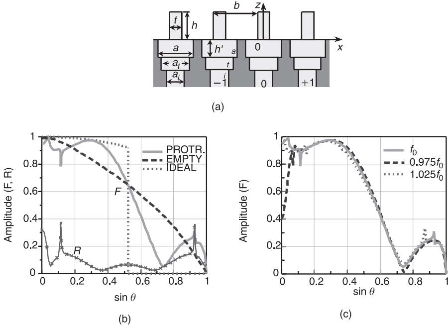
Figure 8.19 (a) Geometry of a parallel plate array with protruding dielectric elements; (b) element pattern and reflection coefficient of array with a_i = 0.4\lambda , a_t = 0.45\lambda , h_t = 0.25\lambda , \epsilon_i = \epsilon_t = 1 , a = 0.57\lambda , h' = 0.3\lambda , b = 0.96\lambda , \epsilon_a = \epsilon = 2 , t = 0.5\lambda , and h = 1.2\lambda ; element pattern of an empty waveguide array with no protrusions, a_i = 0.4\lambda , a_t = 0.65\lambda , h_t = 0.25\lambda , a = 0.9\lambda , h' = 0.7\lambda , b = 0.96\lambda , \epsilon_i = \epsilon_t = \epsilon_a = 1 ; and (c) element pattern of the array with protrusions at frequencies f_0 (reference frequency), 0.975f_0 , and 1.025f_0 . (After: [54].)
