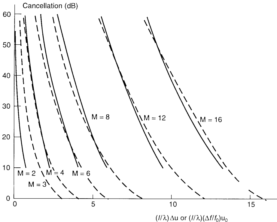
Figure 3.23 Sidelobe cancellation versus number of equispaced pattern nulls M , normalized array length \ell/\lambda , and nulling sector \Delta u . (After: [71, 72].)
