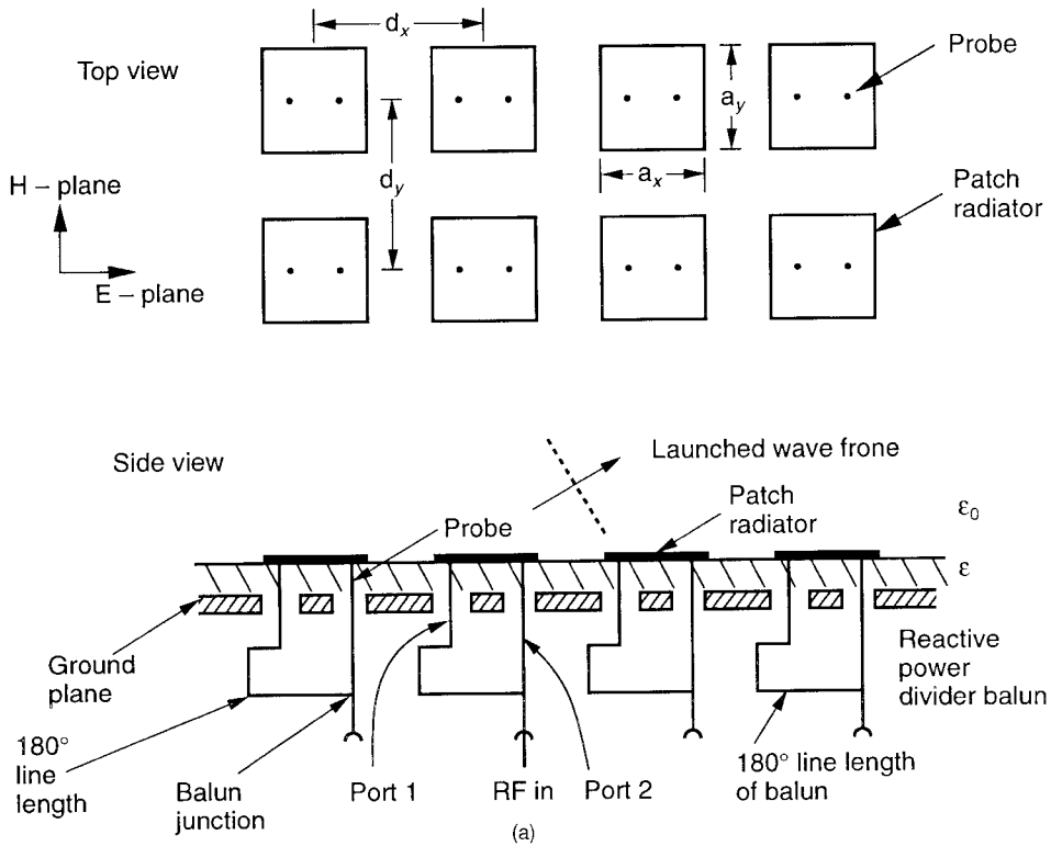
Figure 6.19 Characteristics of dual-probe fed microstrip arrays of rectangular patches: (a) balanced fed patch radiator geometry; and (b) measured and predicted E -plane embedded element pattern of radiator at 1.05f_0 . (From: [59]. © 1991 Electromagnetics Journal. Reprinted with permission.)
