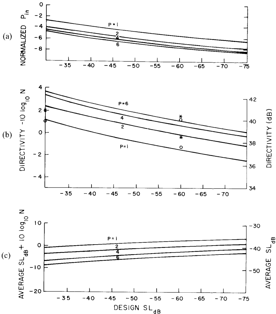
Figure 2.18 (a) Input power, (b) directivity, and (c) average sidelobe level for method 1 (thinning quantization). (From: [40]. © 1991 IEEE. Reprinted with permission.)
