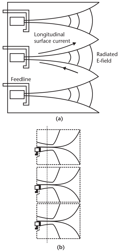
Figure 5.14 Wideband antennas: (a) flared notch; and (b) printed flared dipole “bunny ear.” (After: [72].)
