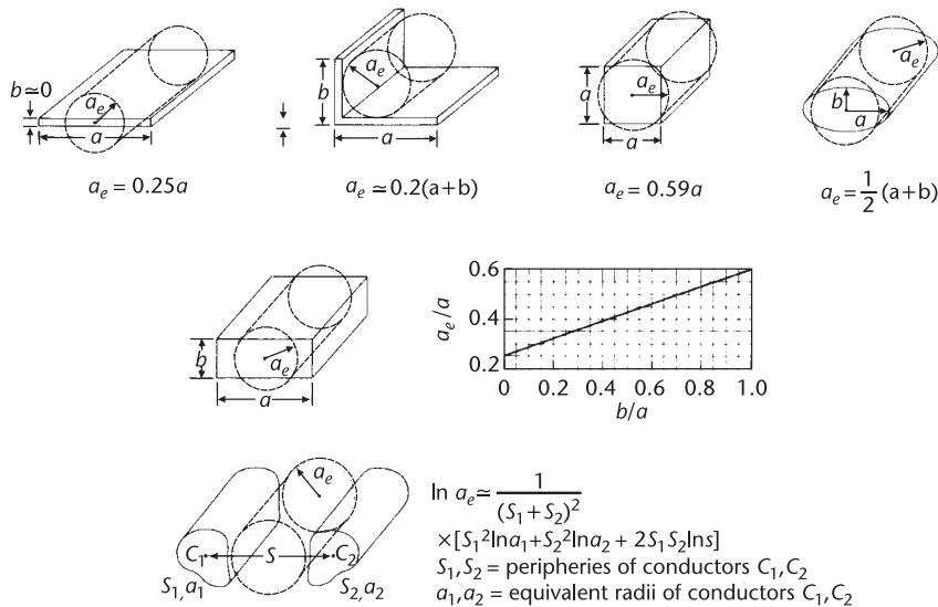
Figure 5.2 Conductor geometrical shapes and their equivalent circular cylinder radii. (From: [2]. © 1997 Harper and Row, Inc. Reprinted with permission.)
