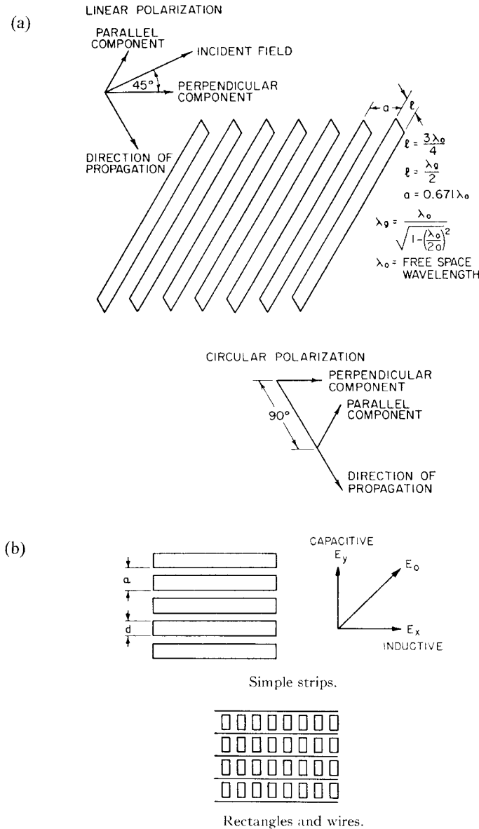
Figure 5.29 Polarizers and polarizing grids for arrays. (a) Quarter-wave polarizer. (From: [157]. © 1950 IEEE. Reprinted with permission.) (b) Lerner polarizer, simple strips and rectangle and wire grids. (From: [159]. © 1965 IEEE. Reprinted with permission.) (c) Meander line polarizer. (From: [160]. © 1973 IEEE. Reprinted with permission.) (d) Element rotation for circular polarized array. (After: [161].)
