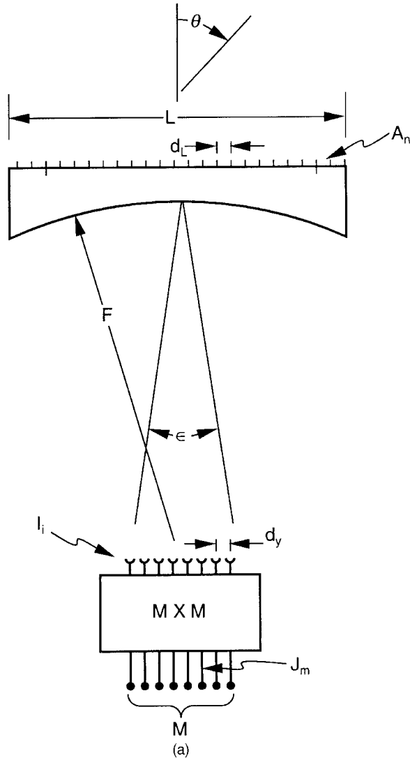
Figure 8.34 Geometry of transform-fed lens antenna: (a) two-dimensional cylindrical lens; and (b) two-dimensional lens with flat back face.
