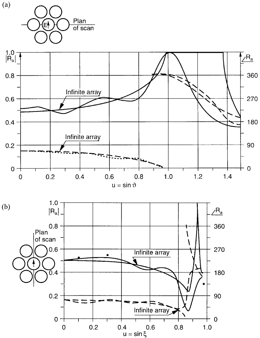
Figure 6.5 Active reflection coefficient of central element of a 127-element array. Infinite array data shown for comparison. Solid lines indicate magnitude, dashed lines indicate phase. Measured values indicated by dots. (a) H -plane scan; and (b) E -plane scan. (From: [38]. © 1974 IEEE. Reprinted with permission.)
