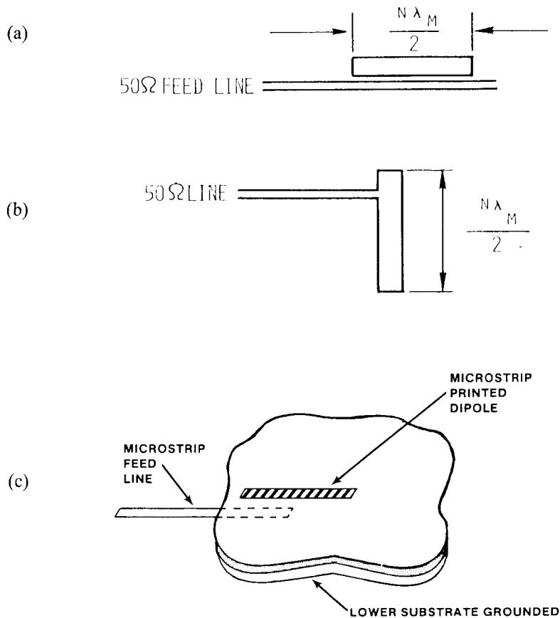
Figure 5.11 Microstrip dipoles for radiation perpendicular to substrate: (a) electromagnetic coupled microstrip dipole with coplanar feed; (b) microstrip dipole fed directly by microstrip line; and (c) electromagnetic coupled microstrip dipole with feed below substrate.
