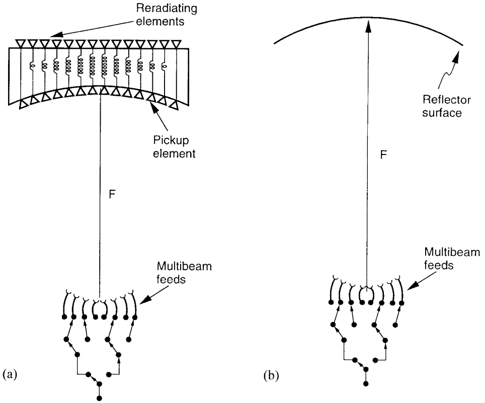
Figure 8.2 (a) Generic lens and (b) reflector multiple-beam systems.
