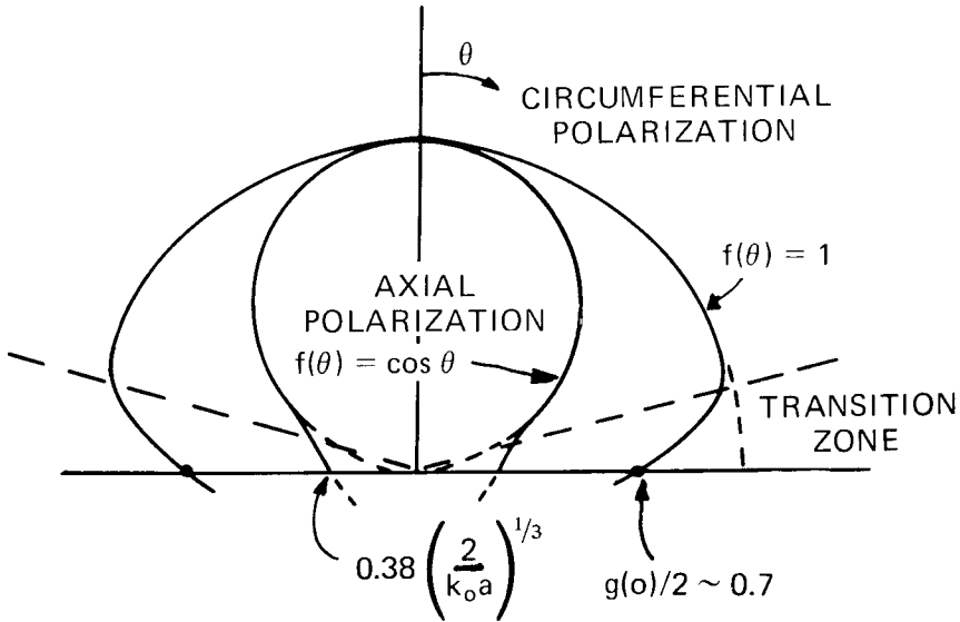
Figure 4.10 The approximate pattern of slot on cylinder of radius a for circumferential polarization [ f(\theta) = 1 ] and axial polarization [ f(\theta) = \cos(\theta) ].
