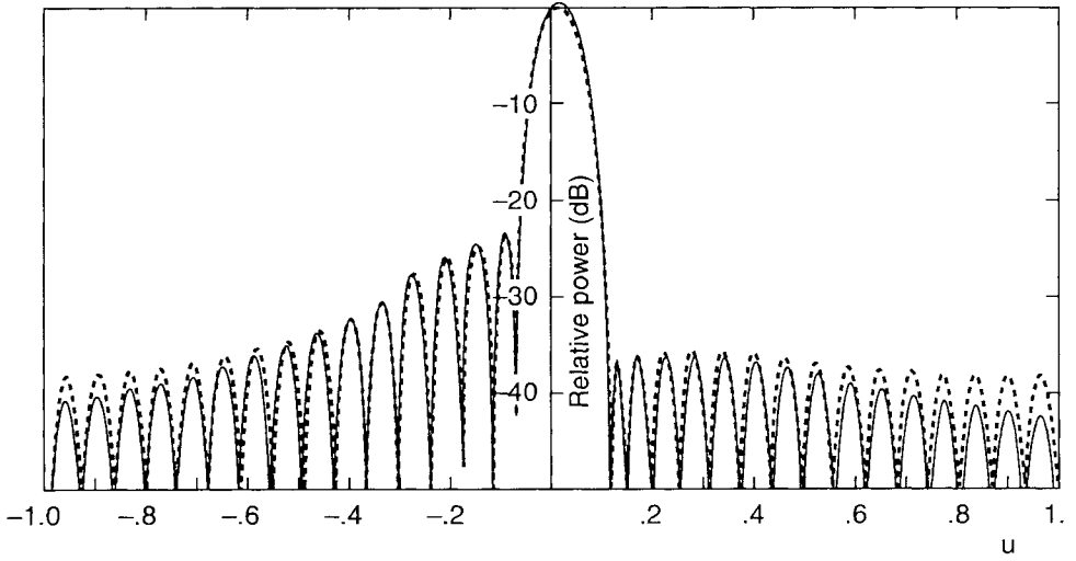
Figure 3.9 Modified Taylor pattern of Elliott. Pattern design for \bar{n}_L = 5 , \bar{n}_R = 7 with -20 -dB left sidelobes and -40 -dB right sidelobes (line pattern solid, array pattern dashed).
