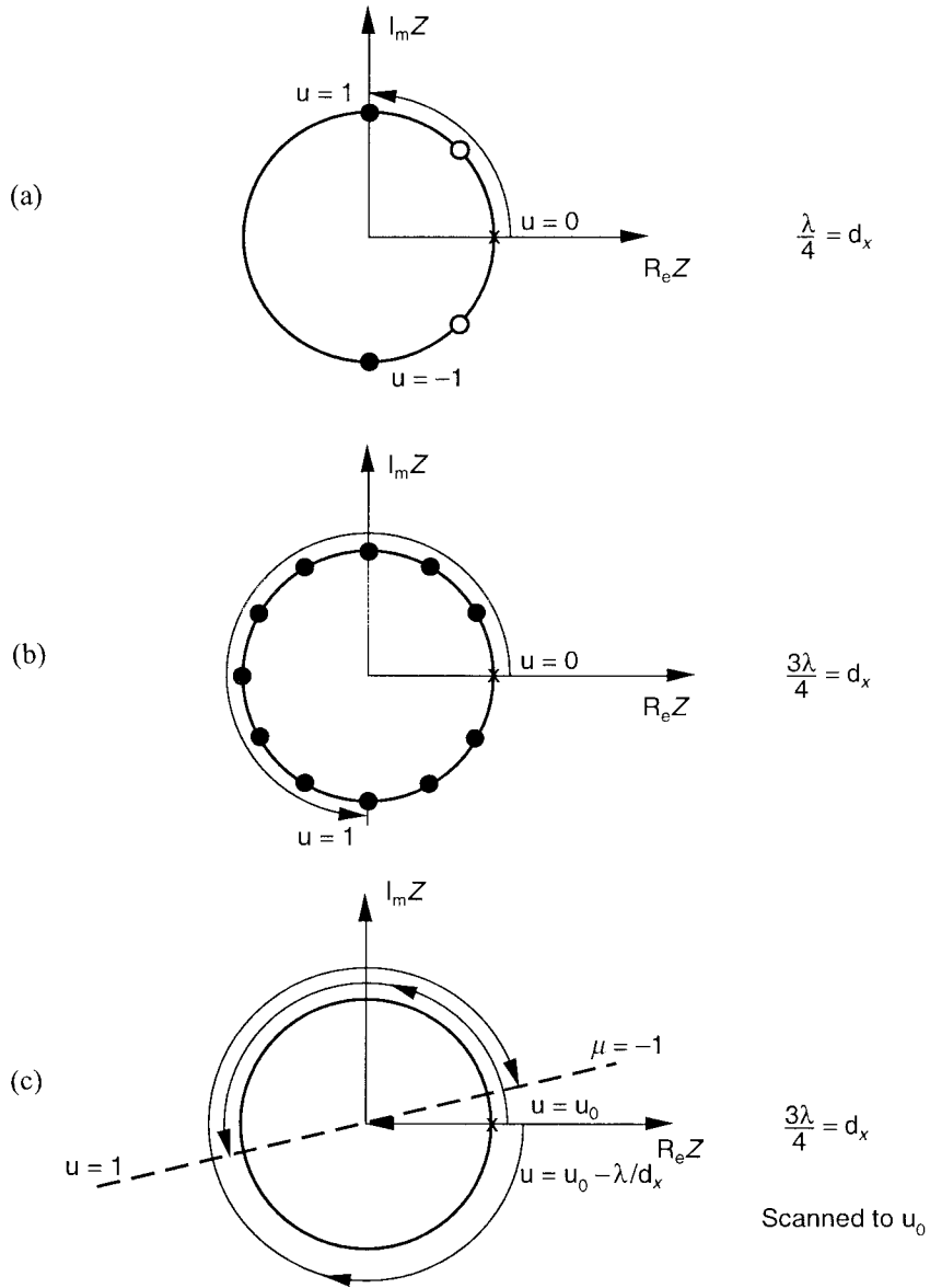
Figure 3.2 Schelkunov unit circle representation of complex root locations for an 8-element uniformly illuminated array: (a) root locations (circles) and path limits (arrow) for positive 0 \leq u \leq 1 with \lambda/4 spaced array; (b) path limit (arrow) for positive u ( 0 \leq u \leq 1 ) of array with 3\lambda/4 spacing; and (c) path limits (arrows) for array with 3\lambda/4 spacing scanned to u_0 ; clockwise arrow for u_0 \leq u \leq 1 , counterclockwise arrow for -1 \leq u \leq u_0 .
