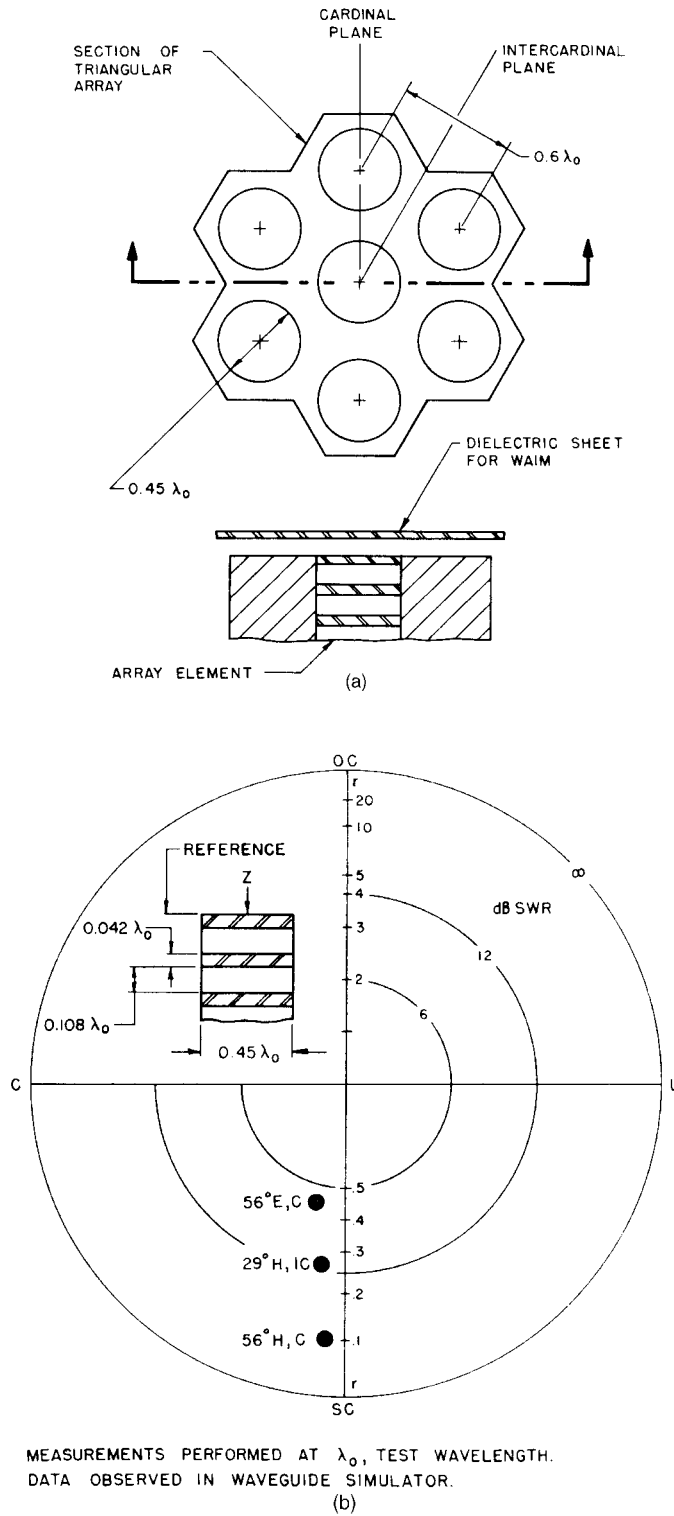
Figure 6.23 Dielectric WAIM sheets for scan matching: (a) array geometry; and (b) measured reflection of array element before impedance matching. (From: [81]. © 1966 IEEE. Reprinted with permission.)
