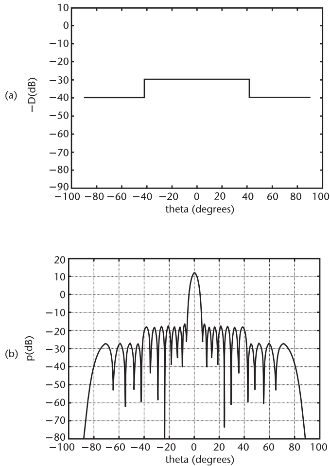
Figure 3.25 Synthesized pattern with -30 - and -40 -dB sidelobe levels: (a) desired level; and (b) resulting pattern. (From: [79]. © 1990 IEEE. Reprinted with permission.)
