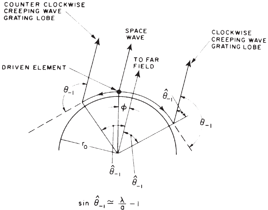
Figure 6.26 Wave contributions in forward (lit) region of element patterns of circular array on a conducting cylinder. (From: [85]. © 1972 Artech House, Inc. Reprinted with permission.)
