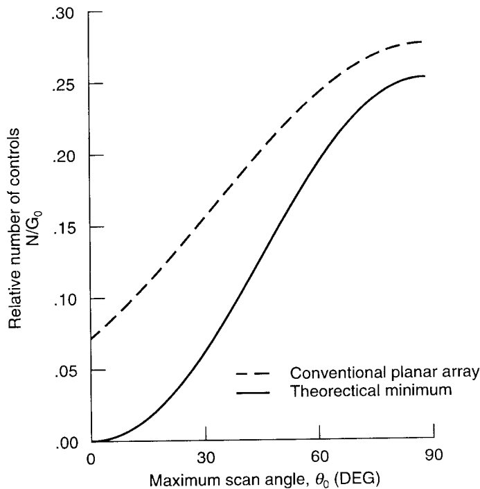
Figure 8.8 Number of controls needed to scan a conical volume. (After: [34].)
