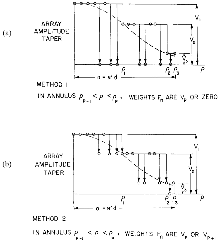
Figure 2.16 Thinning and quantizing geometries: (a) ideal taper (dashed) and method 1 source weight options; and (b) ideal taper (dashed) and method 2 source weight options. (From: [40]. © 1991 IEEE. Reprinted with permission.)
