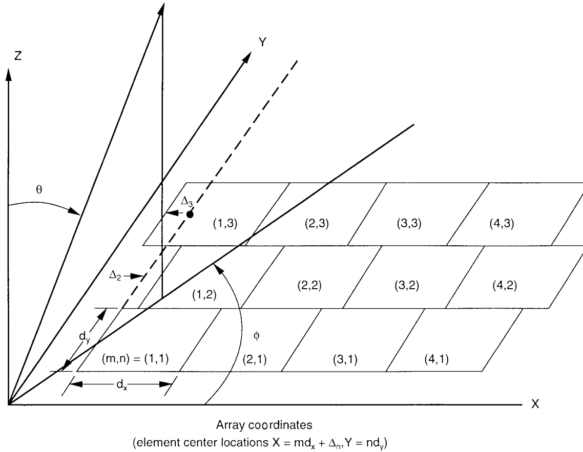
Figure 2.11 Array grating with displaced rows.
