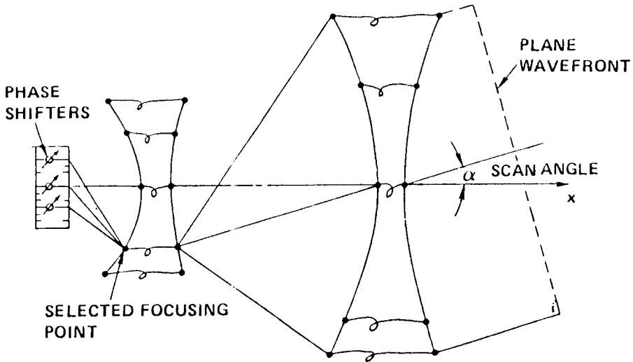
Figure 8.31 Dual-lens limited field-of-view system. (After: [75].)
