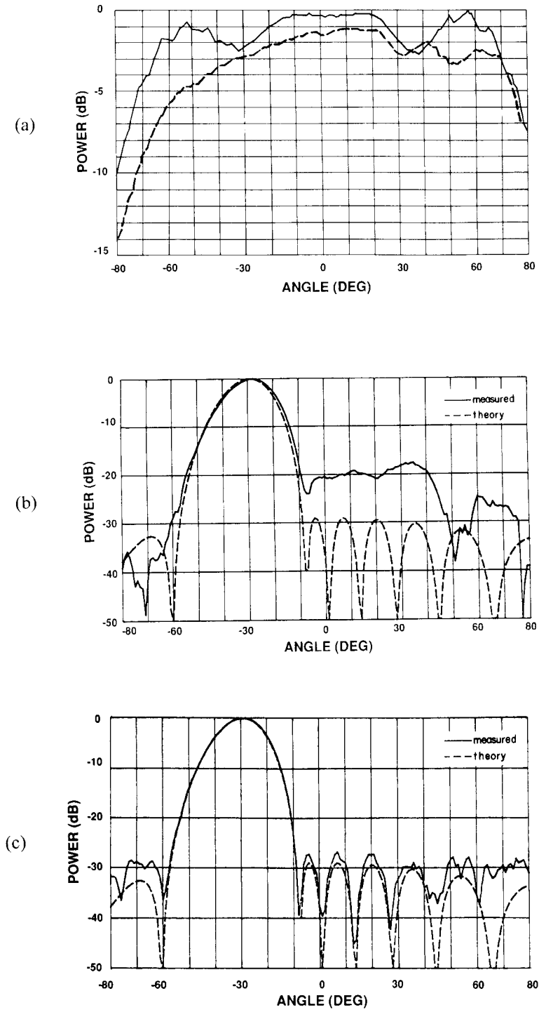
Figure 3.26 Pattern control using measured element patterns: (a) the measured pattern magnitudes for center (solid line) and edge (dashed line) elements in an 8-element array; (b) 30-dB Chebyshev patterns without coupling compensation (solid line = measured; dashed line = theory; dashed line is ideal); and (c) 30-dB Chebyshev patterns with coupling compensation. Dashed pattern is ideal. (From: [80]. © 1990 IEEE. Reprinted with permission.)
