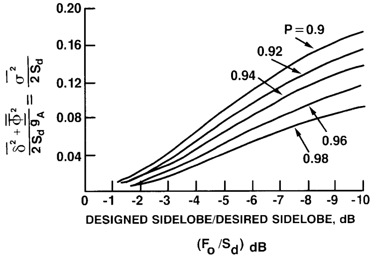
Figure 7.3 Normalized array error, or normalized residual sidelobe level, versus designed to desired sidelobe level ratio. (After: [7, 8].)
