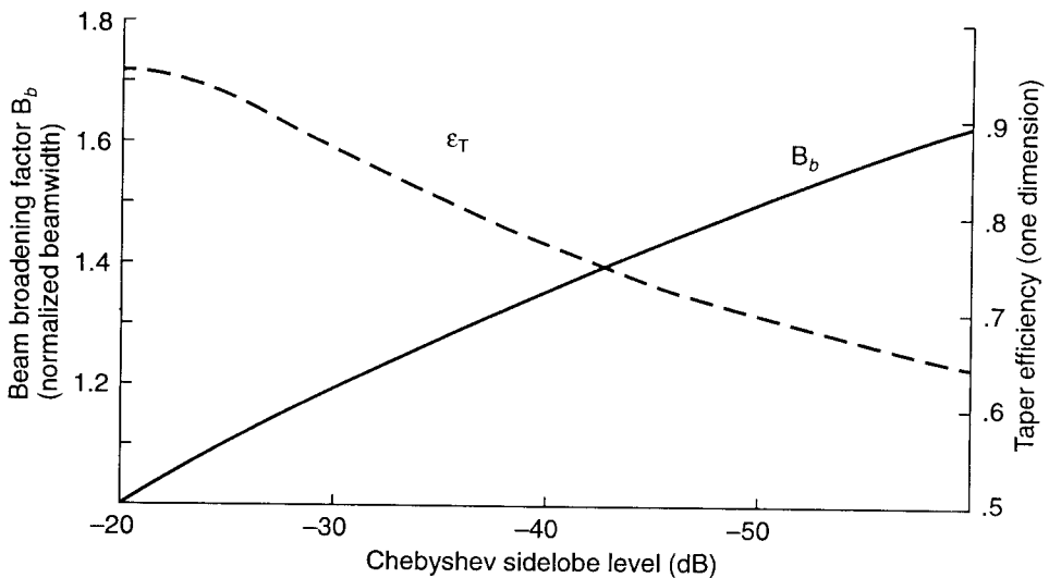
Figure 1.9 Beam broadening (solid line) and taper efficiency (dashed line) versus sidelobe level.
