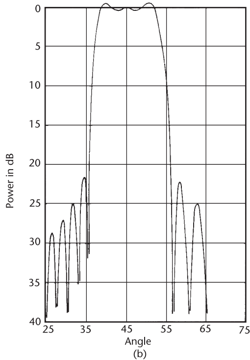
Figure 8.32 Dual-transform (overlapped subarray) system using space-fed lens and transform feed: (a) geometry showing feed array near-field patterns of several subarray input terminals; and (b) subarray pattern (scanned off axis by phase shifters in lens). (From: [29]. © 1972 Artech House, Inc. Reprinted with permission.)
