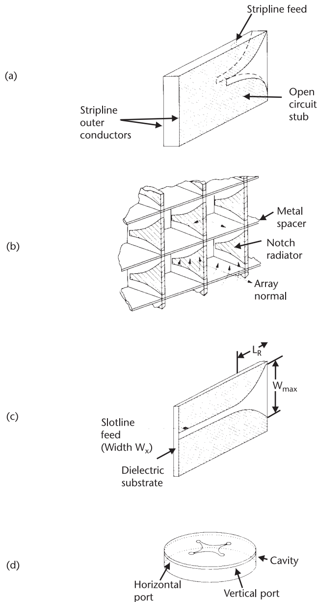
Figure 5.13 Notch type radiators: (a) flared-notch strip line-fed radiator; (b) two-dimensional flared-notch array; and (c) Vivaldi slot line element. (After: [64].) (d) Cavity-backed arrangement of four microstrip-fed flared slot lines. (After: [68].)
