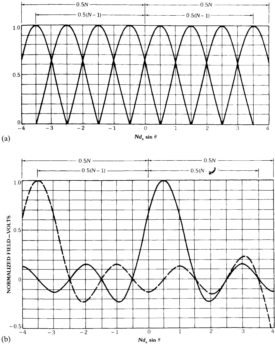
Figure 3.3 Synthesis method of Woodward and Lawson: (a) orthogonal Woodward beams for array of N elements (plotted to first zeros); (b) two orthogonal beams (plotted over domain of orthogonality) with i = 1/2 (solid) and i = -7/2 (dashed); and (c) pulse-shaped pattern of Figure 3.1 synthesized by Woodward procedure (solid curve for ideal and pattern of 16-element array, dashed curve for 8-element array). (From: [10]. © 1988 Van Nostrand Reinhold, Inc. Reprinted with permission.)
