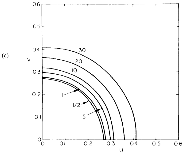
Figure 8.13 Metallic grid angular filter geometry: (a) metal grid filter; (b) equivalent circuit of metal grid filter; and (c) passband characteristics of metal grid filter (numbers are in decibels).
