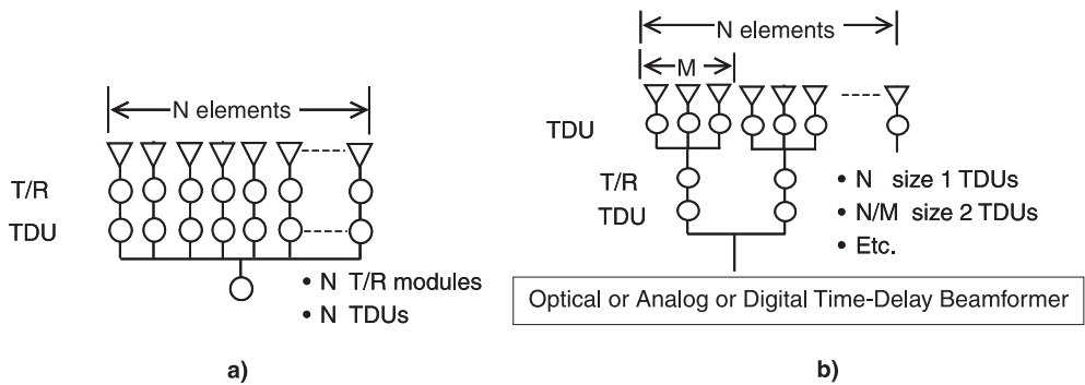
Figure 1.24 Wideband array control: (a) array with TDUs; and (b) array with cascaded TDUs.
