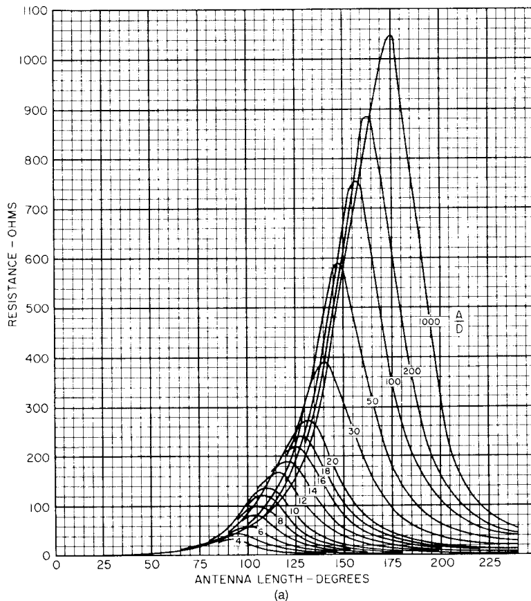
Figure 5.4 Impedance characteristics of monopole antennas: (a) monopole resistance versus length A , for diameter D ; and (b) monopole reactance versus length A . (From: [7]. © 1952 RCA Review. Reprinted with permission.)
