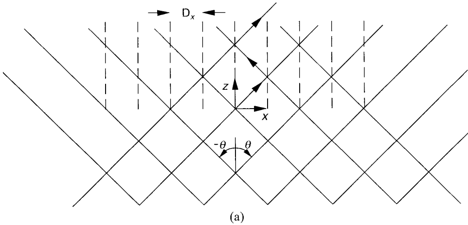
Figure 6.28 Waveguide simulator geometries. (a) Basic TE 10 mode simulator; (b) equivalent infinite array represented by simulator; and (c) higher order TE 10 mode simulator.
