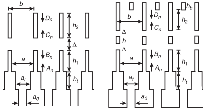
Figure 8.17 Arrays of dual-mode waveguides for scanning in the E -plane (left) and H -plane (right). (From: [42]. © 1998 IEEE. Reprinted with permission.)
