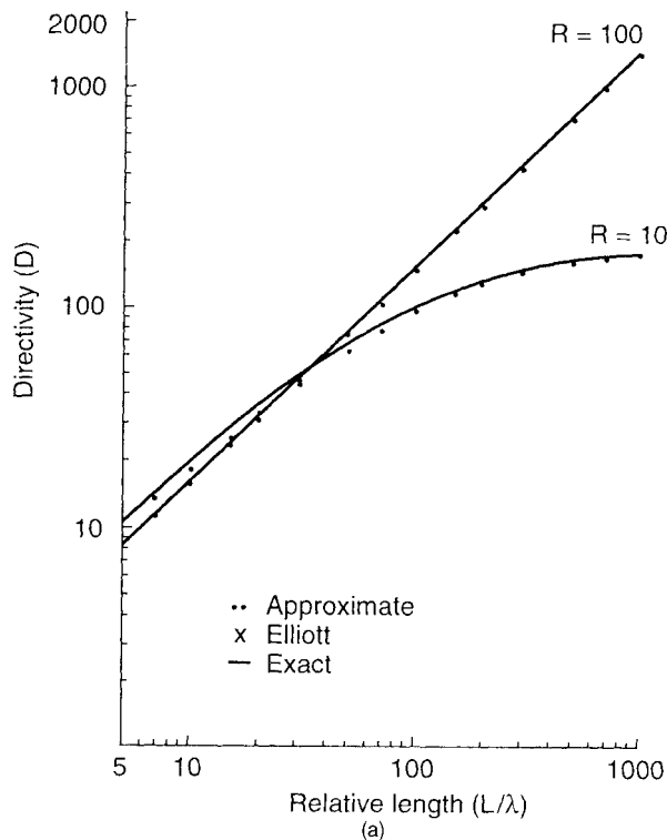
Figure 3.5 Characteristics of Chebyshev patterns: (a) Array directivity versus length for -20 -dB ( R = 10 ) and -40 -dB ( R = 100 ) sidelobe arrays: comparison between approximation of Drane (....), Elliott (xxxx), and exact values. (From: [17]. © 1968 IEEE. Reprinted with permission.) (b) Array directivity versus length. Note: text uses L in place of Elliott's Lz ; sidelobe levels are -15 to -60 dB. (From: [18]. © 1966 Academic Press, Inc. Reprinted with permission.) (c) Array beamwidth versus length for -20 - and -40 -dB sidelobe arrays: comparison between approximation of Drane, Elliott, and exact values. (From: [17]. © 1968 IEEE. Reprinted with permission.) (d) Taper efficiency \epsilon_T = D/N_T versus sidelobe level.
