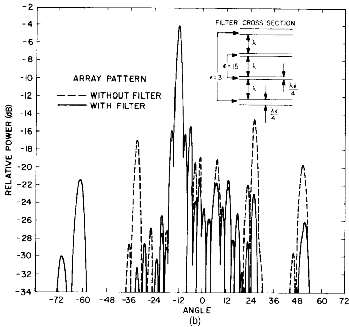
Figure 8.14 Limited field-of-view array: (a) test array with dielectric angular filter; and (b) scanned array pattern with and without dielectric filter (element spacing 2.9\lambda ).
