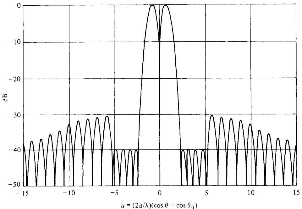
Figure 3.11 Iterated difference pattern of Elliott. Pattern has four inner sidelobes symmetrically depressed. (From: [26]. © 1976 IEEE. Reprinted with permission.)
