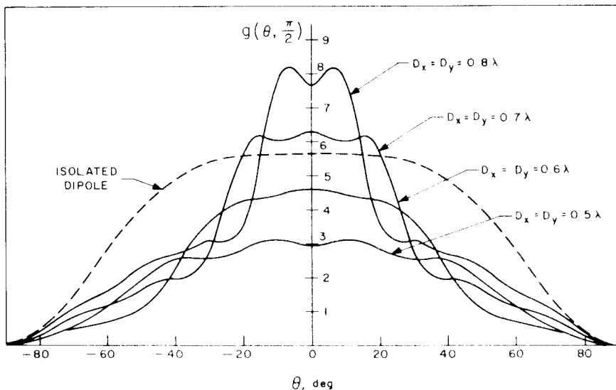
Figure 6.1 H -plane element gain functions for a center element of a 7-by-9-element dipole array ( \lambda/2 dipoles, \lambda/4 above ground.) Element spacings denoted D_x and D_y . Note: dashed curve is for isolated dipole over ground. (From: [6]. © 1966 Academic Press, Inc. Reprinted with permission.)
