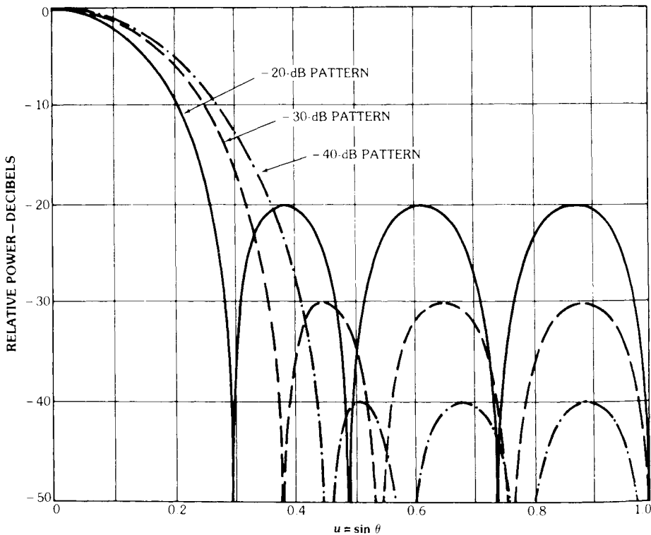
Figure 3.4 Patterns of Dolph-Chebyshev arrays with eight elements ( -20 -, -30 -, -40 -dB sidelobes). (From: [10]. © 1988 Van Nostrand Reinhold, Inc. Reprinted with permission.)
