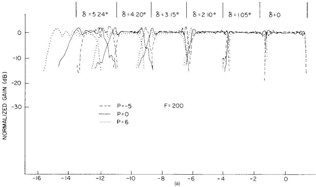
Figure 8.37 Radiation characteristics of off-axis transform-fed lens: (a) subarray patterns for off-axis feeds; and (b) maximum sidelobe radiation level for scanned feeds at fixed offset angles.
