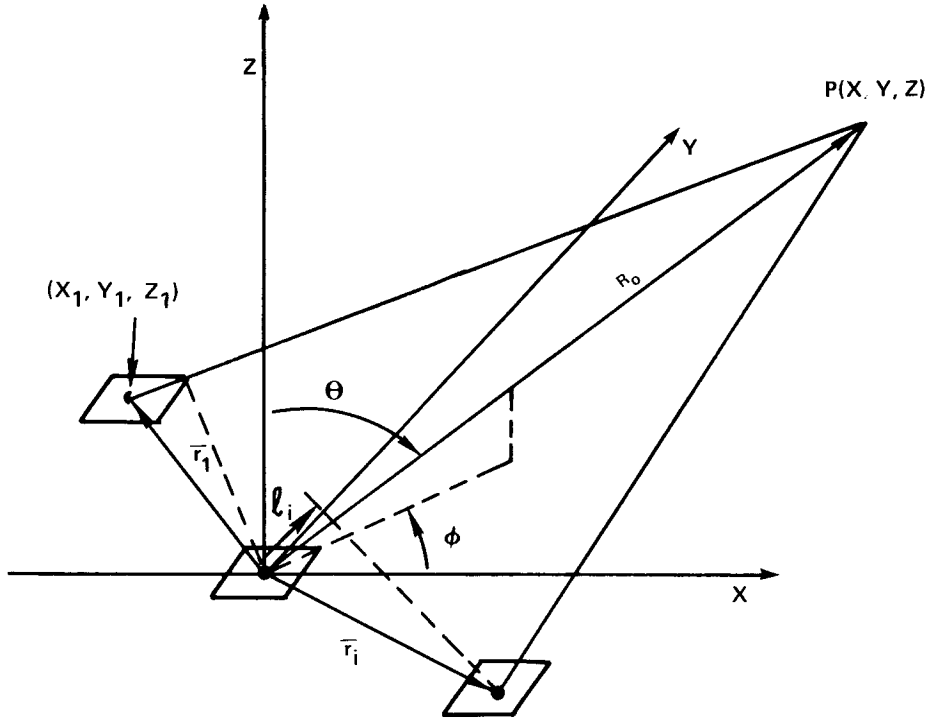
Figure 1.5 Generalized array configuration.
