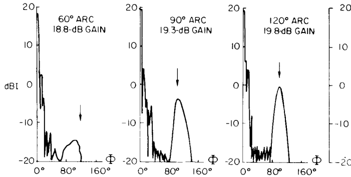
Figure 4.15 Radiation characteristics of sector arrays. Maximum gain E-plane patterns for sector array of ka = 86 , b/\lambda = 0.65 . Arrays occupy sectors of 60^\circ , 90^\circ , and 120^\circ [assumed \cos(\phi - \phi_n) element pattern]. (From: [41]. © 1972 Artech House, Inc. Reprinted with permission.)
