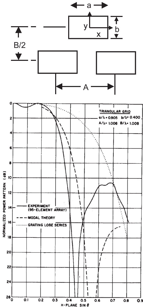
Figure 6.6 Array power pattern ( H -plane scan of triangular grid array). (From: [20]. © 1968 IEEE. Reprinted with permission.)
