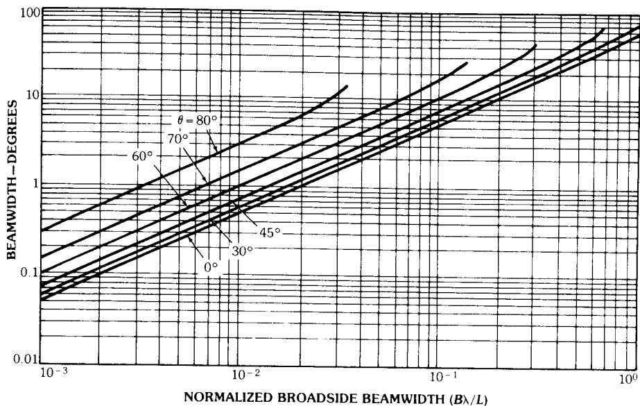
Figure 1.10 Beamwidth variation with scan.
