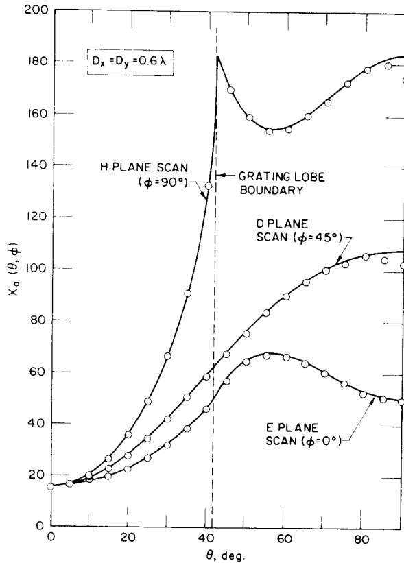
Figure 6.17 Variation in active reactance as a function of scan angle for three different planes of scan and for array of \lambda/2 dipoles mounted \lambda/4 over a ground screen. Solid lines from infinite array theory. Circles from element-by-element calculation for 65 \times 149 -element array. (From: [6]. © 1966 Academic Press, Inc. Reprinted with permission.)
