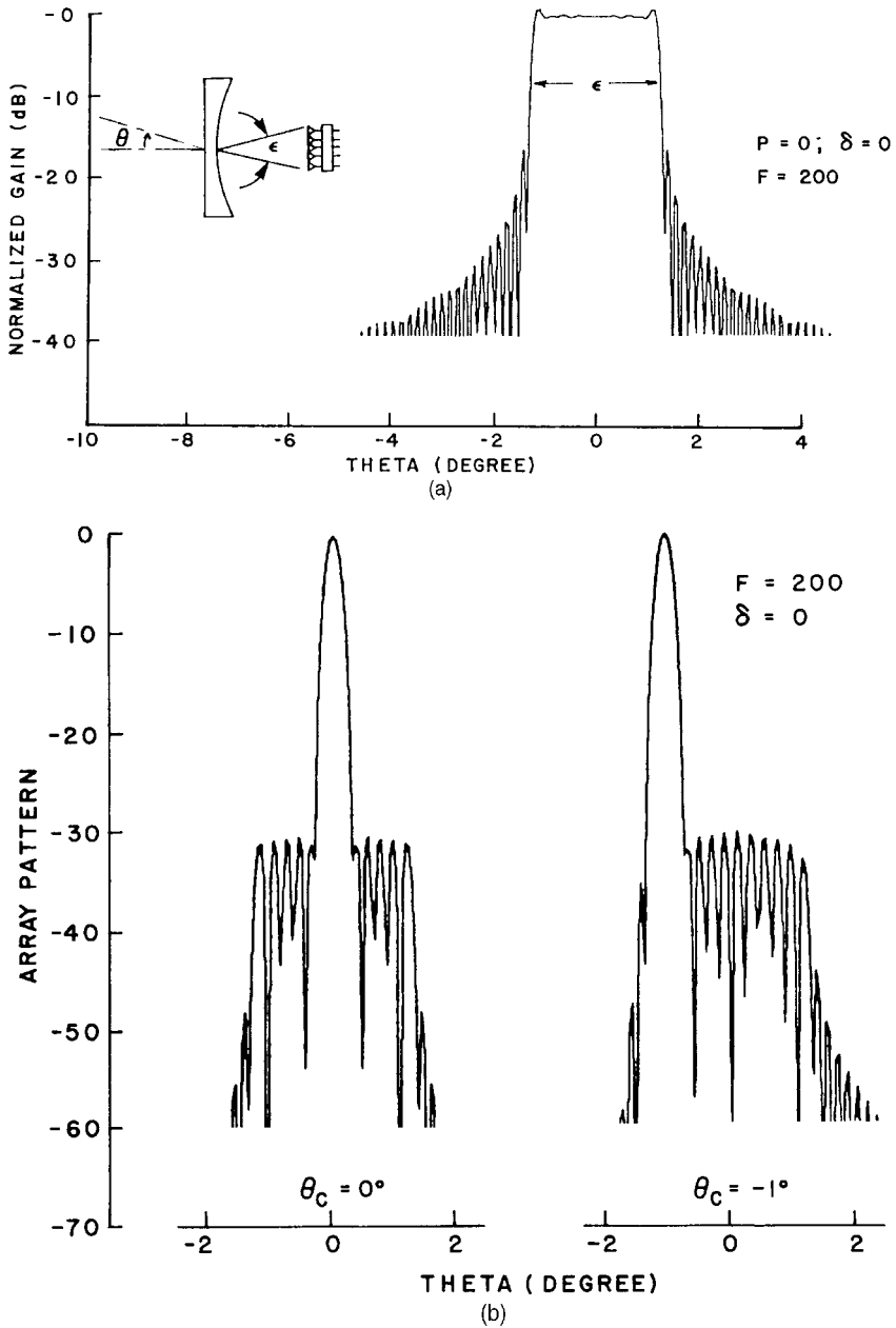
Figure 8.35 Limited field-of-view characteristics of cylindrical lens with dimensions (normalized to wavelength) L = 363.2 ; F = 200 ; array size 12 elements ( 6\lambda ): (a) subarray pattern; and (b) broadside and scanned patterns. (From: [79]. © 1983 IEEE. Reprinted with permission.)
