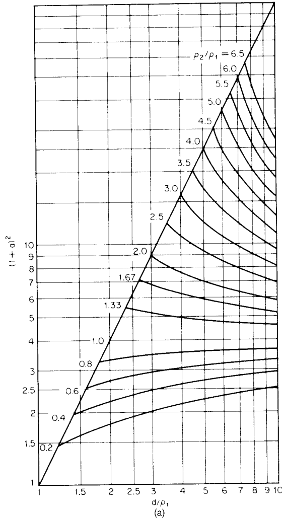
Figure 5.10 Folded dipole parameters: (a) step-up ratio (1 + a)^2 versus \rho_2/\rho_1 and d/\rho_1 ; and (b) conductor ratio \rho_2/\rho_1 versus step-up ratio (1 + a) and d/\rho_1 . (From: [42]. © 1982 IEEE. Reprinted with permission.)
