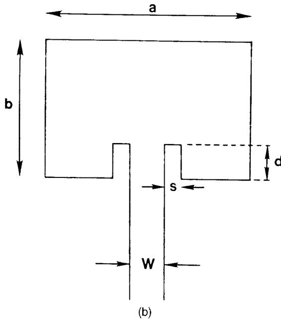
Figure 5.21 Microstrip patch antenna with inset feed: (a) edge input impedance versus patch length b ; and (b) inset feed geometry (substrate thickness h not shown).
