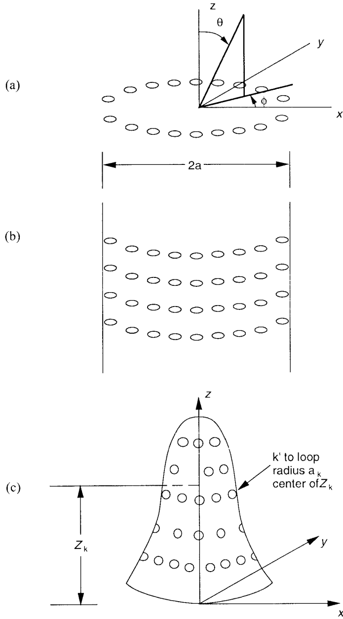
Figure 4.2 Circular and cylindrical array geometries: (a) circular array; (b) cylindrical array; and (c) generalized array conformed to a body of revolution.
