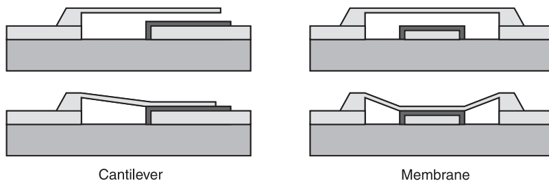
Figure 1.30 Microelectromechanical switches.
