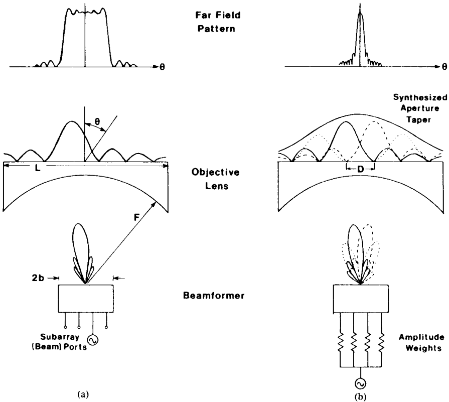
Figure 8.33 Completely overlapped subarray (dual transform) lens perspective: (a) feed illumination and radiated subarray pattern; and (b) synthesized aperture taper and array radiation pattern. (From: [77]. © 1986 IEEE. Reprinted with permission.)
