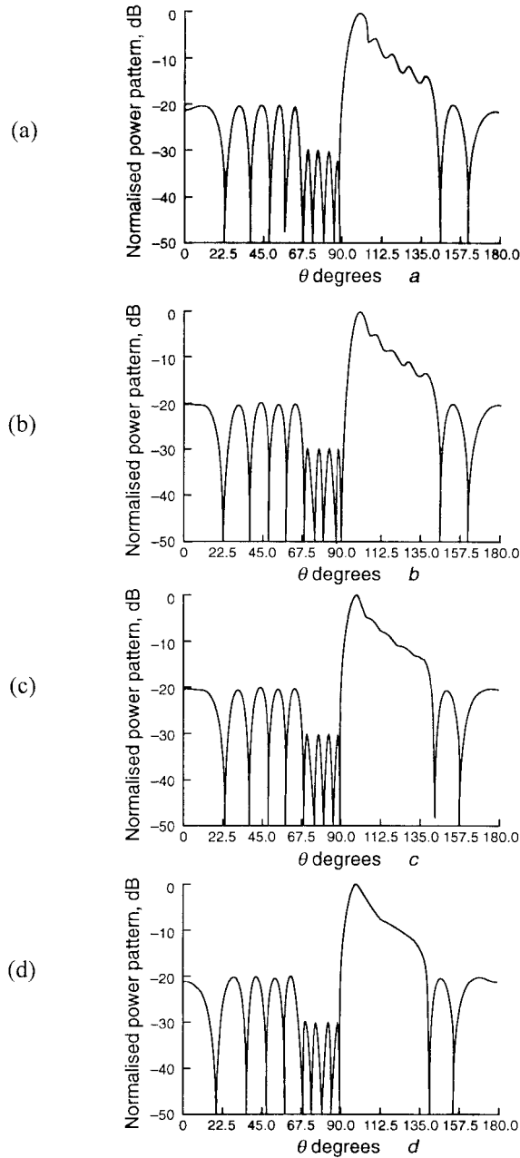
Figure 3.14 Representation of shaped beam with \csc^2 \theta \cos \theta pattern with a 16-element array; d = \lambda/2 . Ripple requirement: (a) \pm 1.5 dB; (b) \pm 1.0 dB; (c) \pm 0.5 dB; and (d) \pm 0.1 dB. (From: [33]. © 1984 IEEE. Reprinted with permission.)
