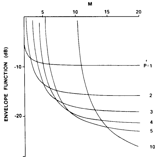
Figure 7.8 Envelope function (decibels) versus number of elements M in subarray with p' as parameter. (From: [16]. © 1984 IEEE. Reprinted with permission.)
