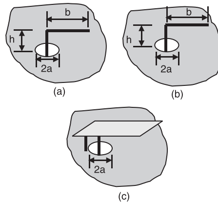
Figure 5.12 Low-profile wire elements: (a) ILA; (b) IFA; and (c) PIFA.
