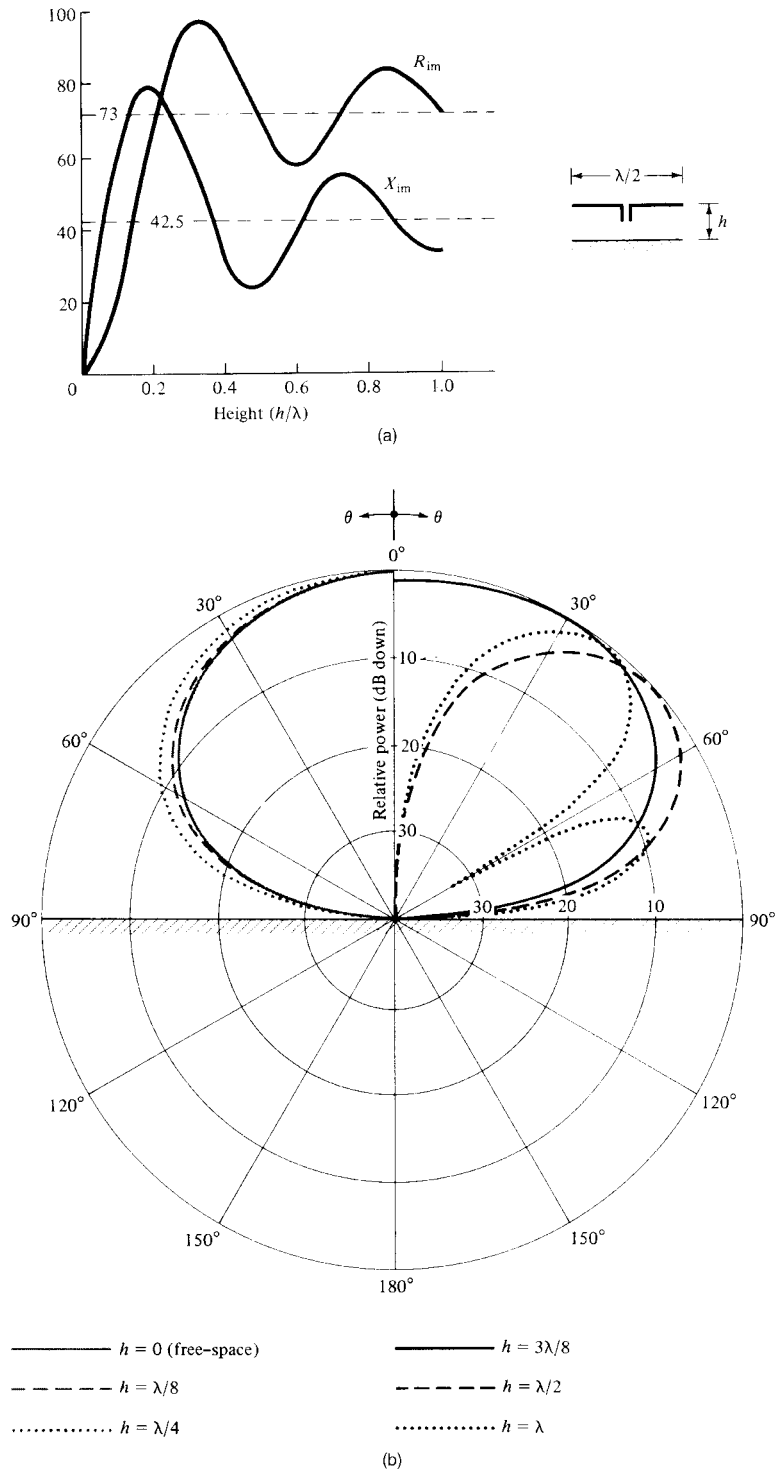
Figure 5.6 Impedance and elevation pattern of horizontal dipole over ground screen. (a) Impedance of horizontal \lambda/2 dipole versus height h above ground. (From: [14]. © 1968 McGraw-Hill, Inc. Reprinted with permission.) (b) Elevation patterns of horizontal infinitesimal dipole versus height h . (From: [15]. © 1997 Harper and Row, Inc. Reprinted with permission.)
