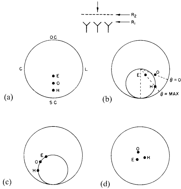
Figure 6.24 Calculation procedure for matching with thin high- k dielectric sheet. (a) Array at R_1 ; (b) array at R_2 ; (c) dielectric WAIM sheet; and (d) array with sheet at R_2 . (From: [81]. © 1966 IEEE. Reprinted with permission.)
