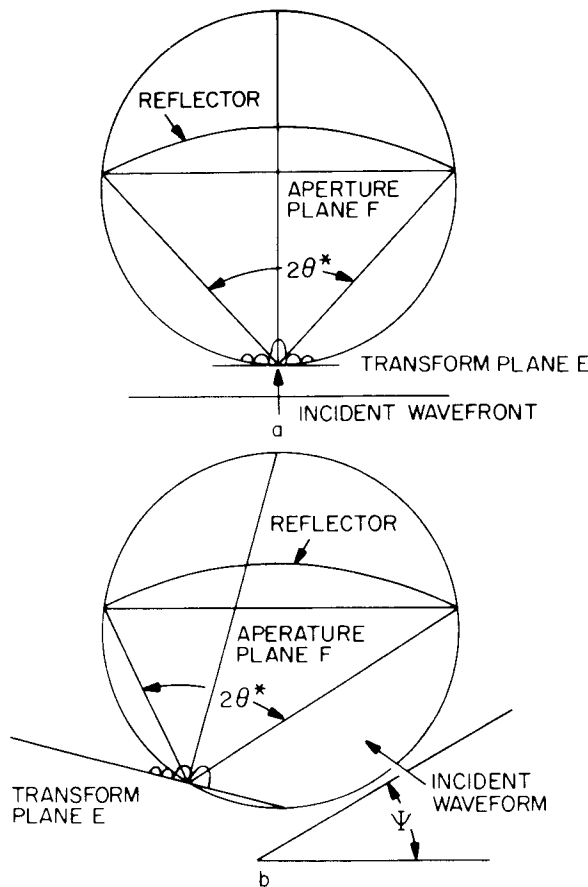
Figure 8.27 (a, b) The focal region fields of a parabola along a circular arc for several incident wave angles. (From: [66]. © 1969 IEE. Reprinted with permission.)
