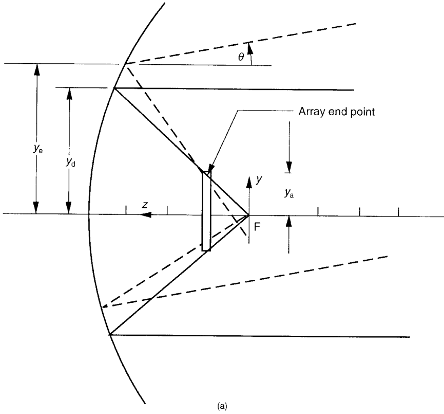
Figure 8.26 Reflector scanned by array: (a) reflector and array geometry showing ray locations for full array utilization (solid line for on-axis beam, dashed for scanned beam); and (b) normalized array size y_e/y_d versus scan angle for oversize ratio R = y_e/y_d . (From: [65]. © 1982 Peter Peregrinus, Ltd. Reprinted with permission.)
