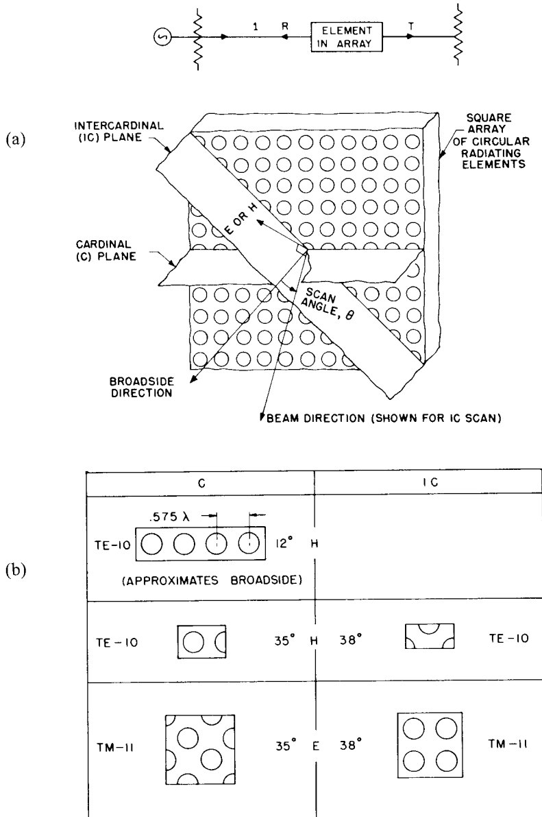
Figure 6.29 Simulator geometries and scan plane definitions: (a) cardinal and intercardinal planes; and (b) a collection of five simulators for arrays of circular waveguides. (From: [100]. © 1965 IEEE. Reprinted with permission.)
