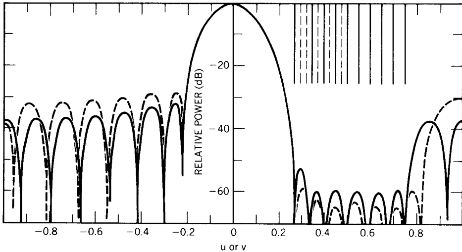
Figure 3.20 Adapted pattern of a 16-element array with quiescent -40 -dB Chebyshev pattern. Response to 10 (solid line) and 15 (dashed line) interfering sources. (From: [66]. © 1989 John Wiley and Sons, Inc. Reprinted with permission.)
