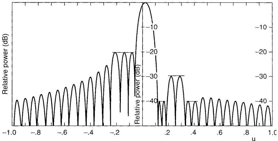
Figure 3.10 Iterated sum pattern of Elliott. Pattern design for \bar{n}_L = 4 , \bar{n}_R = 7 (solid horizontal lines indicate constrained sidelobe levels).
