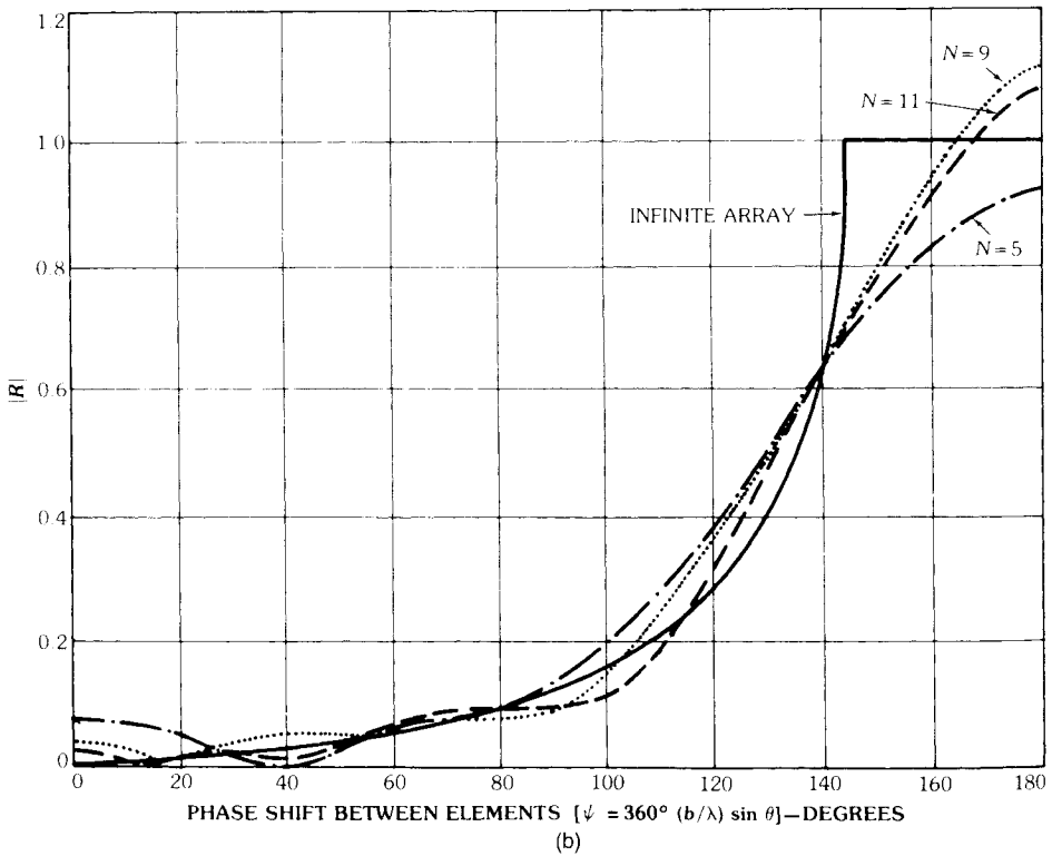
Figure 2.6 (a) Element pattern P(\theta) and reflection coefficient R of center element in unloaded waveguide array [ b\lambda = a/\lambda = 0.4 ]: radiation patterns. (b) Element pattern P(\theta) and reflection coefficient R of center element in unloaded waveguide array [ b\lambda = a/\lambda = 0.4 ]: reflection coefficients. (From: [6]. © 1970 IEEE. Reprinted with permission.)
