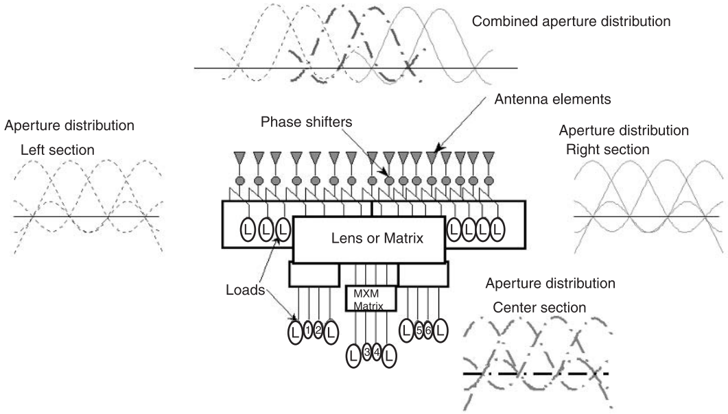
Figure 8.44 Network realization of modular feed for partial overlapping of transform feeds (without synthesis). (From: [84]. © 2001 IEEE. Reprinted with permission.)
