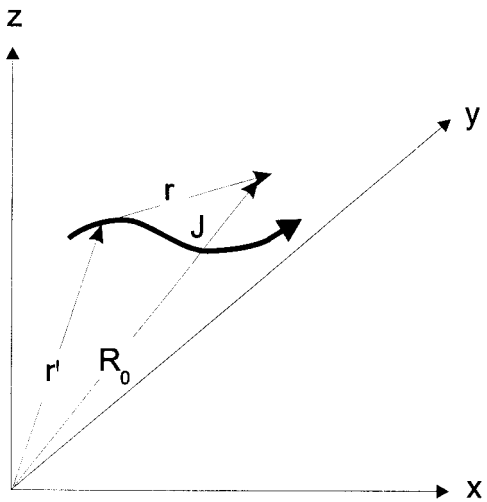
Figure 2.1 Radiation from electric and magnetic current sources.
