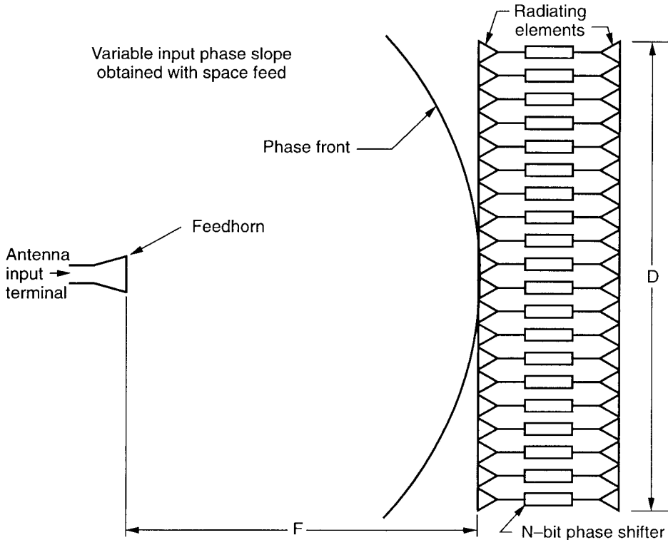
Figure 7.9 Variable input phase slope obtained with space feed. (After: [17].)
