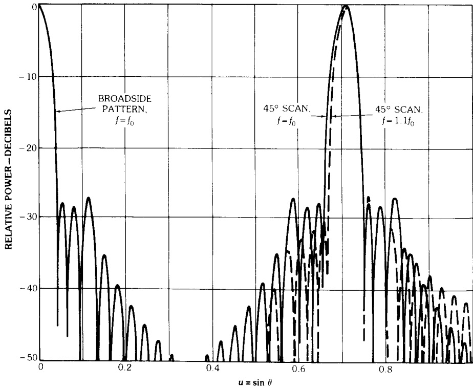
Figure 8.42 Pattern characteristics of 64-element array fed by overlapped subarray beamformer.
