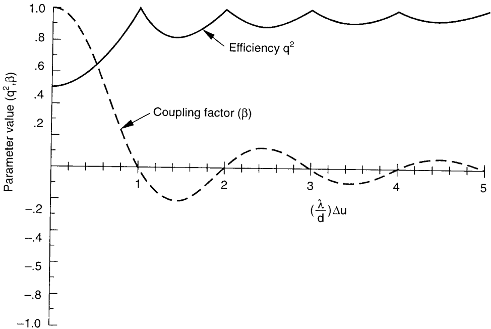
Figure 8.4 Orthogonality loss in two-beam system.
