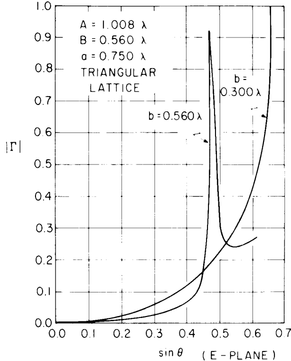
Figure 6.9 Blindness location versus waveguide aperture size with constant lattice spacing. (From: [39]. © 1968 IEEE. Reprinted with permission.)
