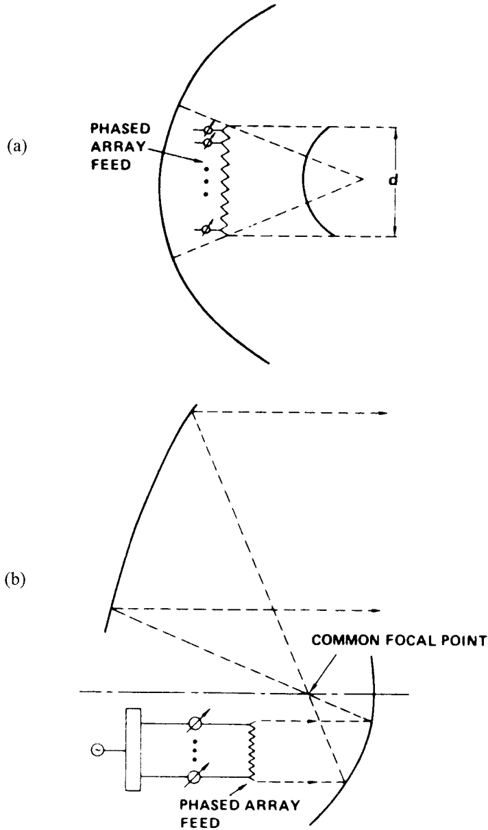
Figure 8.28 Dual-reflector systems for limited field of view: (a) near-field Cassegrainian geometry; and (b) offset-fed Gregorian geometry. (After: [67, 68].)
