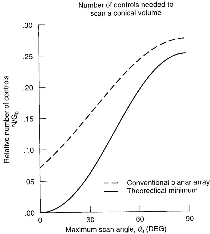
Figure 1.18 Required controls for arrays with limited field of view.
