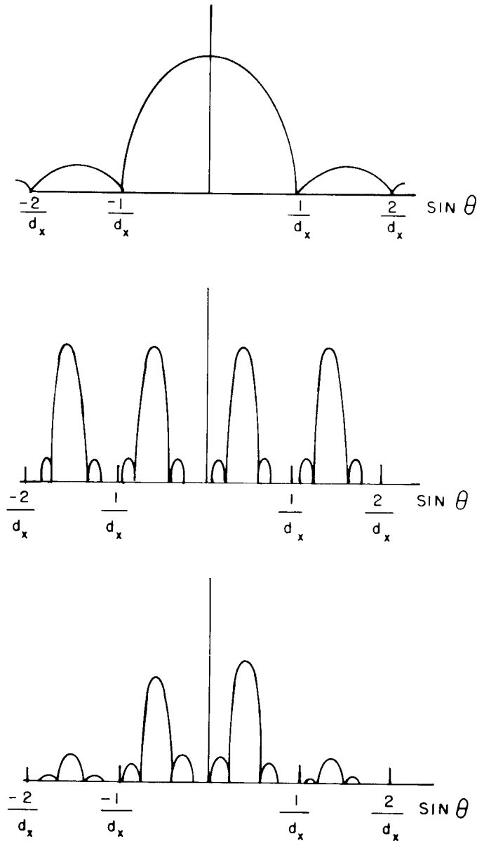
Figure 8.9 Element pattern (top), array factor (middle), and array pattern (bottom) for E -plane uniformly illuminated (horn) aperture.
