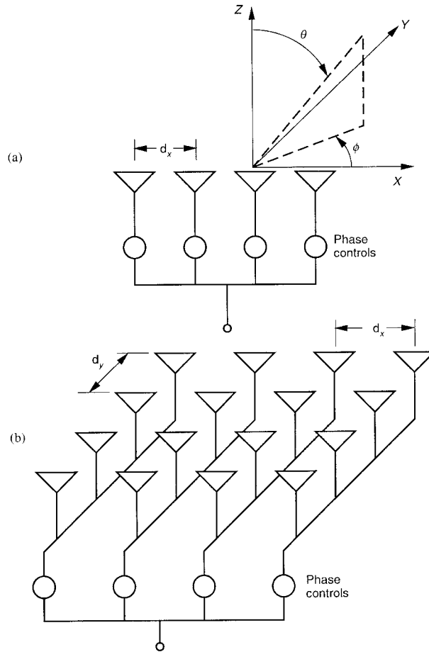
Figure 1.6 Array geometries for scanning in one plane: (a) individual radiators; and (b) columns of elements.
