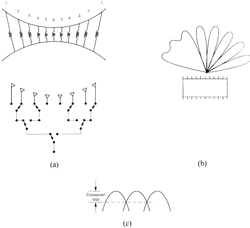
Figure 8.1 Multiple-beam antenna systems: (a) basic multiple-beam antenna and switching tree for eight-beam system; (b) combined shaped and pencil beam system; and (c) beam crossover.
