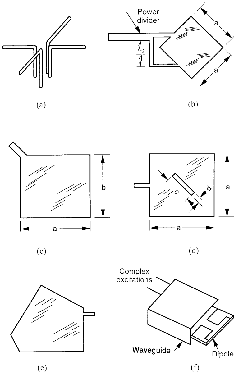
Figure 5.28 Elements for radiating circular polarization. (a) Crossed dipole element for radiating both circular polarizations. (b) Circularly polarized microstrip patch, orthogonal feeds. (c) Circularly polarized microstrip patch. (From: [106]. © 1981 IEEE. Reprinted with permission.) (d) Circularly polarized microstrip patch. (After: [153].) (e) Circularly polarized microstrip patch. (From: [154]. © 1975 IEEE. Reprinted with permission.) (f) Dipole slot circularly polarized element. (After: [155].)
