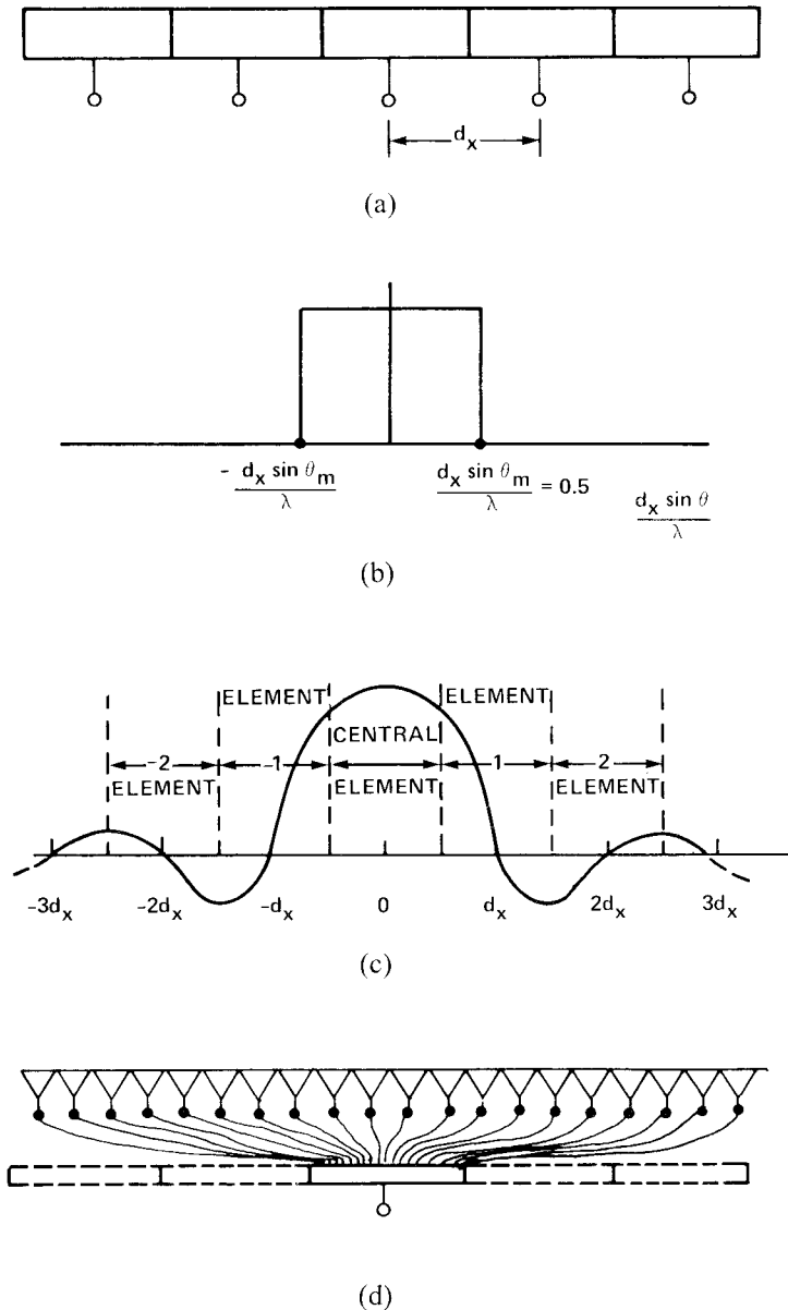
Figure 8.10 Element or subarray aperture distribution for ideal limited field-of-view scanning system: (a) oversized elements of subarrays for limited scan; (b) ideal element pattern for limited scan system ( \cos \theta suppressed); (c) subarray distribution for scan to (d_x/\lambda) \sin \theta = 0.5 ; and (d) overlapped feed distribution network.
