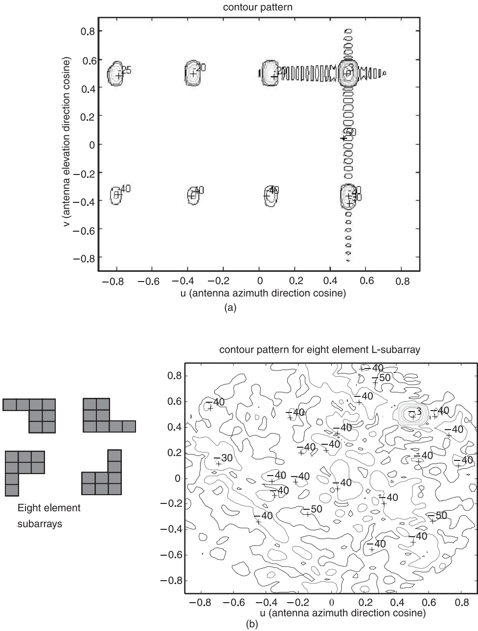
Figure 8.21 Arrays of regular and irregular subarrays: (a) contour pattern of array with 256 periodic rectangular subarrays at f = 1.03f_0 ; and (b) contour pattern of array with 256 irregular subarrays at f = 1.03f_0 .
