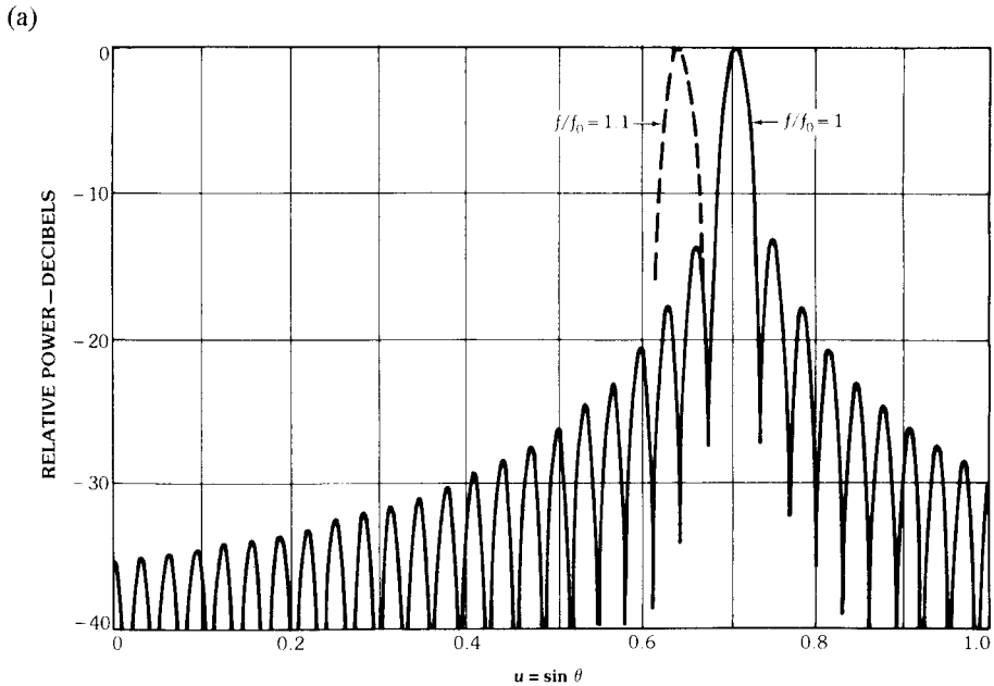
Figure 8.41 Broadband characteristics of an array of contiguous subarrays. (a) Pattern of uniformly illuminated array organized with phase shift steering. (b) Pattern of 64-element array with eight contiguous subarrays. (c) Grating lobe levels for phased arrays with time-delayed contiguous subarrays. (From: [82]. © 1984 IEEE. Reprinted with permission.)
