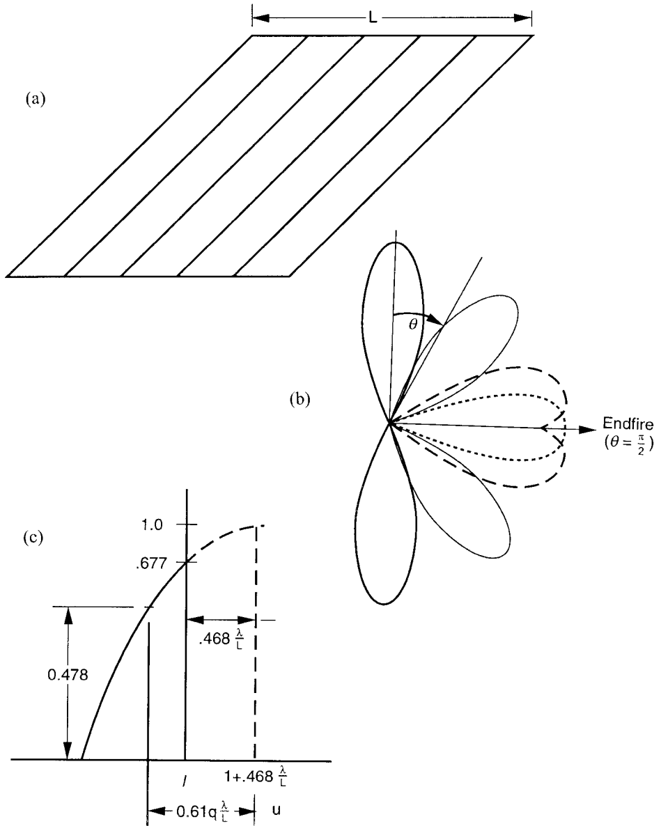
Figure 2.12 Scanning to endfire: (a) array of directive elements; (b) beam shape near horizon; and (c) conditions for Hansen-Woodyard endfire gain.
