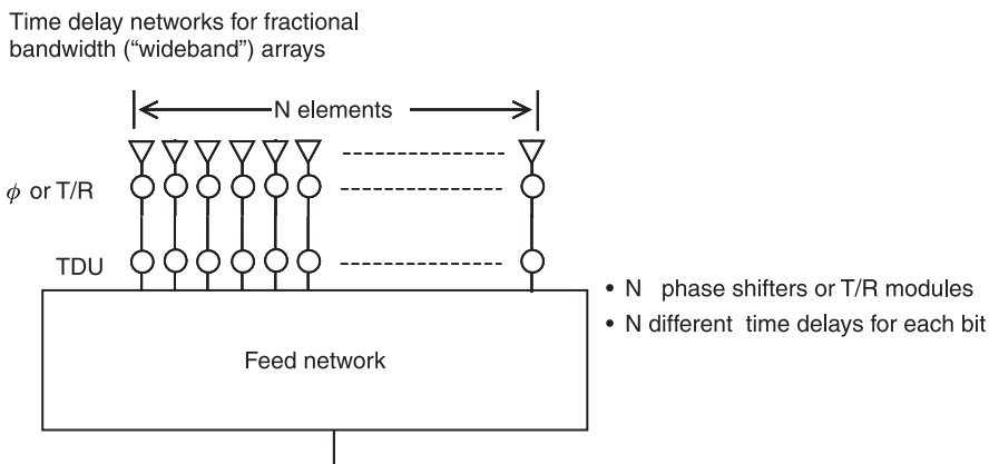
Figure 1.26 Network for scanning about fixed time delays.
