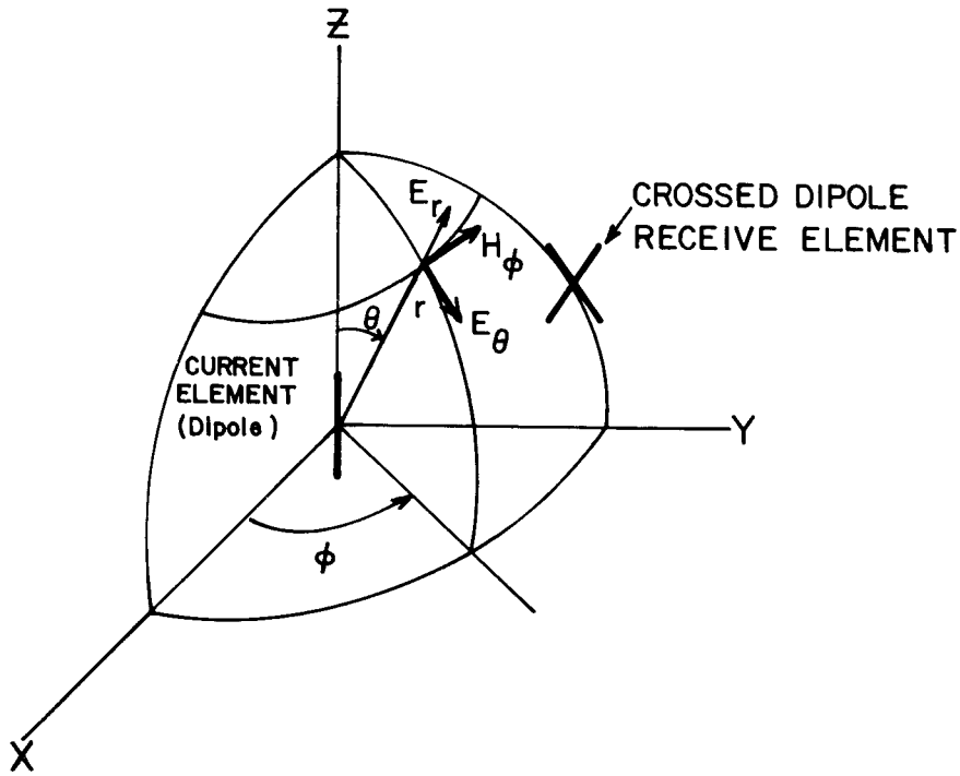
Figure 1.3 Polarization characteristics of ideal dipole antenna.
