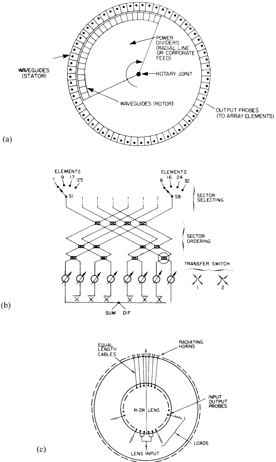
Figure 4.6 Commutating networks for circular and cylindrical arrays. (a) Waveguide commutator. (b) Switch network. (From: [30]. © 1969 IEEE. Reprinted with permission.) (c) R-2R Lens. (From: [31]. © 1970 IEEE. Reprinted with permission.)
