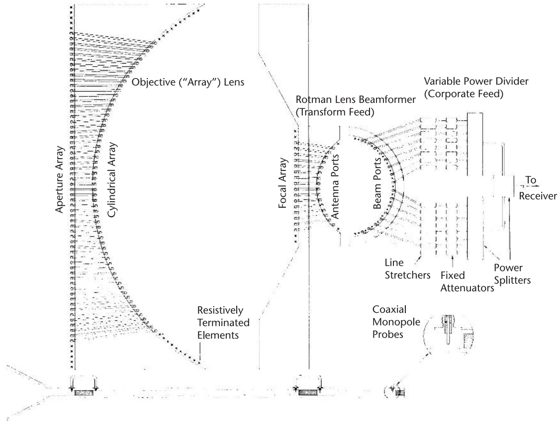
Figure 8.38 Antenna layout drawing of cylindrical lens fed by Rotman lens beamformer. (From: [77]. © 1986 IEEE. Reprinted with permission.)
