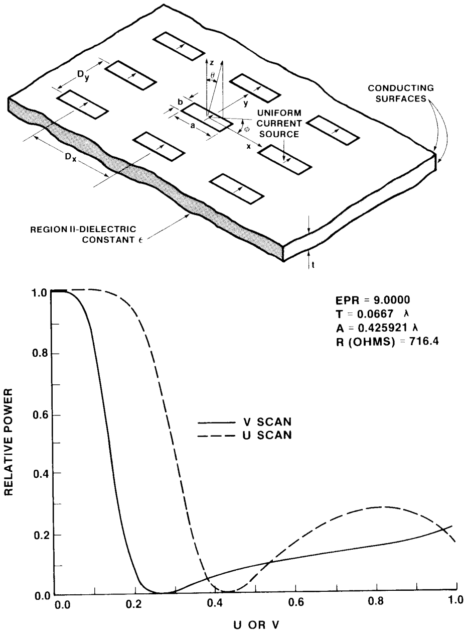
Figure 6.14 Geometry (top) and performance (bottom) of slot arrays without cavities. (From: [51]. © 1987 IEEE. Reprinted with permission.)
