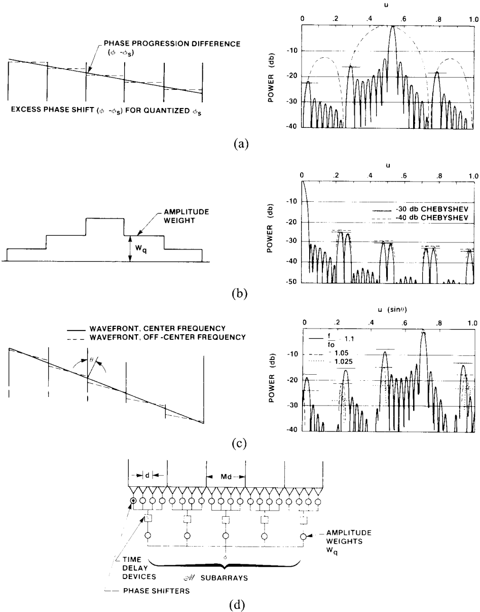
Figure 7.4 Three types of contiguous subarrays and their radiation patterns. All data for 64-element arrays with \lambda/2 spacing between elements and 8 elements per subarray: (a) case 1: discrete phase shifter states (equal amplitude weights); (b) case 2: taper at subarray input ports (ideal phase progression); (c) case 3: time delay at subarray ports (equal amplitude weights); and (d) array of contiguous subarrays. (From: [16]. © 1984 IEEE. Reprinted with permission.)
