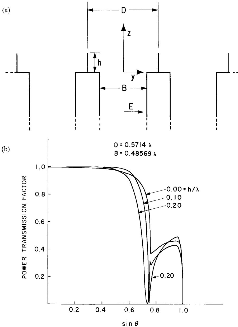
Figure 6.12 Radiating characteristics of parallel plane arrays with metallic fences. Note: power transmission factor is 1 - |\Gamma|^2 . (a) Geometry; (b) array power transmission factor for various fence heights; and (c) array power transmission factor for various fence heights. (From: [45]. © 1972 IEEE. Reprinted with permission.)
