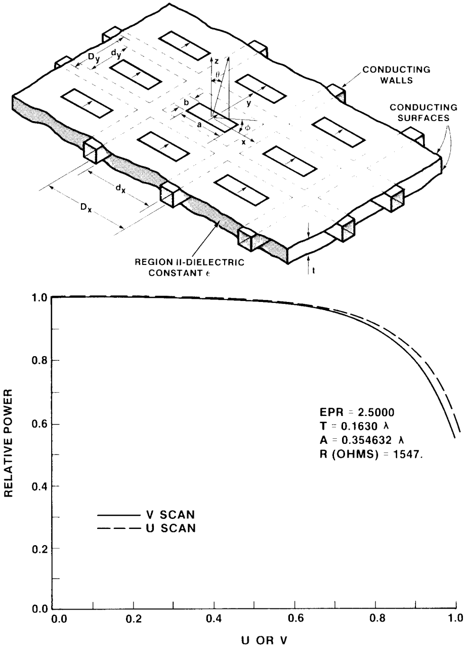
Figure 6.15 Geometry (top) and performance (bottom) of slot arrays with cavities. (From: [51]. © 1987 IEEE. Reprinted with permission.)
