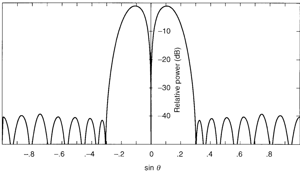
Figure 1.4 Low-sidelobe Bayliss radiation pattern.
