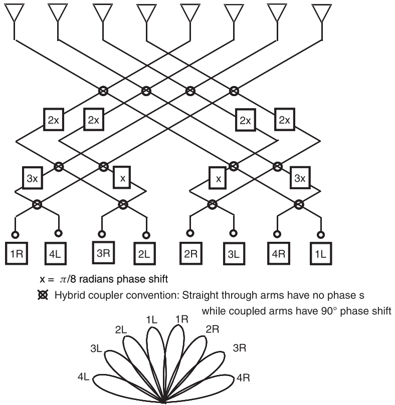
Figure 1.22 Eight-element, eight-beam Butler matrix and radiated beams.
