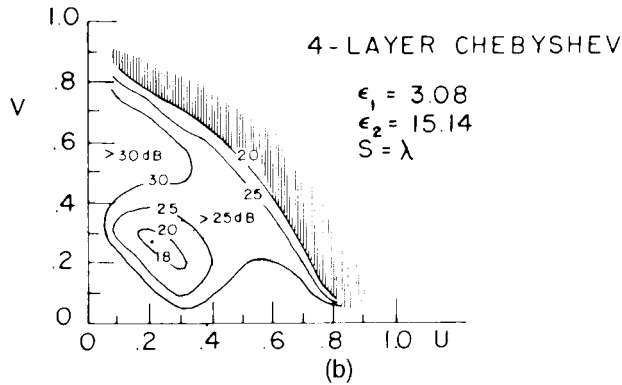
Figure 8.12 Dielectric layer angular filter geometry and performance: (a) dielectric layer filter; and (b) filter angular transmission characteristics.
