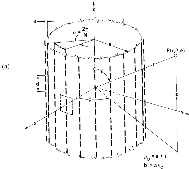
Figure 6.27 Periodic dipole array on a conducting circular cylinder. (a) Geometry; (b) H -plane voltage element gain pattern for cylindrical and reference planar arrays ( b/\lambda = 0.6 ; d/\lambda = 0.7 ; ka = 120 ); (c) H -plane voltage element gain pattern ( d/\lambda = 0.7 ; ka = 120 ) for azimuth spacing b/\lambda = 0.5, 0.6, 0.7 ; and (d) H -plane element gain power pattern (dB) ( b/\lambda = 0.6 ; d/\lambda = 0.7 ) for cylinder radii ka = 30, 60, 120, 240 . (From: [86]. © 1985 IEEE. Reprinted with permission.)
