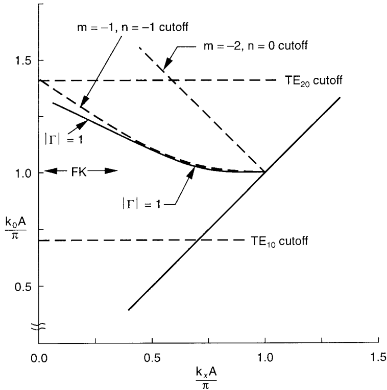
Figure 6.11 k - \beta diagram showing array null locus of the triangular grid array of Farrell and Kuhn (see Figure 6.10) but with dimension a/A reduced to 0.709. (From: [47]. © 1970 IEEE. Reprinted with permission.)
