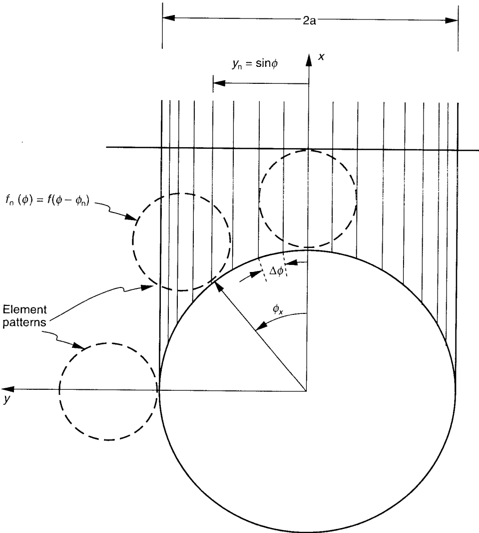
Figure 4.16 Array element patterns and projection to synthesize low-sidelobe pattern.
