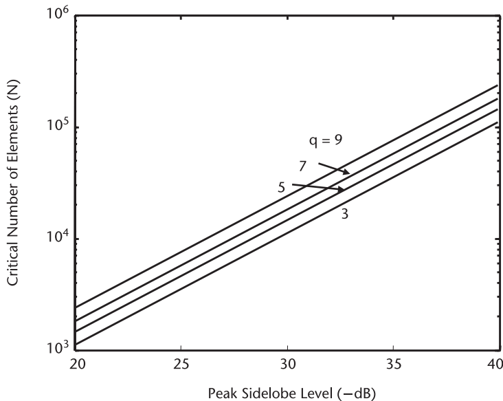
Figure 2.14 Number of elements required as a function of peak sidelobe level for various values of a = 10^q wavelengths with a 90% probability.
