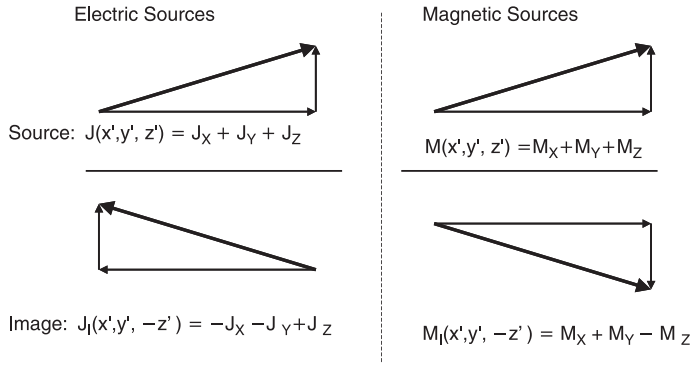
Figure 2.2 Image principle for electric and magnetic currents.
