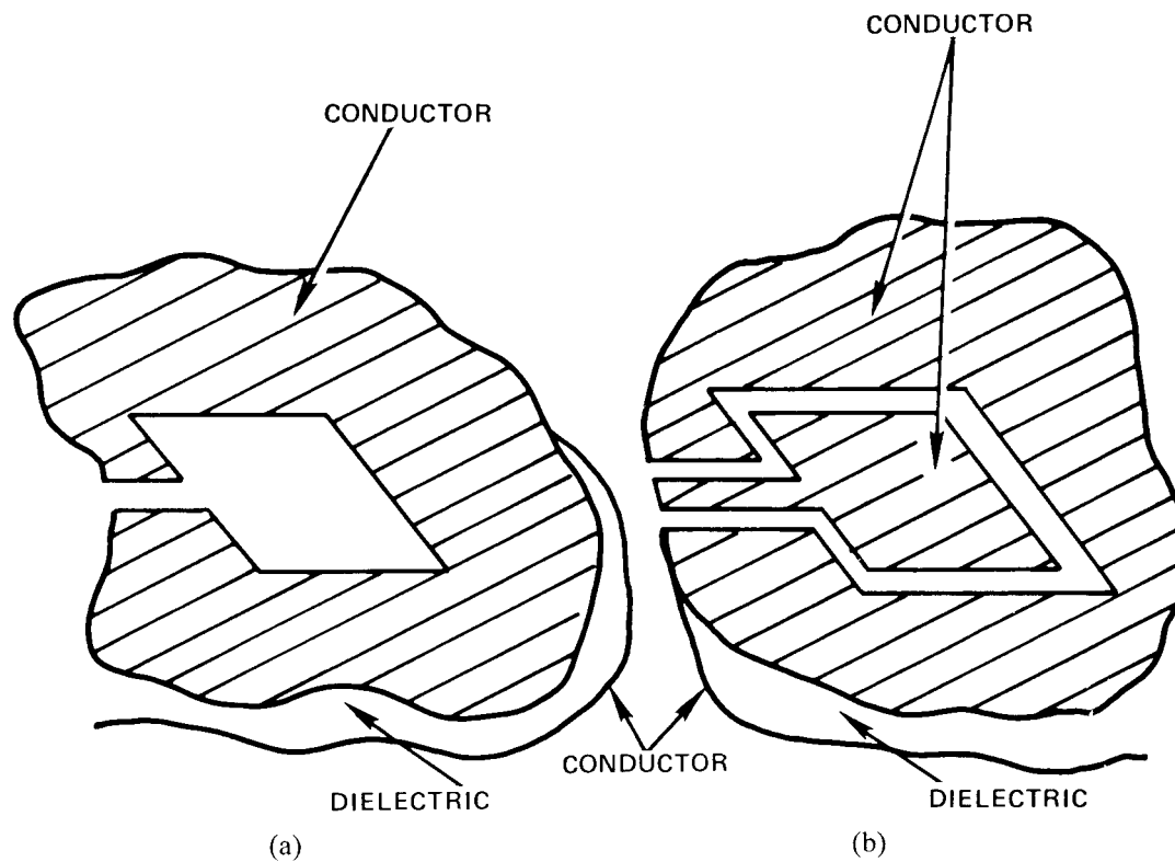
Figure 5.23 Other printed circuit radiators: (a) slot line antenna; and (b) coplanar strip line antenna.
