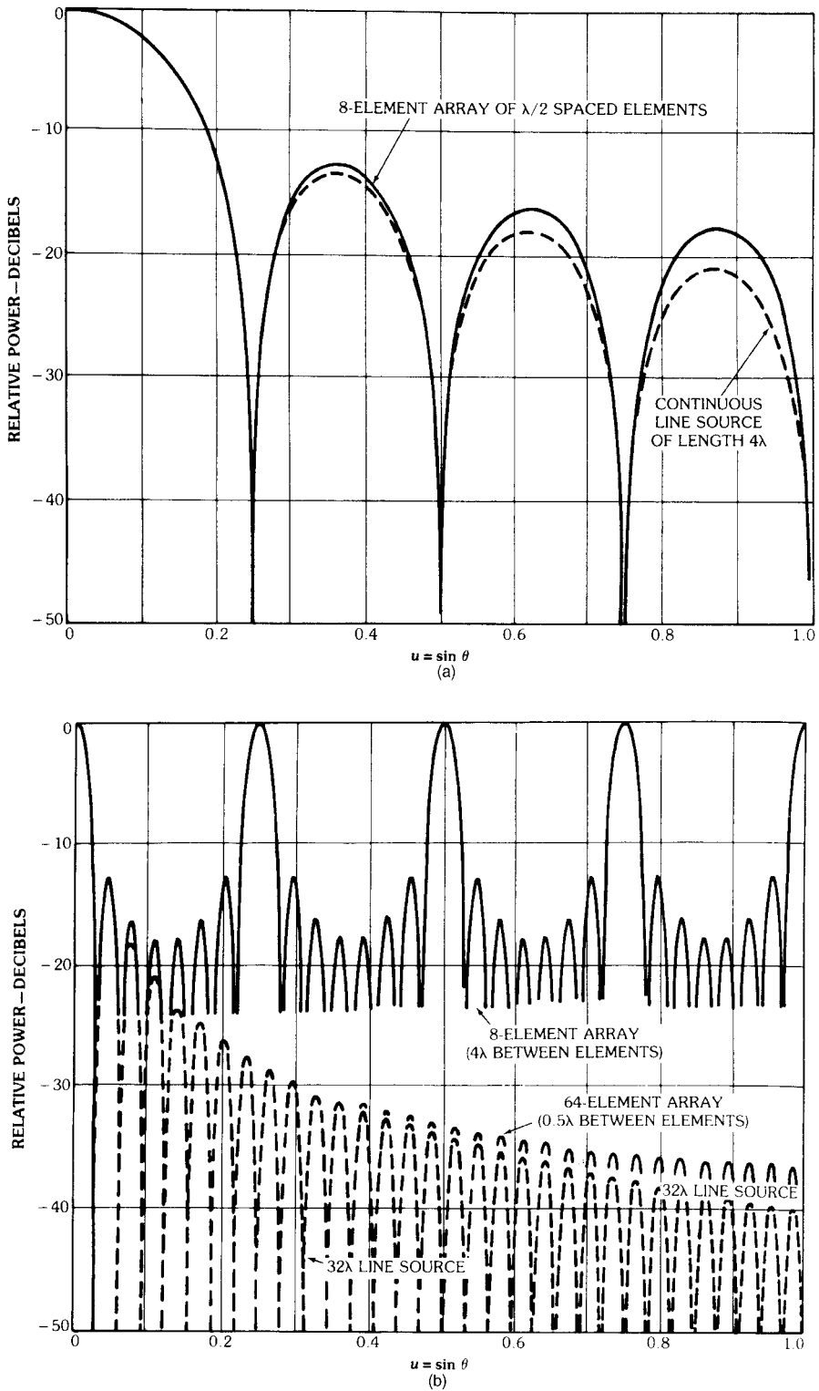
Figure 2.7 Line source patterns and array patterns: (a) patterns of 4\lambda line source and 8-element array with \lambda/2 spacing; and (b) patterns of uniformly illuminated 64-element array with 0.5\lambda spacing, 32\lambda line source, and 8-element array with 4\lambda spacing.
