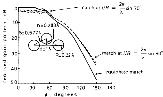
Figure 6.25 Element gain pattern, circumferential plane, and circumferential polarization ( R = 11.61\lambda ). Other dimensions shown. (From: [82]. © 1983 Peter Peregrinus, Ltd. Reprinted with permission.)
