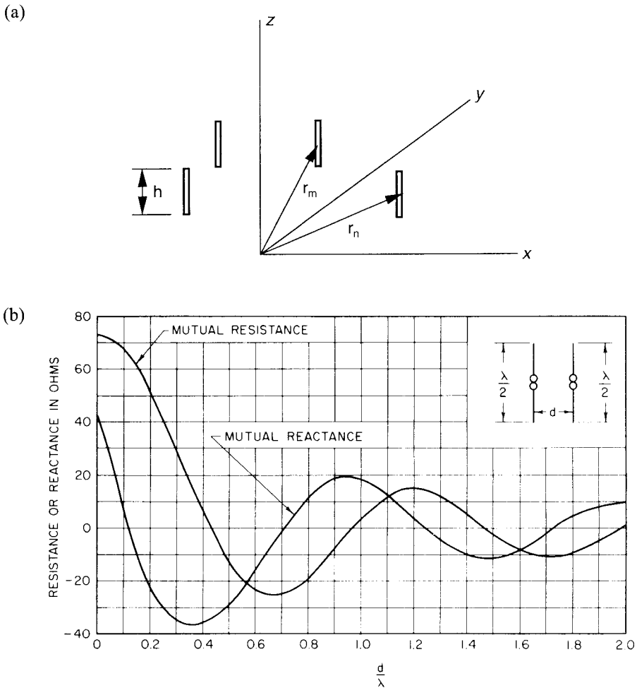
Figure 6.2 Mutual coupling of dipole antennas: (a) Geometry of array of dipoles with centers at \mathbf{r}_n = \hat{x}x_n + \hat{y}y_n ; and (b) mutual impedance Z_{12} between two dipoles. (From: [9]. © 1984 McGraw-Hill, Inc. Reprinted with permission.)
