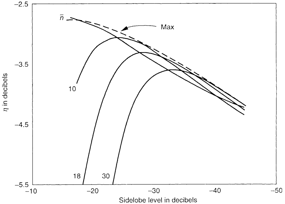
Figure 3.16 Relative directivity of Bayliss patterns. (From: [7]. © 1968 Bell System Technical Journal. Reprinted with permission.)
