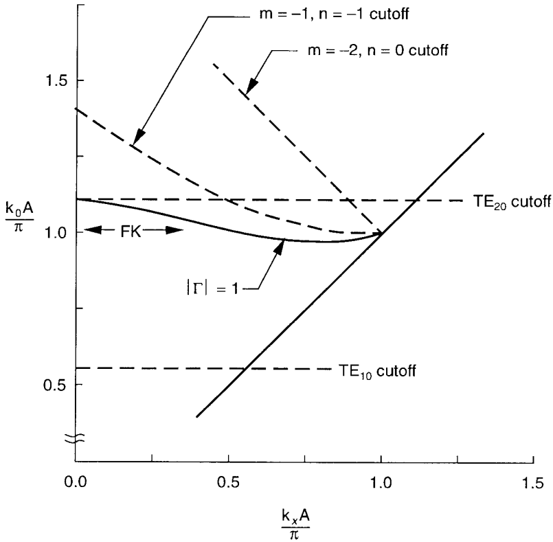
Figure 6.10 k - \beta diagram showing array null locus for the triangular grid array of Farrell and Kuhn, with B/A = 1 ; a/A = 0.898 ; b/A = 0.397 . (From: [47]. © 1970 IEEE. Reprinted with permission.)
