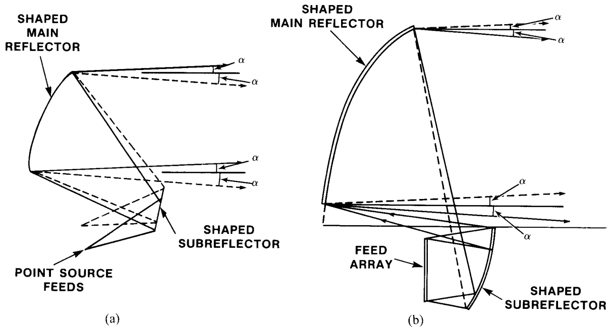
Figure 8.30 Dual-reflector bicollimated systems. (a) Multiple-beam Cassegrainian system. (b) Limited field-of-view scanning system. (From: [73]. © 1984 IEEE. Reprinted with permission.)
