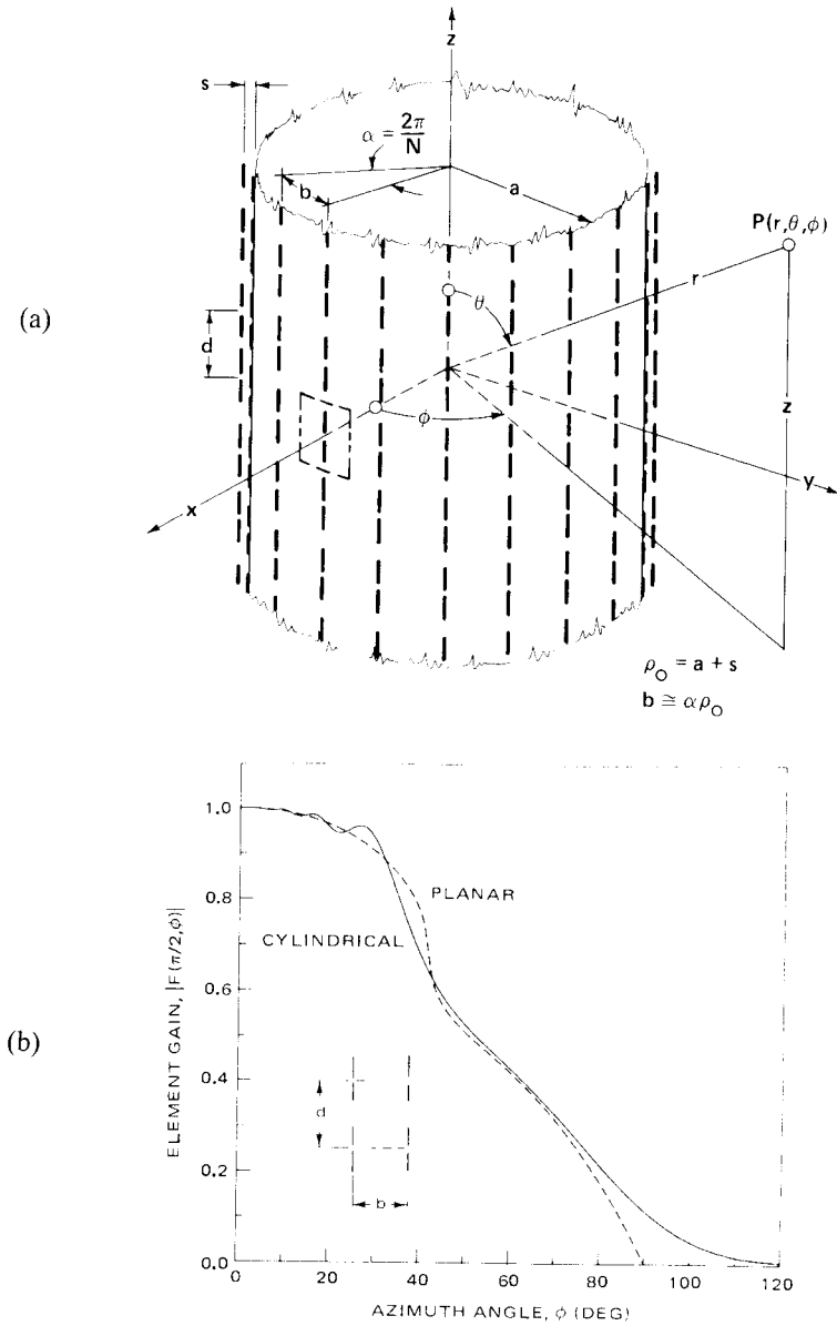
Figure 4.11 Element patterns of dipoles on arrays on cylinders: (a) geometry of the circular array of dipoles in a rectangular lattice; (b) H-plane voltage element gain patterns for cylindrical and reference planar arrays ( b/\lambda = 0.6, d/\lambda = 0.7, ka = 120 ). H-plane voltage element gain pattern: (c) parameter: ( d/\lambda = 0.7, ka = 120 ); azimuth spacing b/\lambda = 0.5, 0.6, 0.7 ; and (d) parameter: ( b/\lambda = 0.6, d/\lambda = 0.7 ); ka = 30, 60, 240 . (From: [39]. © 1983 IEEE. Reprinted with permission.)
