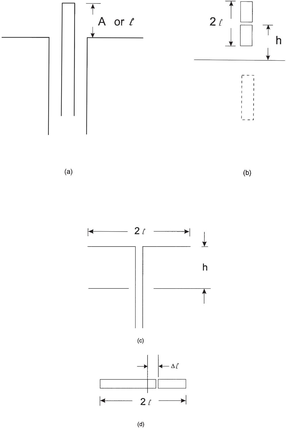
Figure 5.3 Basic wire radiating elements: (a) vertical monopole excited by coaxial feed; (b) vertical dipole and its image; (c) horizontal dipole antenna; and (d) off-center excitation of the dipole.
