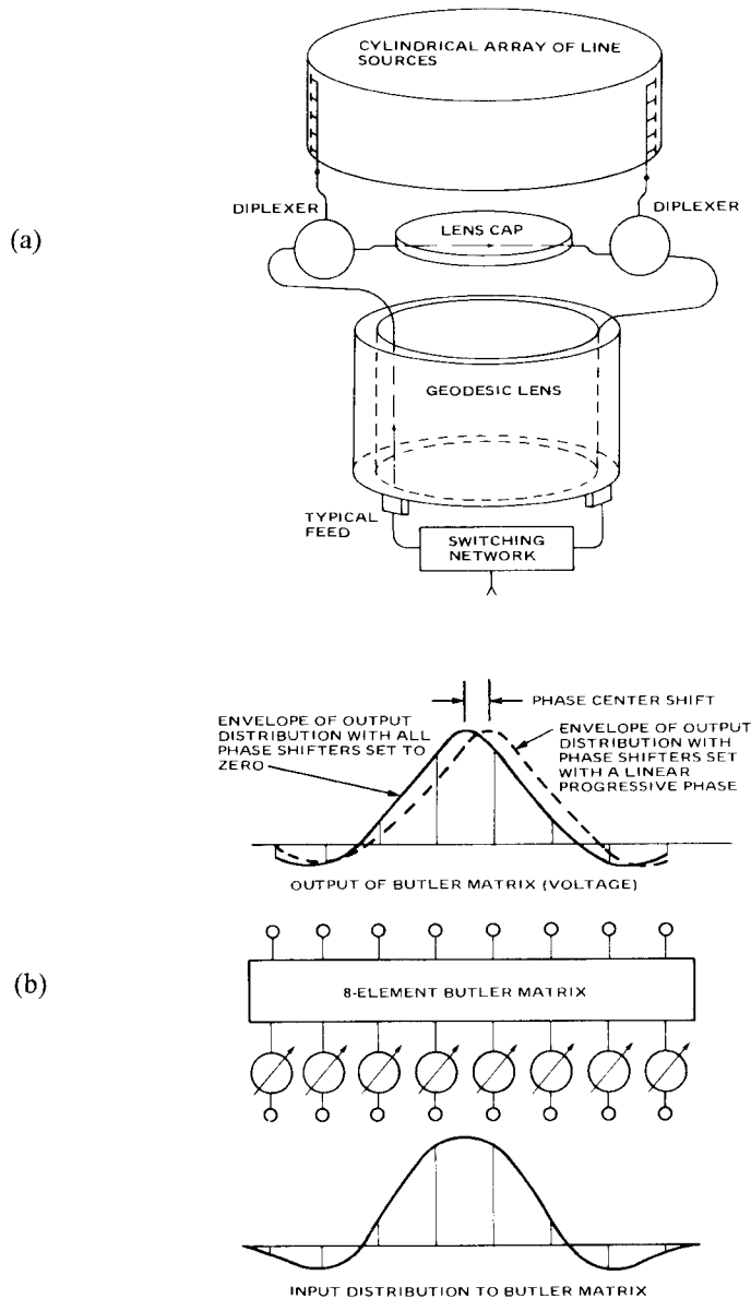
Figure 4.7 Electronically scanned array: (a) system configuration; and (b) fine beam steering with diode phase shifters and Butler matrix. (From: [32]. © 1974 IEEE. Reprinted with permission.)
