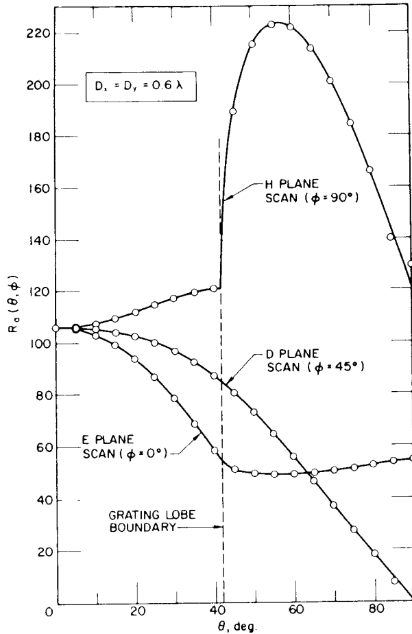
Figure 6.16 Dipole array scanning data for three different planes of scan. Dipoles are \lambda/4 above ground, array spacing 0.6\lambda . (From: [6]. © 1966 Academic Press, Inc. Reprinted with permission.)
