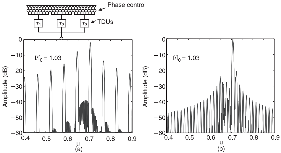
Figure 8.43 Comparison of radiation patterns for arrays of 16 subarrays with 32 elements each: (a) pattern of array of contiguous subarrays; and (b) pattern of uncompensated partially overlapped sections of overlapped subarrays. (From: [84]. © 2001 IEEE. Reprinted with permission.)
