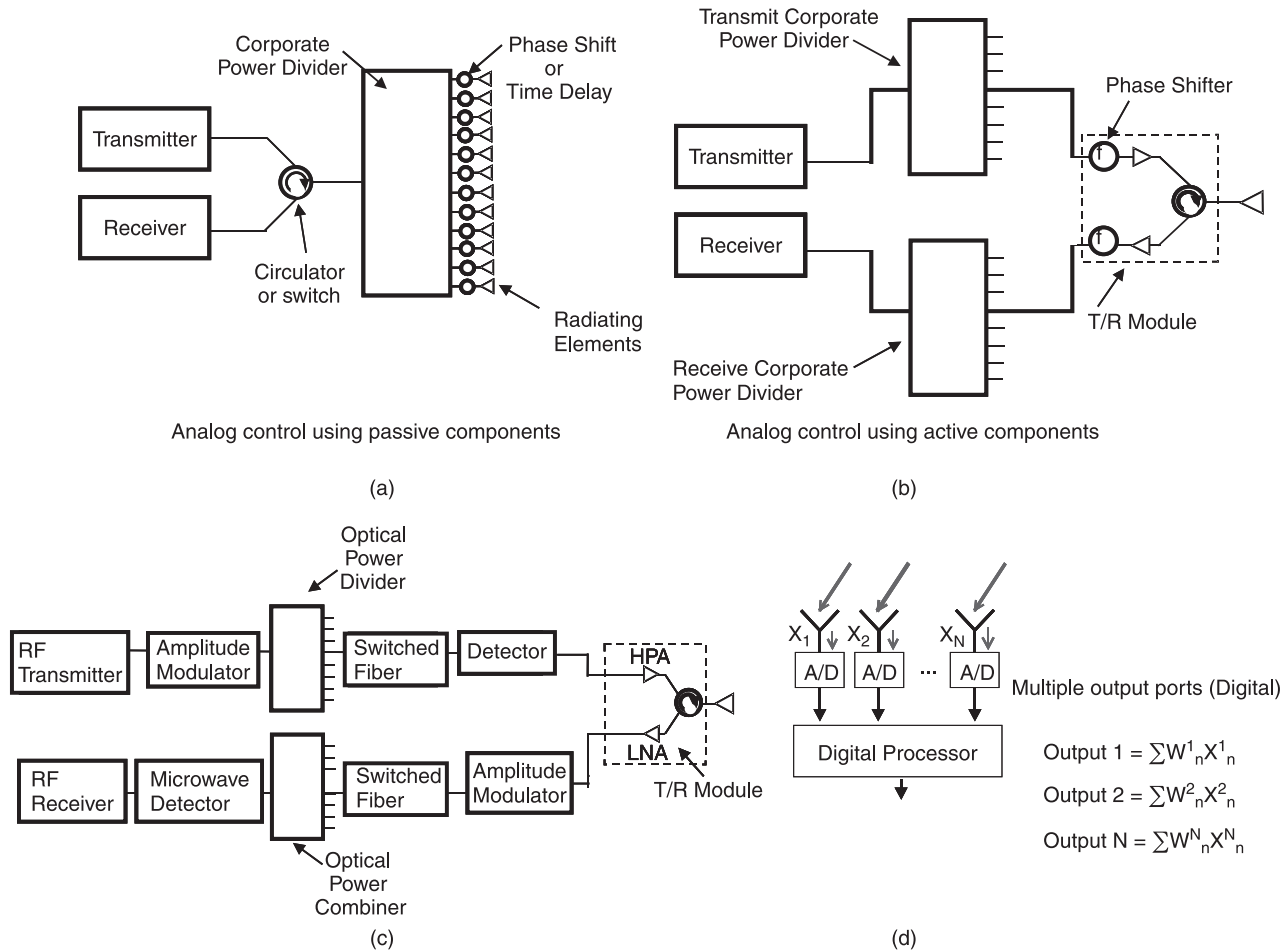
Figure 1.27 Array control modalities: (a) analog control using passive components; (b) analog control using active components; (c) optical control; and (d) digital control.
