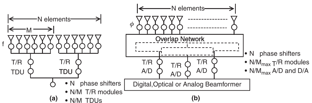
Figure 1.25 Architectures for fractional bandwidth wideband arrays: (a) phased array with contiguous time-delayed subarrays; and (b) phased array with time-delayed overlapped subarrays.
