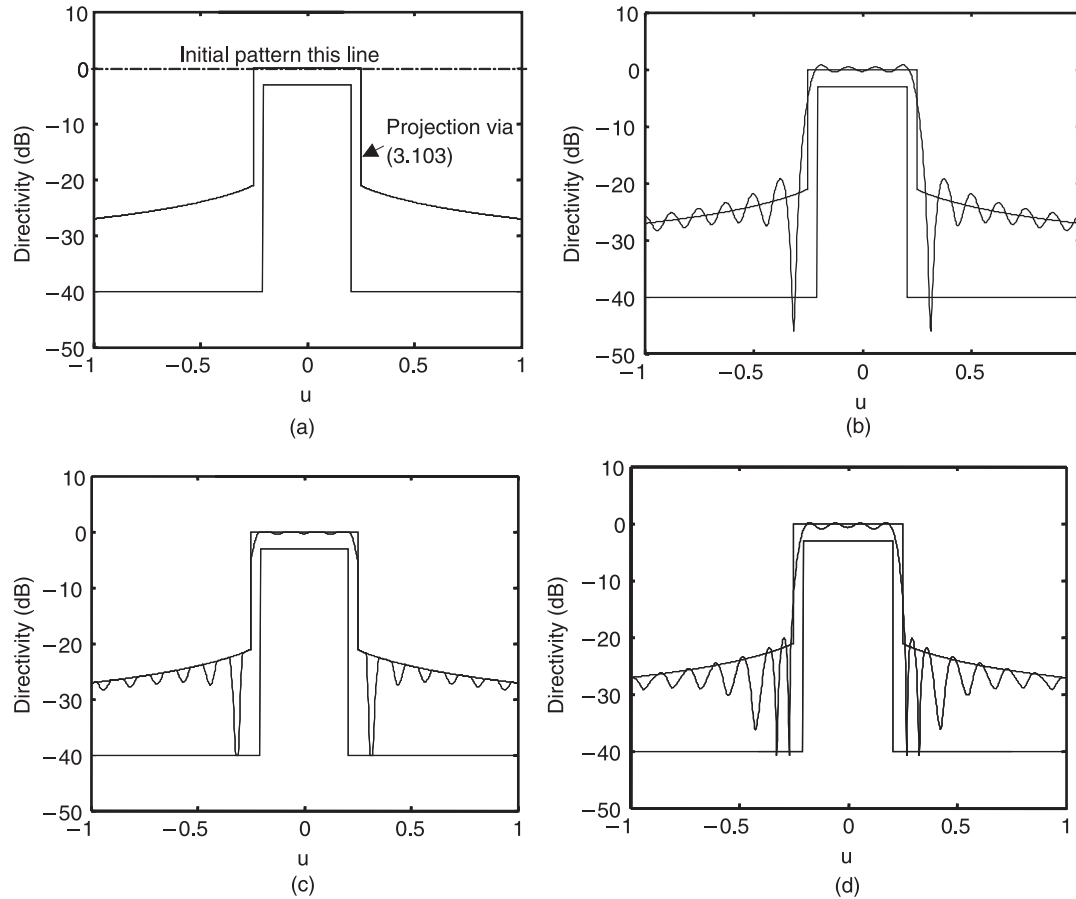
Figure 3.15 Synthesis of a pulse-shaped pattern using the method of alternating projection: (a) mask set chosen for projection (initial estimate shown as straight line at 0 dB); (b) radiation pattern of the first projection-upper mask of (a); (c) projection of the pattern of (b) onto the mask set; and (d) result of tenth iteration.
