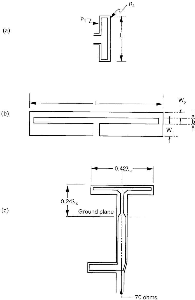
Figure 5.9 Folded dipole antennas: (a) basic folded dipole antenna; (b) strip folded dipole geometry; and (c) strip folded dipole. (From: [40]. © 1985 IEEE. Reprinted with permission.) (d) Folded dipole excited by microstrip balun. (After: [41].)
