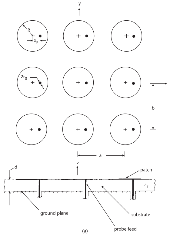
Figure 6.18 Reflection coefficient of an infinite array of circular patch elements fed by single probes as computed with idealized source and improved source models ( \epsilon_r = 2.55 , d = 0.06\lambda_0 , R = 0.166\lambda_0 , x_p = 0.083\lambda_0 , r = 0.0004\lambda_0 , a = 0.51\lambda_0 ). (a) Geometry; and (b) reflection coefficient magnitude. (From: [58]. © 1990 IEEE. Reprinted with permission.)
