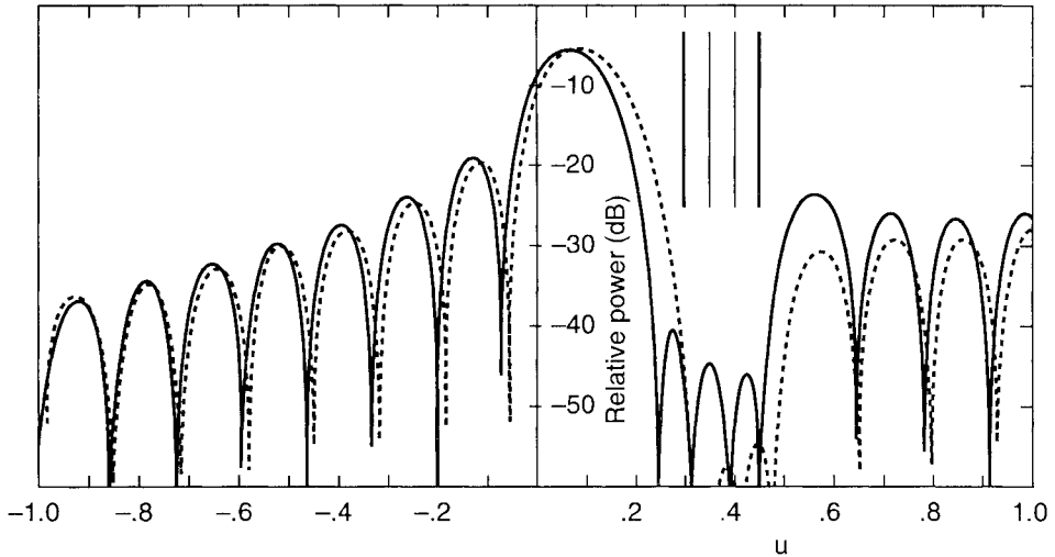
Figure 3.21 Adapted patterns of 8-element multiple-beam array. Quiescent beam at u = 0.0625 interference levels (relative to quiescent pattern) 99 (solid) and 1,000 (dashed).
