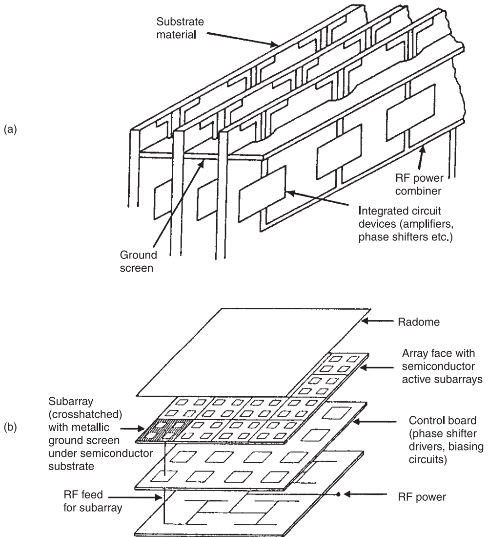
Figure 1.19 Basic array construction: (a) dipole array showing "brick" construction; and (b) microstrip patch array showing "tile" construction.
