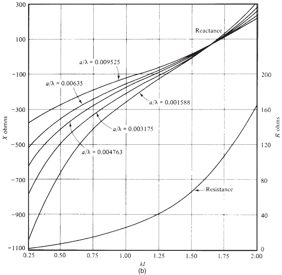
Figure 5.5 Impedance functions and impedance of isolated dipole. (a) Impedance functions R(k\ell) and X(k\ell) . (From: [3]. © 1984 McGraw-Hill, Inc. Reprinted with permission.) (b) Dipole resistance and reactance. (From: [9]. © 1951 Prentice Hall, Inc. Reprinted with permission.)
