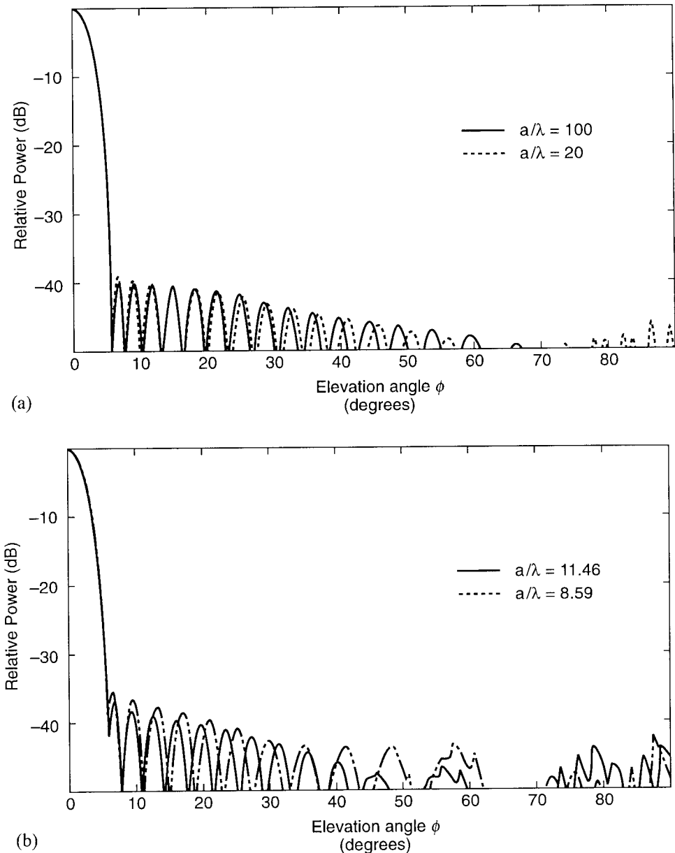
Figure 4.17 Synthesized patterns of circular sector array with projected Taylor distribution \bar{n} = 8 , sidelobe level -40 dB: (a) a/\lambda = 100 (solid), 20 (dashed); (b) a/\lambda = 11.46 ( 90^\circ sector) (solid), 8.59 ( 120^\circ sector) (dashed).
