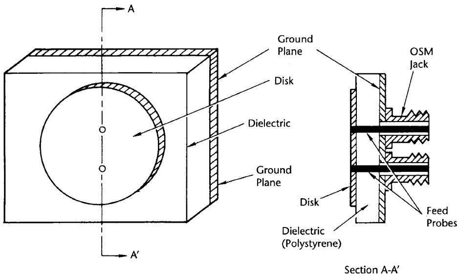
Figure 5.22 Circular disk excited by antiphase feed (Collings radiator).
