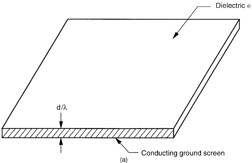
Figure 6.8 Structures supporting “surface waves”: (a) Dielectric slab structure. (b) Normalized propagation constants for TE and TM waves. (From: [40]. © 1984 IEEE. Reprinted with permission.) (c) Monopole array supporting “surface wave (spectrum).” (d) Shorted corrugated structure.
