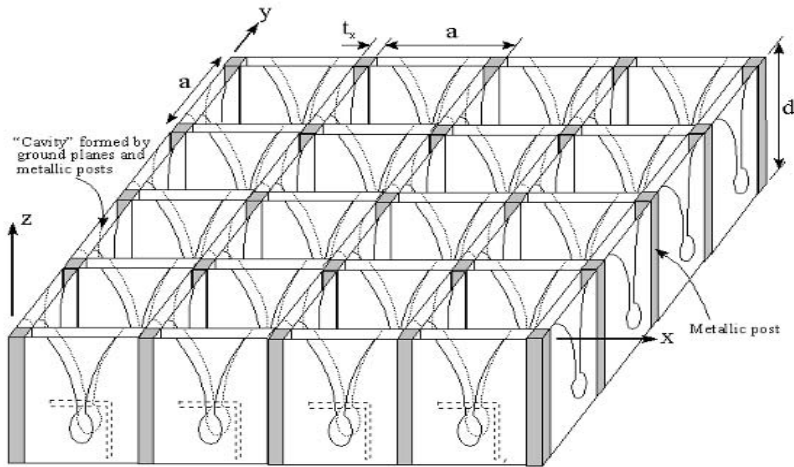
Figure 6.21 A dual polarized TSA array. Elements are separated by metallic posts, and the array is backed by a metallic ground plane at z = -d . (From: [65]. © 2000 IEEE. Reprinted with permission.)
