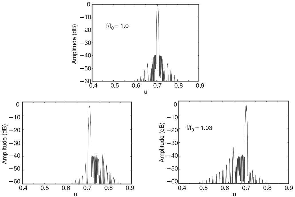
Figure 8.45 Radiation patterns of array with synthesized subarray patterns at center frequency and band edges. (From: [84]. © 2001 IEEE. Reprinted with permission.)
