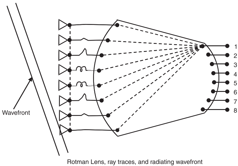
Figure 1.23 Rotman lens, ray traces, and radiated wavefront.
