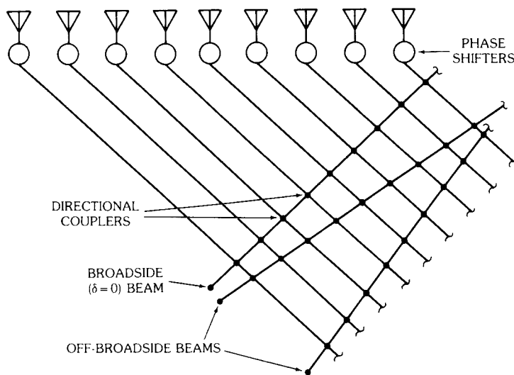
Figure 8.6 Constrained Blass time-delayed multiple-beam forming circuit (shown here feeding a phase-scanned array).
