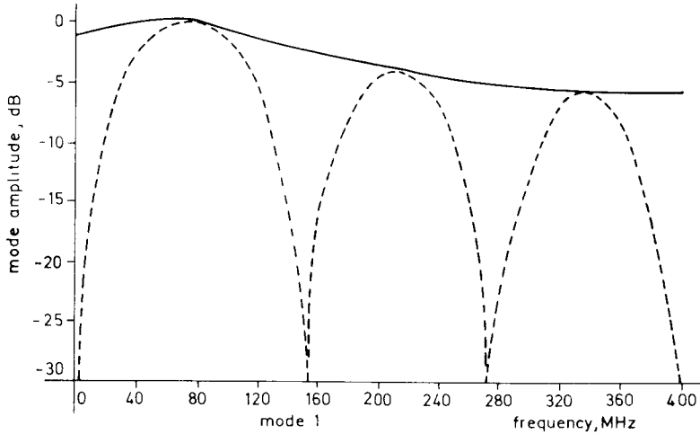
Figure 4.5 Theoretical results showing the stability of mode 1 versus frequency due to the use of directional elements of the form (1 + \cos \phi) (solid curve) and omnidirectional (dashed curve) elements for 2\lambda radius array at 300 MHz. (From: [23]. © 1983 Peter Peregrinus Ltd. Reprinted with permission.)
