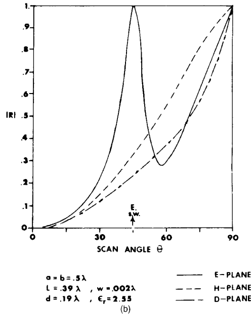
Figure 6.13 Array radiation and grating lobe loci compared with slow “surface wave” loci: (a) Surface wave circle diagram; (b) E , H , and diagonal plane scan data showing blindness in E -plane; and (c) reflection coefficient contour plot showing loci of the surface wave for unloaded dielectric surface. (From: [40]. © 1984 IEEE. Reprinted with permission.)
