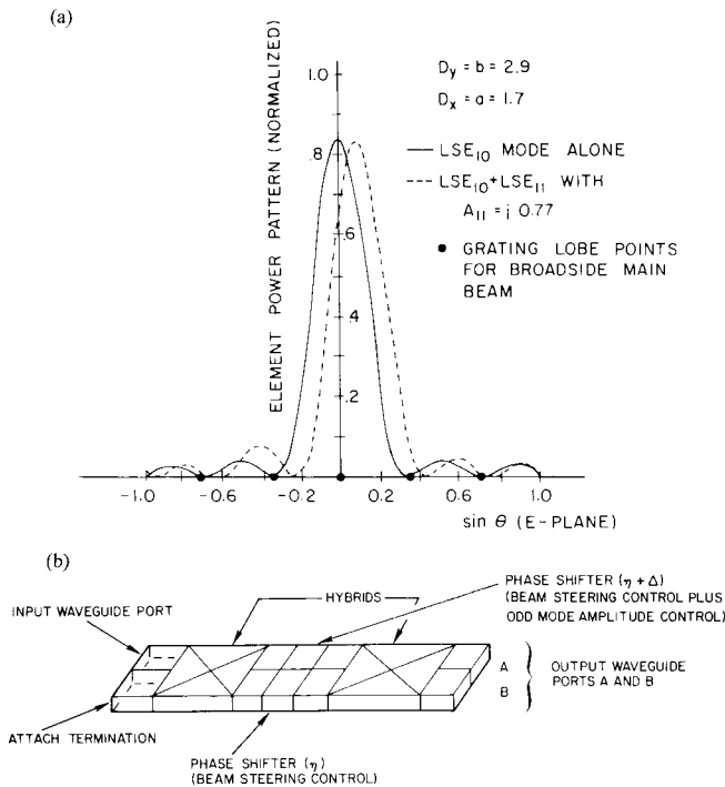
Figure 8.11 Multimode horn apertures for limited field of view: (a) control of element pattern null for grating lobe suppression; (b) circuit for nulling; (c) E -plane horn and lens with odd-mode amplitude control; and (d) locus of grating lobe power levels and main beam scan.
