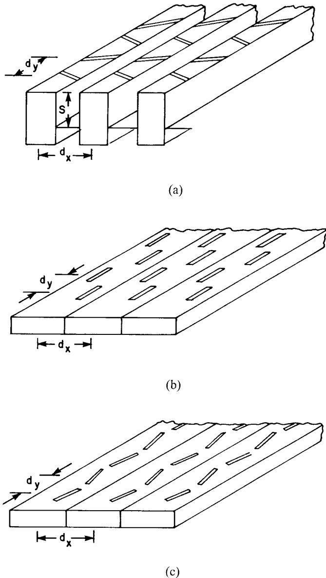
Figure 5.25 Waveguide slot array geometries: (a) edge slot array; (b) displaced longitudinal slot array; and (c) inclined series slot array.
