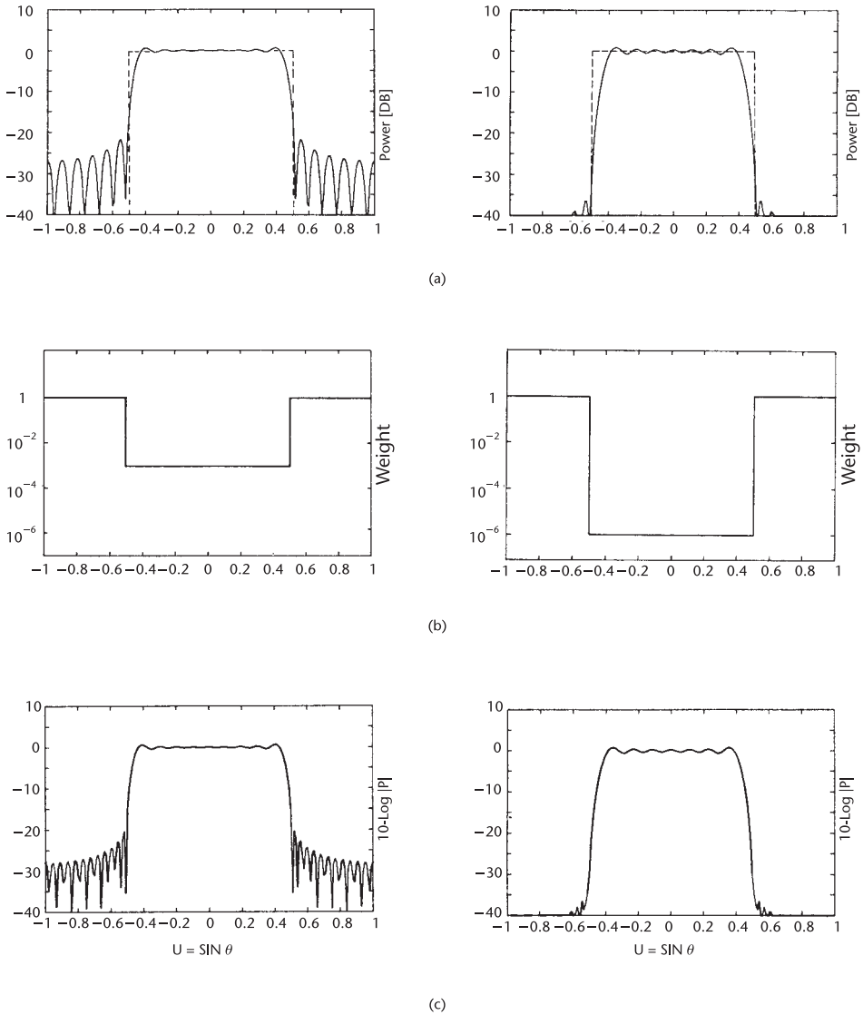
Figure 3.12 Gaussian power pattern synthesis. Curves at left use 30-dB weighting function. Curves at right use 60-dB weighting function. Upper curves (a) show desired pattern (dashed) and optimum realizable power pattern (solid). Center curves (b) show weighting functions. Lower curves (c) show best harmonic approximation (magnitude only). (From: [31]. © 1970 IEEE. Reprinted with permission.)
