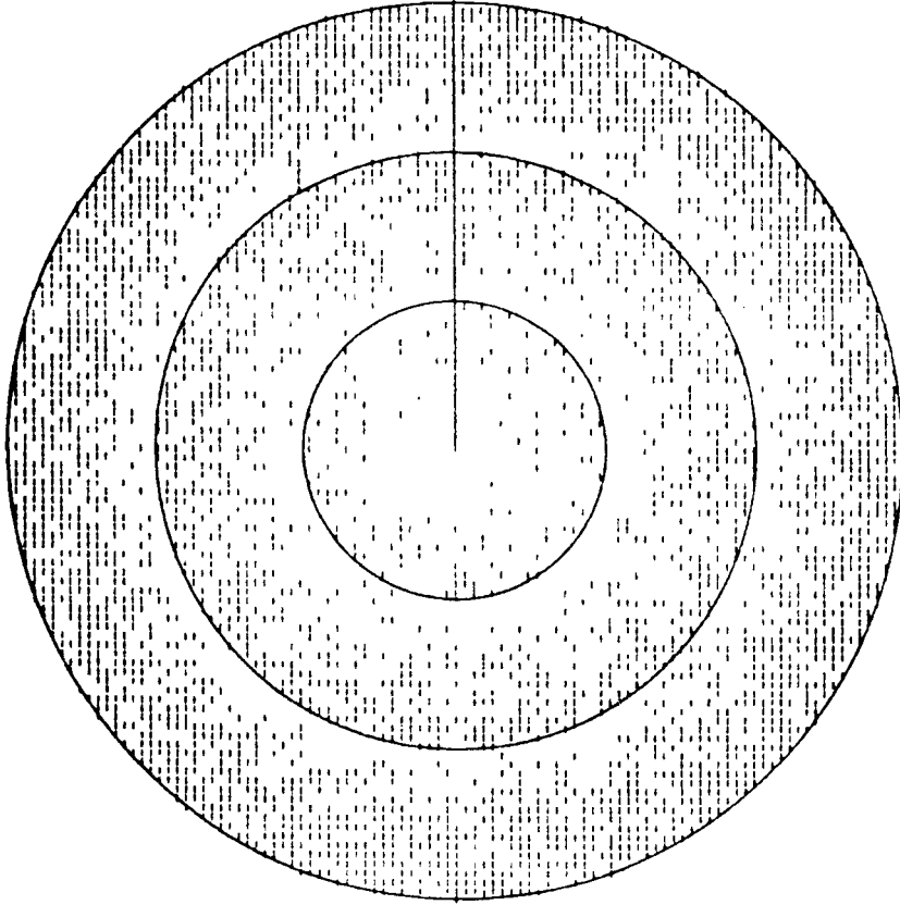
Figure 2.17 Distribution of nonexcited (thinned) elements for an array with three quantized steps. (From: [40]. © 1991 IEEE. Reprinted with permission.)
