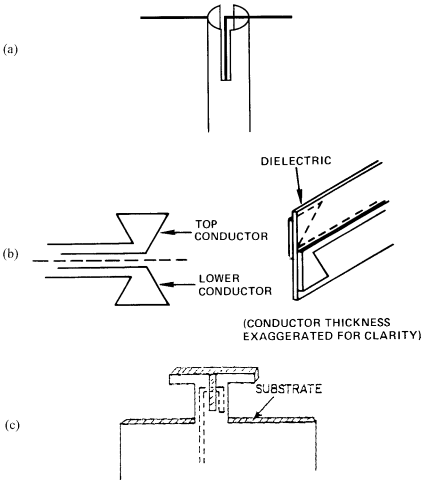
Figure 5.7 Practical wire antennas and feeds. (a) Split tube balun feed for dipole antenna. (b) Bowtie dipole excited by coplanar strips transmission line. (From: [16]. © 1974 IEEE. Reprinted with permission.) (c) Microstrip-fed dipole and balun for radiation endfire to substrate. (From: [17]. © 1987 Horizon House Publications, Inc. Reprinted with permission.) (d) Bowtie dipole excited by microstrip, slot line, and coplanar strip transitions. (From: [18]. © 1986 Microwaves and RF News. Reprinted with permission.)
