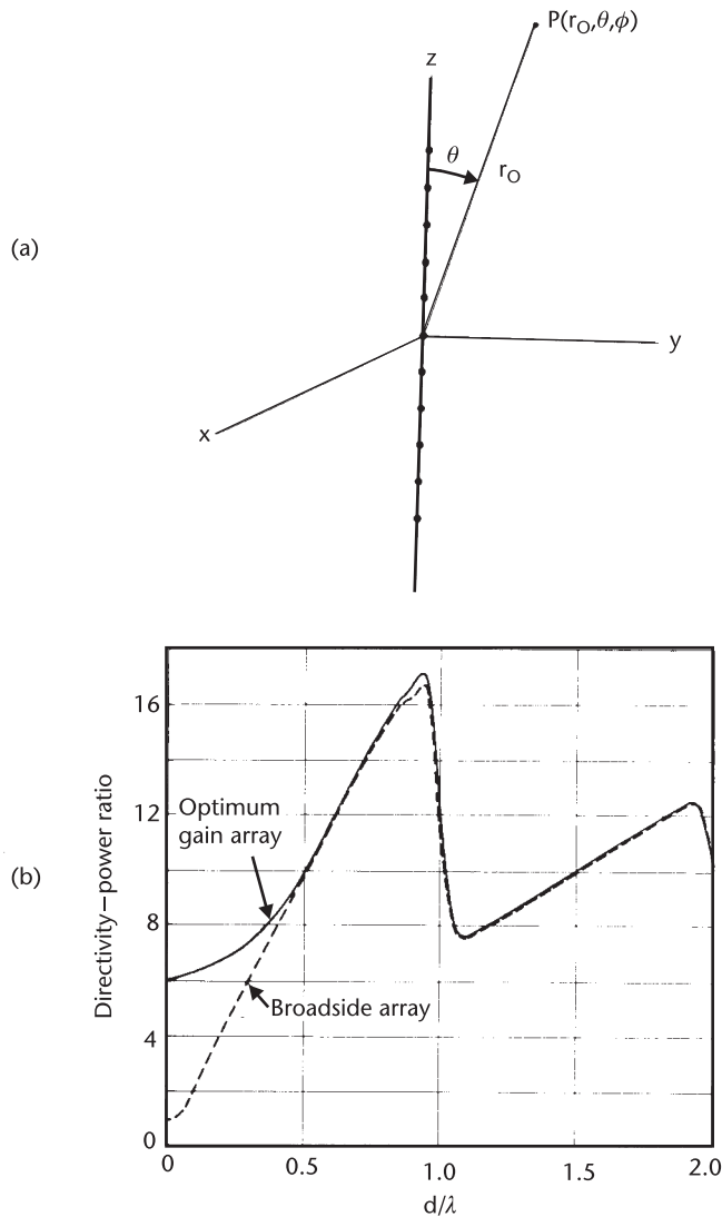
Figure 2.9 Directivity of an array of omnidirectional elements: (a) array geometry; and (b) array directivity for a 10-element array. (From: [11]. © 1964 IEEE. Reprinted with permission.)
