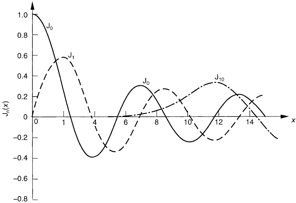
Figure 4.3 Bessel functions J_p(ka) versus radial parameter ka for p = 1, 2, 10 .
