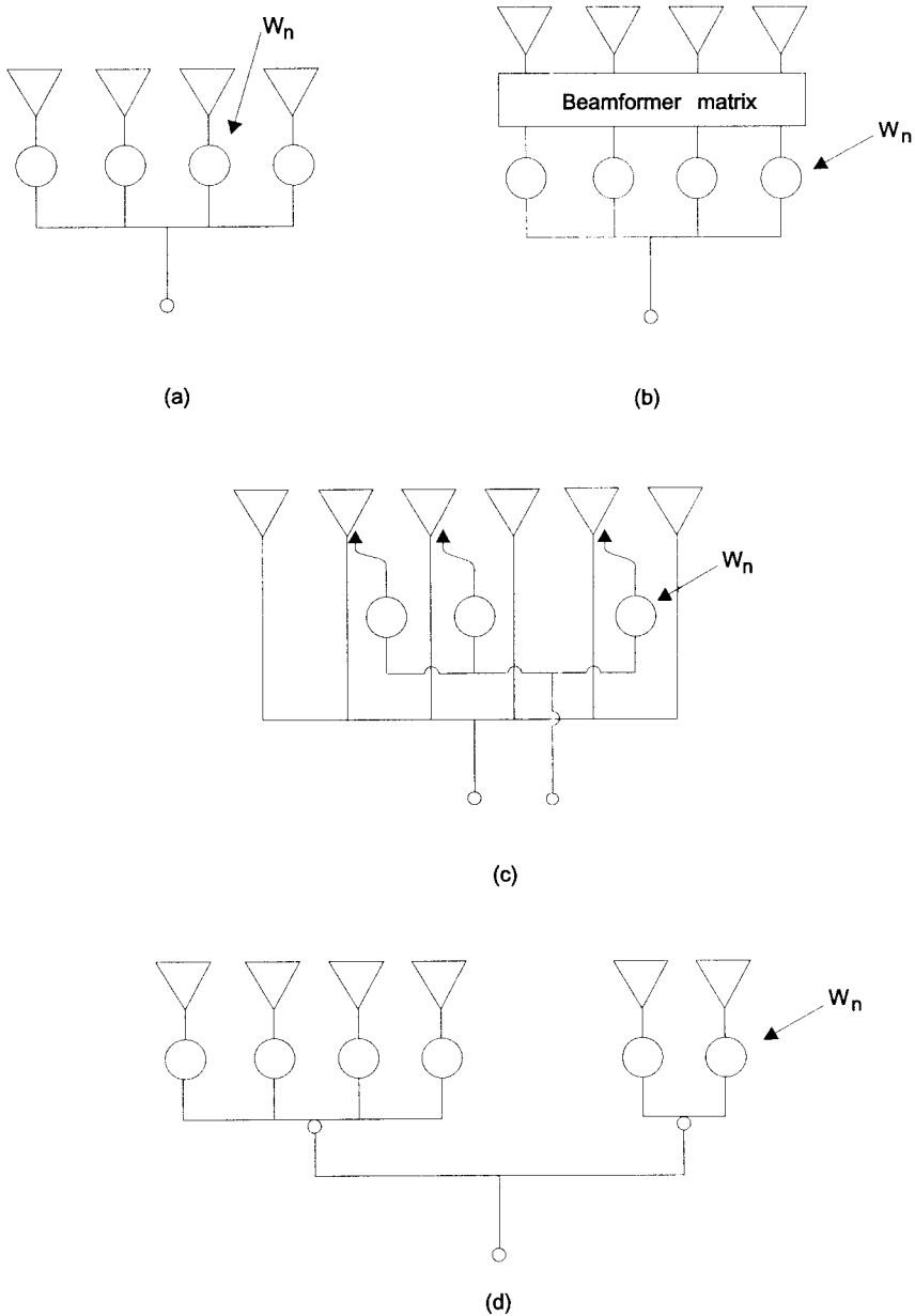
Figure 3.17 Adaptive array configurations: (a) fully adaptive array (element weighting); (b) fully adaptive array with multiple-beam feed (beam space adaptivity); (c) partially adaptive array; and (d) array with multiple canceler elements.
