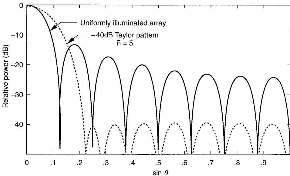
Figure 1.7 Radiation characteristics of uniformly illuminated and low-sidelobe 16-element arrays.
