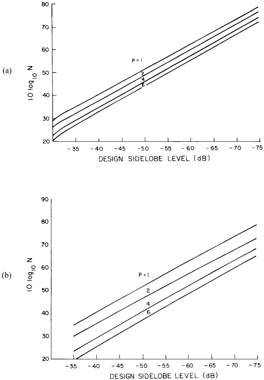
Figure 2.20 Number of array elements for average sidelobe level equal to design sidelobe level: (a) method 1; and (b) method 2. (From: [40]. © 1991 IEEE. Reprinted with permission.)
