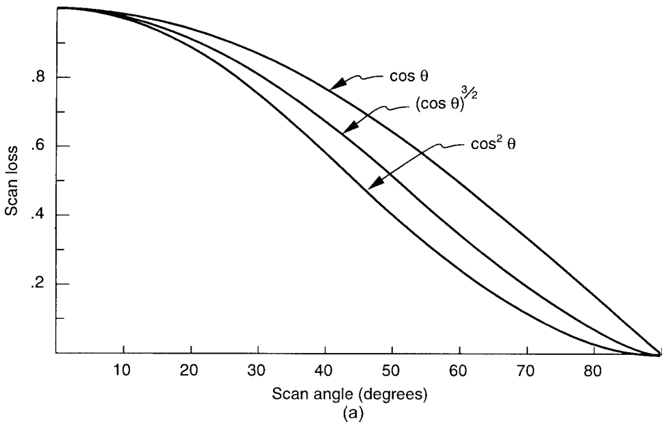
Figure 1.11 (a) Typical scan loss curves. (b) Scan loss with array blindness. (From: [23]. © 1968 IEEE. Reprinted with permission.)
