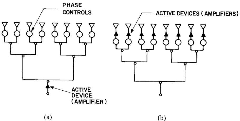
Figure 1.15 Active and passive array configurations: (a) passive array; and (b) active array.
