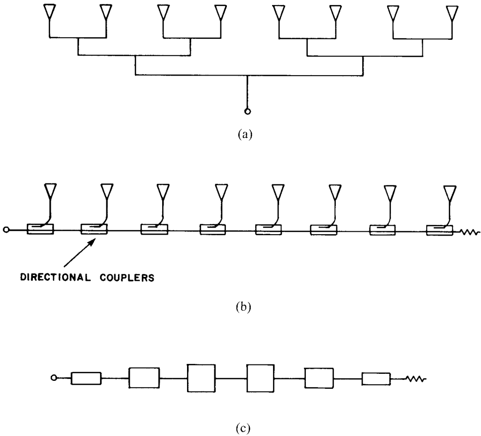
Figure 5.24 Column array configurations: (a) parallel (equal line length) corporate feed; (b) series-fed array; and (c) series-fed microstrip patch array.
