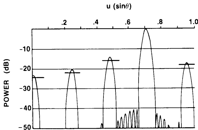
Figure 7.11 Power pattern for array with time delay at subarray ports and a 40-dB Chebyshev taper f/f_0 = 1.05 . (From: [16]. © 1984 IEEE. Reprinted with permission.)
