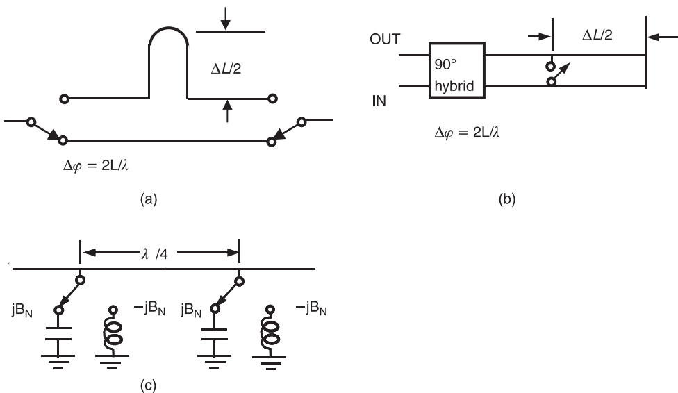
Figure 1.29 Microwave phase shifter circuits: (a) switched line phase shifter; (b) reflection phase shifter; and (c) loaded line shifter.
