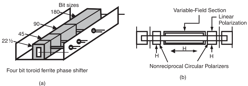
Figure 1.28 Ferrite phase shifter configurations. (a) Four-bit toroid ferrite phase shifter. (b) Dual-mode latching ferrite phase shifter. (From: [44]. © 1970 IEEE. Reprinted with permission.)
