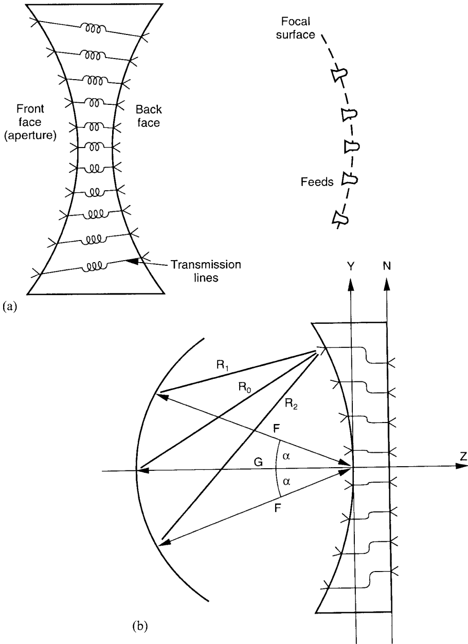
Figure 8.7 Several multiple-beam lens and reflector systems: (a) generic bootlace lens; (b) Rotman lens; and (c) reflector with displaced feed for multiple-beam radiation. (From: [18]. © 1988 Artech House, Inc. Reprinted with permission.)
