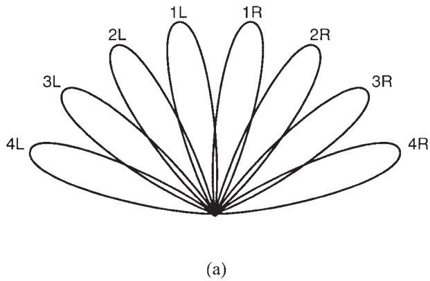
Figure 8.5 Constrained circuits for forming multiple beams: (a) eight-beam, eight-element Butler matrix; (b) two orthogonal beams (plotted for N = 8 ) with i = 1/2 and i = -7/2 ; (c) beam cluster motion as function of frequency; and (d) beam cluster geometry for time-delayed beams.
