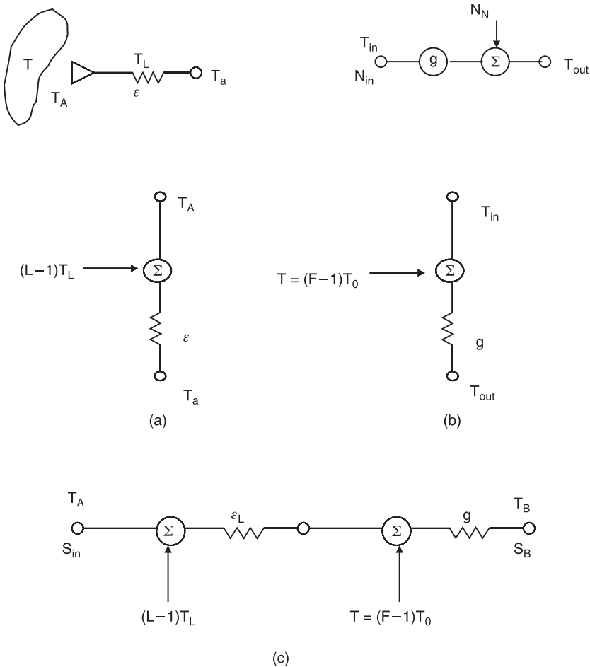
Figure 1.2 Antenna noise temperature flow graphs: (a) two-port network with loss; (b) two-port network with amplification; and (c) lossy two port with following amplifier.
