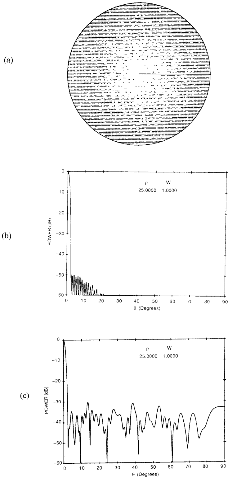
Figure 2.13 Circular array with elements removed: (a) geometry (dashes show elements removed); (b) desired Taylor pattern (filled array); and (c) thinned array pattern.
