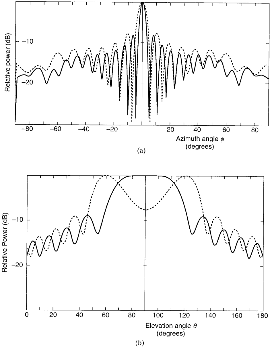
Figure 4.4 Radiation patterns for 30-element array of omnidirectional elements. Cylinder radius 4.7746\lambda : (a) Azimuth plane patterns (\theta, \theta_0) = (90, 90) solid curve, (\theta, \theta_0) = (45, 45) dashed curve; (b) elevation patterns for \phi = \phi_0 = 0 dashed curve and for array scanned to \theta_0 = 90^\circ (solid), 60^\circ (dashed); and (c) elevation patterns for \theta_0 = 45^\circ (solid) and 30^\circ (dashed).
