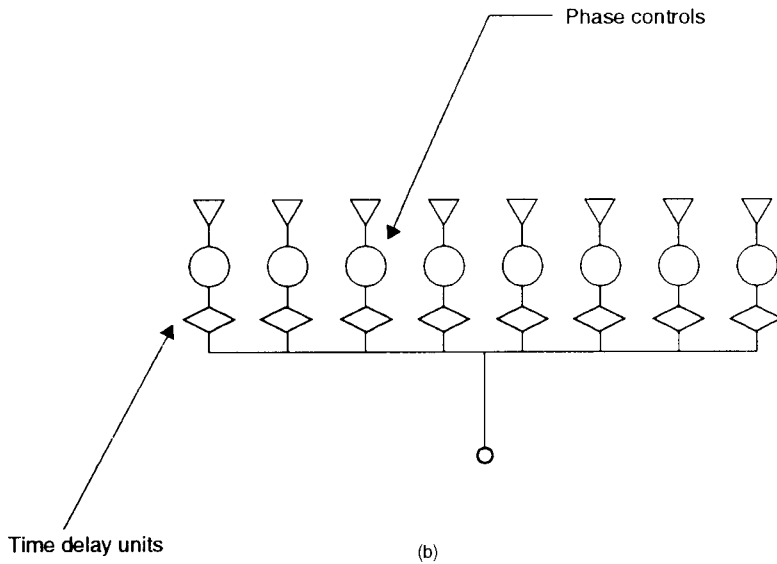
Figure 8.40 Wideband scanning array feeds: (a) array-fed by time-delayed beamformer; (b) array fed by time-delay units and phase shifters; and (c) array of contiguous subarrays with time delay at the subarray level. (From: [81]. © 1981 IEEE. Reprinted with permission.)
