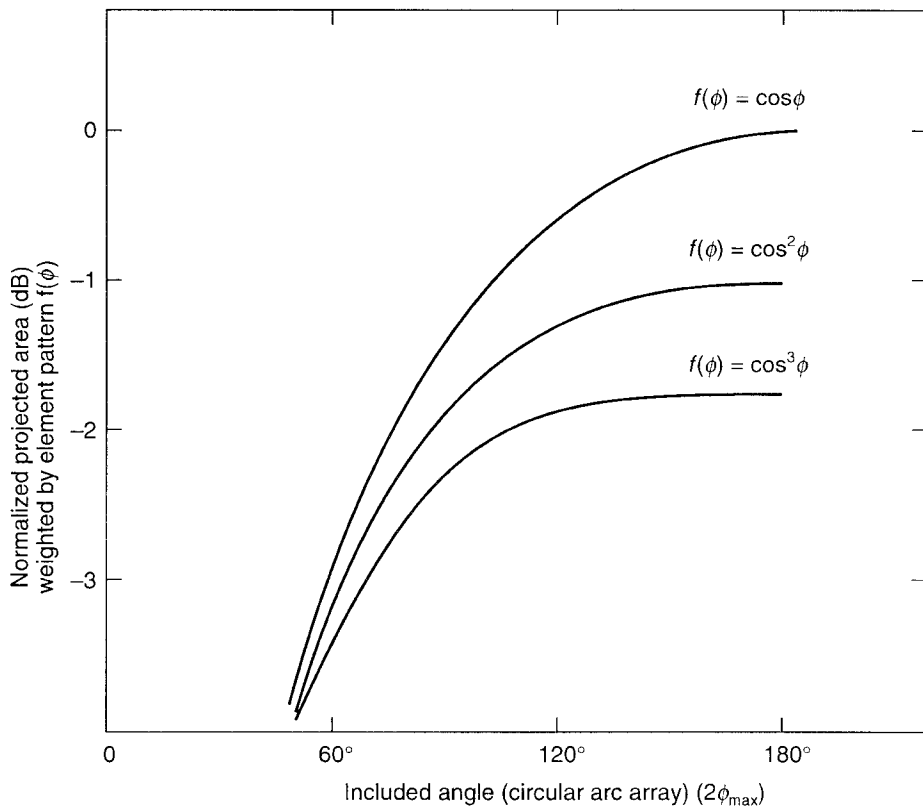
Figure 4.14 Normalized gain for various element patterns.
