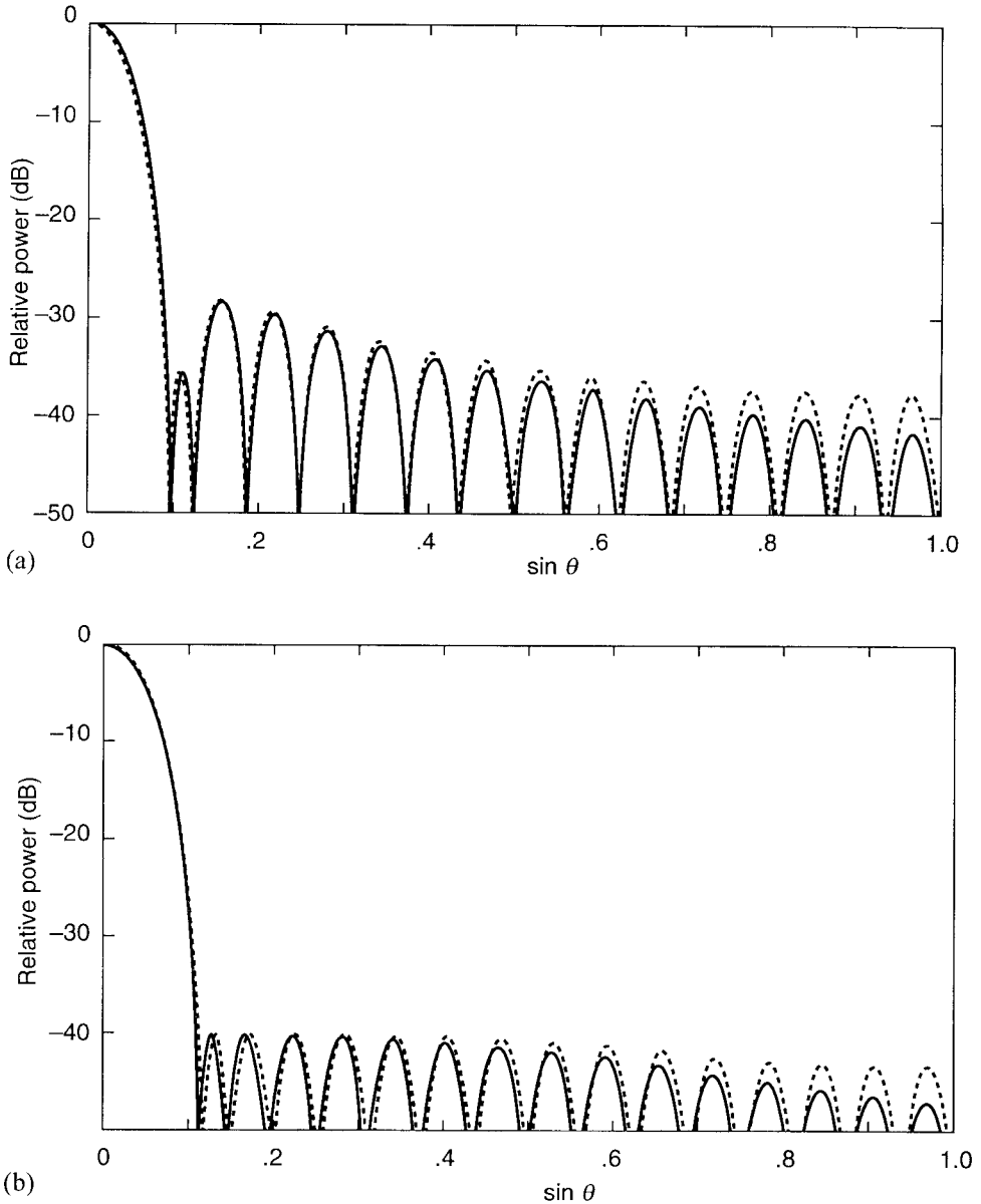
Figure 3.6 Taylor patterns of line sources and 32-element arrays. (a) Array with Taylor \bar{n} = 2 , -40 -dB sidelobe pattern (solid curve from function, dashed curve from array currents). (b) Array with Taylor \bar{n} = 11 , -40 -dB sidelobe pattern (solid curve from function, dashed curve from array currents). (c) Taylor \bar{n} aperture distributions for -25 -dB sidelobe level. (From: [15]. © 1983 Peter Peregrinus Ltd. Reprinted with permission.)
