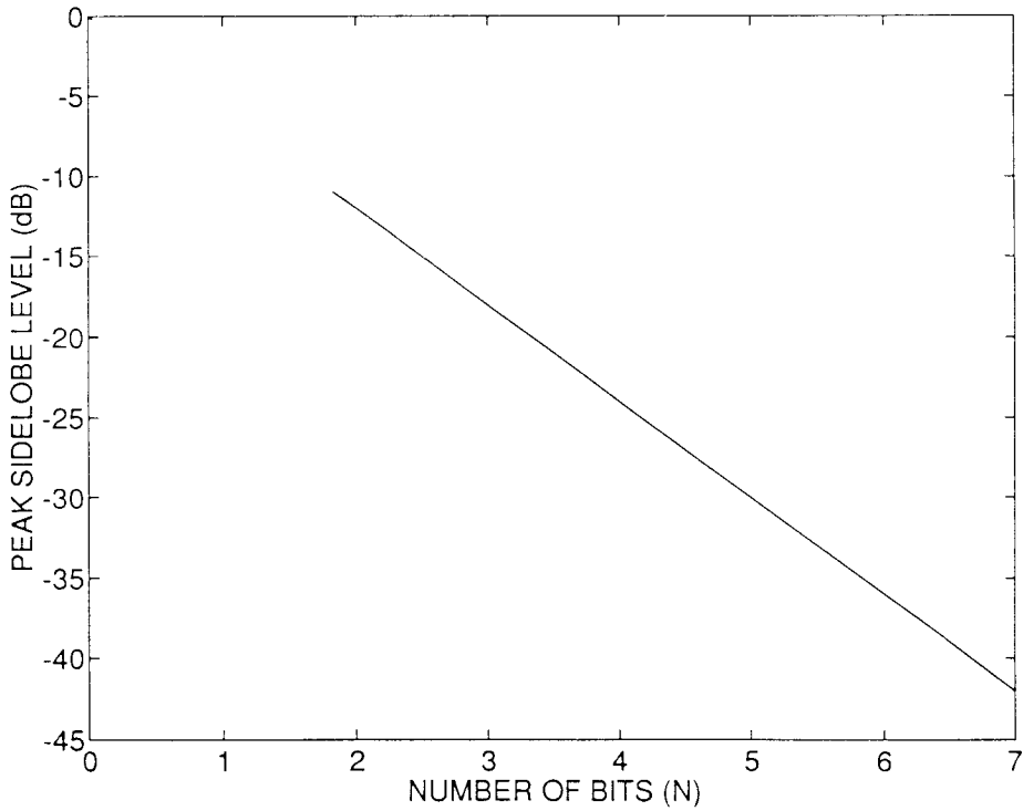
Figure 7.6 Peak sidelobes (decibels) due to N bits of quantization. (After: [17].)
