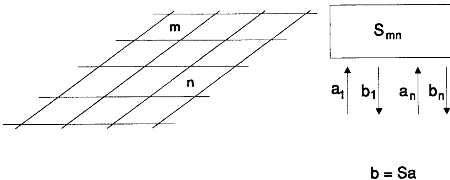
Figure 2.5 Scattering matrix representation for interelement coupling of waveguide apertures.
