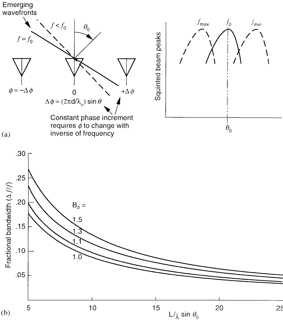
Figure 1.14 Wideband effects in phased array performance: (a) beam squint for a phased array (wavefronts and beam peak motion); (b) array 3-dB bandwidth versus (L/\lambda) \sin \theta_0 ( B_b is beam broadening factor); (c) array or subarray length (L/\lambda) \sin \theta_0 versus bandwidth (MHz) ( B_b is beam broadening factor); and (d) narrow pulse incident on array (array fill time).
