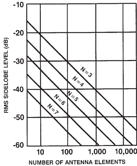
Figure 7.7 RMS sidelobes due to phase quantization. (After: [17].)
