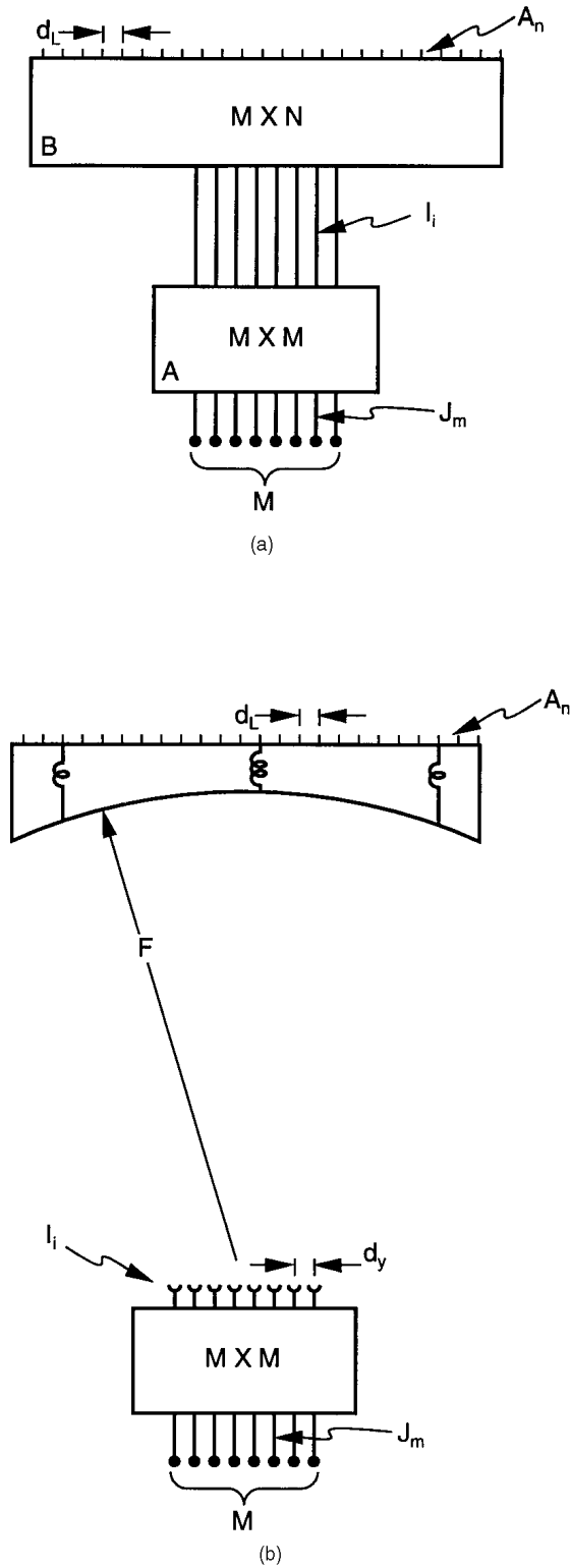
Figure 8.22 Cascaded multiple-beam networks of completely overlapped subarray formation: (a) constrained network of cascaded multiple-beam networks; and (b) space-fed network.
