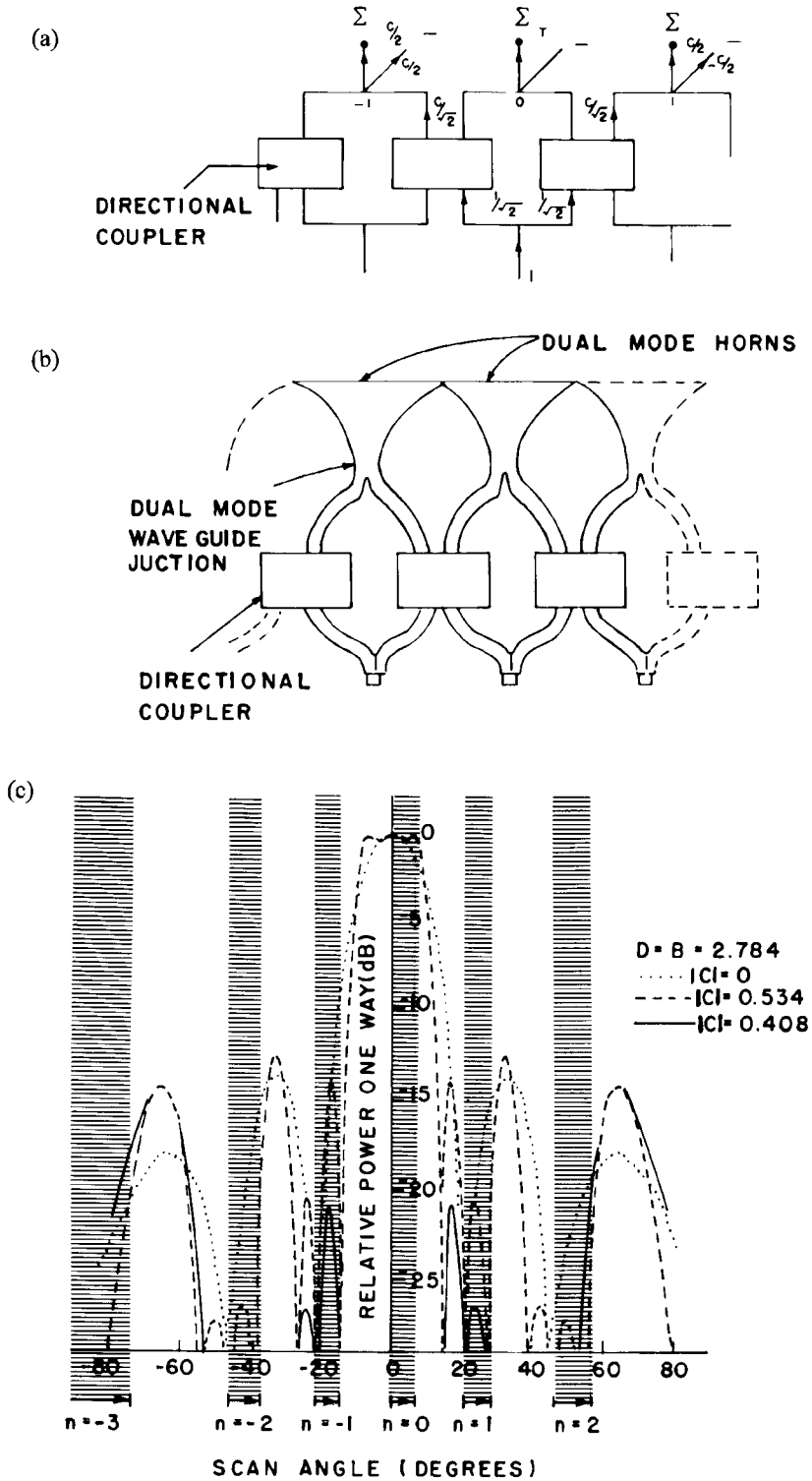
Figure 8.16 Overlapped subarray with higher order mode overlap: (a) circuit for overlapped array excitation; (b) waveguide network for overlapped array of horns; and (c) subarray pattern of overlapped elements. (From: [36]. © 1974 IEEE. Reprinted with permission.)
