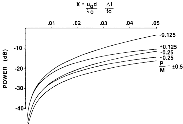
Figure 7.10 Quantization lobe power for array with time delay at subarray ports. (From: [16]. © 1984 IEEE. Reprinted with permission.)
