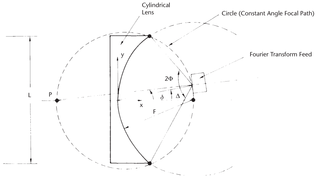
Figure 8.36 Geometry of off-axis feed and two-dimensional cylindrical lens.
