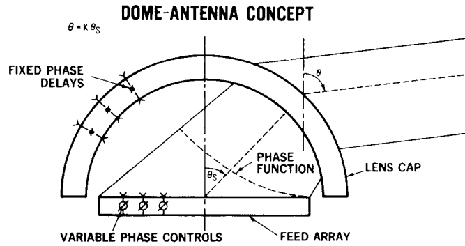
Figure 4.20 Hemispherical dome array for scan to \theta = K\theta_s .
