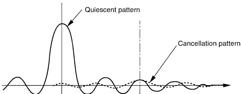
Figure 3.19 Quiescent pattern and canceler beam for single source of interference. (From: [63]. © 1976 IEEE. Reprinted with permission.)
