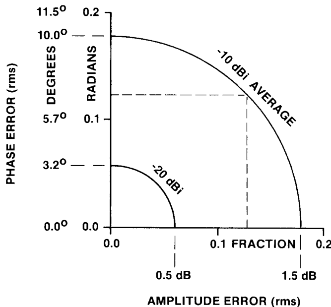
Figure 7.1 Array average (residual) sidelobes (relative to isotropic radiation) due to phase and amplitude error. Element gain \pi assumed. (After: [11].)
