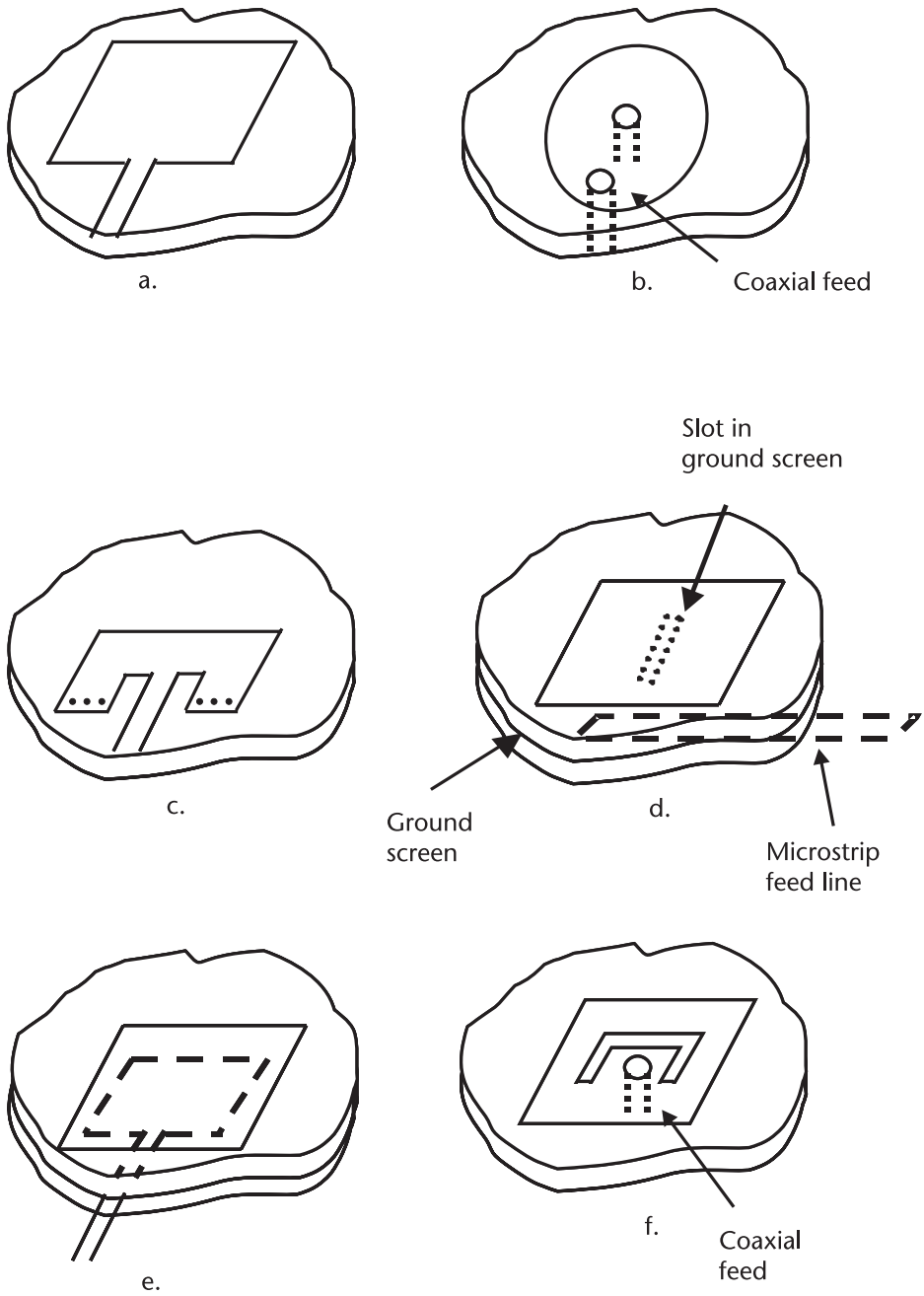
Figure 5.19 Microstrip patch elements: (a) rectangular patch with microstrip feed; (b) circular patch with coaxial feed; (c) shorted quarter-wave patch; (d) slot coupled patch; (e) electromagnetically coupled patch; and (f) coaxially fed patch with u-slot.
