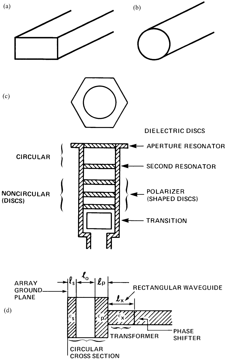
Figure 5.17 Waveguide radiating elements. (a) Rectangular waveguide. (b) Circular waveguide. (c) Circularly polarized waveguide element for triangular grid array. (From: [87]. © 1968 IEEE. Reprinted with permission.) (d) Doubly tuned waveguide element. (From: [88]. © 1974 IEEE. Reprinted with permission.)
