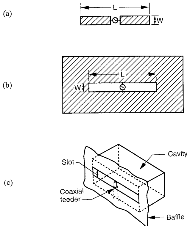
Figure 5.15 Fundamental slot and dipole strip antennas: (a) strip dipole; (b) equivalent slot in ground screen; and (c) cavity-backed slot antenna.
