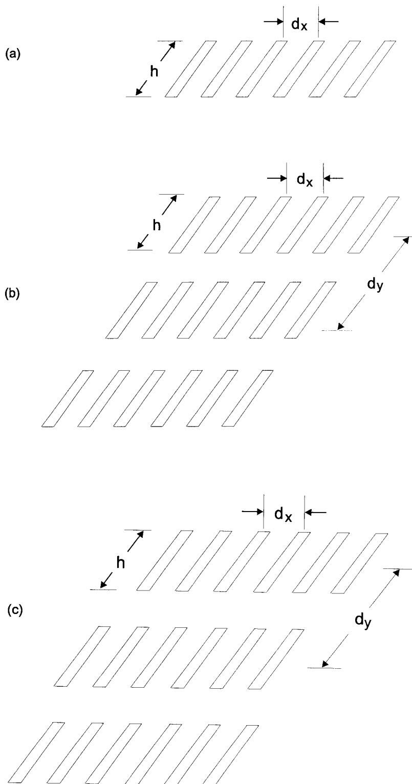
Figure 6.4 Infinite array geometries: (a) one-dimensional array; (b) two-dimensional array on a rectangular grid; and (c) two-dimensional array on a triangular grid.
