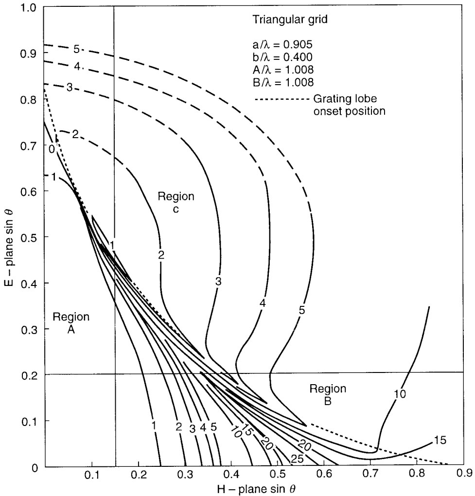
Figure 6.7 Contour map (in decibels) of scanned peak of power pattern. (After: [20].)
