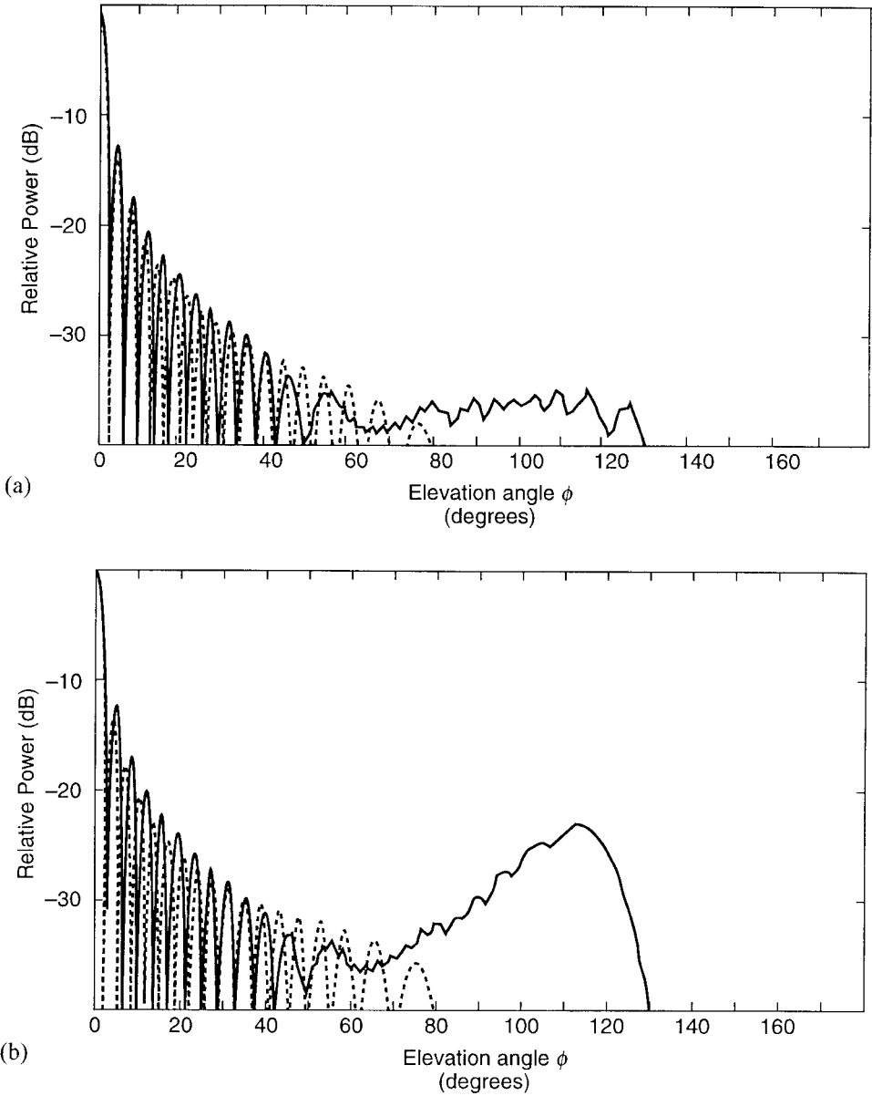
Figure 4.13 Patterns of uniformly illuminated sector arrays on cylinders with radius 11.46\lambda ( 90^\circ sector—solid curve) and 200\lambda (dashed curve): (a) 36-element array with 0.5\lambda spacing; and (b) 30-element array with 0.6\lambda spacing.
