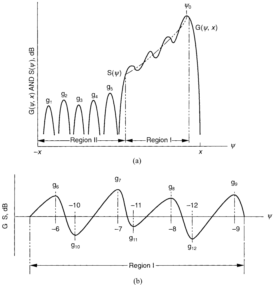
Figure 3.13 Synthesis of shaped power pattern: (a) complete pattern showing shaped region, sidelobe region, desired contour (dashed), and sidelobe topography; and (b) ripple peaks and troughs in region I relative to the desired contour. (From: [33]. © 1984 IEEE. Reprinted with permission.)
