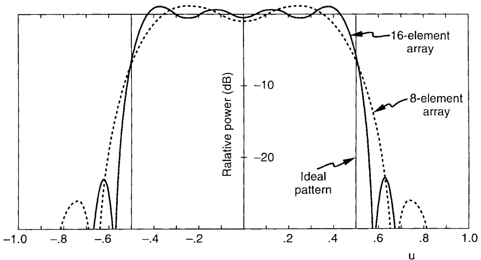
Figure 3.1 Fourier series synthesized representation of pulse-shaped pattern (solid curves for ideal and pattern of 16-element array, dashed curve for 8-element array).
