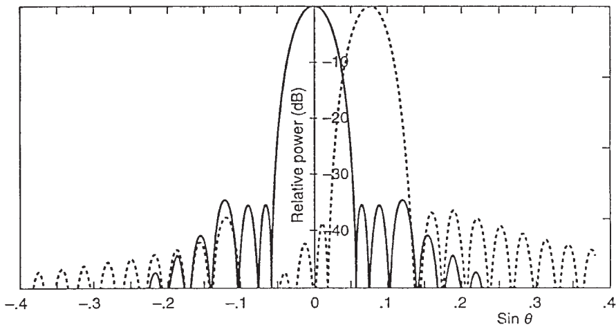
Figure 8.24 Limited field-of-view scanning of constrained overlapped subarray feed (64-element array and 8 subarrays with -40 -dB Chebyshev illumination).
