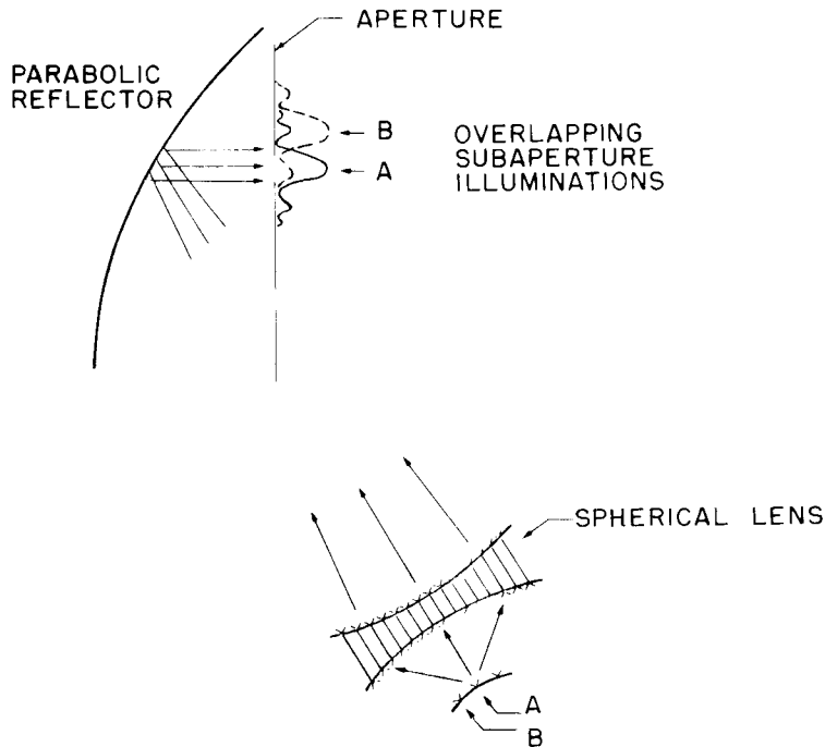
Figure 8.29 Lens/reflector geometry for completely overlapped subarray system. (From: [69]. © 1975 IEEE. Reprinted with permission.)
