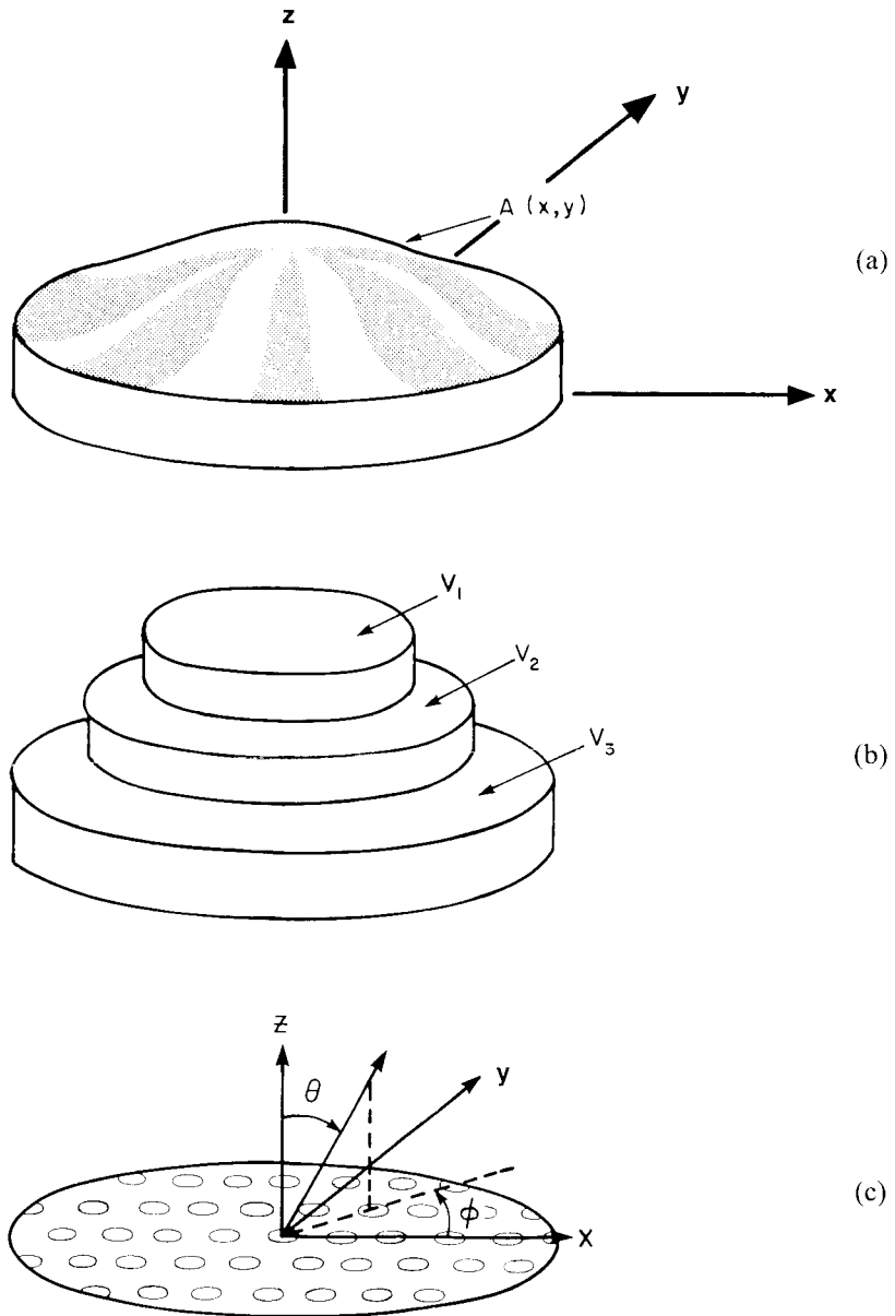
Figure 2.15 Array with quantized amplitude taper: (a) array amplitude taper A(x, y) ; (b) quantized amplitude taper; and (c) array aperture and coordinates. (From: [40]. © 1991 IEEE. Reprinted with permission.)
