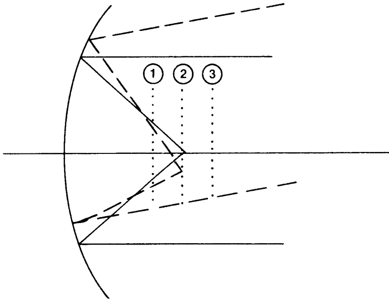
Figure 8.25 Feed plane locations for a scanned reflector: (1) feed at plane closer than focal plane (plane 1); (2) feed at plane passing through focal point; (3) feed at plane beyond focal plane.
