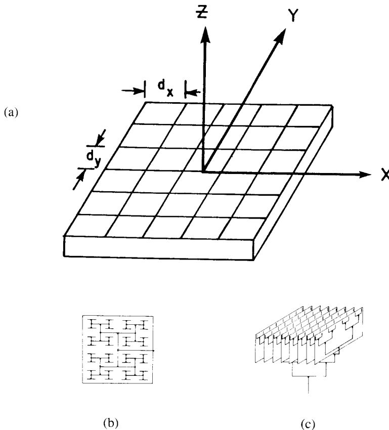
Figure 1.8 Array geometry for two-dimensional scanning: (a) generalized planar array geometry; (b) equal line-length planar feed; and (c) equal line-length column feeds.
