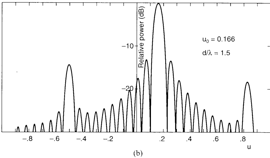
Figure 8.15 Phase interpolation networks for limited field of view. (a) Basic network and signal amplitude at interpolated port. (b) End-of-scan pattern for 21-element array ( u_0=0.166 and 1.5\lambda between subarrays). (From: [43]. © 1970 IEEE. Reprinted with permission.)
