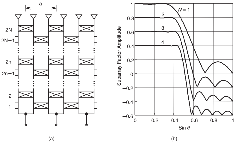
Figure 8.18 Subarray factors for various cascaded chess networks: (a) the N -cascaded chess network; and (b) subarray factor for the case of 1, 2, 3, and 4 optimized cascades. (After: [42].)
