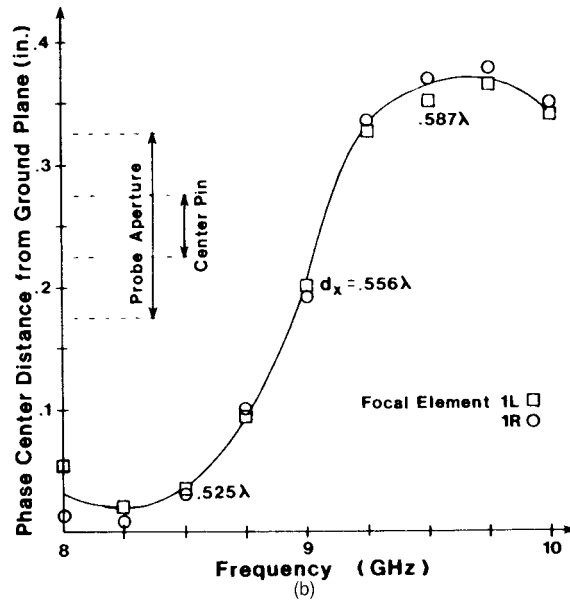
Figure 8.39 Element pattern characteristics for microwave lens feeds. (a) Monopole characteristics in array. (After: [80].) (b) Phase center location versus frequency ( 0.556\lambda spacing). (From: [77]. © 1986 IEEE. Reprinted with permission.)
