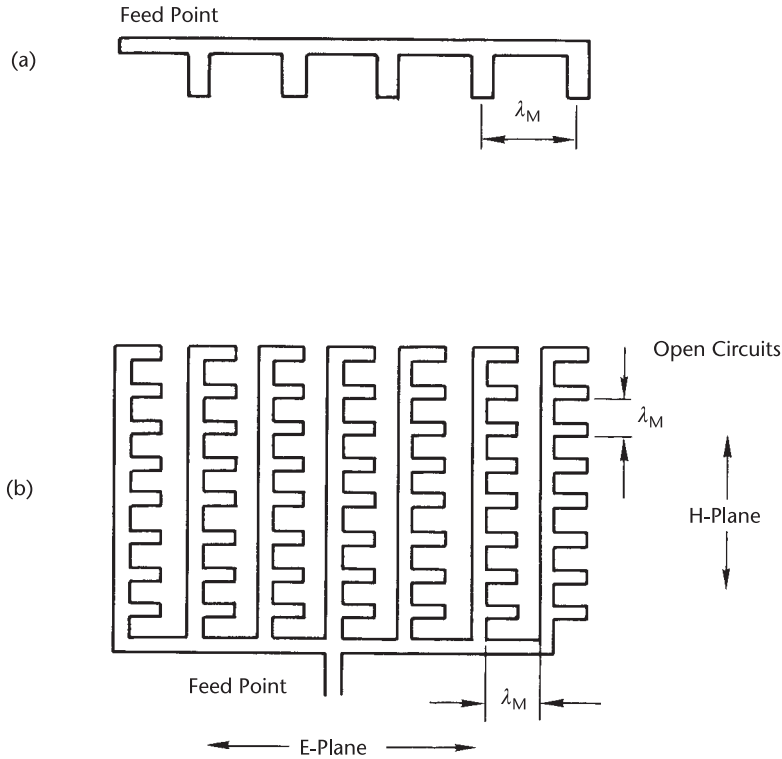
Figure 5.26 Comb line arrays: (a) series-fed comb line array; and (b) planar array of series-fed comb line arrays. (From: [149]. © 1977 IEEE. Reprinted with permission.)
