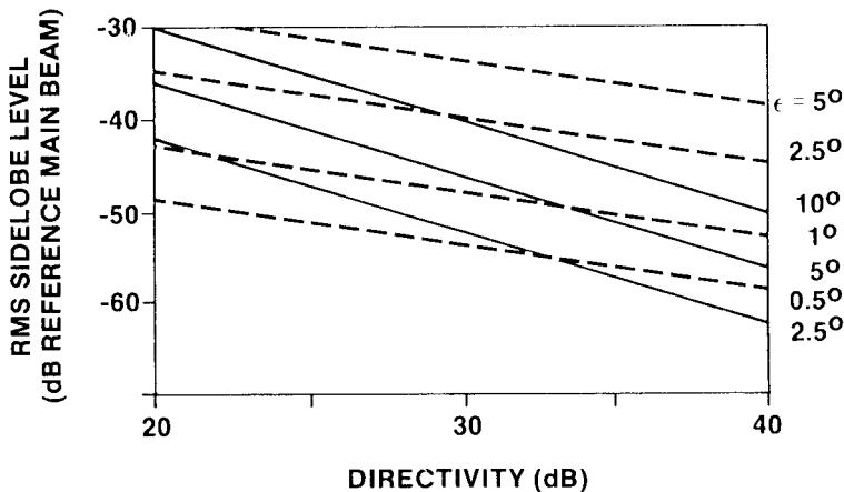
Figure 7.2 Average sidelobes due to phase error (relative to beam peak) for a square array. Element gain \pi assumed. Solid line for two-dimensional array of independent phase shifters, dashed line for array of columns. (After: [12].)
