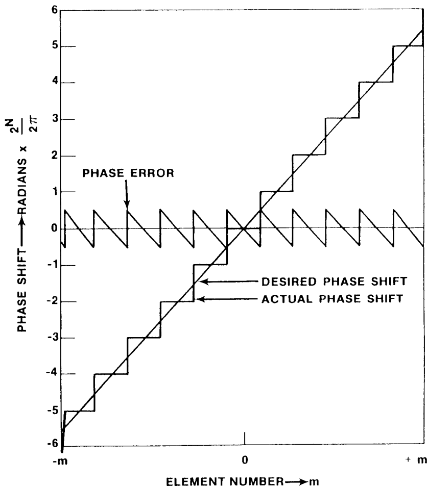
Figure 7.5 Phase error due to phase quantization. (After: [17].)
