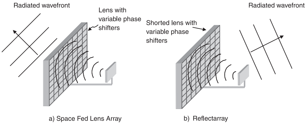
Figure 1.20 Array space feed networks: (a) space-fed lens array; and (b) reflectarray.
