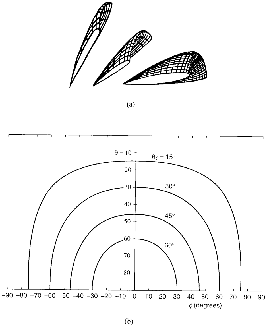
Figure 2.8 Beam shape for scanned fan beam and pencil beam arrays: (a) beam shape versus scan angle for fan beam (linear array) antenna; (b) beam peak contours near endfire; and (c) beam shape versus scan position for a pencil beam. (From: [10]. © 1985 Peninsula Publishing Company. Reprinted with permission.)
