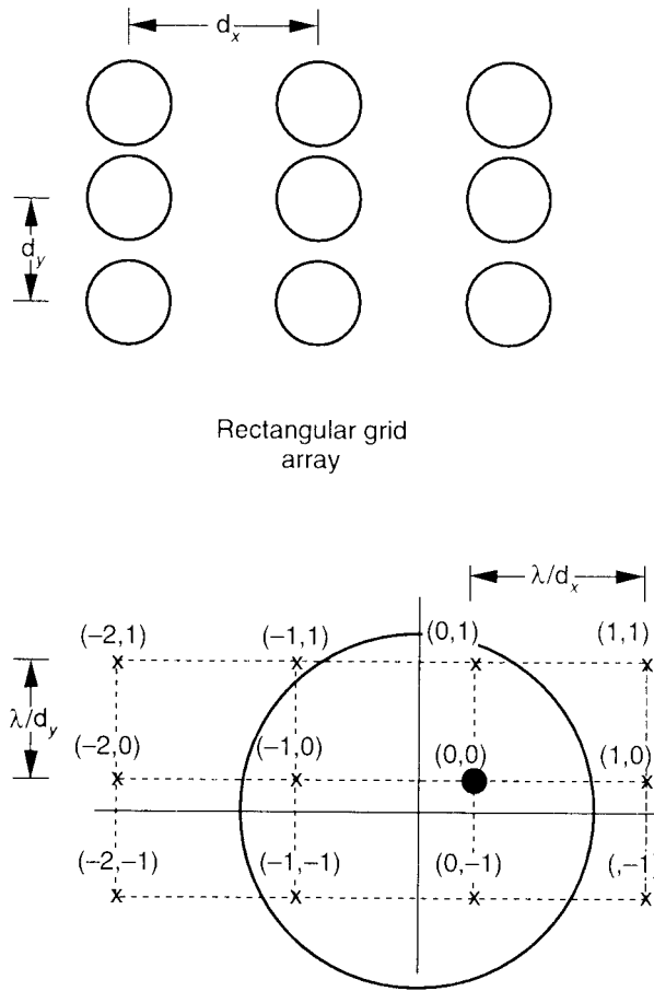
Figure 1.13 Grating lobe spectrum for planar arrays with rectangular grids.
