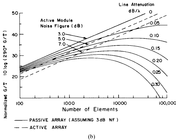
Figure 1.16 Gain and G/T limitations due to circuit losses: (a) passive array gain; and (b) passive and active array G/T (assuming matched array).
