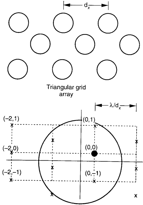
Figure 2.10 Geometry and grating lobe lattice of a triangular grid array.
