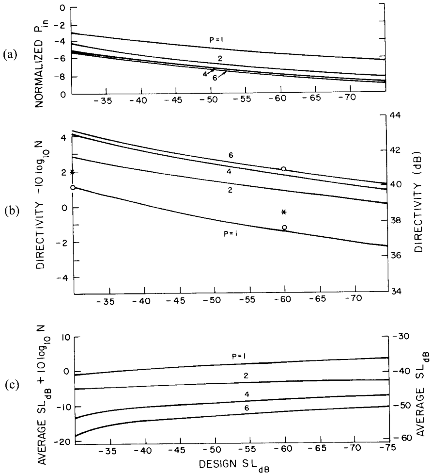
Figure 2.19 (a) Input power, (b) directivity, and (c) average sidelobe level for method 2 (quantization). (From: [40]. © 1991 IEEE. Reprinted with permission.)
