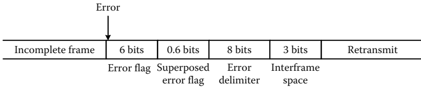
FIGURE 13.5 Error frame format in CAN.
