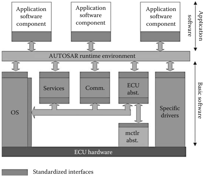
FIGURE 4.5 AUTOSAR reference architecture.
