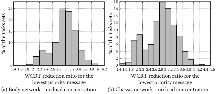
FIGURE 14.3 Reduction ratio of the WCRT for the lowest priority frames when offsets are used. The distribution is computed over the results obtained on a sample of 1000 random body networks (left-hand graphic) and chassis networks (right-hand graphic). The network load is uniformly distributed over the ECUs (i.e., no concentration). The x -axis is the WCRT reduction ratio (bins of size: 0.2) and the y -axis is the percentage of networks having that level of gain.
