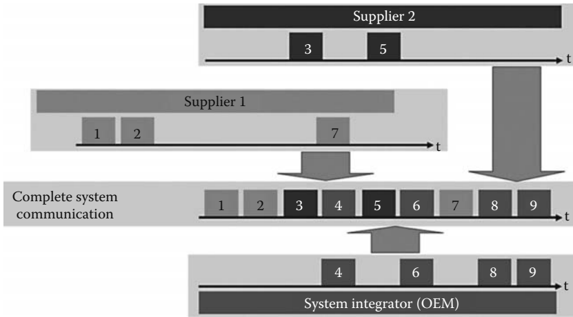
FIGURE 5.4 Example of FlexRay compossability. (Copyright by DECOMSYS, Member of Elektrobit. With permission.)
