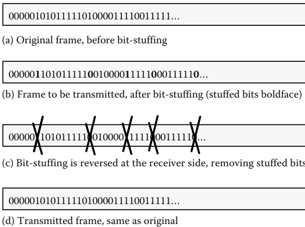
FIGURE 13.6 Bit-stuffing example; from sender to receiver.
