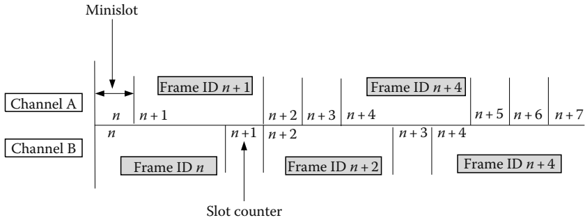
FIGURE 4.2 Example of message scheduling in the dynamic segment of the FlexRay communication cycle.
