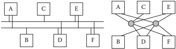
FIGURE 5.7 Bus topology (left) and active star topology (right).
