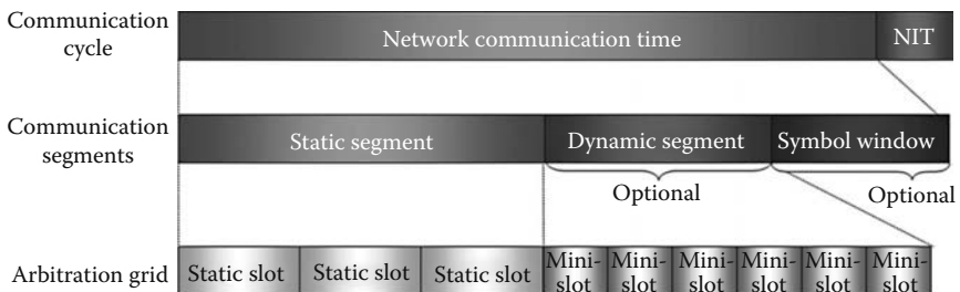
FIGURE 5.2 FlexRay communication cycle. (Copyright by DECOMSYS, Member of Elektrotbit. With permission.)
