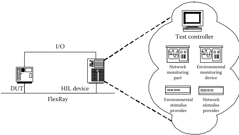
FIGURE 12.13 Test setup for closed-loop approach.
