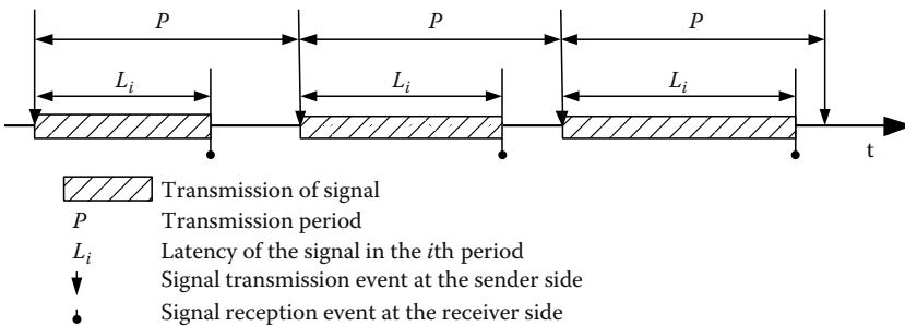
FIGURE 12.3 Characteristics for a periodic signal exchange.
