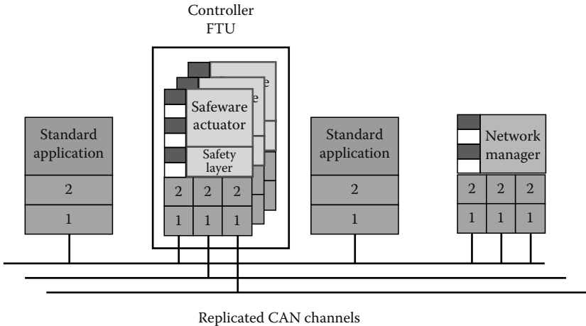
FIGURE 6.13 The FlexCAN architecture.
