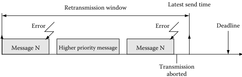
FIGURE 6.17 Typical TCAN message transmission scenario.
