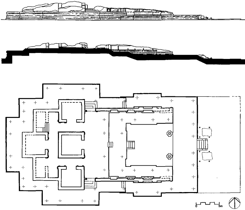
96 Plan, section and elevation of excavated residence, royal centre, Vijayanagara, fifteenth–sixteenth centuries
