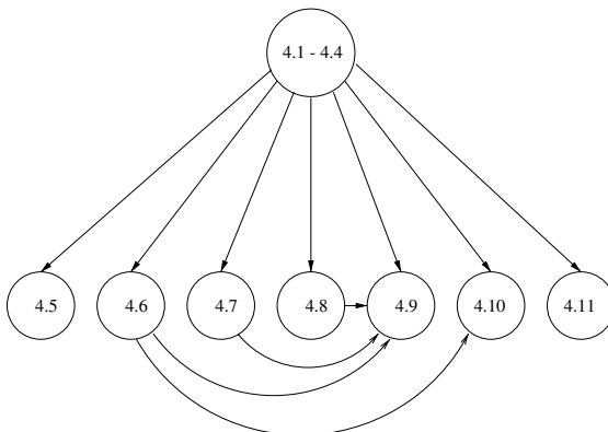
Figure 4.3: The dependence structure of this chapter.
