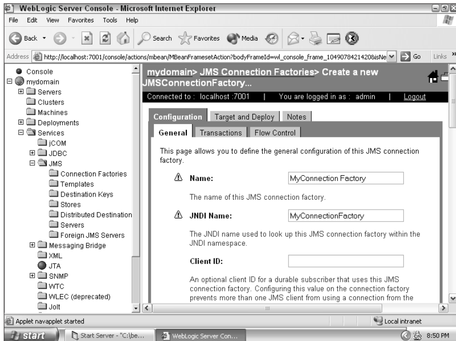
Figure 15-2: A new connection factory.
