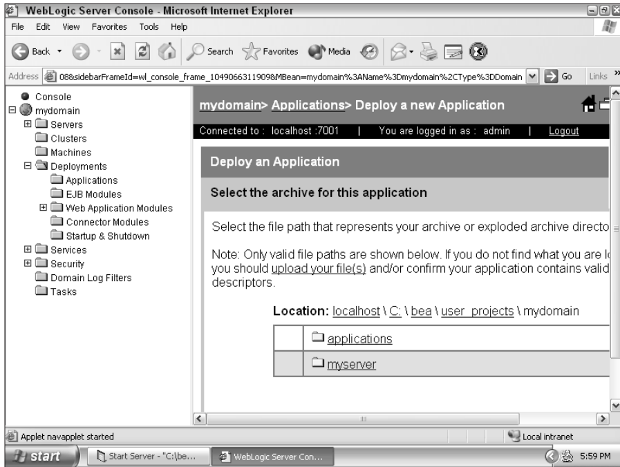
Figure 8-2: Deploying a new application.
