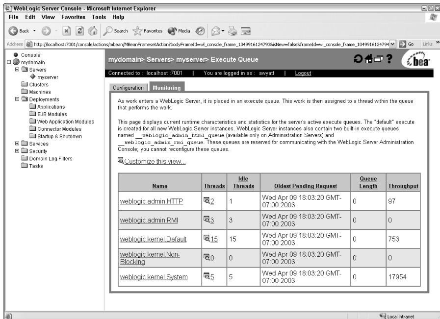
Figure 17-3: Active queues.
