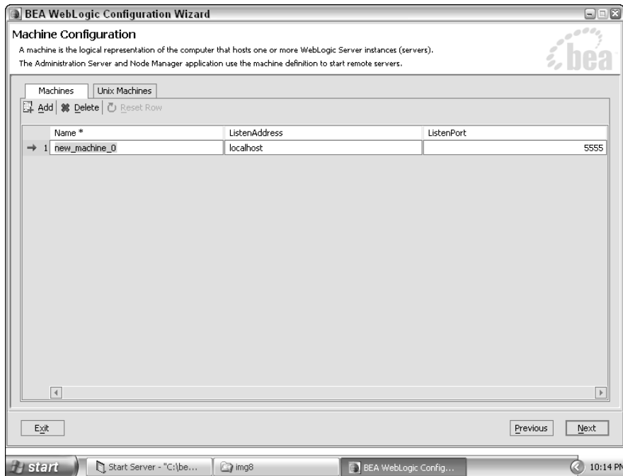
Figure 16-7: Configure machines.
