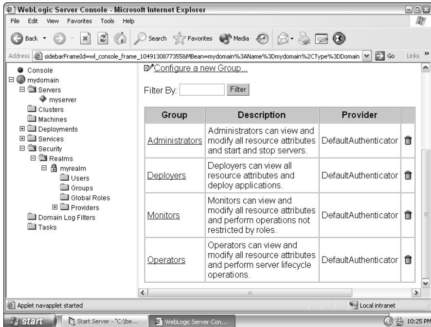
Figure 18-8: Realm groups.
