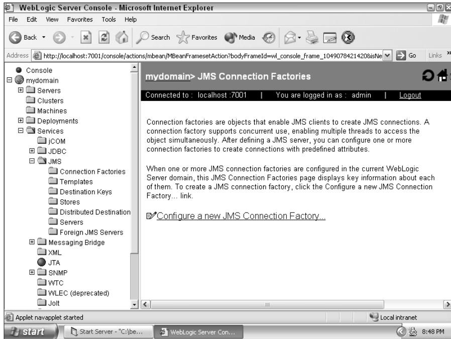
Figure 15-1: All current connection factories.
