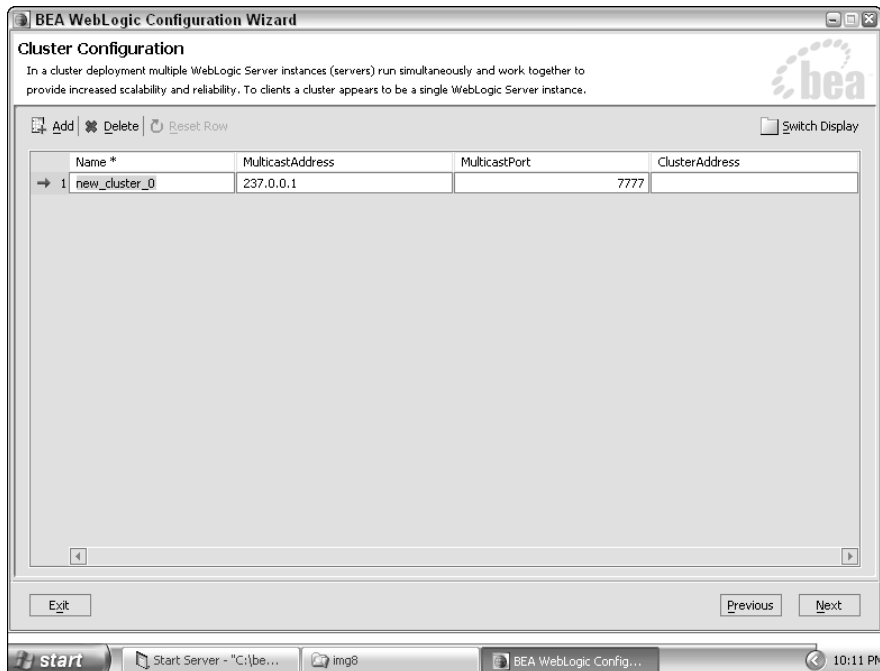
Figure 16-5: Configure the cluster.
