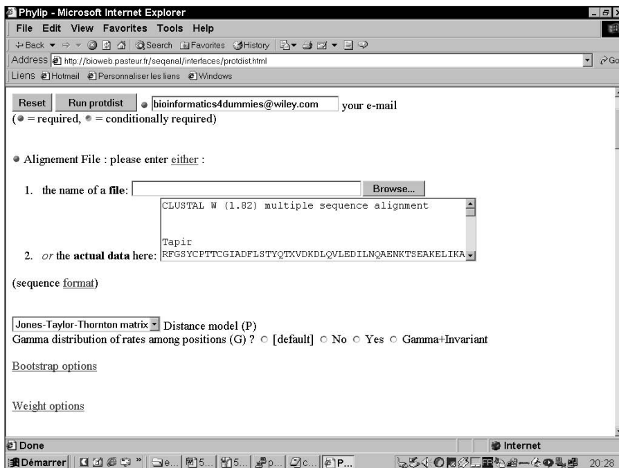
Figure 13-8: ProtDist server.
