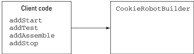
Figure 7-7: Separating out the construction code into the Cookie Robot Builder class.
