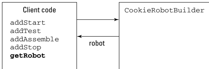
Figure 7-8: Sending the robot to the client code.
