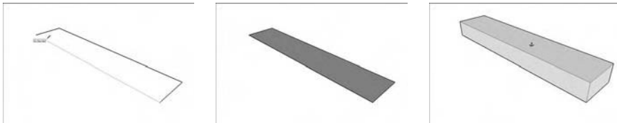
Figure 4-26: Model a single step, making sure that the depth and height are accurate.
