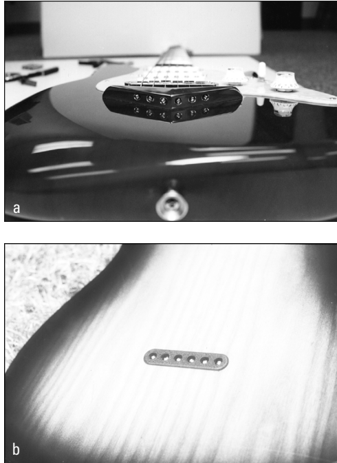
Figure 17-6: Strings pass through the bridge in the direction of the headstock (a). Strings pass through the bridge from the back of the guitar (b).
