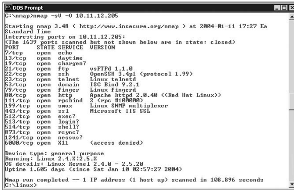
Figure 11-5: Using Nmap to determine the OS kernel version of a Linux server.
