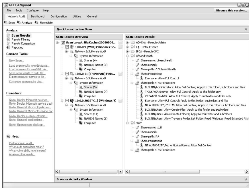
Figure 10-10: Using LANguard's share finder to seek out Windows shares.
