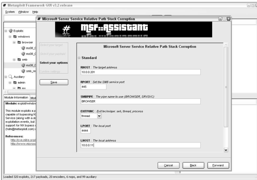
Figure 10-16: Entering required remote and IP address.
