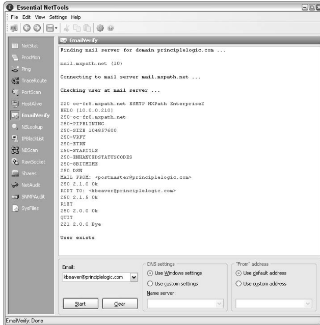
Figure 13-7: Using EmailVerify to verify an e-mail address.
