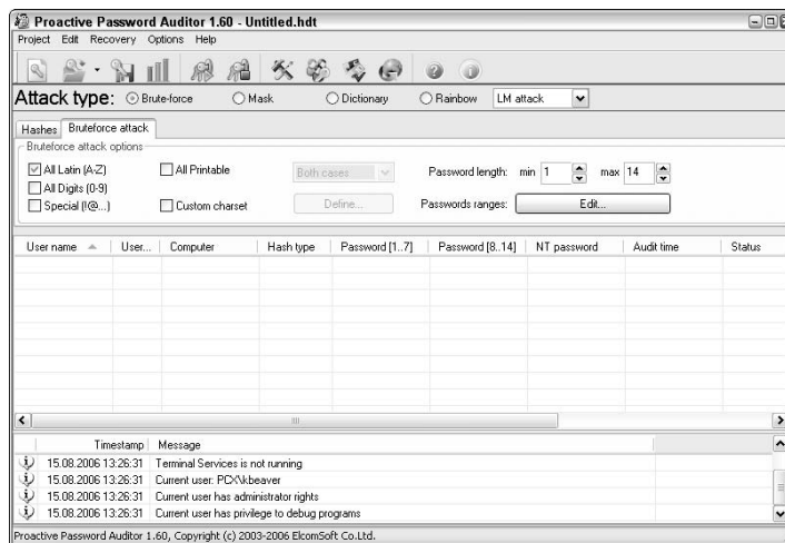
Figure 7-1: Brute-force password-cracking options in Proactive Password Auditor.
