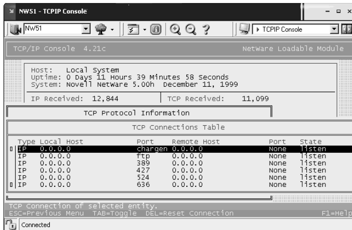
Figure 12-7: Using tcpcon to show open TCP ports on a NetWare server.
