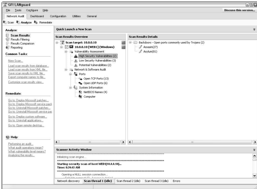
Figure 10-2: Gathering detailed vulnerabilities of a Windows Server with LANguard.
