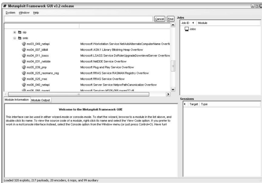
Figure 10-13: Browsing the available exploits.
