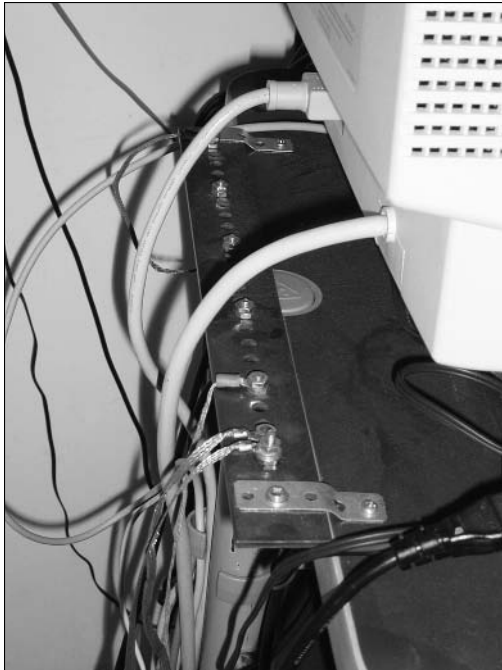
Figure 13-10: A copper ground bus installed in my shack.
