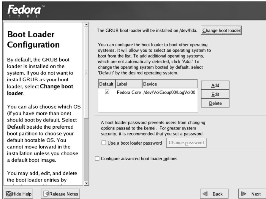
Figure 3-8: The Boot Loader Configuration screen.
