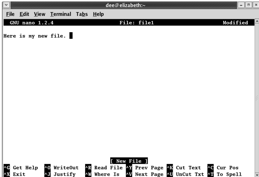
Figure 16-1: The file file1 open in the nano editor in Fedora Core 3.
