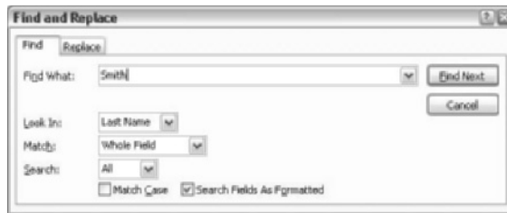
Figure 3-4: Finding data.
