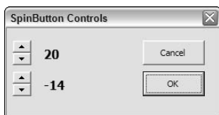
Figure 17-15: SpinButton controls.
