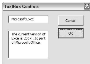
Figure 17-16: TextBox controls.
