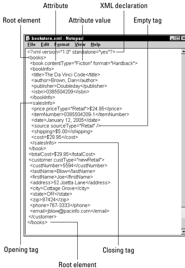
Figure 5-1: Dissecting the different parts of a well- formed XML document.
