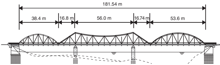
FIG 30. Flisa Bridge, Norway
