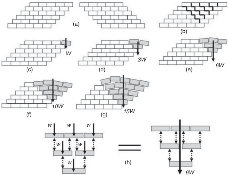
FIG 9. Behaviour of a corbel wall
