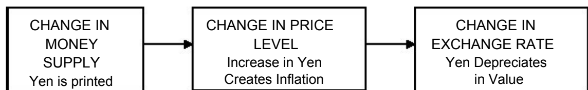
Figure 3.5 Monetary Model
