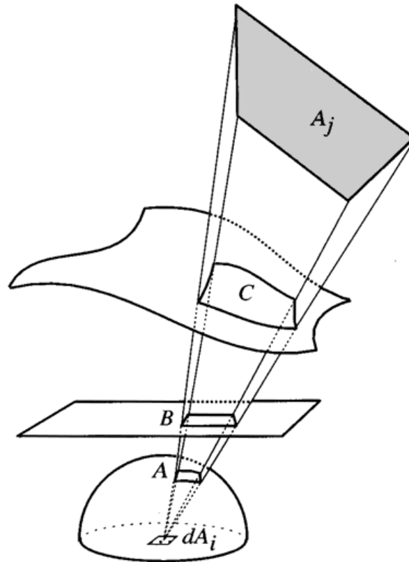
Figure 4.9: Areas with same form factor. Areas A , B , and C , have the same form factor as A_i from dA_i .
