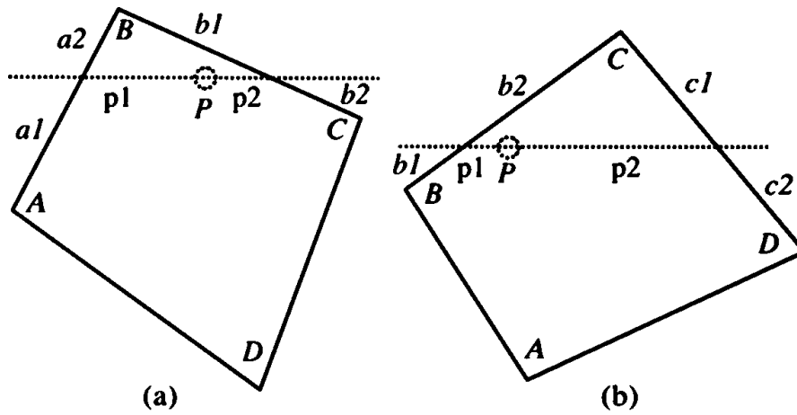
Figure 9.7: Gouraud interpolation.
