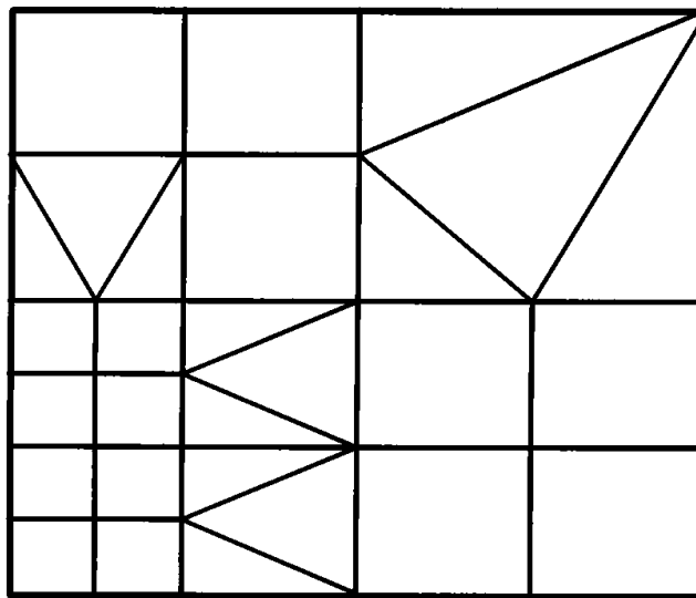
Figure 8.7: Tri-quadtree used to eliminate t -vertices.
