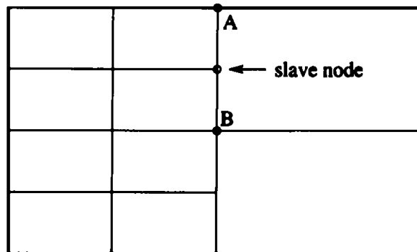
Figure 8.6: T -vertices treated as slave nodes.
