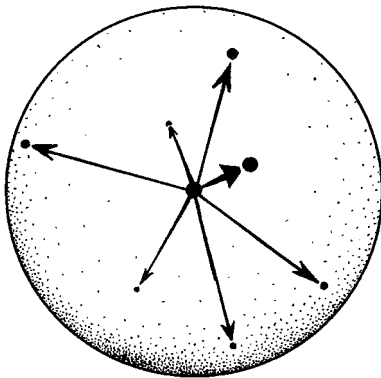
Fig. 22.14 Majorana’s description of the general (projective) spin state for a massive particle of spin \frac{n}{2} , given by n unordered points on the Riemann sphere. We can think of these points to be contributing spin \frac{1}{2} , in accordance with the prescription of Fig. 22.10. The symmetrical product of these spins gives the total. (In 2-spinor notation, the complete spin state is the symmetric n -valent spinor, which factorizes \psi_{AB\dots F} = \alpha_{(A}\beta_B \cdots \varphi_F) , where \alpha_A, \beta_A, \dots, \varphi_A , determine the n points, as in Fig. 22.10.)
