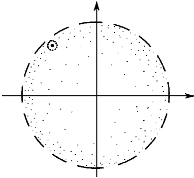
Fig. 7.4 The open unit disc |z| < 1 . Any point strictly inside, no matter how close to the circumference, is surrounded by much smaller circle whose interior still lies strictly within unit circle. On the other hand, for the closed disc |z| \leq 1 , this fails for points on the boundary.
