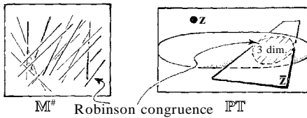
Fig. 33.14 We can obtain a ‘real’ picture of a non-null twistor Z^z by first passing to its complex conjugate Z_\alpha , thus defining a complex projective plane in \mathbb{P}^3\mathbb{T} . This plane is fixed by its intersection with \mathbb{P}^3\mathbb{N} , which is a 3-real-dimensional locus. This locus defines a 3-parameter family of light rays in \mathbb{M}^\# called a Robinson congruence.
