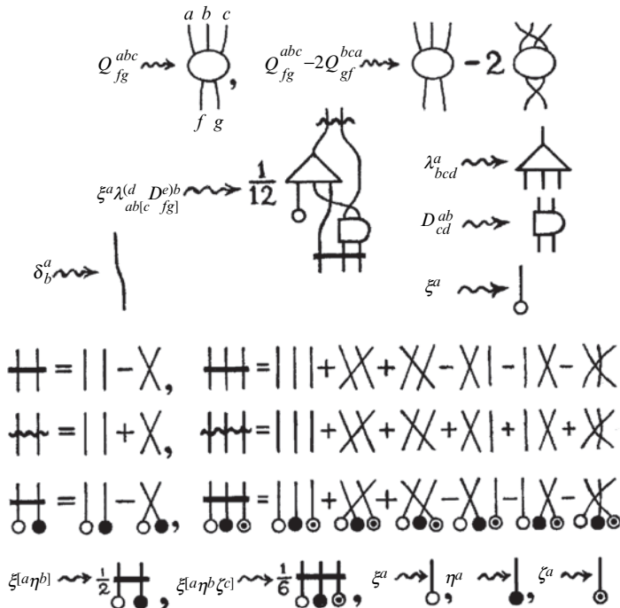
Fig. 12.17 Diagrammatic tensor notation. The [\frac{3}{2}] -valent tensor Q is represented by an oval with 3 arms and 2 legs, where the general [\frac{p}{q}] -valent tensor picture would have p arms and q legs. In an expression such as Q_{fg}^{abc} - 2Q_{gf}^{bca} , the diagrammatic notation uses positioning on the page of the ends of the arms and legs to keep track of which index is which, instead of employing individual index letters. Contractions of tensor indices are represented by the joining of an arm and a leg, as illustrated in the diagram for \xi^a \lambda_{ab}^{(d} D_{c}^{e)b} . This diagram also illustrates the use of a thick bar across index lines to denote antisymmetrization and a wiggly bar to represent symmetrization. The factor \frac{1}{12} in the diagram results from the fact that (to facilitate calculations) the normal factorial denominator for symmetrizers and antisymmetrizers is omitted in the diagrammatic notation (so here we need \frac{1}{2!} \times \frac{1}{3!} = \frac{1}{12} ). In the lower half of the diagram, antisymmetrizers and symmetrizers are written out as ‘disembodied’ expressions (by use of the diagrammatic representation of the Kronecker delta \delta_b^a that will be introduced in §13.3, Fig. 13.6c). This is then used to express the (multivector) wedge products \xi \wedge \eta and \xi \wedge \eta \wedge \zeta .
