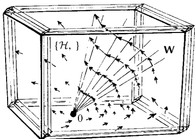
Fig. 22.2 The Hamiltonian flow \{\mathcal{H},\} (a vector field) defines an infinitesimal linear transformation of state space \mathbf{W} , giving the change in the state after an infinitesimal time. To get the (unitary) change after a finite time, we must ‘exponentiate’ this infinitesimal Hamiltonian action.
