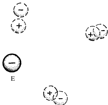
Fig. 26.10 Vacuum polarization: the physical basis of charge renormalization. The electron E induces a slight charge separation in virtual electron–positron pairs momentarily created out of the vacuum. This somewhat reduces E’s effective charge from its bare value—unfortunately by an infinite factor, according to direct calculation.
