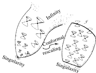
Fig. 33.8 The null-cone structure of a Lorentzian manifold \mathcal{M} is equivalent to its conformal structure. A conformal rescaling of \mathcal{M} affects its metric, but not its causality properties. (A metric g conformally rescales to g' if g' = \Omega^2 g , the scalar field \Omega being everywhere positive.) In favourable circumstances, such rescalings can be useful for ‘bringing into view’ singularities and infinite regions.
