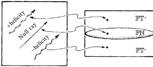
Fig. 33.6 The real 5-manifold \mathbb{IPN} divides projective twistor space \mathbb{IPT} into two complex-3-manifold pieces \mathbb{IPT}^+ and \mathbb{IPT}^- , these representing massless particles of positive and of negative helicity, respectively.
