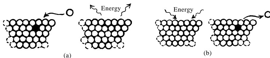
Fig. 24.3 Positrons as ‘holes’ in Dirac’s ‘sea’ of negative-energy electron states. Dirac proposed that almost all negative energy states of the electron are filled, the Pauli principle preventing an electron from falling into such a state. The occasional unoccupied such state—a ‘hole’ in this negative-energy sea—would appear as an antielectron (positron), thereby having positive energy. (a) An electron falling into such a hole would be interpreted as the annihilation of the electron and positron, with the release of energy—the sum of the positive contributions from the electron and positron. (b) In reverse, the supplying of sufficient energy to the Dirac sea could produce an electron-positron pair. (The pictures are schematic only, the lattice structure depicted having no actual relevance to Dirac’s sea.)
