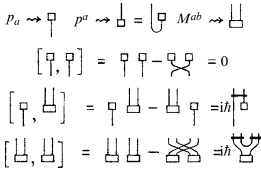
Fig. 22.18 Diagrammatic form of the relativistic 4-momentum and 6-angular momentum quantum commutators [p_a, p_b] = 0, [p_a, M^{bc}] = i\hbar(g_a^b p^c - g_a^c p^b), [M^{ab}, M^{cd}] = i\hbar(g^{bc} M^{ad} - g^{bd} M^{ac} + g^{ad} M^{bc} - g^{ac} M^{bd}).
