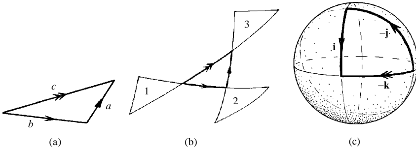
Fig. 11.4 (a) Translations in the Euclidean plane represented by oriented line segments. The double-arranged segment represents the composition of the other two, by the triangle law. (b) For rotations in Euclidean 3-space, the segments are now great-circle arcs drawn on the unit sphere, each representing a rotation through twice the angle measured by the arc (about an axis perpendicular to its plane). To see why this works, reflect the triangle made by the arcs, in each vertex in turn. The first rotation takes triangle 1 into triangle 2, the second takes triangle 2 into triangle 3, and the composition takes triangle 1 into triangle 3. (c) The quaternionic relation \mathbf{ij} = \mathbf{k} (in the form \mathbf{i}(-\mathbf{j}) = -\mathbf{k} ), as a special case. The rotations are each through \pi , but represented by the half-angle \frac{\pi}{2} .
