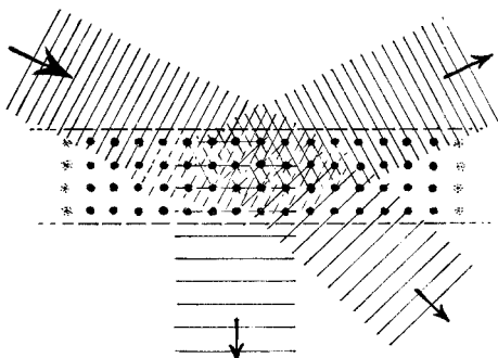
Fig. 21.2 The Davisson–Germer experiment. A beam of electrons of 3-momentum \mathbf{p} encounters a material of periodic crystalline structure. Scattering or reflection occurs when the atomic pattern matches with that of the electrons, these being regarded as waves with a wavelength \lambda related to the magnitude of the momentum p according to \lambda = h/p , where h is Planck’s constant.
