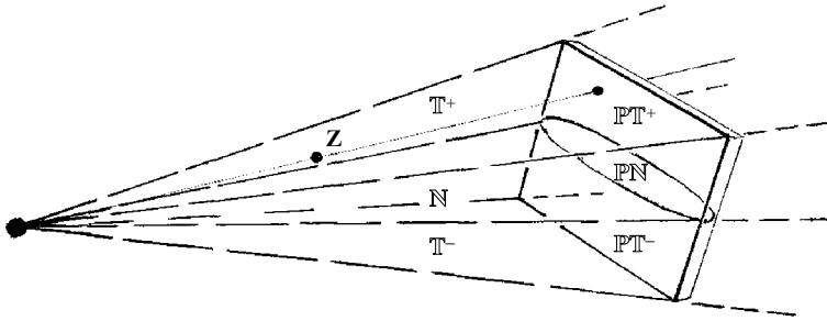
Fig. 33.11 Twistor space \mathbb{T} is a complex vector space with a pseudo-Hermitian metric. The projective twistor space \mathbb{IP}\mathbb{T} (a \mathbb{C}\mathbb{P}^3 ) is the space of rays (1-dimensional subspaces) in \mathbb{T} . Thus, if a twistor Z has coordinates (Z^0, Z^1, Z^2, Z^3) , the ratios Z^0:Z^1:Z^2:Z^3 determine the corresponding point in \mathbb{IP}\mathbb{T} . The 7-real-dimensional subspace \mathbb{N} (of null twistors: \bar{Z}_\alpha Z^\alpha = 0 ) divides twistor space \mathbb{T} into the complex 3-spaces \mathbb{T}^+ (of positive twistors: \bar{Z}_\alpha Z^\alpha > 0 ) and \mathbb{T}^- (of negative twistors: \bar{Z}_\alpha Z^\alpha < 0 ). The respective projective versions of these spaces are the 5-real-dimensional \mathbb{IP}\mathbb{N} (representing light rays in \mathbb{M}^\# ) and the two complex 3-manifolds \mathbb{IP}\mathbb{T}^+ (representing positive helicity massless particles) and \mathbb{IP}\mathbb{T}^- (representing negative helicity massless particles).
