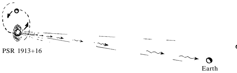
Fig. 19.9 The Hulse–Taylor double neutron star system PSR 1913 + 16. One member is a pulsar which sends out precisely timed electromagnetic signals that are received at Earth, enabling the orbits to be determined with extraordinary accuracy. It is observed that the system loses energy in exact accord with Einstein’s prediction of energy-carrying gravitational waves emitted by such a system. These waves are ripples in the spacetime vacuum, where the energy–momentum tensor vanishes. (Not to scale.)
