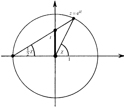
Fig. 9.9 Geometry of t = \tan \frac{\chi}{2} .
