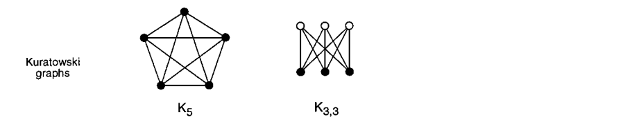
Figure 2 Some special graphs.
