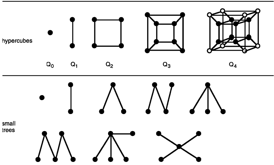
Figure 2 Some special graphs.
