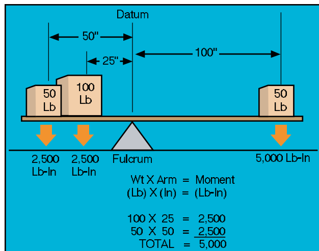
Figure 8-4. Establishing a balance.
