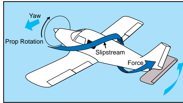
Figure 3-31. Corkscrewing slipstream.
