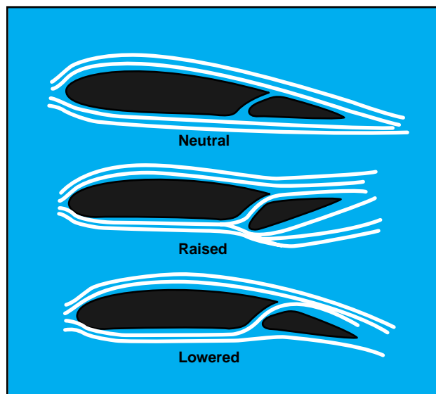
Figure 4-4. Frise-type ailerons.
