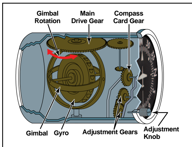
Figure 6-18. A heading indicator displays headings based on a 360° azimuth, with the final zero omitted. For example, a 6 represents 060°, while a 21 indicates 210°. The adjustment knob is used to align the heading indicator with the magnetic compass.
