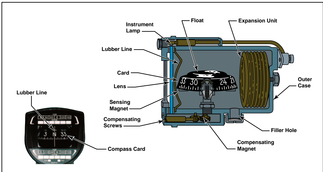
Figure 6-20. Magnetic compass.
