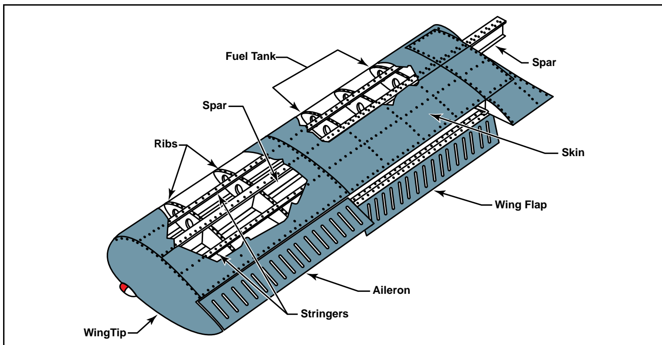
Figure 1-6. Wing components.
