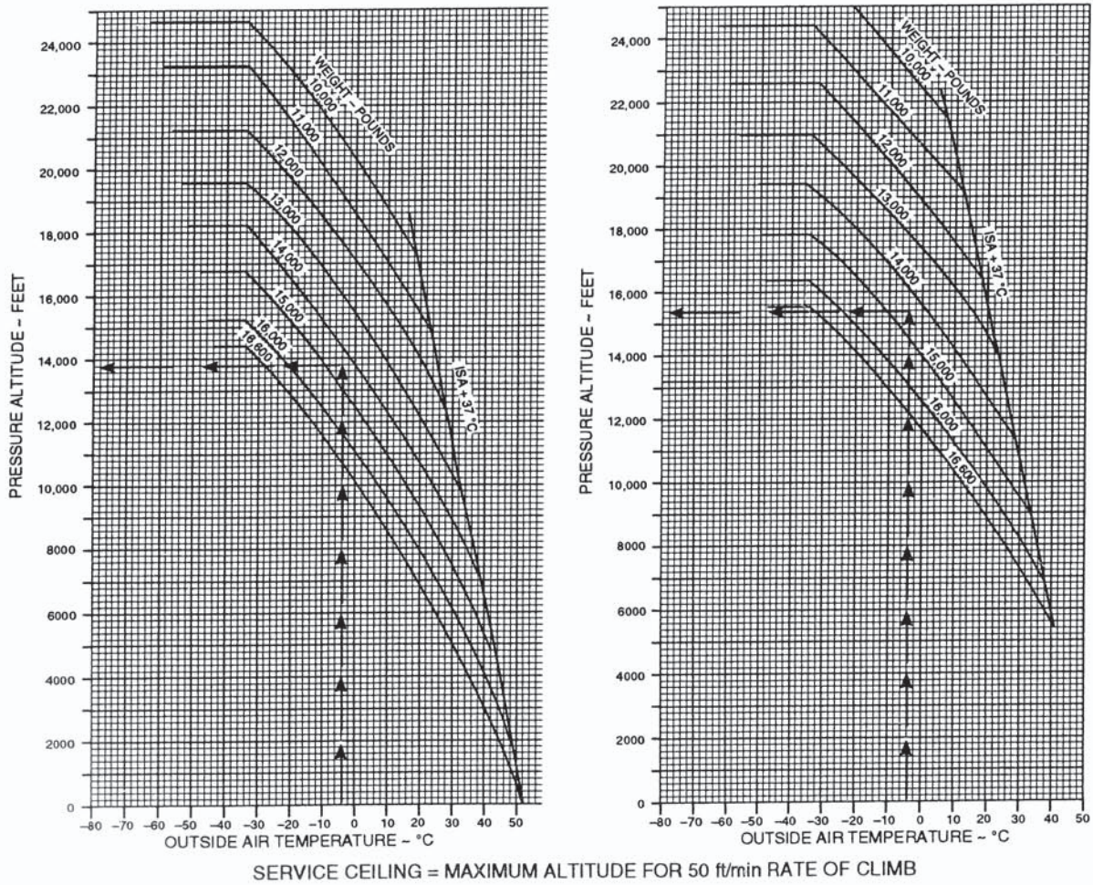
Figure 9-47. Service ceiling—One engine inoperative.
