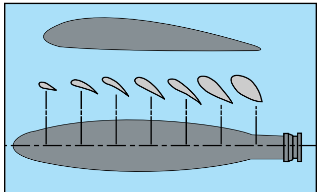
Figure 3-26. Airfoil sections of propeller blade.
