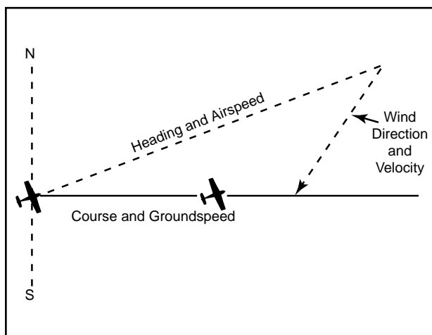
Figure 14-17. Principle of the wind triangle.
