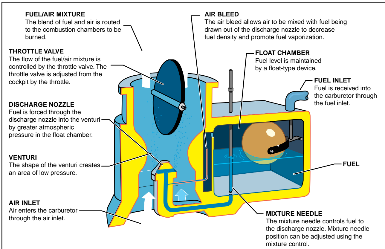
Figure 5-7. Float-type carburetor.
