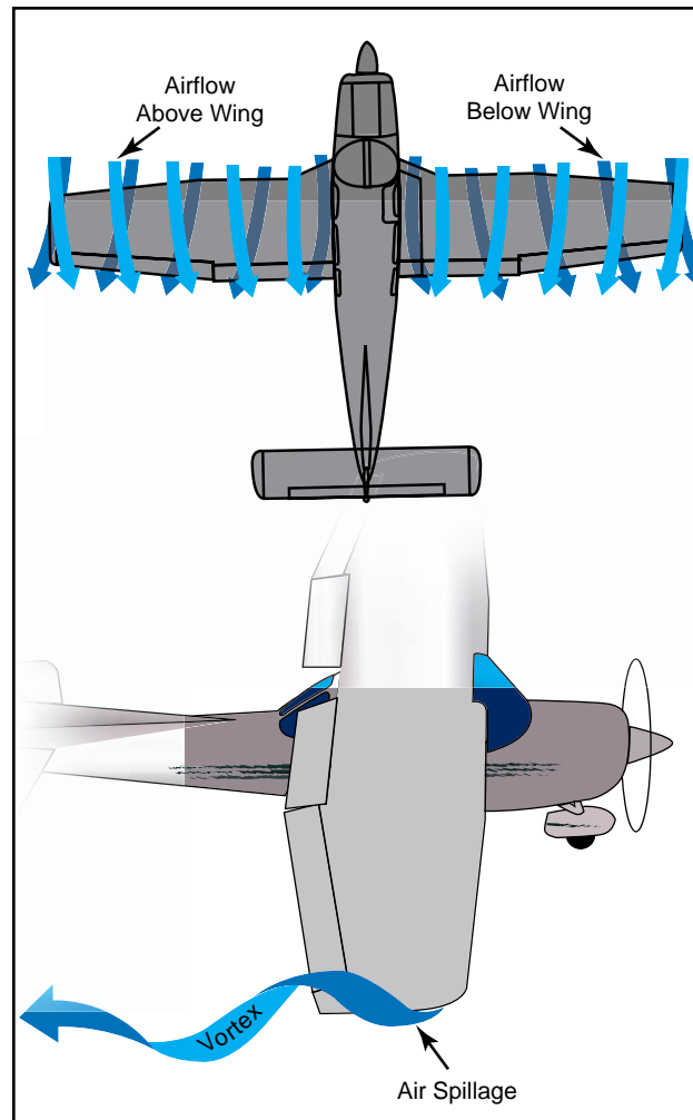
Figure 3-4. Wingtip vortices.
