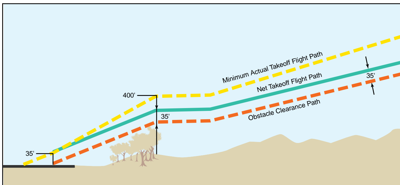
Figure 9-39. Takeoff obstacle clearance requirements.
