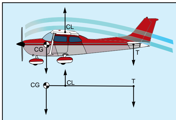
Figure 3-12. Longitudinal stability.
