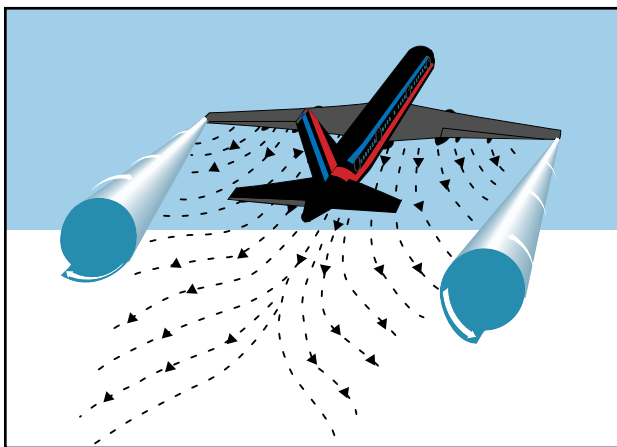
Figure 12-17. Vortex generation.
