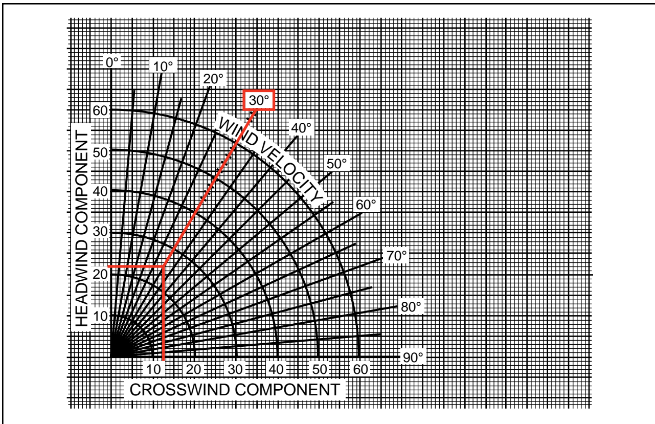
Figure 9-32. Crosswind component chart.
