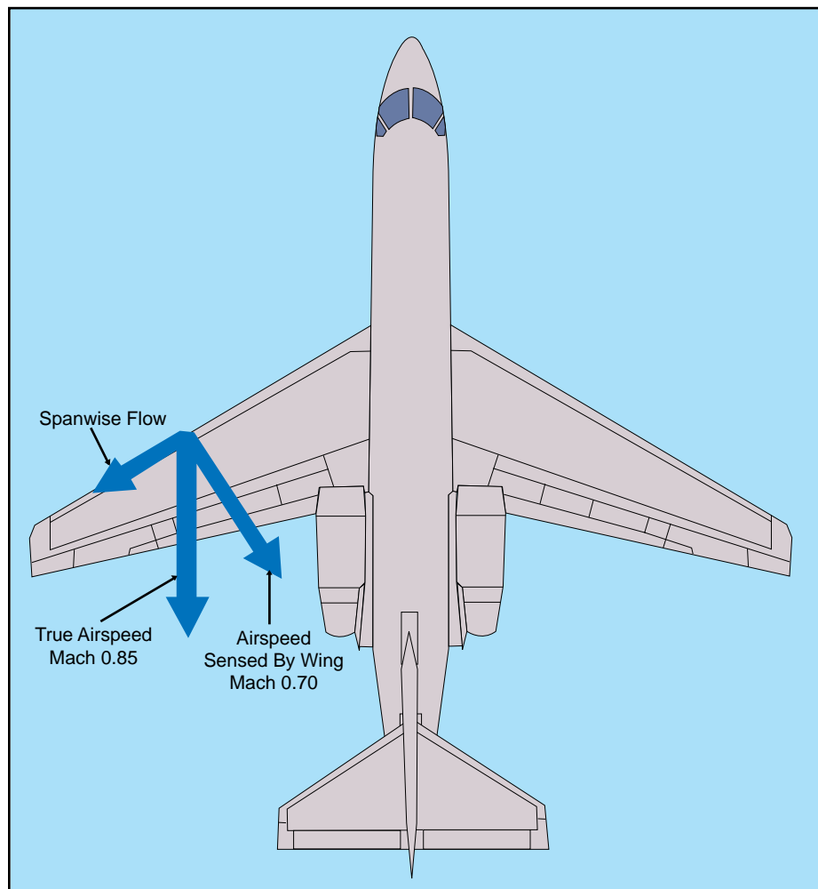
Figure 3-44. Sweepback effect.
