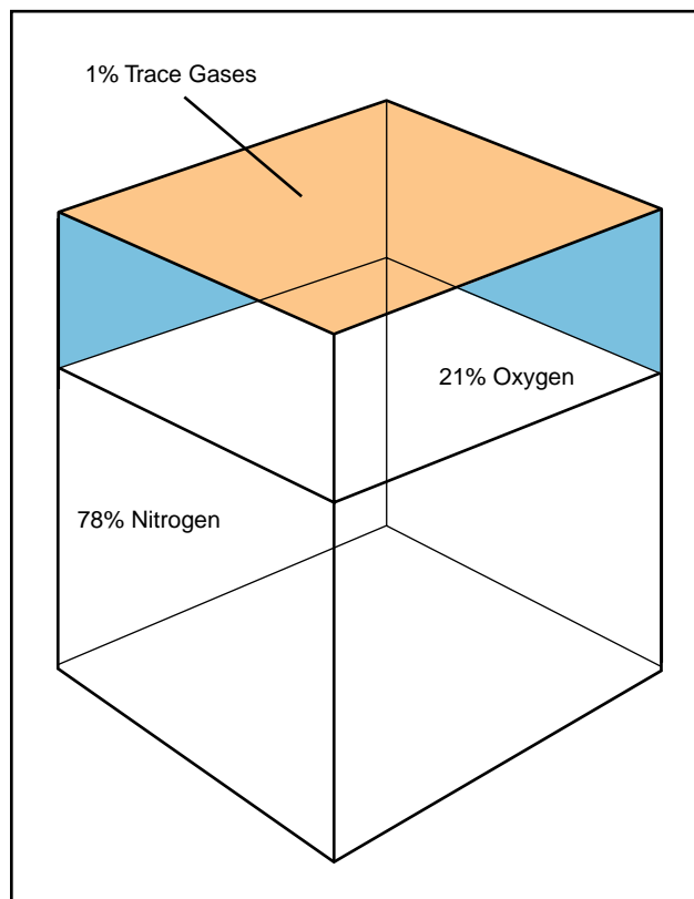
Figure 10-1. Composition of the atmosphere.
