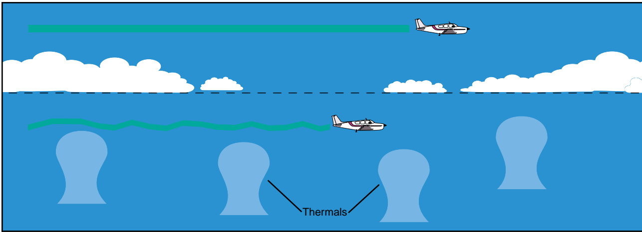
Figure 10-12. Convective turbulence avoidance.
