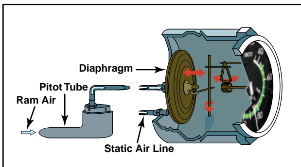
Figure 6-6. Airspeed indicator.
