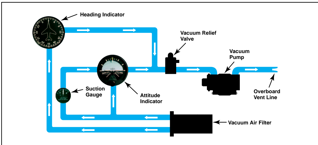
Figure 6-13. Typical Vacuum System.
