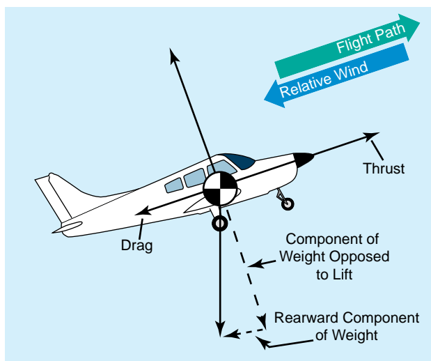
Figure 3-2. Force vectors during a stabilized climb.
