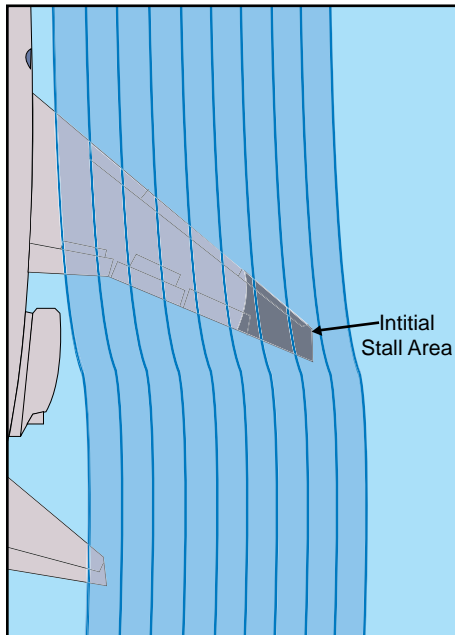
Figure 3-45 Wingtip stall.
