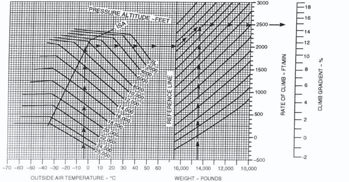
Figure 9-44. Climb – Two engines—Flaps up.
