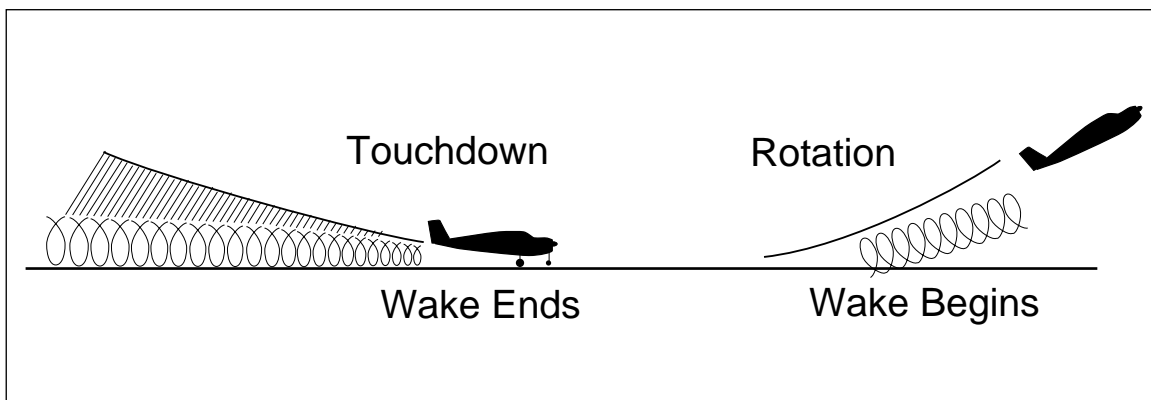
Figure 12-18. Vortex behavior.
