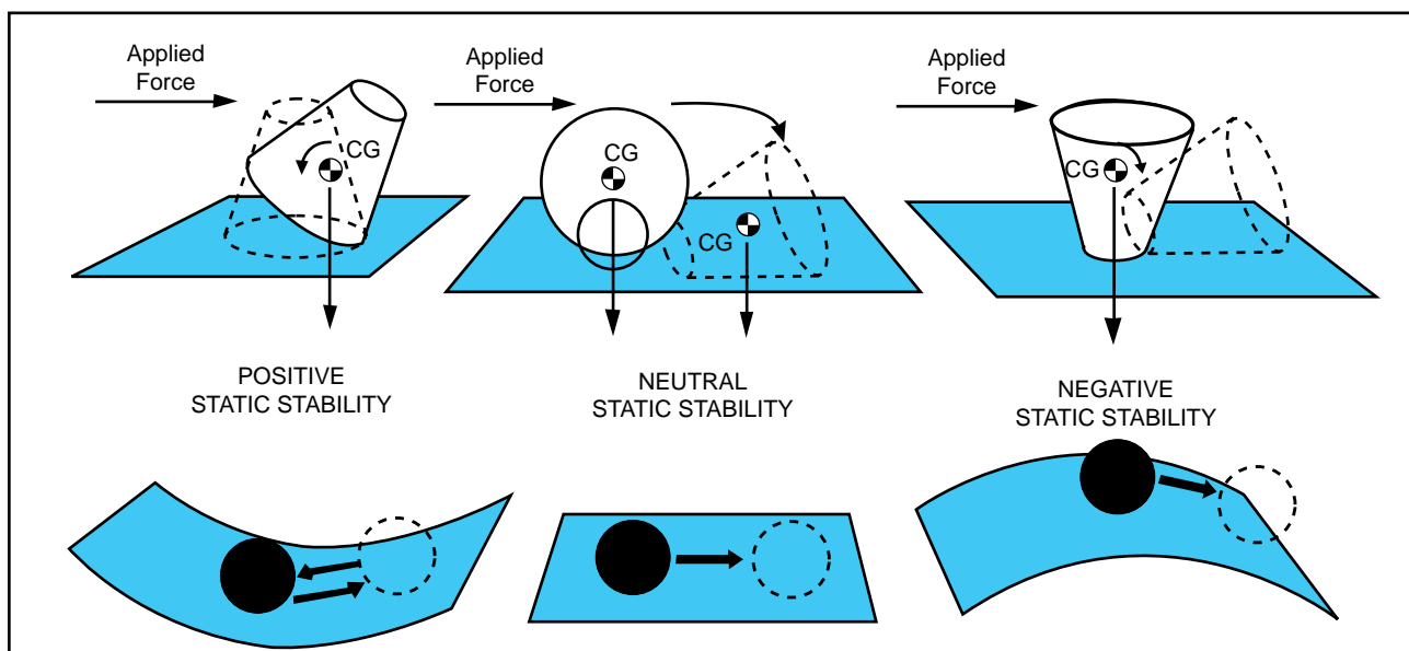
Figure 3-10. Types of stability.
