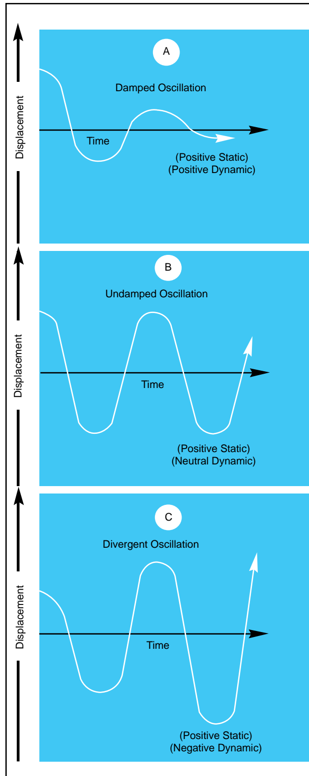
Figure 3-11. Damped versus undamped stability.
