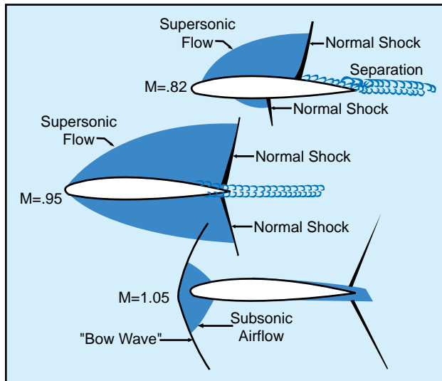
Figure 3-43. Shock waves.
