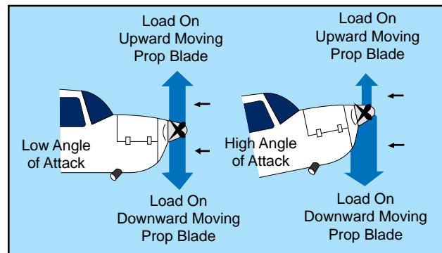
Figure 3-34. Asymmetrical loading of propeller (P-factor).
