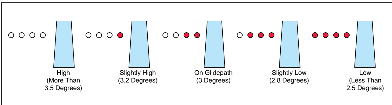
Figure 12-7. Precision approach path indicator.
