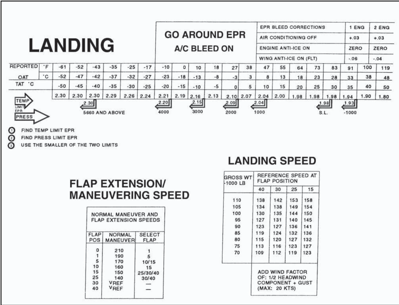
Figure 9-58. Landing performance chart.
