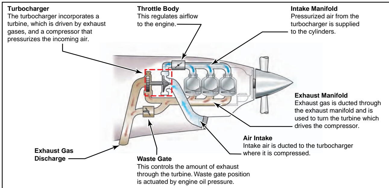
Figure 5-12. Turbocharger components.
