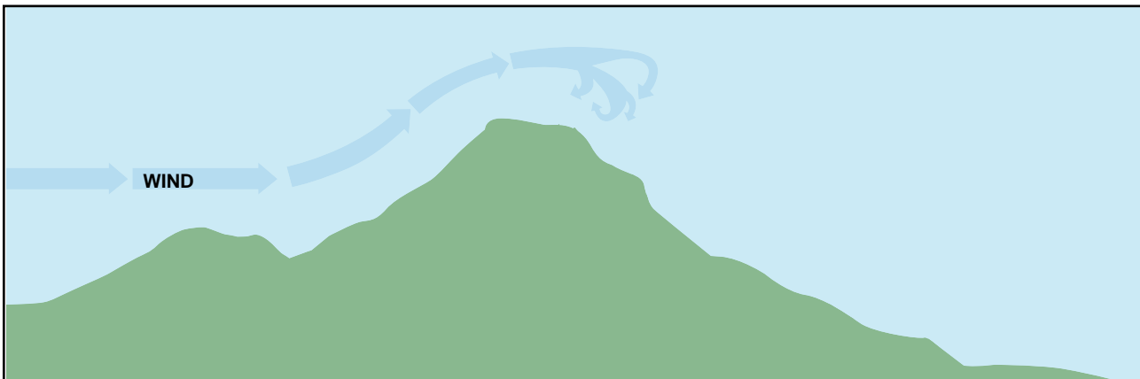
Figure 10-16. Turbulence encountered over and around mountainous regions.
