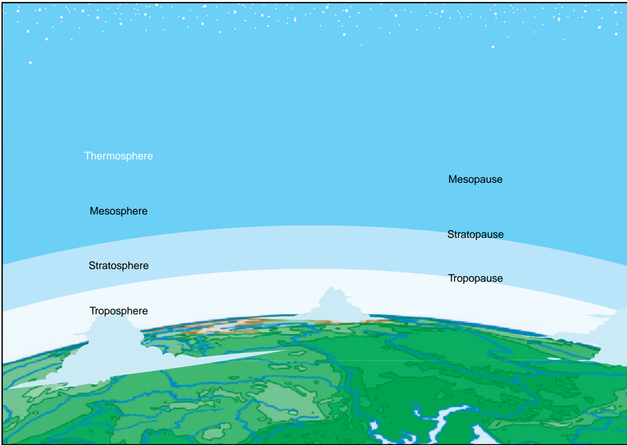
Figure 10-2. Layers of the atmosphere.
