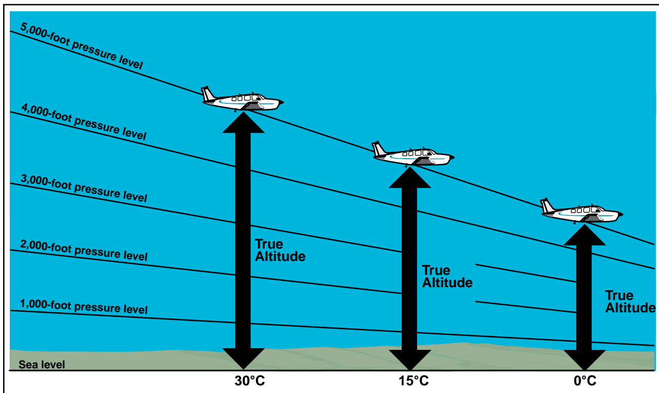
Figure 6-3. Effects of nonstandard temperature on an altimeter.
