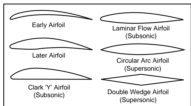
Figure 2-6. Airfoil designs.
