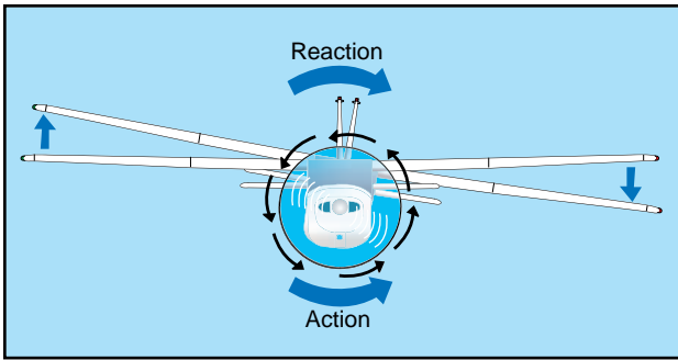
Figure 3-30. Torque reaction.
