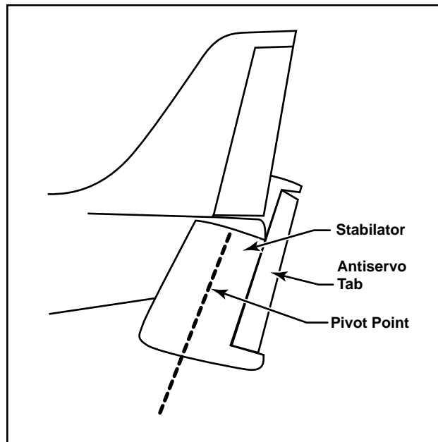
Figure 1-8. Stabilator components.
