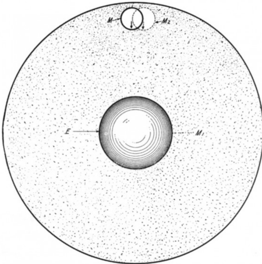
Fig. 2. — Tesla's Conception of the Rotation of the Moon, M , Around the Earth, E ; the Moon, In This Demonstration Hypothesis, Being Considered as Embedded In a Solid Mass, M_1 . If, As Commonly Believed, the Moon Rotates, This Would Be Equally True For a Portion of the Mass M_1 , and the Part Common to Both Bodies Would Turn Simultaneously In "Opposite" Directions.
