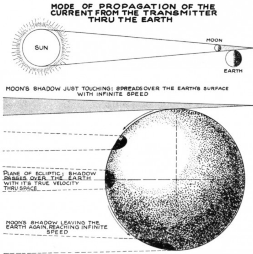
Fig. 8. — This Diagram Illustrates How, During a Solar Eclipse, the Moon's Shadow Passes Over the Earth With Changing Velocity, and Should Be Studied In Connection With Fig. 9. The Shadow Moves Downward With Infinite Velocity at First. Then With Its True Velocity Thru Space, and Finally With Infinite Velocity Again.
