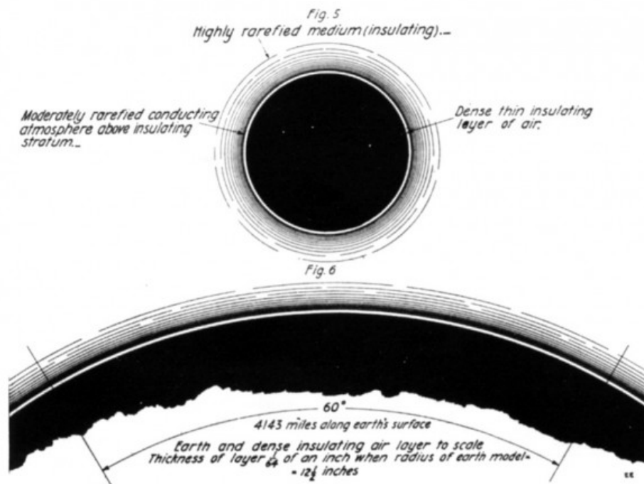
Figs. 5 & 6. — A Section of the Earth and Its Atmospheric Envelope Drawn to Scale. It is Obvious That the Hertzian Rays Cannot Traverse So Thin a Crack Between Two Conducting Surfaces For Any Considerable Distance. Without Being Absorbed, Says Dr. Tesla, in Discussing the Ether Space Wave Theory.
