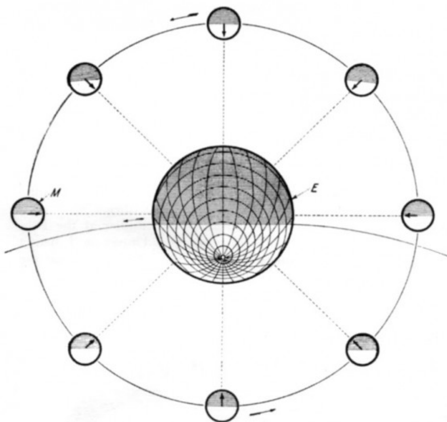
Fig. 1. — It Is Well Known That the Moon, M. , Always Turns the Same Face Toward the Earth, E. , as the Black Arrows Indicate. The Parallel Rays From the Sun Illuminate the Moon In Its Successive Orbital Positions as the Unshaded Semi-circles Indicate. Bearing This in Mind, Do You Believe That the Moon Rotates on Its Own Axis?
