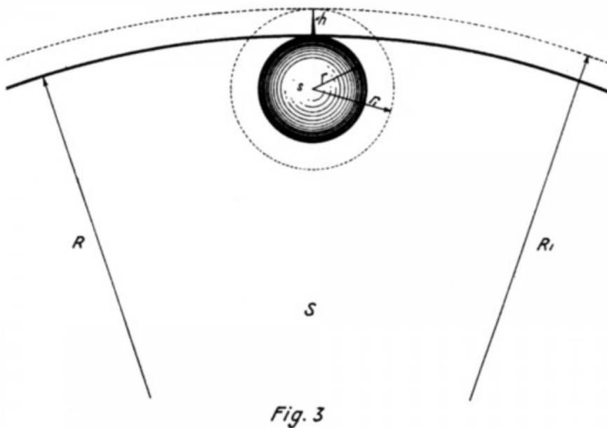
Fig. 3. — Diagram Used to Explain the Fallacy of the Franklin Pointed Lightning Rod, and an Analogy Whereby the Author Shows In a Clear Manner How the Charged Sphere May for Illustration be Considered as Heated to a High Degree, and the Heat Allowed to Escape at a Known Rate.
