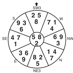
GEN house: Sitting NE3, Facing SW3: 232.5° - 247.5°
