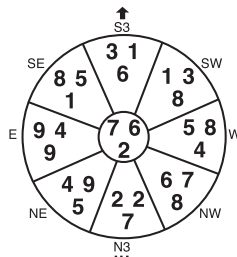
KAN house: Sitting N3, Facing S3: 187.5° - 202.5°
