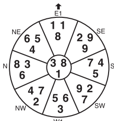
DUI house: Sitting W1, Facing E1: 67.5° - 82.5°
