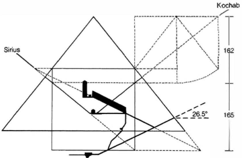
25. The astro-geometry of the shafts and chambers inside the Great Pyramid, with the upper culmination position of the stars taken C.2450BC
