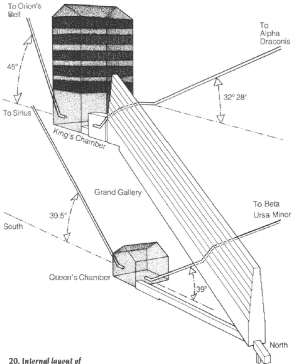
20. Internal layout of the upper chambers of the Great Pyramid and associated shafts Note kinks in the two northern shafts
