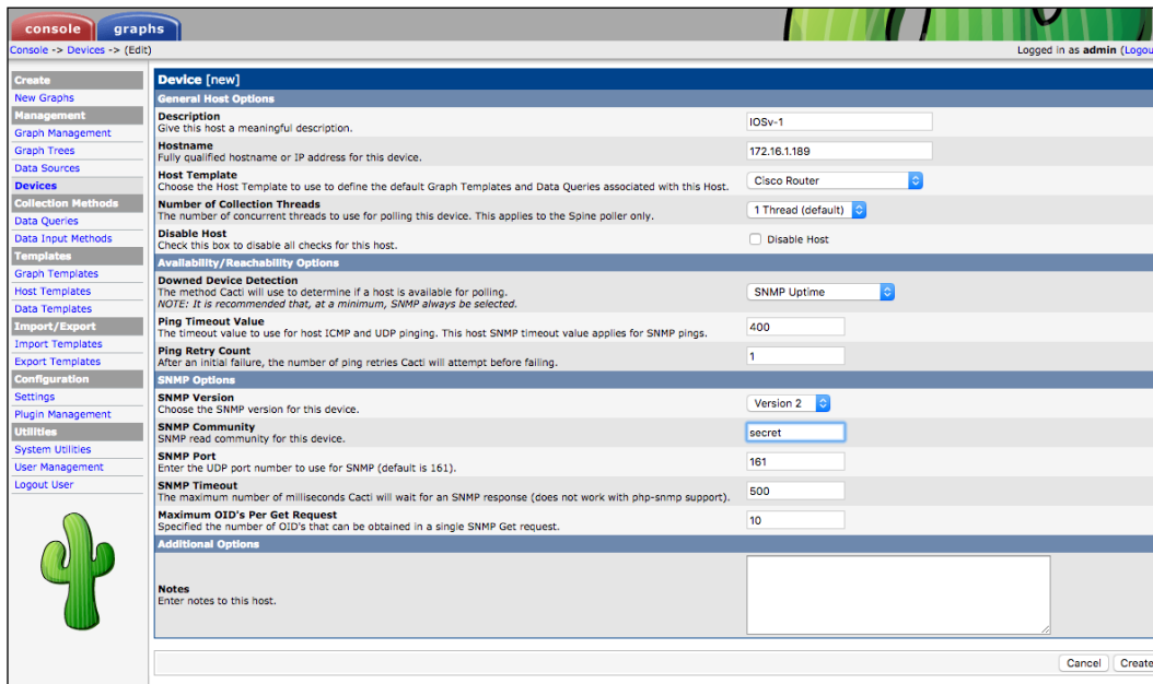
Figure 12: Cacti device edit page
