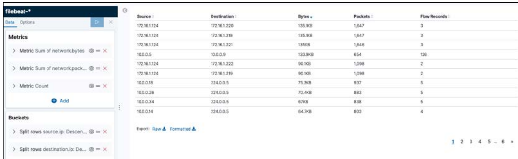
Figure 18: Kibana table
