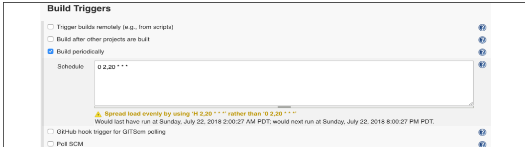
Figure 10: Build trigger
