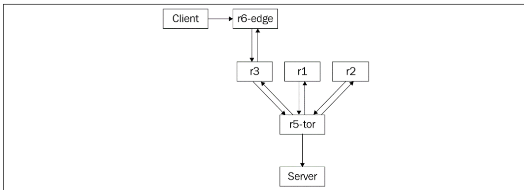
Figure 8: Topology graph 4
