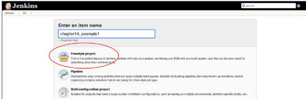
Figure 5: Jenkins item
