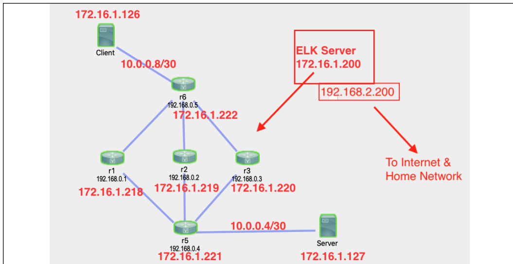
Figure 2: Lab topology
