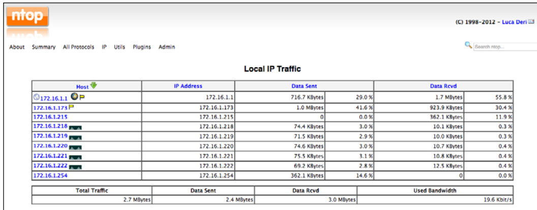
Figure 10: Ntop Local IP Traffic
