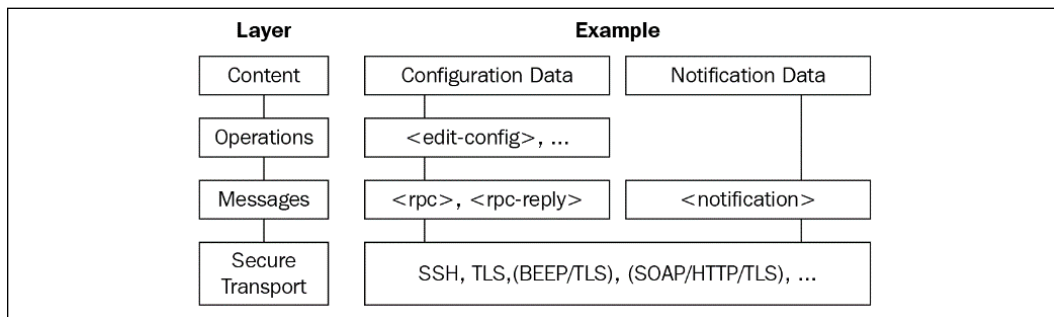
Figure 5: NETCONF model
