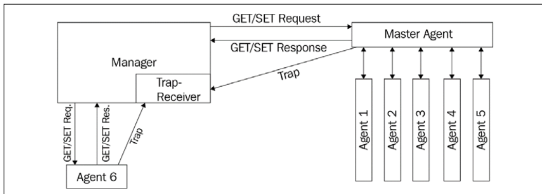
Figure 2: SNMP operations
