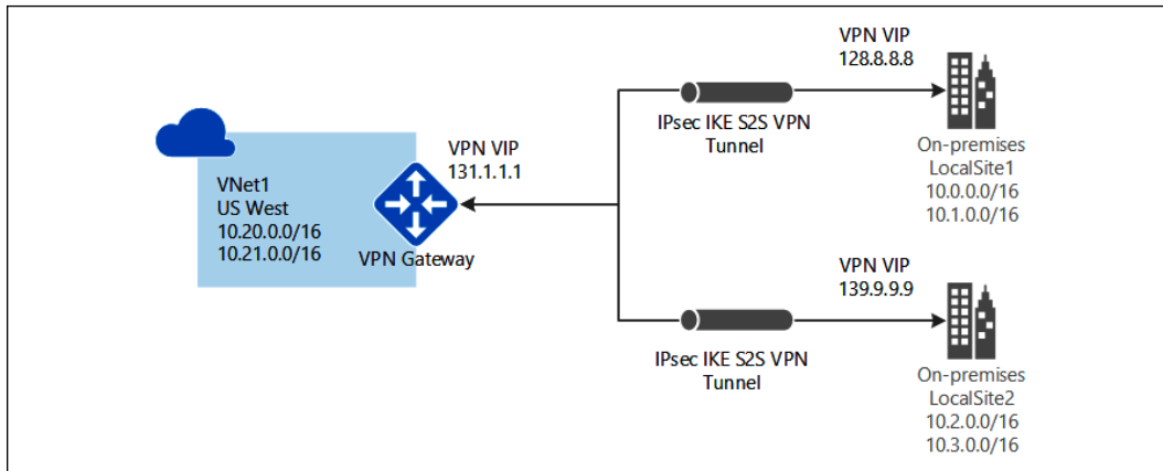
Figure 30: Azure client VPN gateway (source: https://docs.microsoft.com/en-us/azure/vpn-gateway/vpn-gateway-about-vpngateways )
