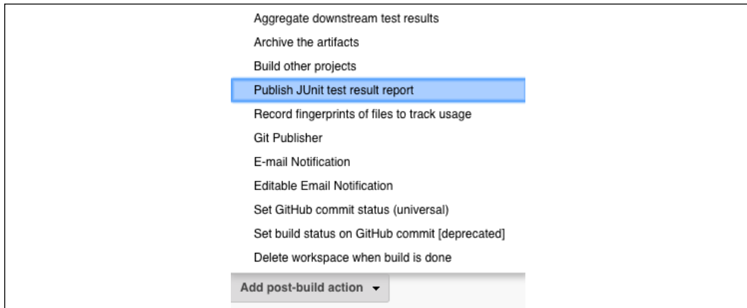
Figure 7: Post-build step
