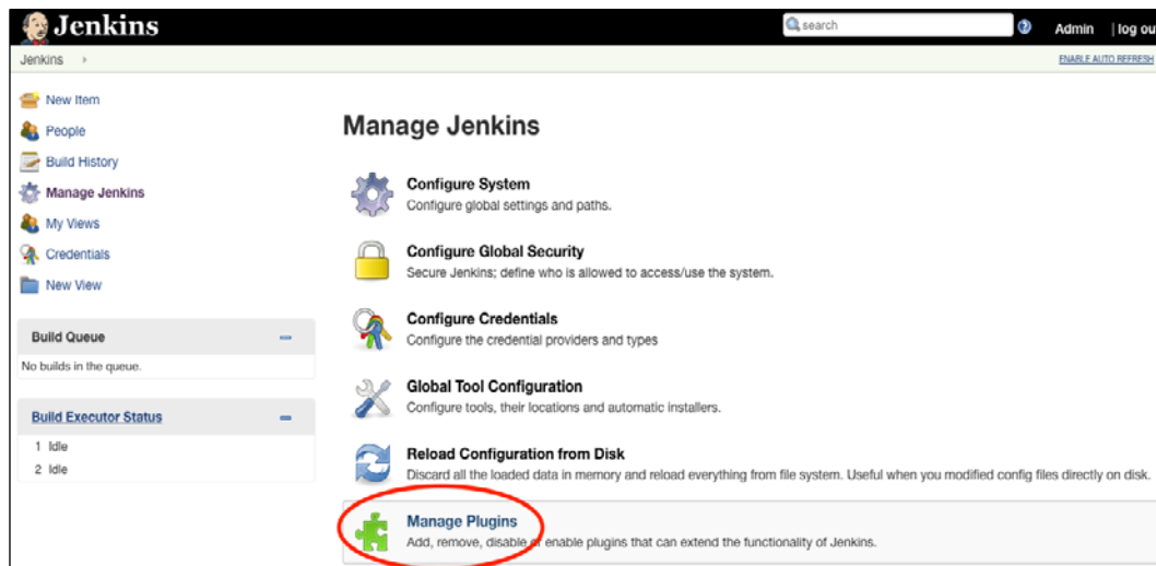
Figure 14: Jenkins plugin
