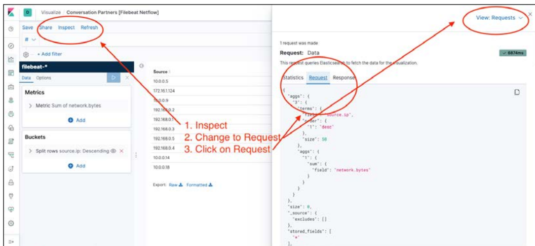
Figure 20: Kibana request
