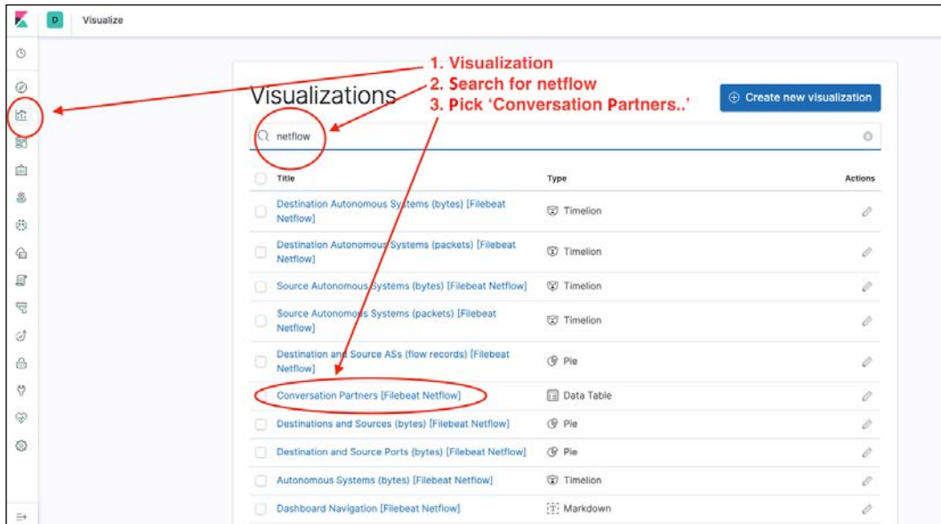
Figure 17: Kibana Visualization
