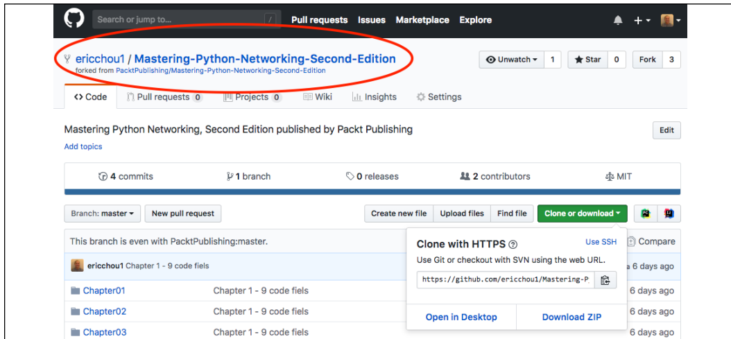
Figure 7: Git Fork
