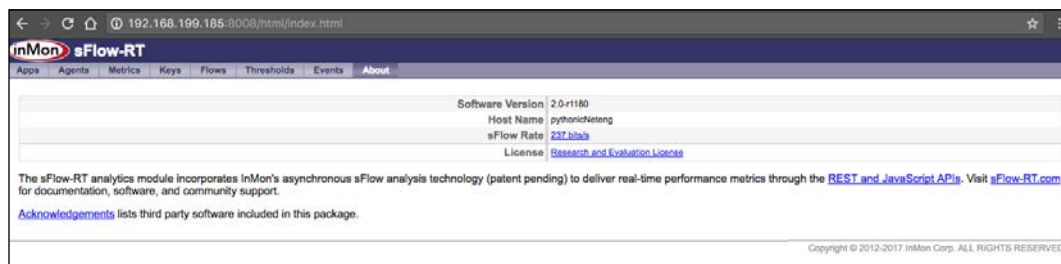
Figure 17: sFlow-RT version
