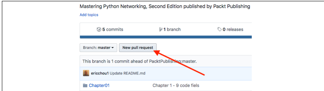
Figure 8: Pull request
