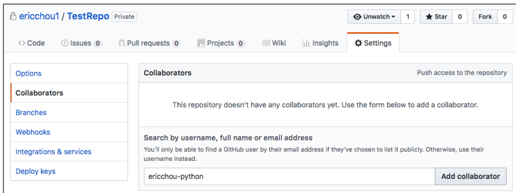
Figure 4: Repository invite
