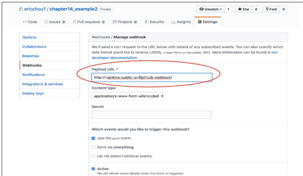
Figure 26: GitHub webhooks
