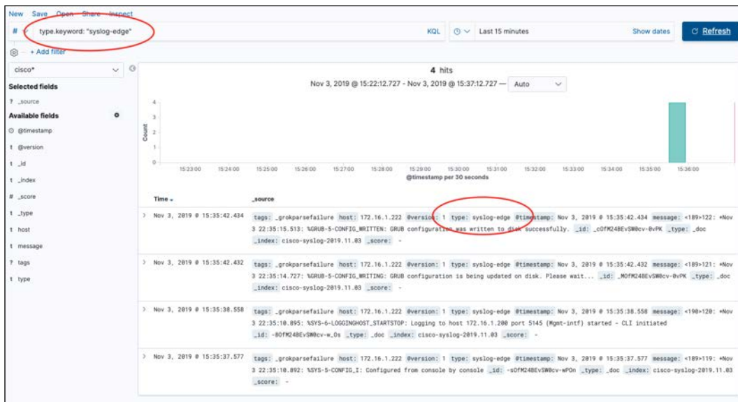
Figure 11: Syslog Index
