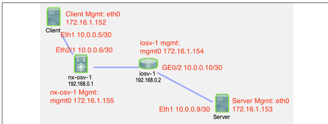
Figure 1: Lab topology
