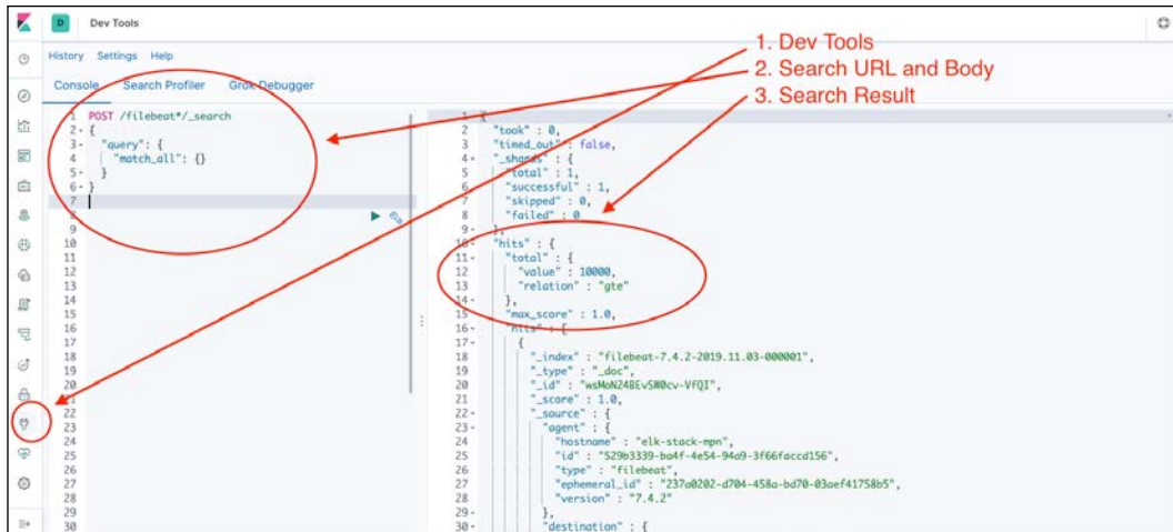
Figure 19: Kibana Dev Tools
