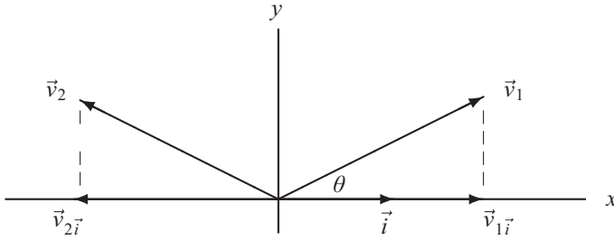
Figure 6.3 Two vectors and their projections onto \vec{i} .
