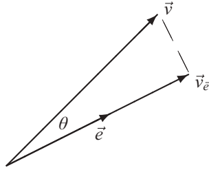
Figure 6.4 Projection onto \vec{e} .
