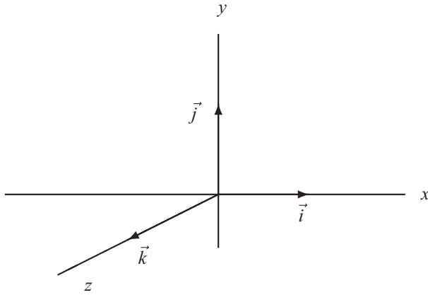
Figure 6.1 Unit vectors along x , y and z axes.
