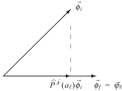
Figure 30.1 Measurement resulting in a change of \vec{\phi}_i to \vec{\phi}_f = \vec{\varphi}_\ell .
