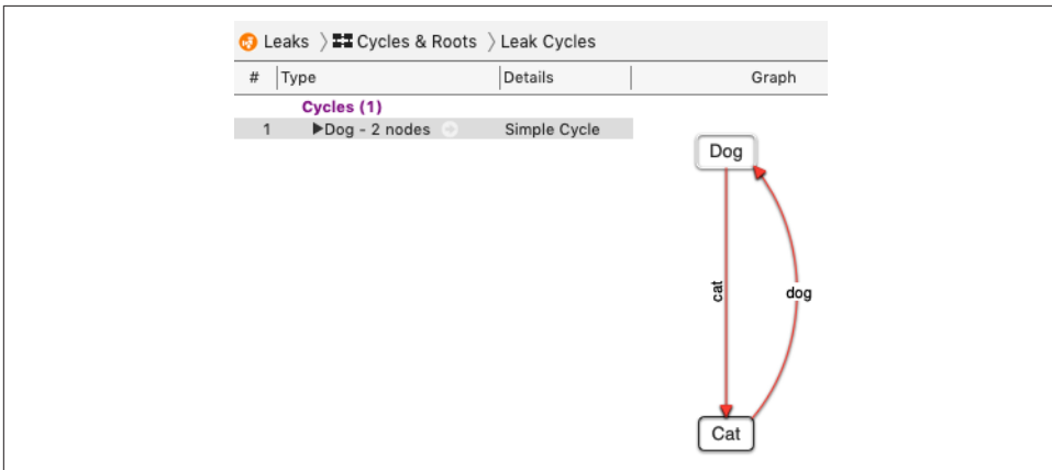
Figure 9-26. Instruments describes a retain cycle
