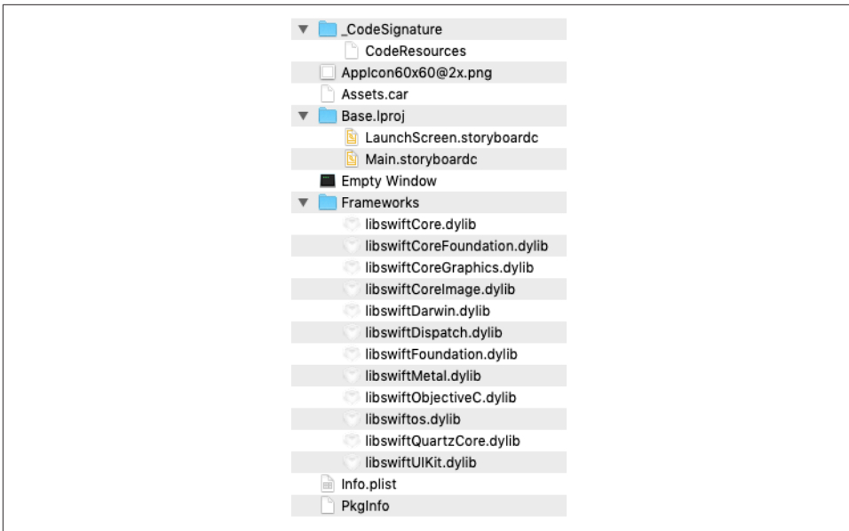
Figure 6-15. Contents of the app package, old style
