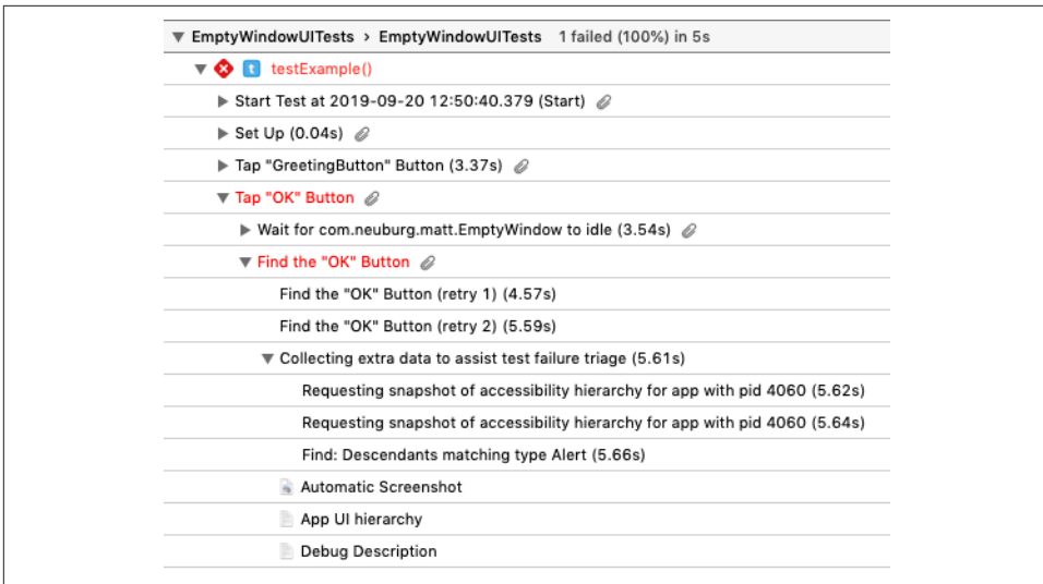
Figure 9-13. The Report navigator displays a failed UI test
