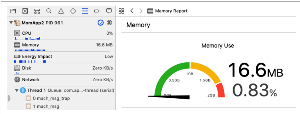
Figure 9-22. The Debug gauges
