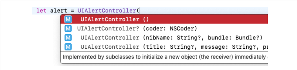
Figure 9-5. The autocomplete menu
