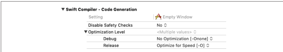
Figure 6-11. How configurations affect build settings
