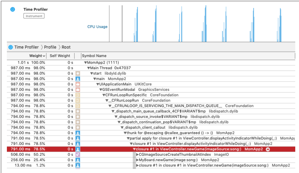
Figure 9-27. Drilling down into the time profile
