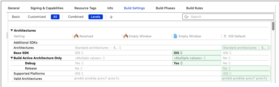
Figure 6-9. Target build settings
