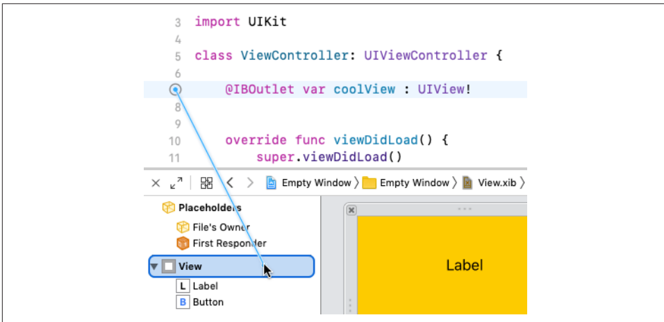
Figure 7-12. Connecting an outlet by dragging from code to nib editor
