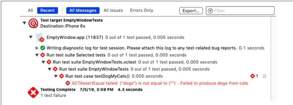
Figure 9-11. The Report navigator describes a test failure
