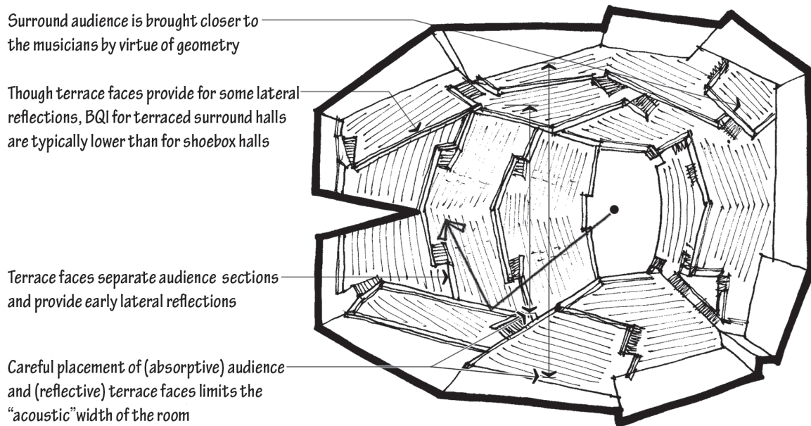
Terraced surround hall
