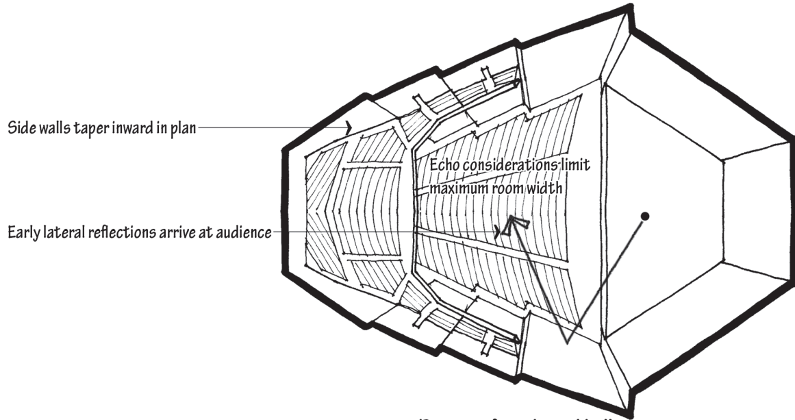
Reverse-fan-shaped hall
