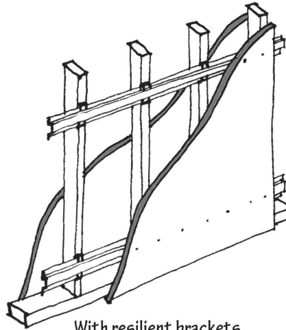
With resilient brackets
