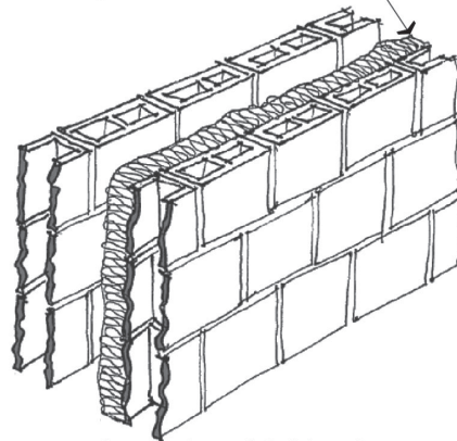
Two wythes of CMU with cavity
