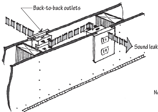
Stud wall with outlets in the same cavity
