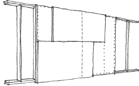
Multilayer gypsum board with staggered panel joints
