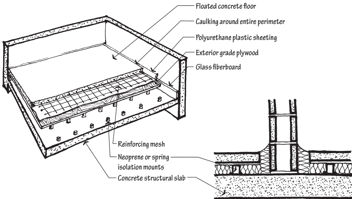
"Floated" floor
