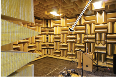
Anechoic Chamber
