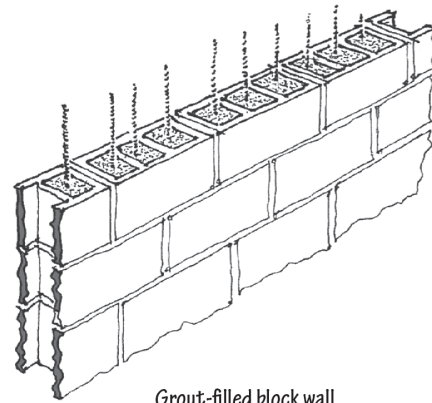
Grout-filled block wall
