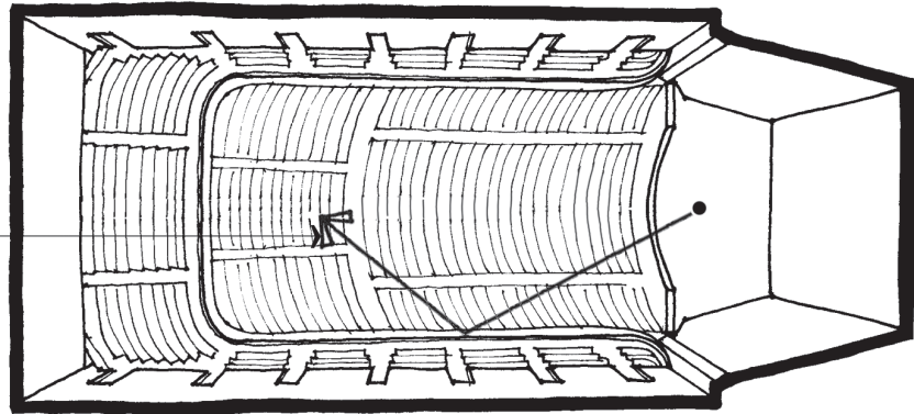
Shoebox hall
