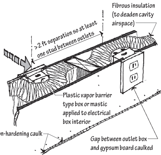
Stud wall with outlets in separate cavities
