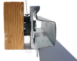
Resilient clip
