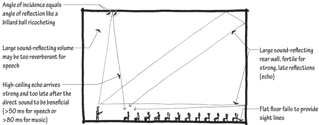
Room not shaped for sound
