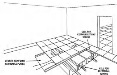
cellular floor
