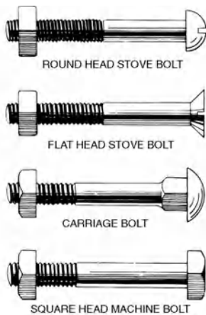
bolts, 1
