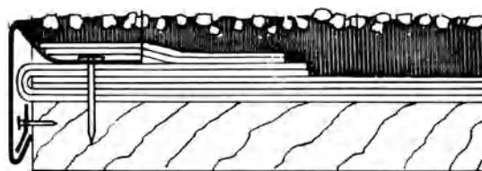
gravel stop
