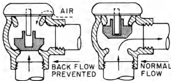
vacuum breaker
