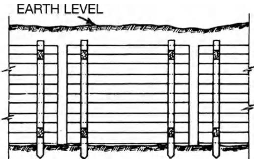
horizontal sheeting
