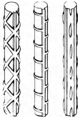
deformed bars
