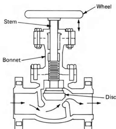
globe valve
