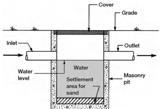
sand interceptor
