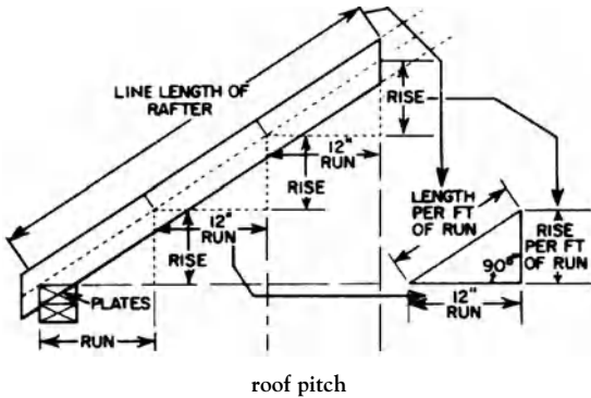
roof pitch
