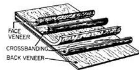
back veneer
