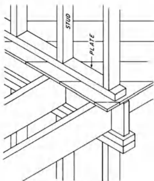
plate, 2
