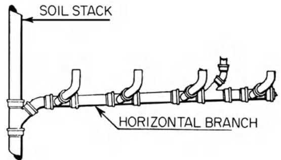
horizontal branch
