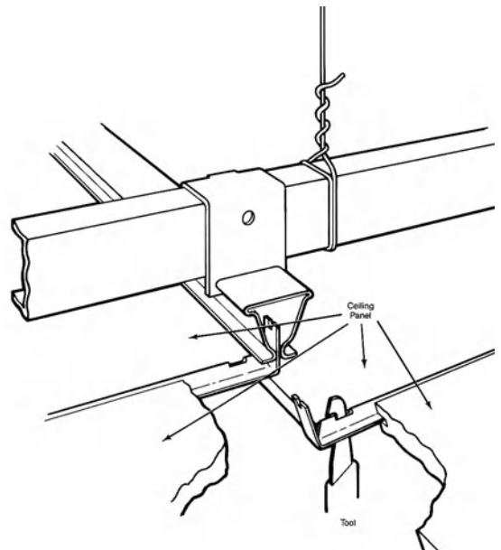
suspended ceiling
