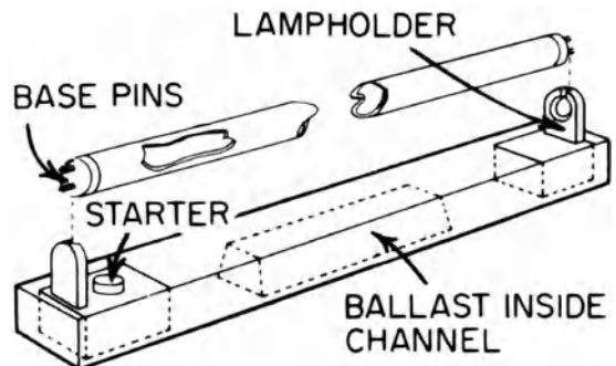
fluorescent lamp
