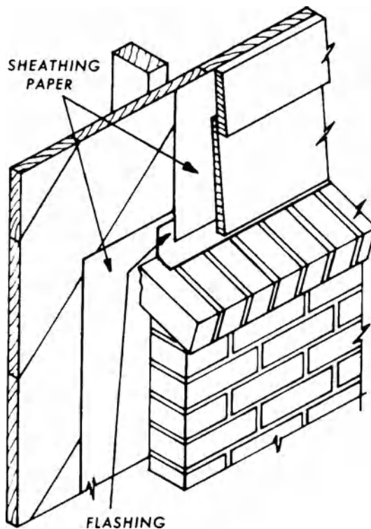
brick veneer
