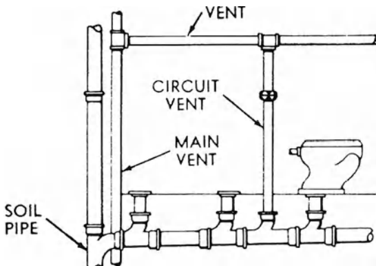
circuit vent
