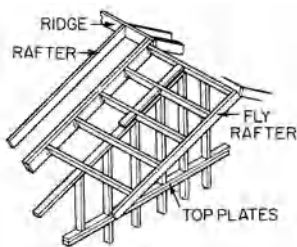
fly rafter
