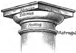
capital: nomenclature
