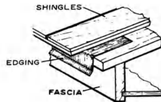
edging, 2
