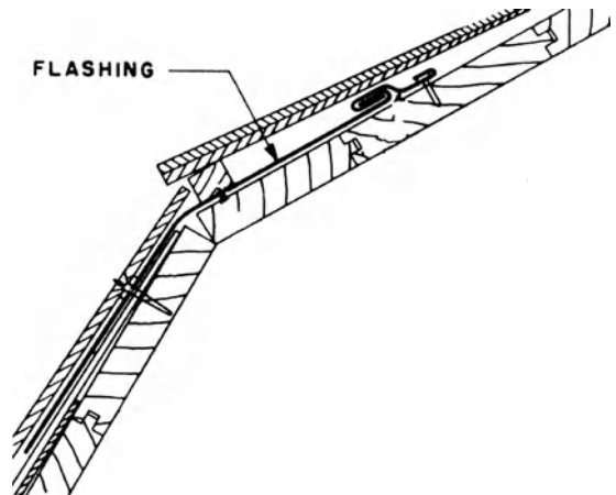
concealed flashing
