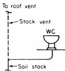
stack vent, 1
