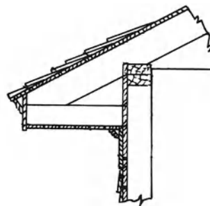
box cornice
