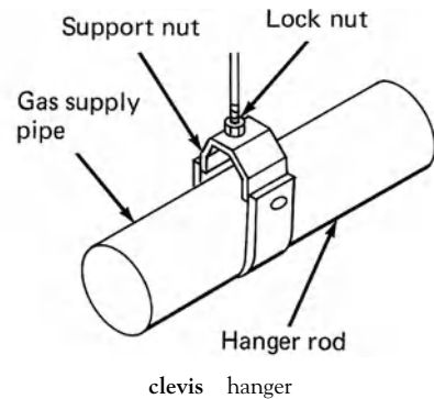
clevis hanger
