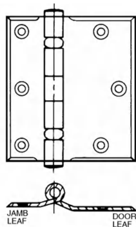
full-surface hinge
