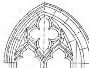
sconcheon arch
