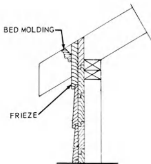
bed molding, 3
