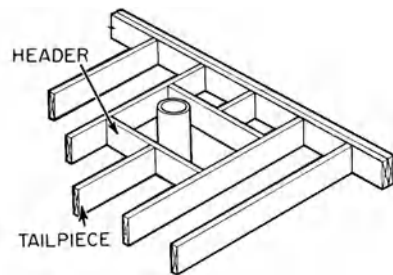
tailpiece, 1
