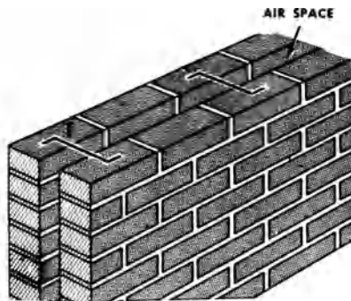
cavity wall
