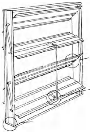
opposed-blade damper
