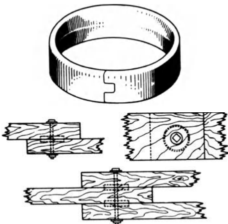
split-ring connector showing a typical joint
