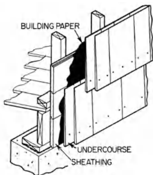
undercourse
