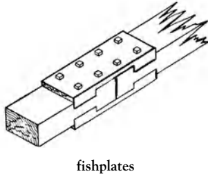
fishplates
