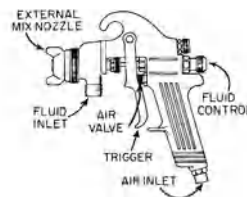
spray gun
