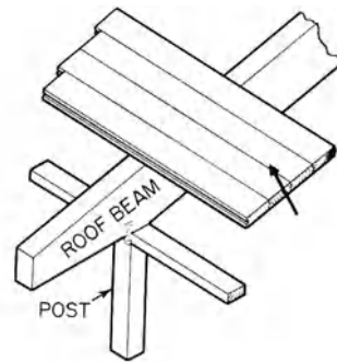
decking, 1
