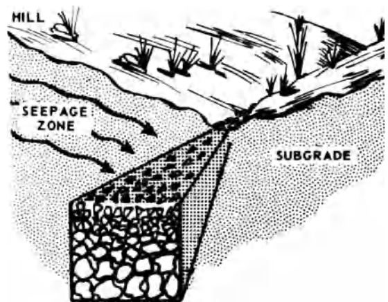
French drain
