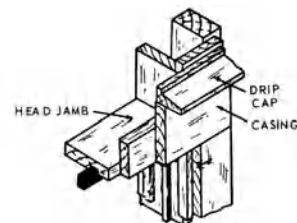
drip cap
