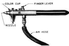
airbrush
