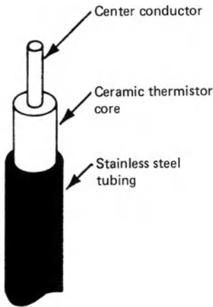
linear-type heat detector
