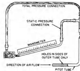
pitot tube
