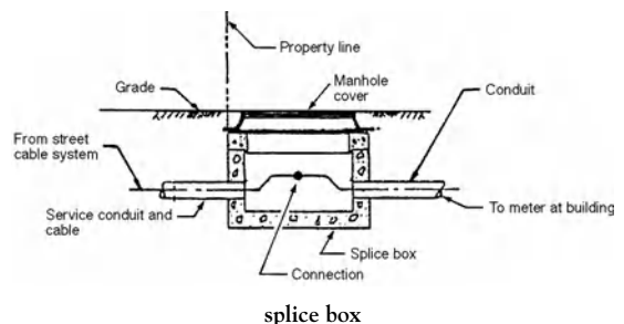
splice box
