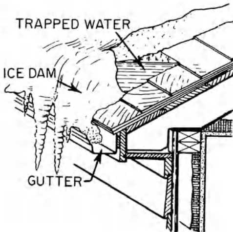
ice dam
