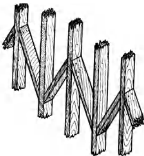
diagonal bridging, 2
