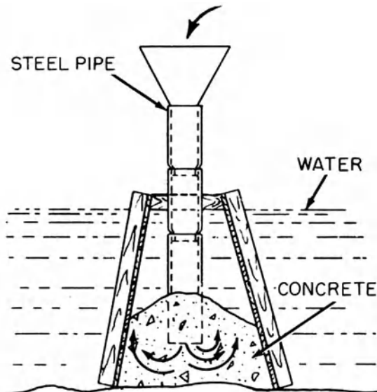
tremie used in placing concrete under water
