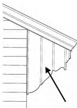
endboard at cornice
