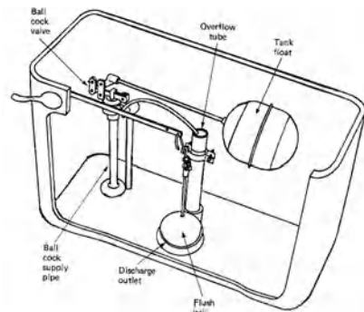
flush tank
