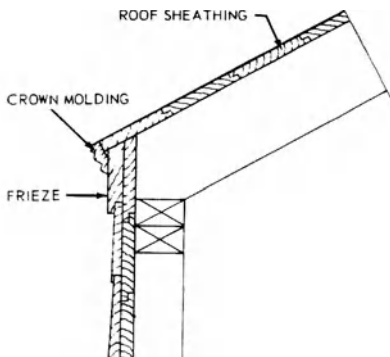
crown molding
