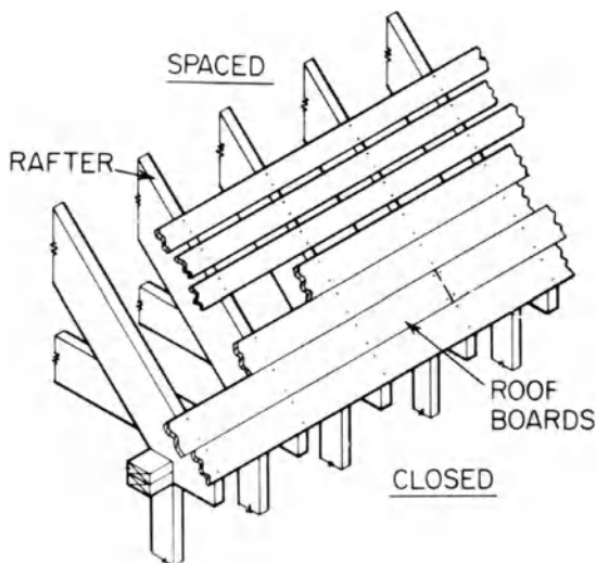
board sheathing
