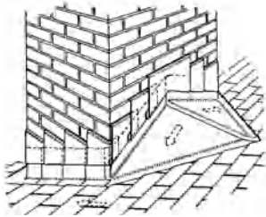
cricket
