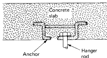
anchor, 9
