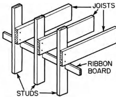
ribbon board, 1
