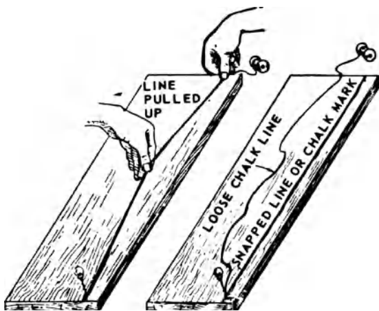
chalk line
