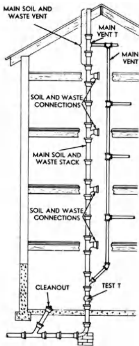
stack, 1: installation
