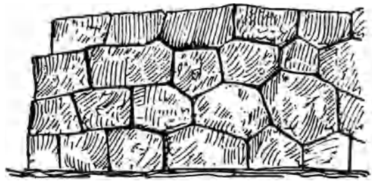
polygonal masonry
