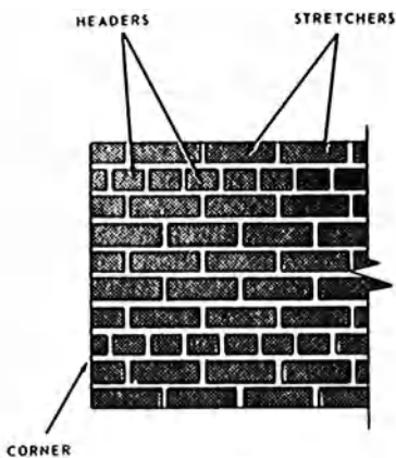
common bond
