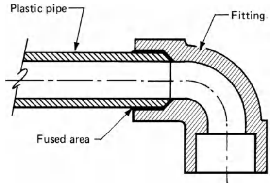
heat-fusion joint
