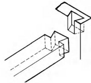
dovetail, 2
