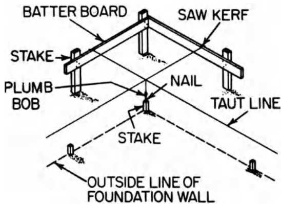
staking out
