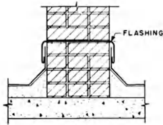
through-wall flashing
