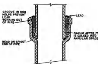
caulked joint
