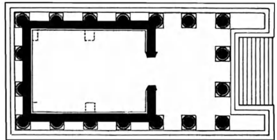
pseudoperipteral
