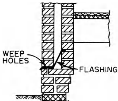
cavity flashing
