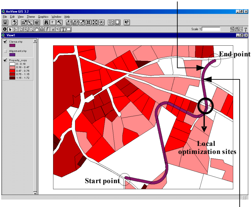
Figure 14.9: A particular alternative initiating local optimization using a real GIS map, Baltimore County, Maryland.
