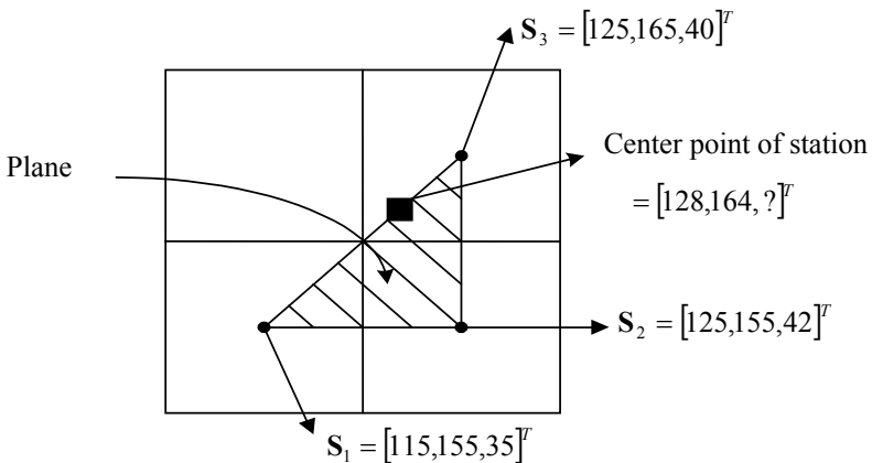
Figure 12.8: Surrounding vectors of station B’s center point.
