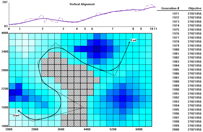
Figure 15.5: Best solution found not incorporating bridges and tunnels for an artificial study area.
