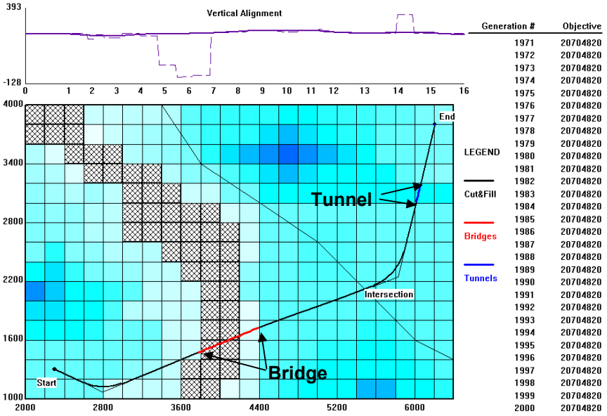
Figure 15.51: The third best solution (scenario 11).
