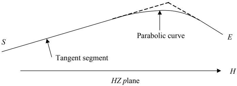
Figure 3.4: A typical vertical alignment on the HZ Plane.
