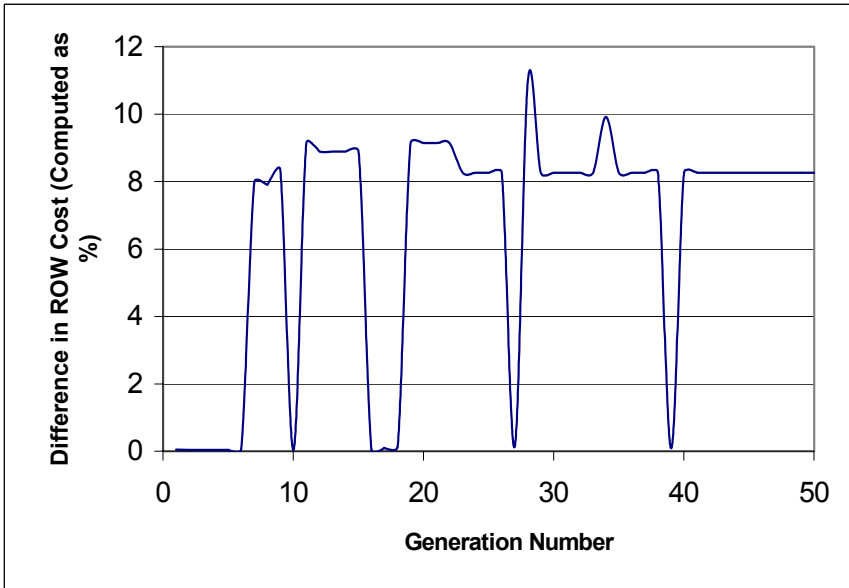
Figure 10.21: Effects of compactness analysis.
