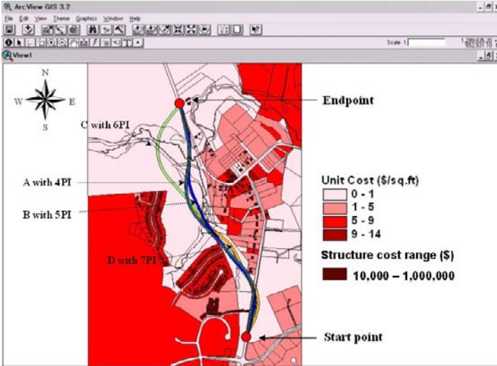
Figure 10.36: Optimized horizontal alignments for different PI's.
