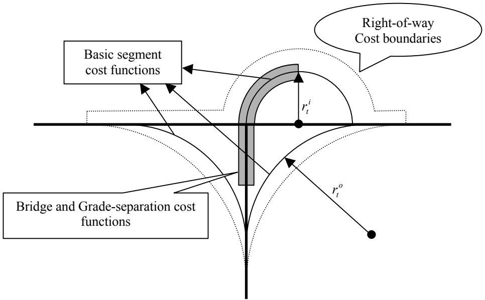
Figure 12.31: Centerlines of a typical trumpet interchange, major design criteria and separated parts for each cost function.
