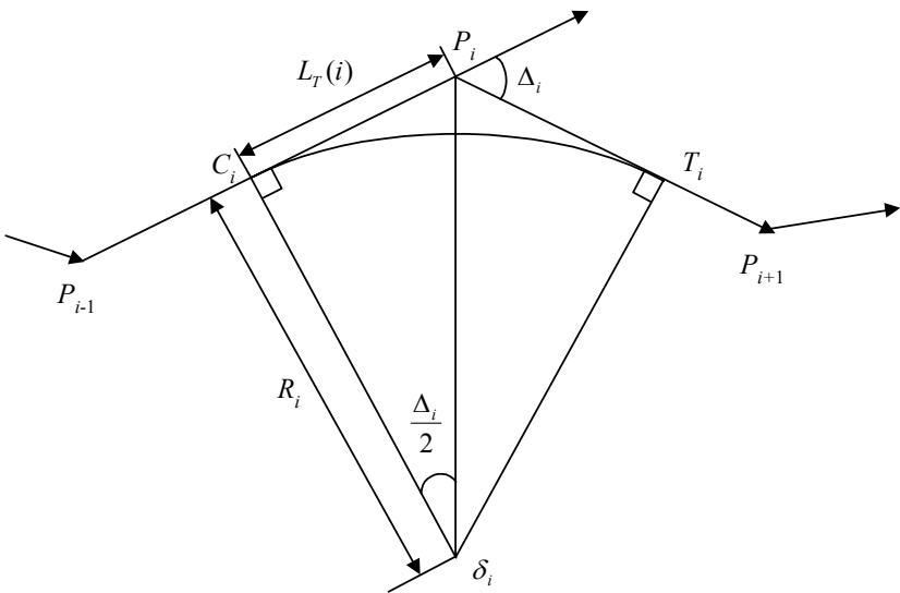
Figure 4.7: The geometric specification of a circular curve.
