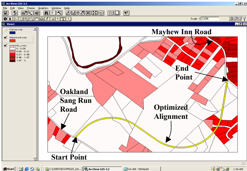
Figure 15.4: Best solution with the planar interpolation using a real GIS map.
