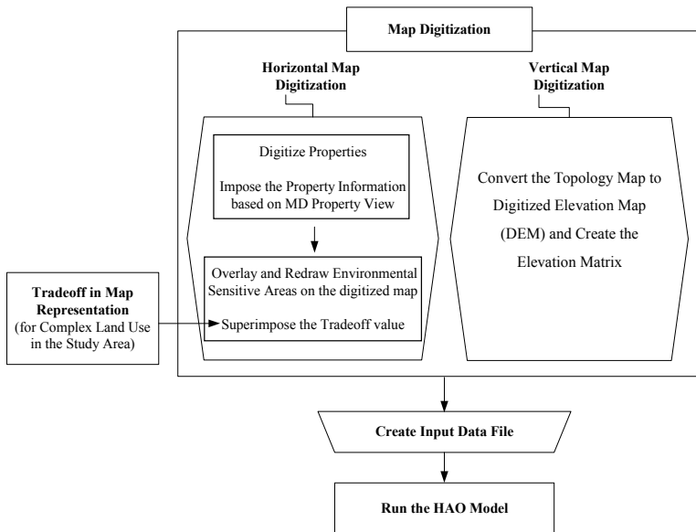
Figure 10.30: Procedure for the HAO model application.
