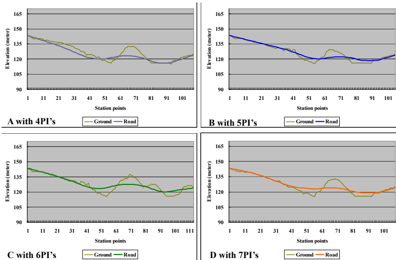
Figure 10.37: Optimized vertical alignments for different PI's.
