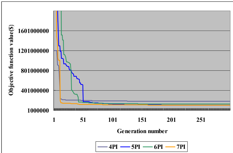
Figure 10.38: Changes in objective function value over successive generations.
