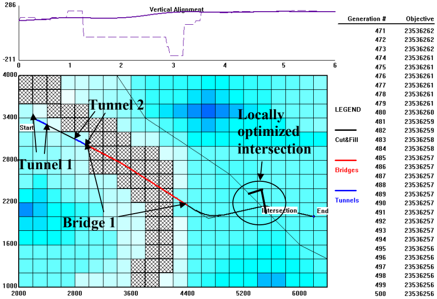
Figure 15.32: The optimized solution involving local intersection optimization with moved start and end points.
