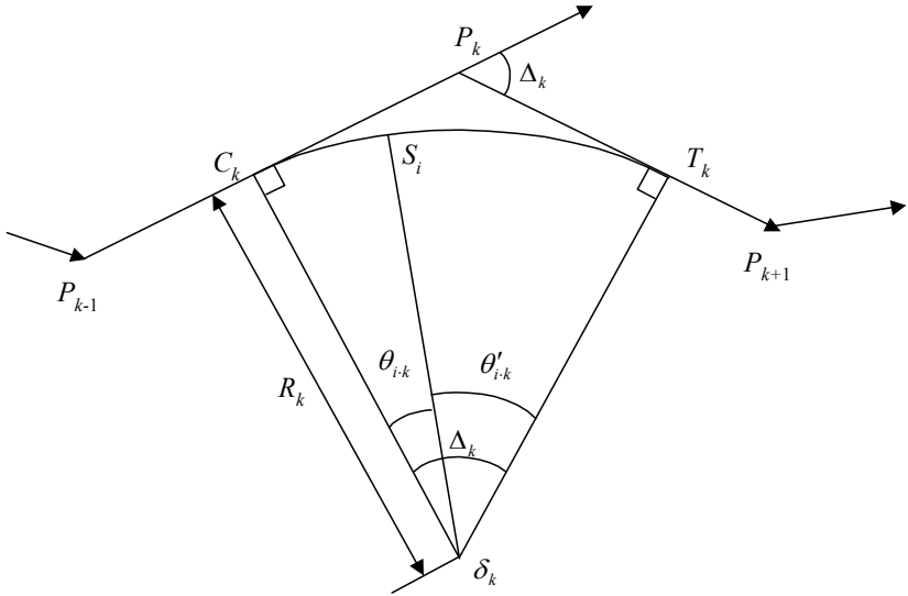
Figure 7.7: Station point on a circular curve of the horizontal alignment.
