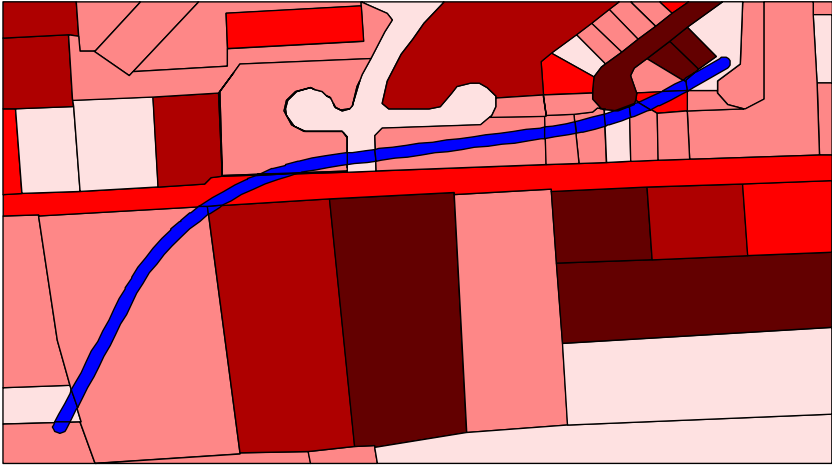
Figure 10.17: Optimized alignment at the 500 th generation for the Baltimore county case.
