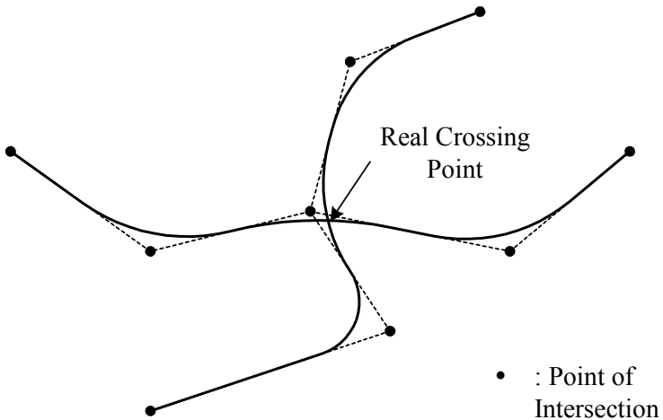
Figure 12.9: Points of intersections (PI's) and final crossing point deviating from its original PI.
