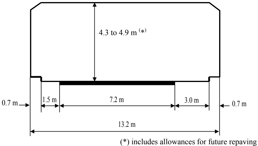
Figure 11.5: AASHTO typical desirable cross section and clearances for a two-lane tunnel.
