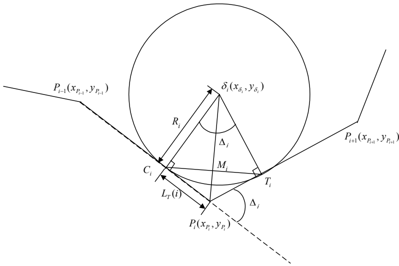
Figure 4.13: The geometric relations among C_i , T_i , \delta_i , and M_i .
