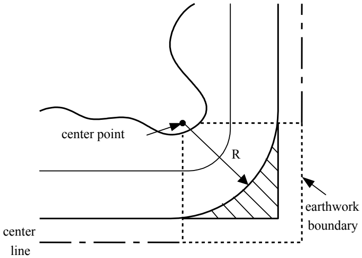
Figure 12.15: A simplified quadrant of a typical fill intersection.
