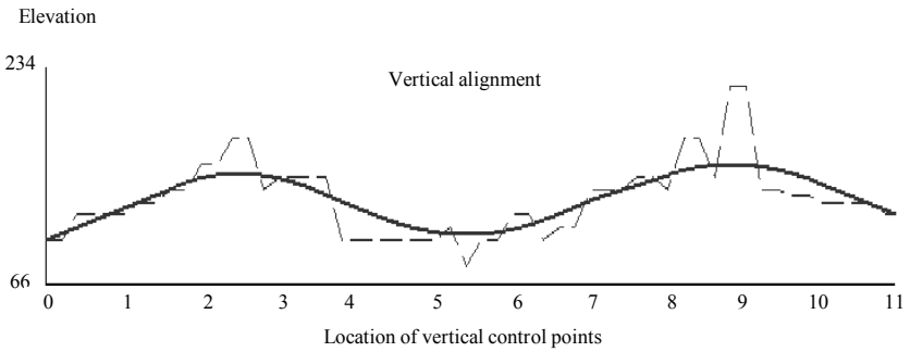
Figure 9.17: The vertical alignment of the fourth best solution for test example 1.
