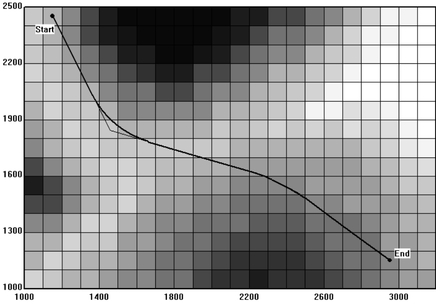
Figure 9.24: The optimized horizontal alignment found by Model 3 for test example 2.
