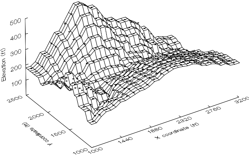
Figure 9.22: 3D View of test example 2.
