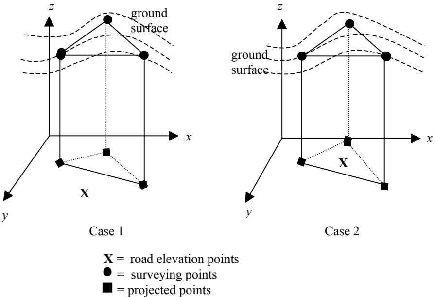
Figure 12.5: Two possible cases when projecting ground elevations onto xy plane.
