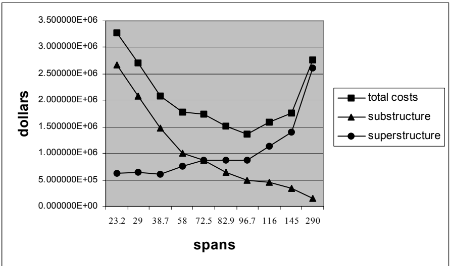
Figure 15.30: Optimized span and cost breakdown for bridge 2, considering a high water constraint and integer numbers of piers.
