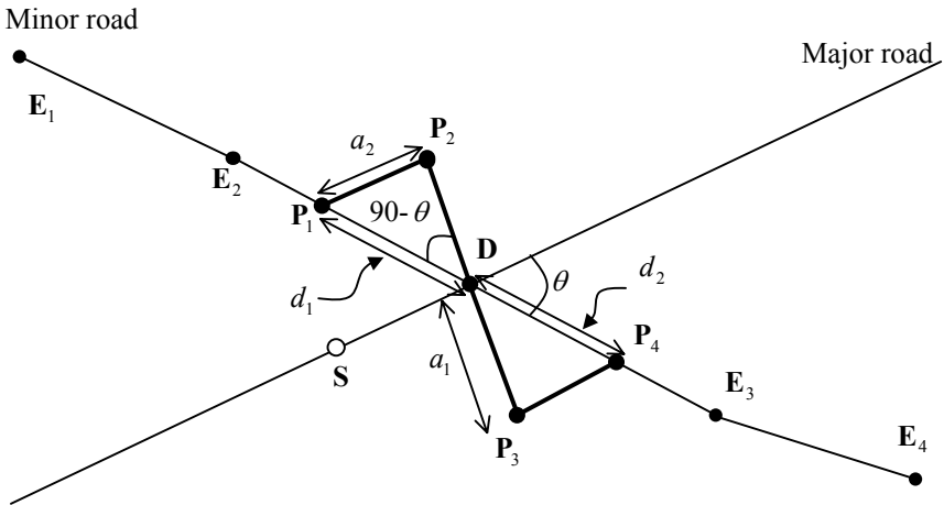
Figure 14.5: Alternative with minimum leg length.
