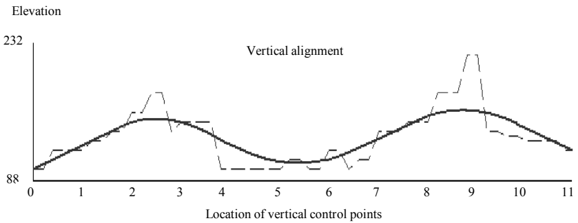
Figure 9.15: The vertical alignment of the third best solution for test example 1.
