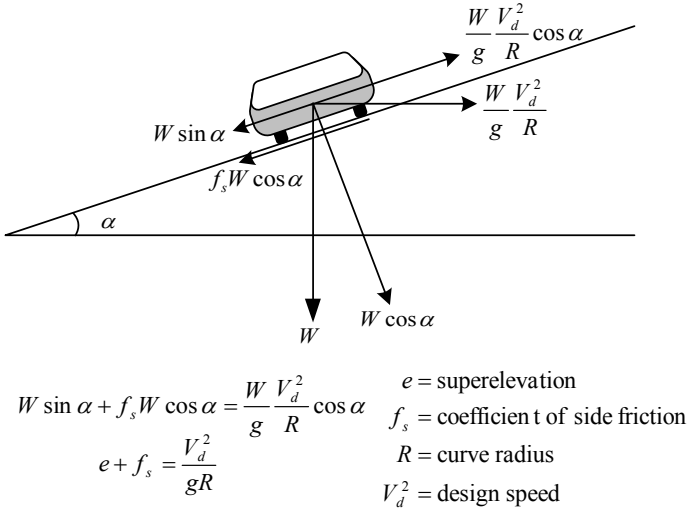
Figure 2.2: The physical relations among design speed, superelevation, coefficient of side friction, and curve radius.
