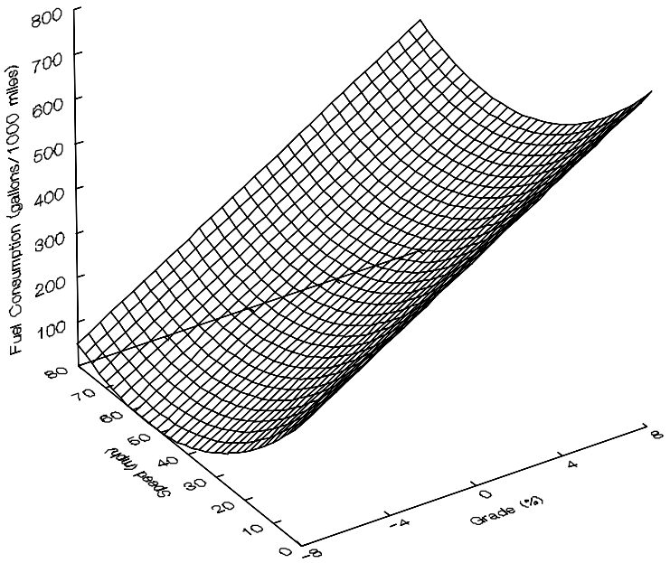
Figure 4.21: Regression function of fuel consumption: 3-S2 diesel truck.
