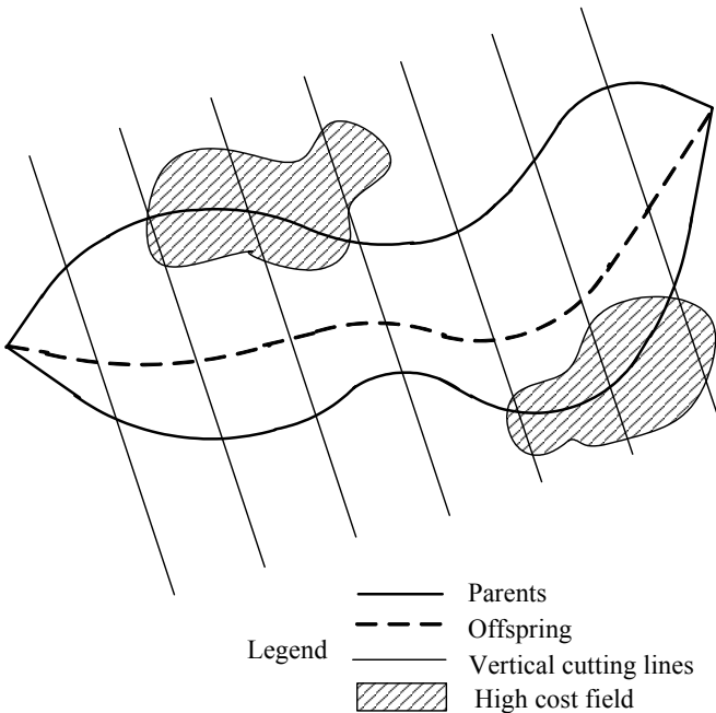
Figure 5.7: An example of an arithmetic crossover operator.
