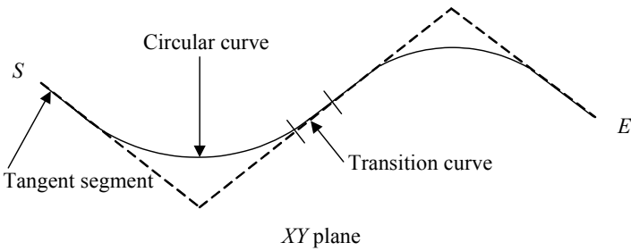
Figure 3.2: A typical horizontal alignment on the XY plane.
