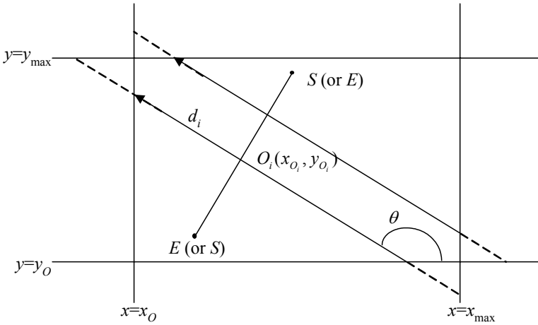
Figure 4.6: d_{iU} and d_{iL} when 90^\circ < \theta < 180^\circ .
