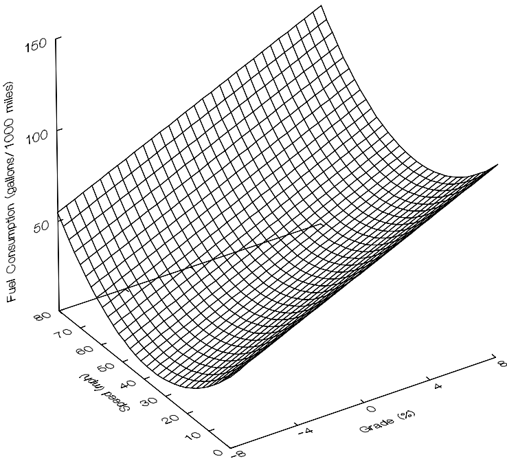
Figure 4.17: Regression function of fuel consumption: medium car.
