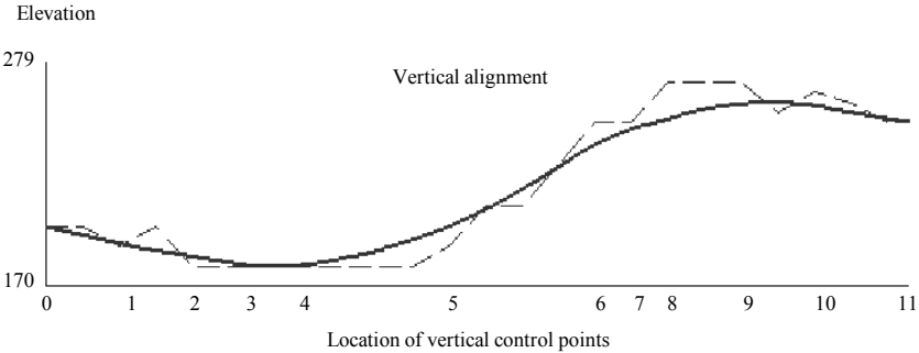
Figure 9.27: The optimized vertical alignment found by Model 4 for test example 2.
