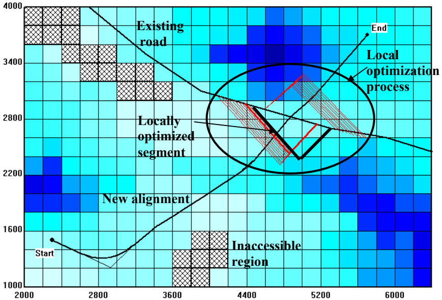
Figure 14.7: Artificial study area after 30 generations.
