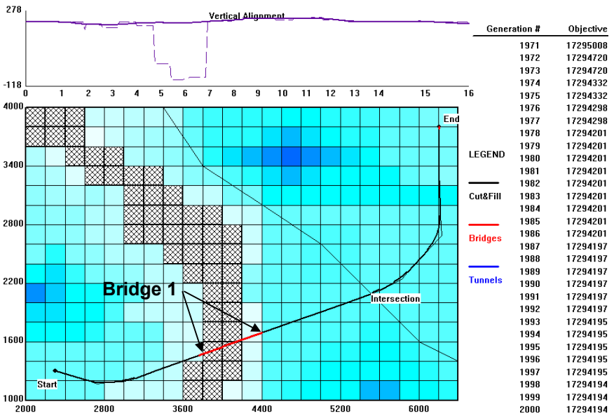
Figure 15.41: The best solution among three replications for scenario 2.
