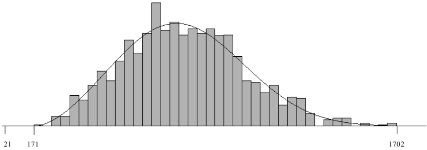
Figure 9.37: The fitted Weibull distribution of the objective value of Model 4 for test example 3.
