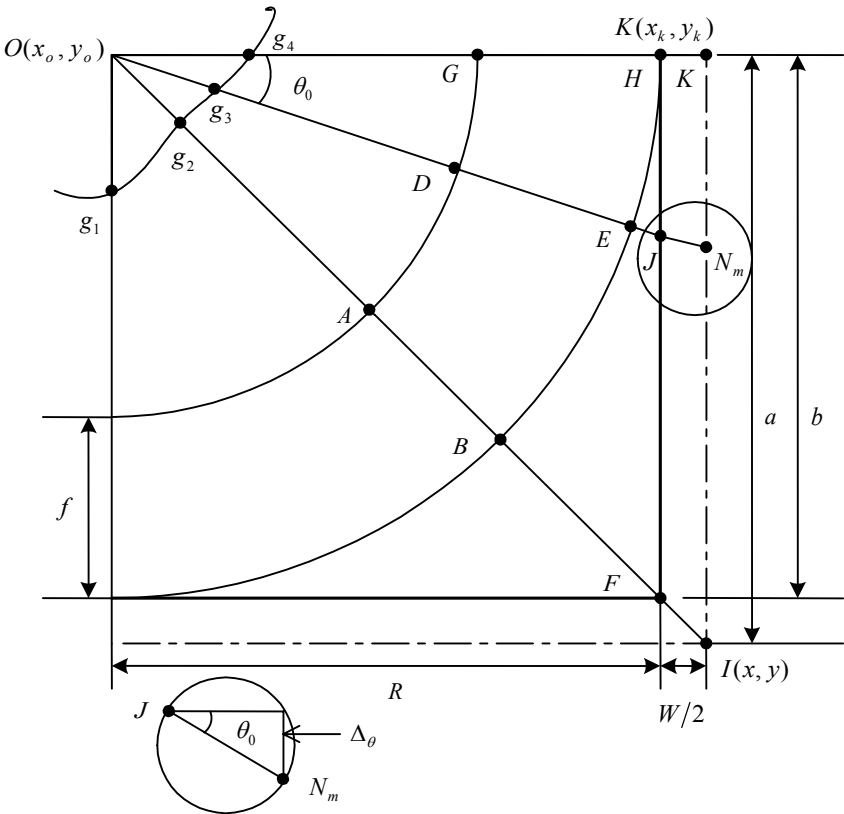
Figure 12.16: Important points for determining coordinates.
