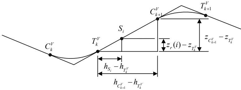
Figure 7.11: Station point on a tangent section of the vertical alignment.
