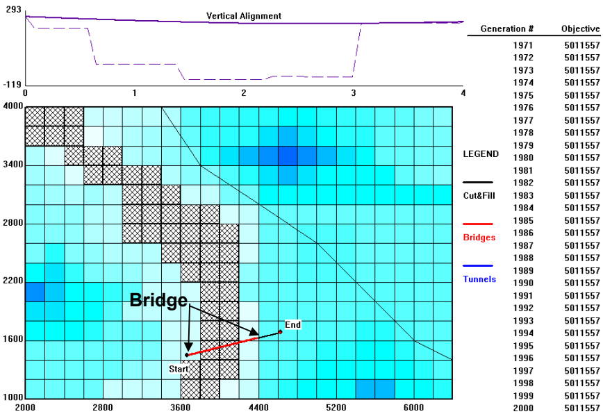
Figure 15.44: Optimized solution for segment 2 under scenario 3.
