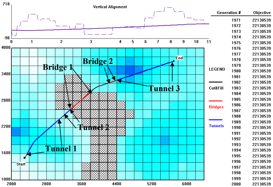
Figure 15.9: New best solution for the artificial study area.
