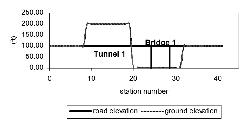
Figure 15.13: Zoomed-in profile of tunnel 1 and bridge 1 for Garrett County example.
