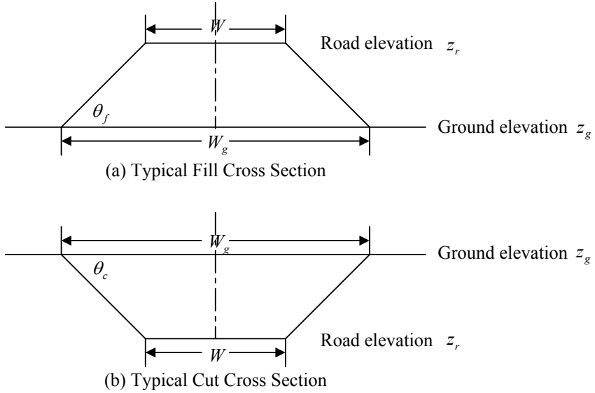
Figure 7.6: Typical fill and cut cross sections.
