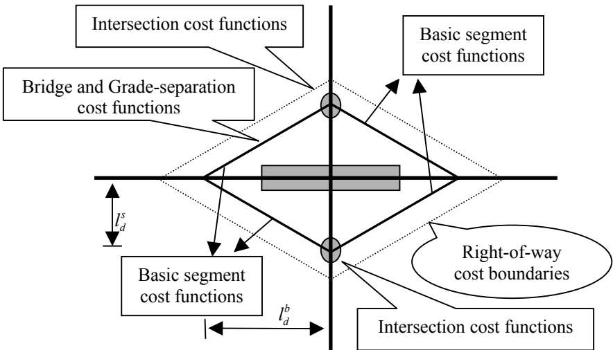
Figure 12.29: Centerlines of a typical diamond interchange, major design criteria and separated parts for each cost function.
