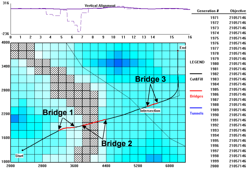
Figure 15.50: The second best solution (scenario 9).
