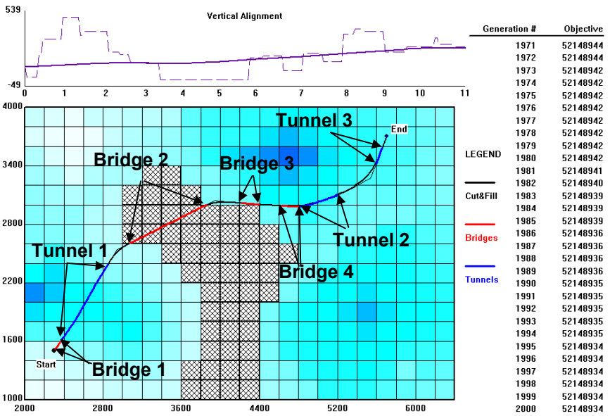
Figure 15.18: Optimized solution (scenario 3) for sensitivity analysis of tunnels.
