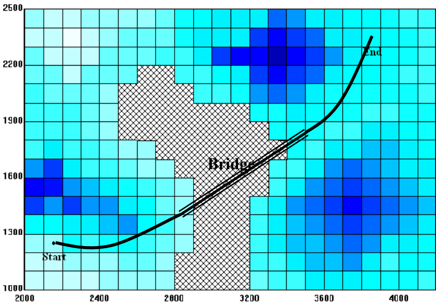
Figure 11.2: Possible solution incorporating bridges into optimization.
