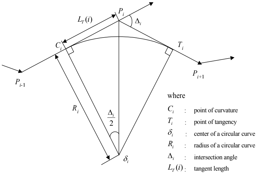
Figure 12.10: Geometric specification of a circular curve.
