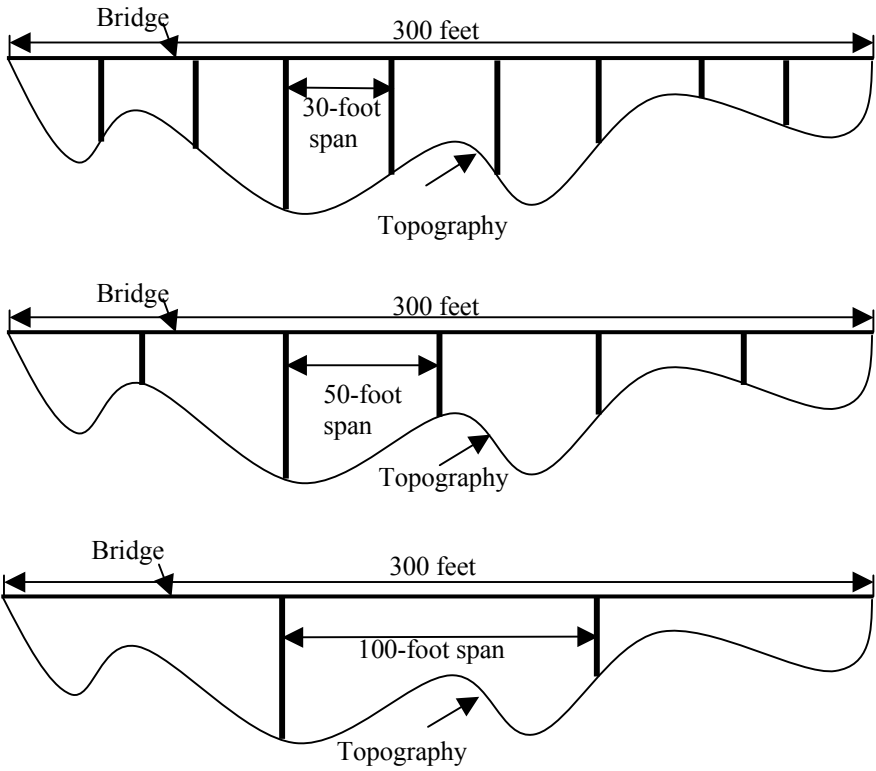
Figure 12.24: Equally spaced piers with varying spans.
