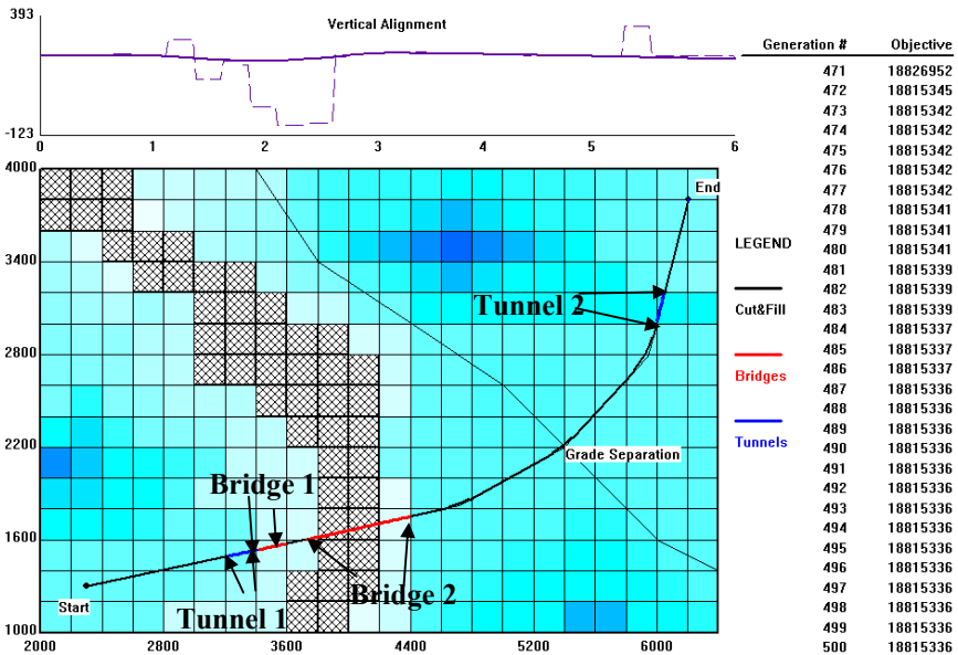
Figure 15.22: Solution for scenario 1.
