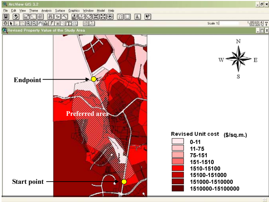
Figure 10.35: Preferred search space for the Brookeville bypass.
