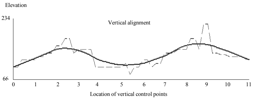
Figure 9.13: The vertical alignment of the second best solution for test example 1.
