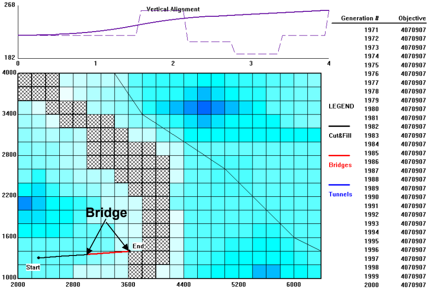
Figure 15.43: Optimized solution for segment 1 under scenario 3.
