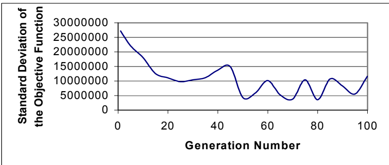
Figure 10.25: Standard deviation of objective function over successive generations.
