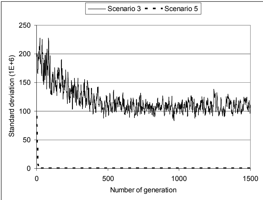
Figure 9.9: Standard deviation of program outputs for scenarios 3 and 5.
