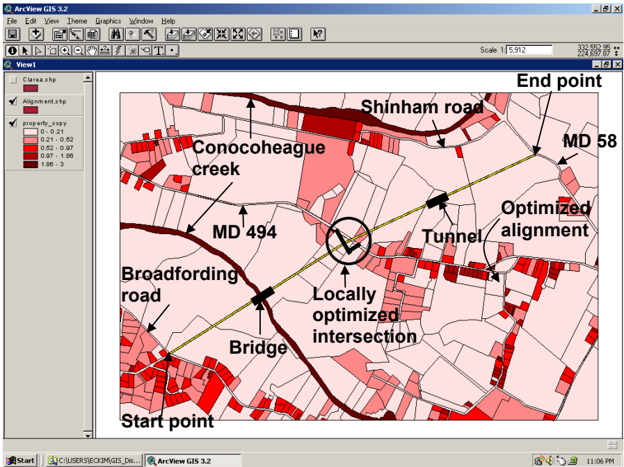
Figure 15.36: Optimized solution for the study area, Washington County, Maryland.
