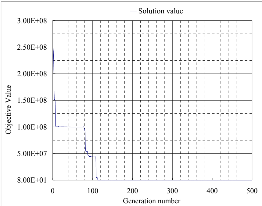
Figure 6.8: Objective values over successive generations for the test example.
