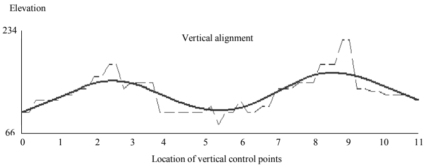
Figure 9.11: The vertical alignment of the first best solution for test example 1.
