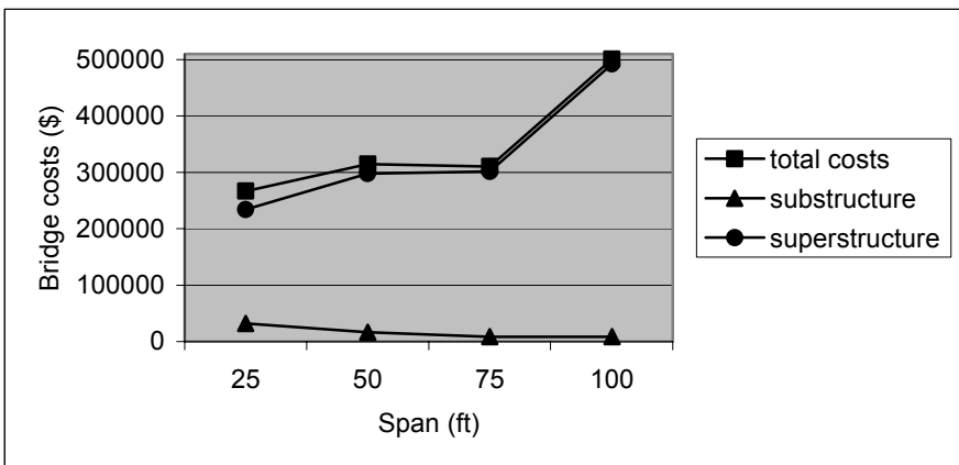
Figure 15.38: Optimized span and cost breakdown of the Washington County bridge.
