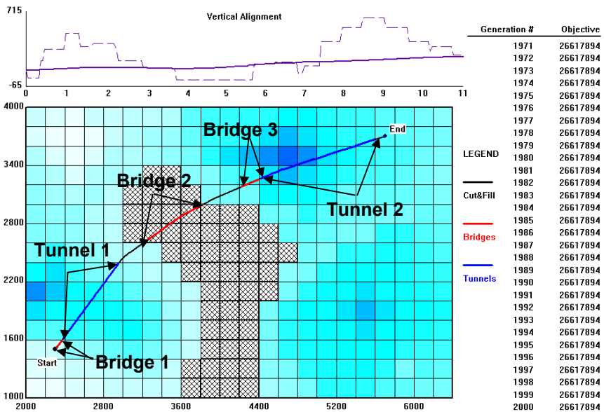
Figure 15.16: Optimized solution (scenario 1) for sensitivity analysis of tunnels.
