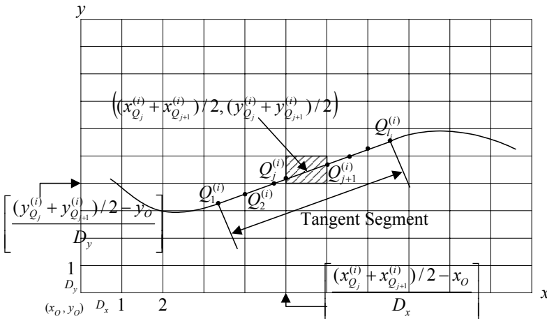
Figure 4.12: Sorted intersection points of a tangent section.
