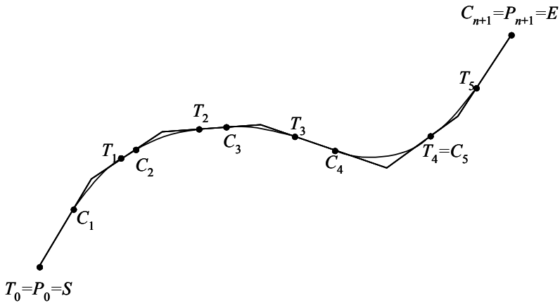
Figure 4.11: An example of points of tangency and curvature.
