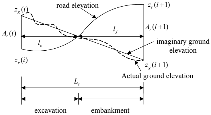
Figure 7.12: Graphical illustration of a change from cut to fill sections.
