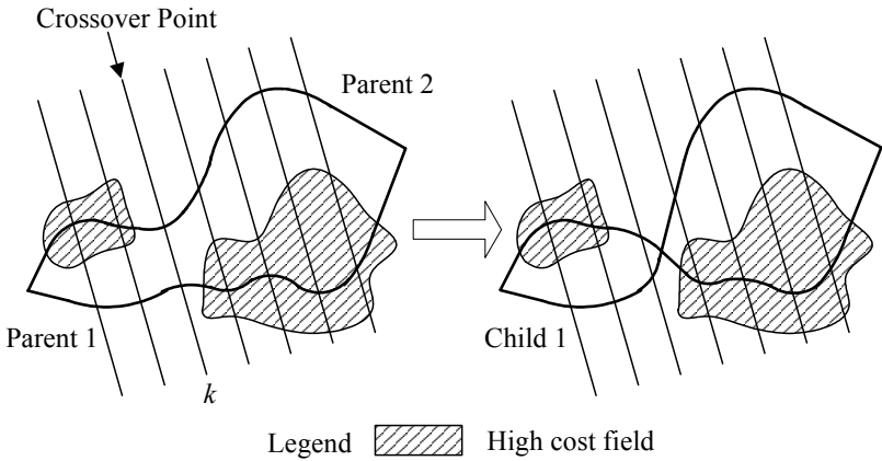
Figure 5.5: An example of a simple crossover operator.
