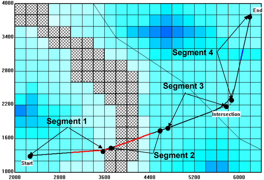
Figure 15.42: Subdividing each segment of the scenario solution 1 for a two-stage optimization.
