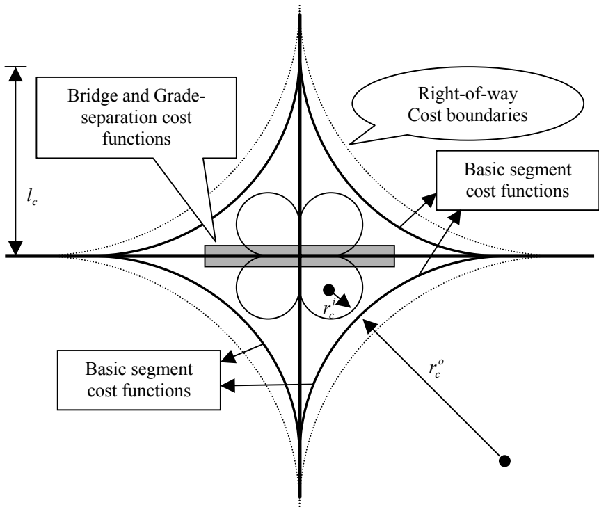
Figure 12.30: Centerlines of a typical clover interchange, major design criteria and separated parts for each cost function.
