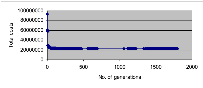
(b) Case of Figure 15.6.
