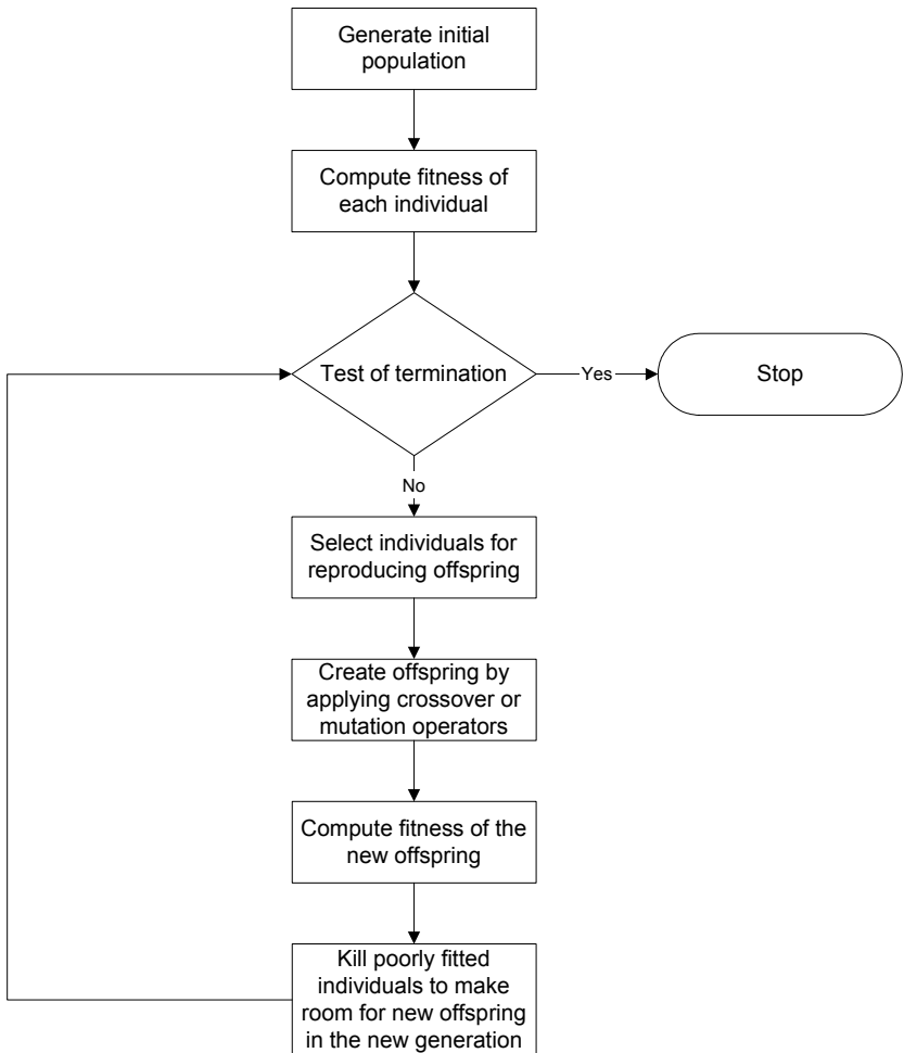
Figure A.1: The structure of Genetic Algorithms.
