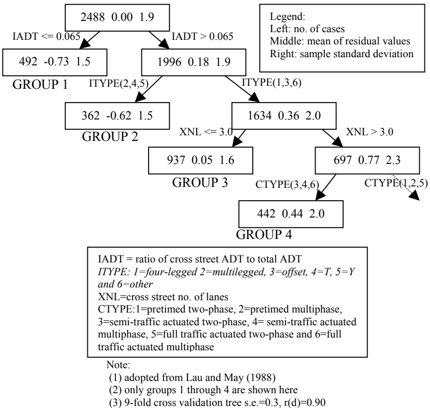
Figure 12.21: Grouping of intersections by CART.
