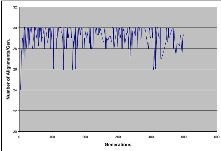
Figure 10.41: Candidate alignments vs. generation number for a map with 900 parcels/m 2 .
