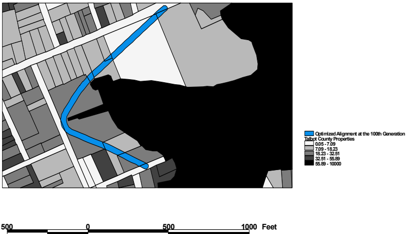
Figure 10.26: Optimized alignment for the Talbot County case obtained at the 100 th generation.
