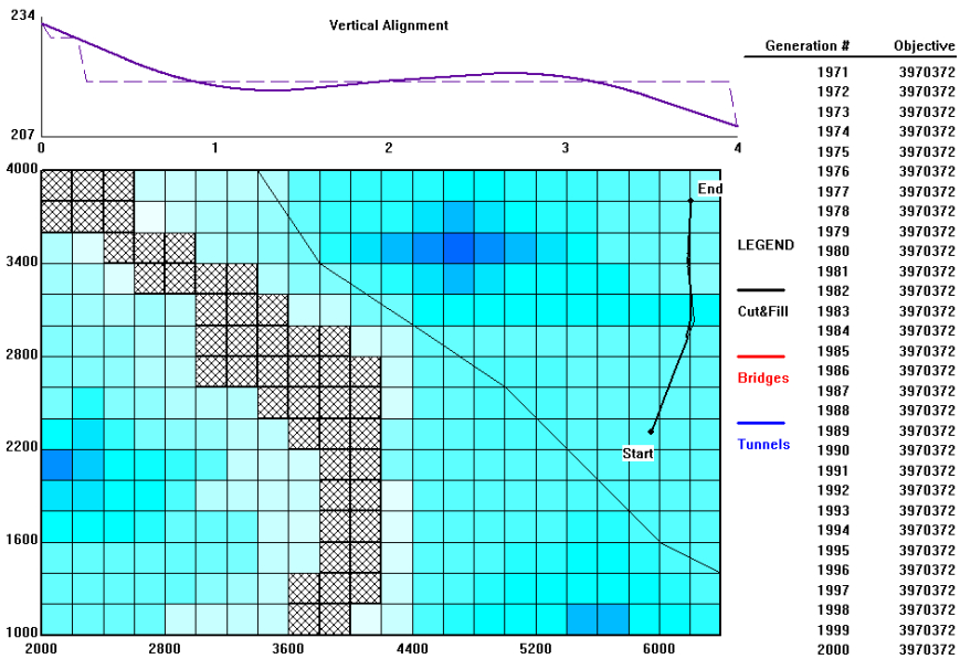
Figure 15.46: Optimized solution for segment 4 under scenario 3.
