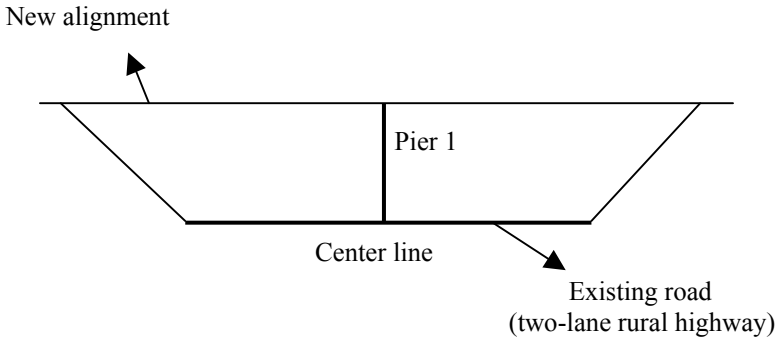
Figure 13.5: A grade separation template for a two-lane rural highway.
