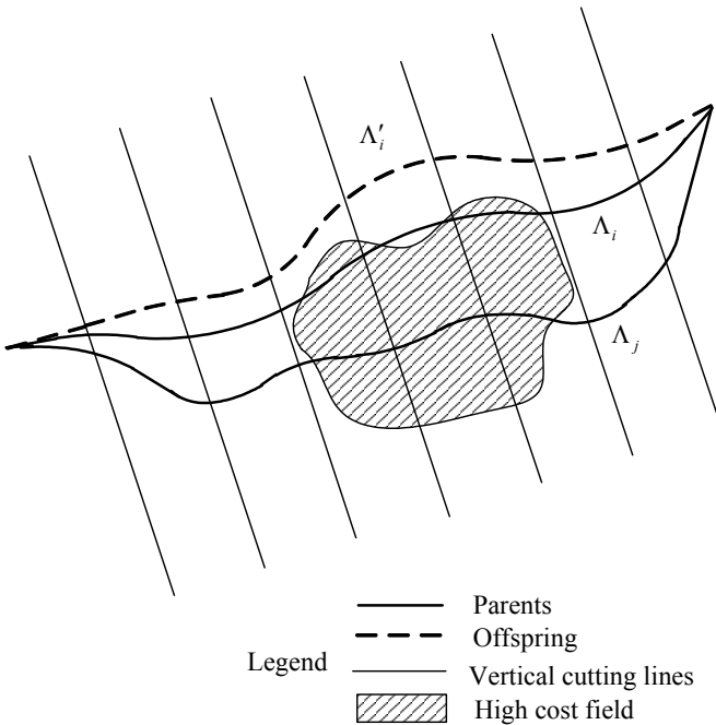
Figure 5.8: An example of a heuristic crossover operator.
