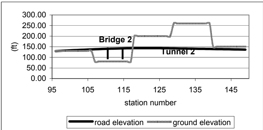
Figure 15.14: Zoomed-in profile of bridge 2 and tunnel 2 for Garrett County example.
