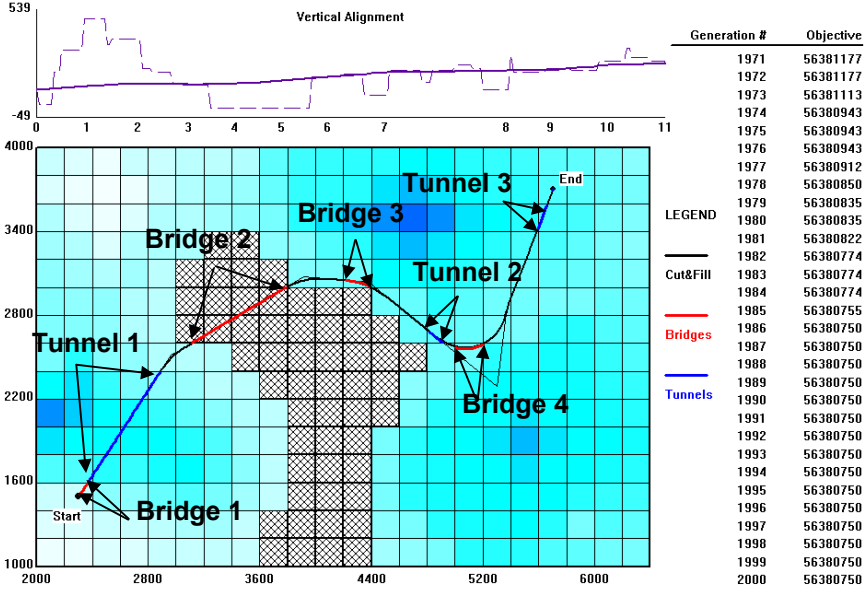
Figure 15.19: Optimized solution (scenario 4) for sensitivity analysis of tunnels.
