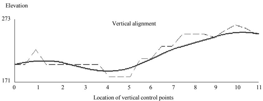
Figure 9.25: The optimized vertical alignment found by Model 3 for test example 2.
