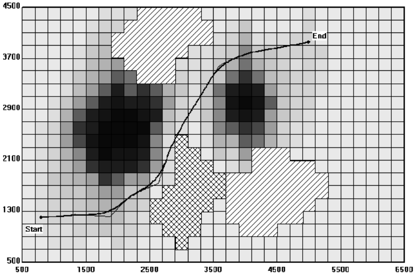
Figure 9.4: The optimized horizontal alignment for test example 1.
