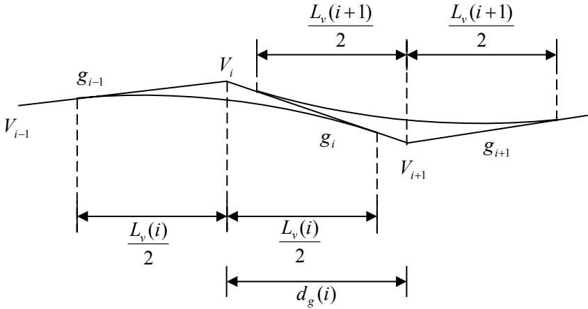
Figure 7.5: An example of discontinuity in vertical curve.
