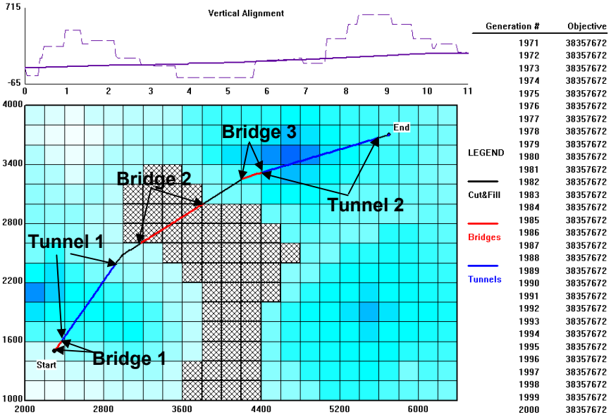
Figure 15.17: Optimized solution (scenario 2) for sensitivity analysis of tunnels.
