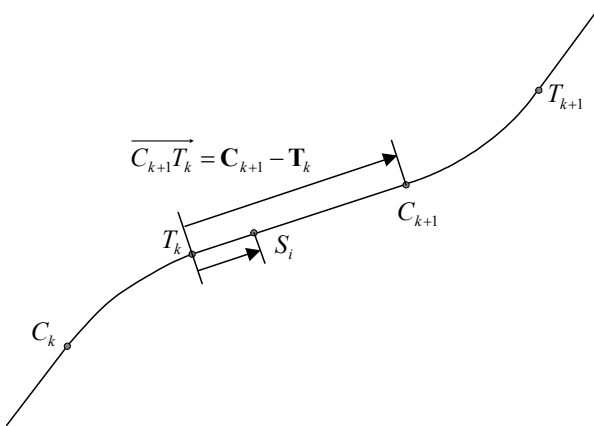
Figure 7.8: Station point on a tangent section of the horizontal alignment.
