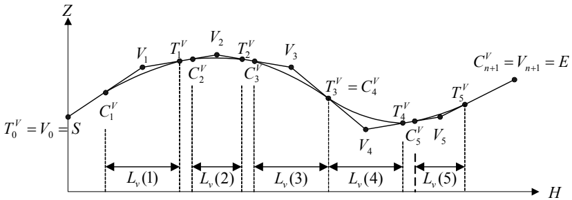
Figure 7.9: An example of vertical alignments.
