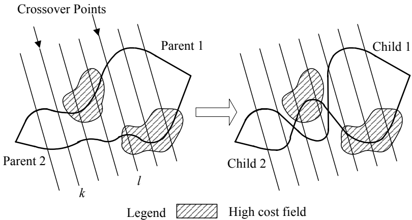
Figure 5.6: An example of a two-point crossover operator.
