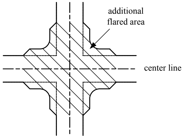
Figure 12.12: A typical four-legged intersection.
