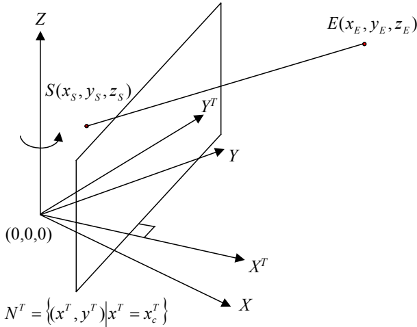
Figure 3.6: The coordinate transformation from XYZ to X^T Y^T Z .
