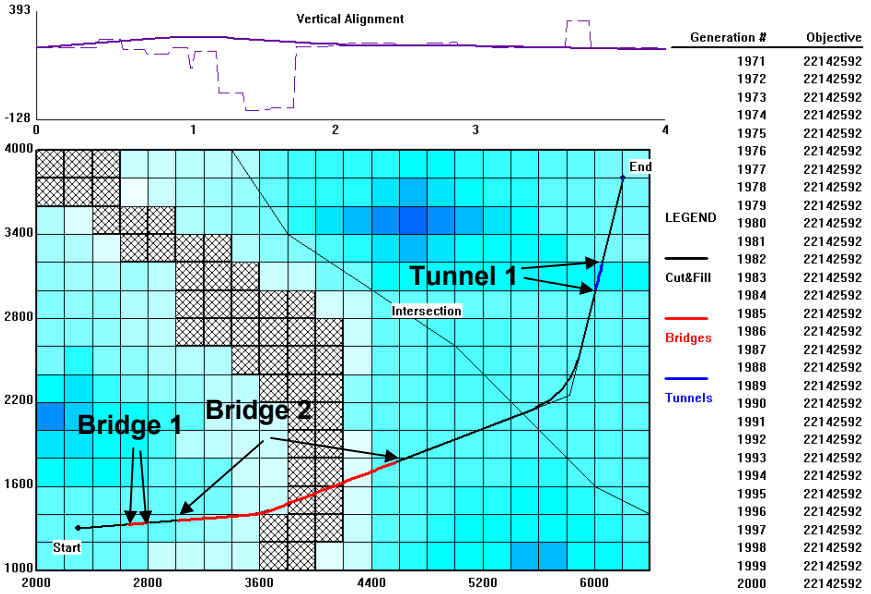
Figure 15.40: The best solution among three replications for scenario 1.
