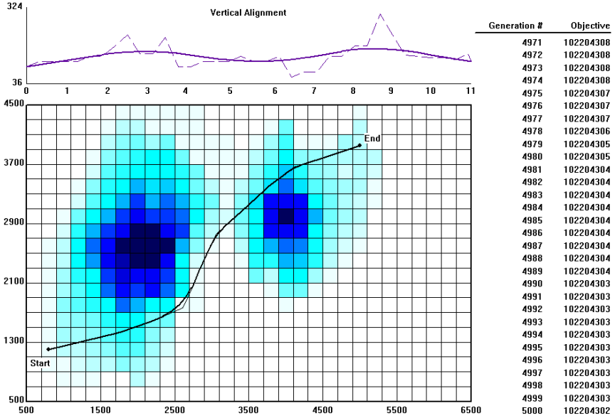
Figure 15.2: New best solution incorporating planar interpolation.
