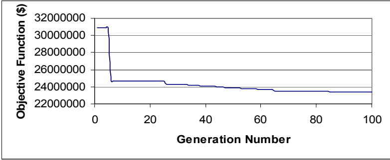
Figure 10.23: Changes in the objective function value through successive generations.
