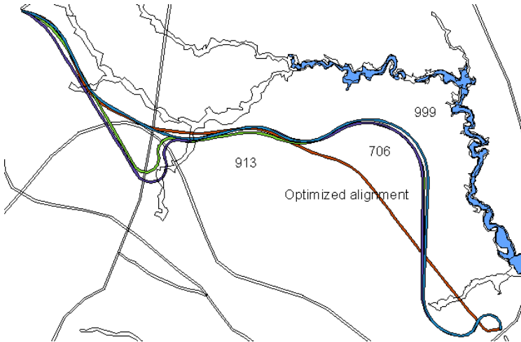
Figure 10.45: Final set of alignments.
