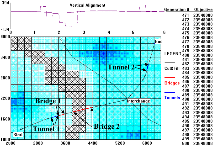
Figure 15.29: Optimized solution, considering a high water constraint and integer numbers of piers.
