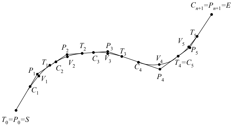
Figure 7.2: Geometric relations of reference points for an alignment on the XY plane.
