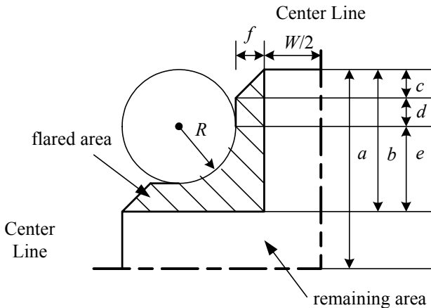
Figure 12.13: Flared and remaining areas of a typical four-legged intersection.
