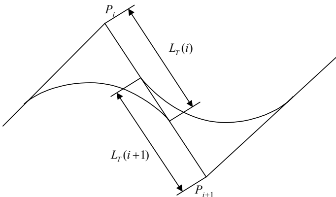
Figure 4.8: An example of discontinuity in horizontal curve.
