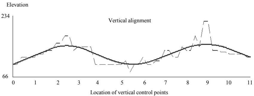
Figure 9.5: The optimized vertical alignment for test example 1.
