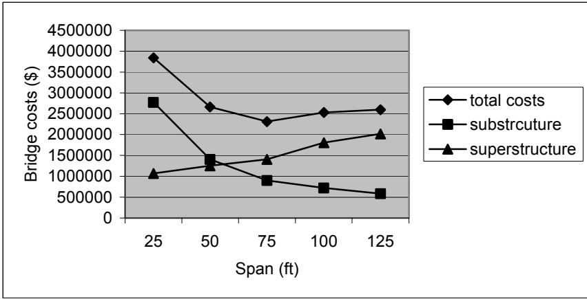
Figure 15.28: Optimal span and cost breakdown for the bridge in scenario 3.
