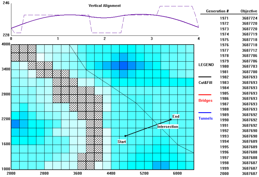
Figure 15.45: Optimized solution for segment 3 under scenario 3.
