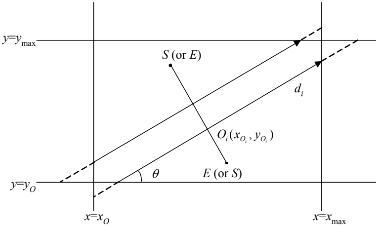
Figure 4.4: d_{iU} and d_{iL} when 0^\circ < \theta < 90^\circ .
