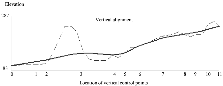
Figure 9.33: The optimized vertical alignment found by Model 3 for test example 3.
