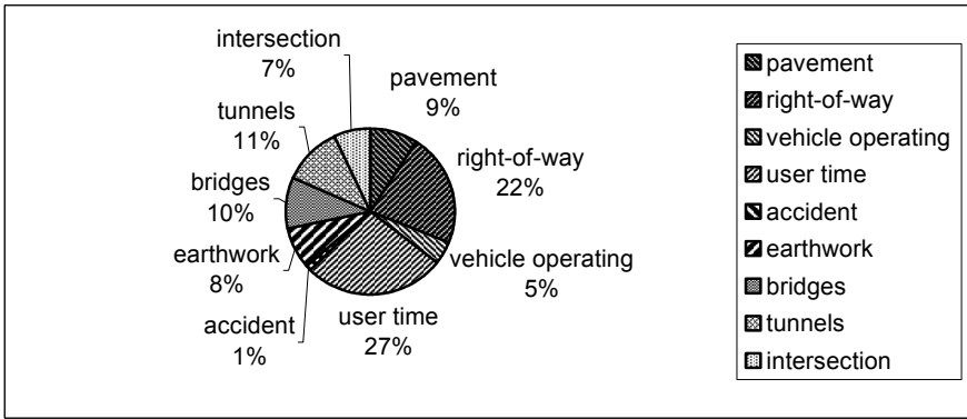
Figure 15.26: Cost breakdown for scenario 2.
