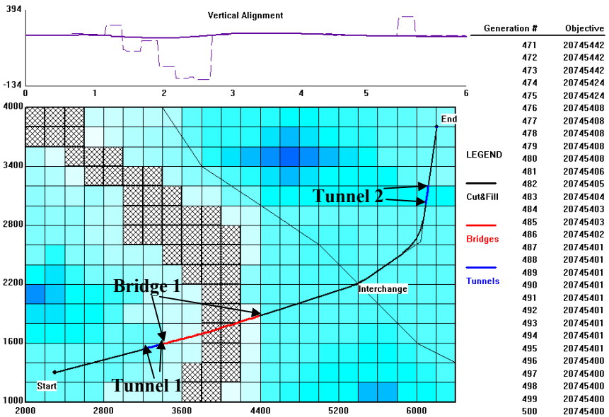
Figure 15.24: Solution for scenario 3.
