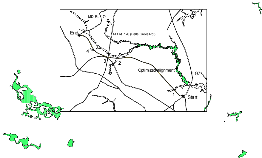
Figure 10.43: Optimized alignment at the 100 th generation.
