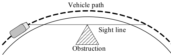
Figure 2.3: Geometry of horizontal sight distance.
