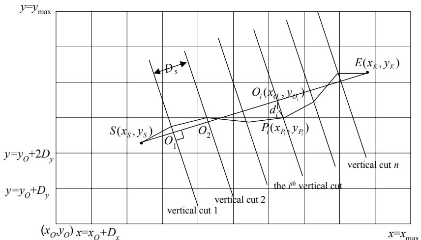
Figure 4.2: Decision variables at each vertical cut.
