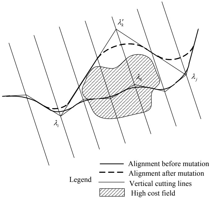
Figure 5.3: A successful example of the curve elimination procedure.
