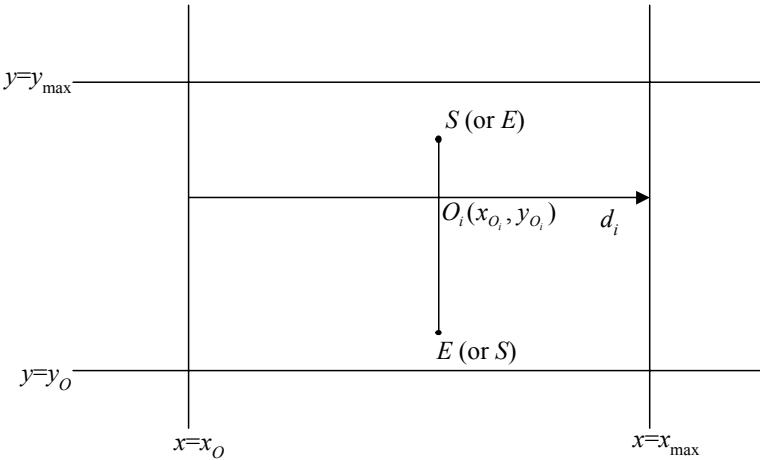
Figure 4.3: d_{iU} and d_{iL} when \theta = 0^\circ or \theta = 180^\circ .
