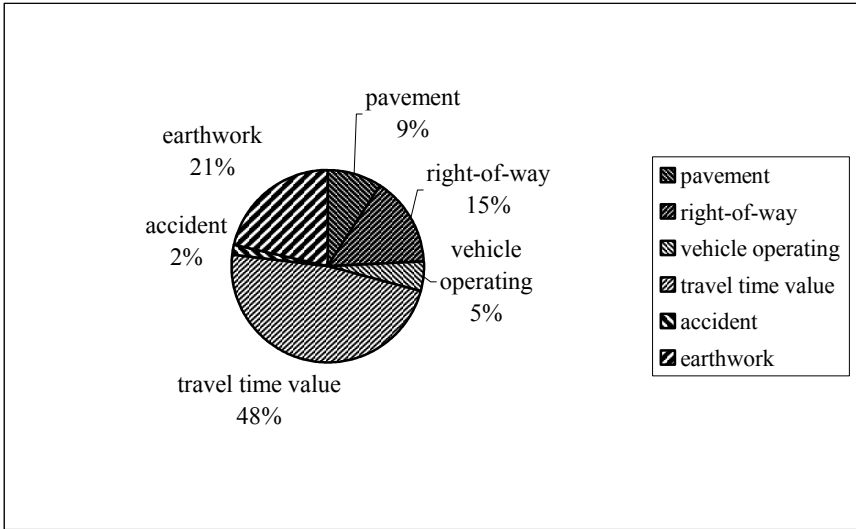
Figure 15.7: Cost breakdown for the alignment in figure 15.5.
