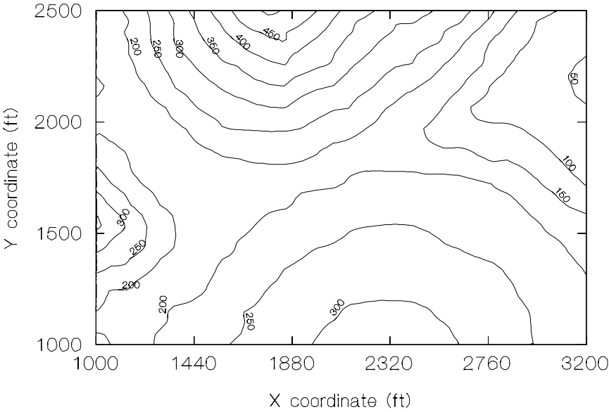
Figure 9.21: Contours of test example 2.
