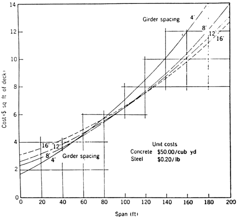
Figure 12.26: Theoretical superstructure costs of the composite girder bridge.
