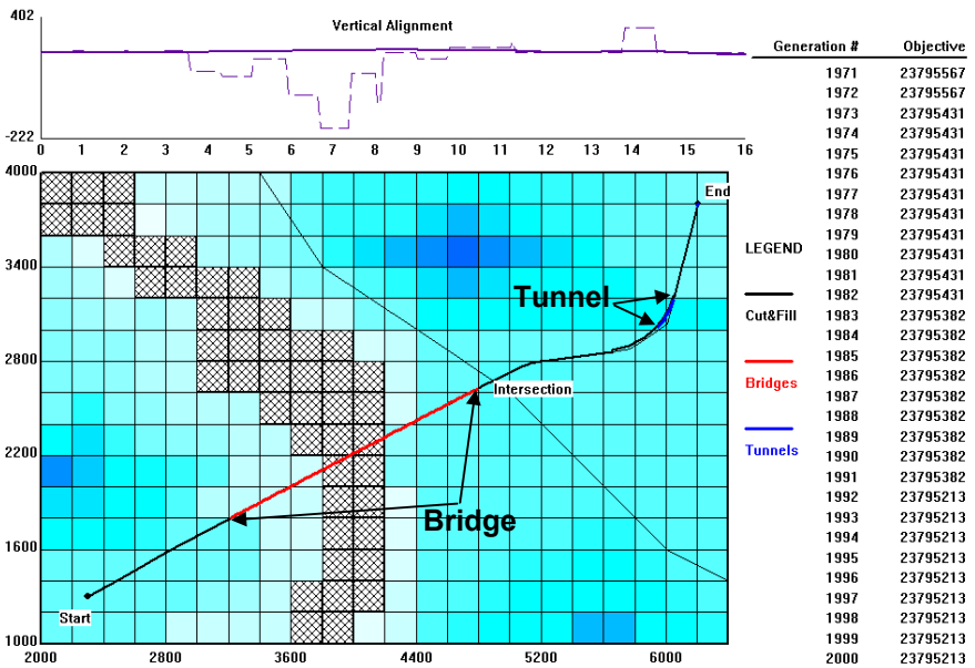
Figure 15.52: The worst solution (scenario 1).
