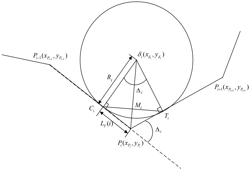
Figure 12.11: Geometric relations among C_i , T_i , \delta_i , and M_i .
