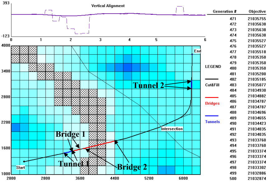
Figure 15.23: Solution for scenario 2.
