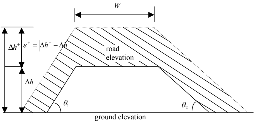
Figure 12.28: Typical cross section with insufficient vertical clearances.
