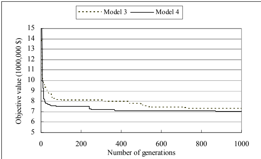
Figure 9.28: Objective value through successive generations for test example 2.
