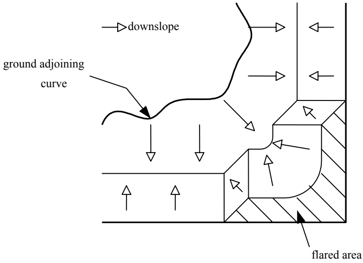
Figure 12.14: Quadrant of a typical fill intersection.
