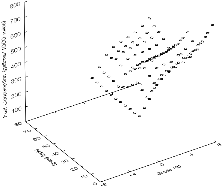
Figure 4.20: Fuel consumption data plots: 3-S2 diesel truck.
