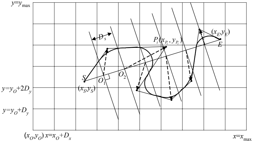
Figure 6.2: An example for modeling backtracking horizontal alignments.
