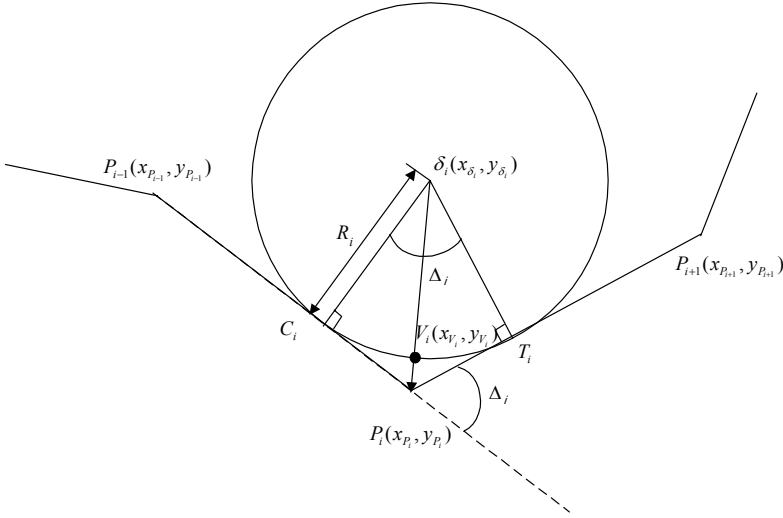
Figure 7.3: The geometric relations among V_i , \delta_i , and P_i .
