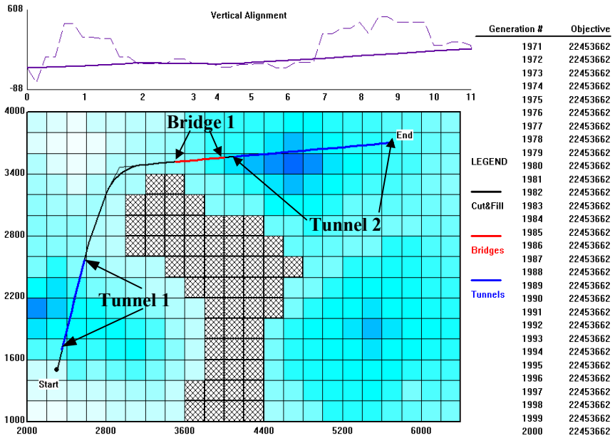
Figure 15.6: New solution with bridges and tunnels for the artificial study area.
