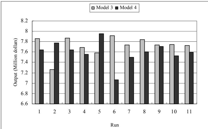
Figure 9.23: Program outputs of Models 3 and 4 for test example 2.
