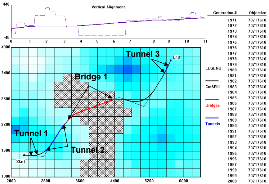
Figure 15.20: Optimized solution (scenario 5) for sensitivity analysis of tunnels.
