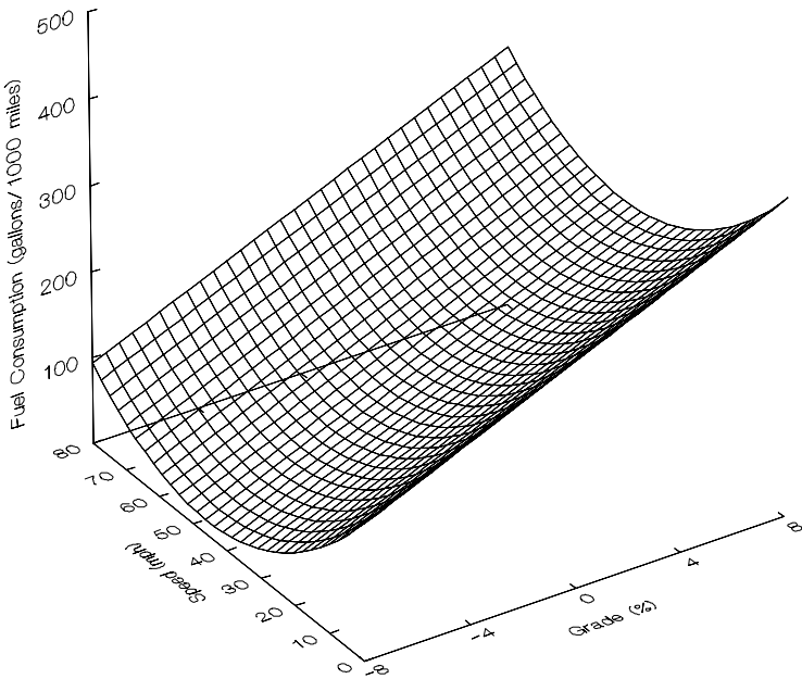
Figure 4.19: Regression function of fuel consumption: 2A-SU truck.
