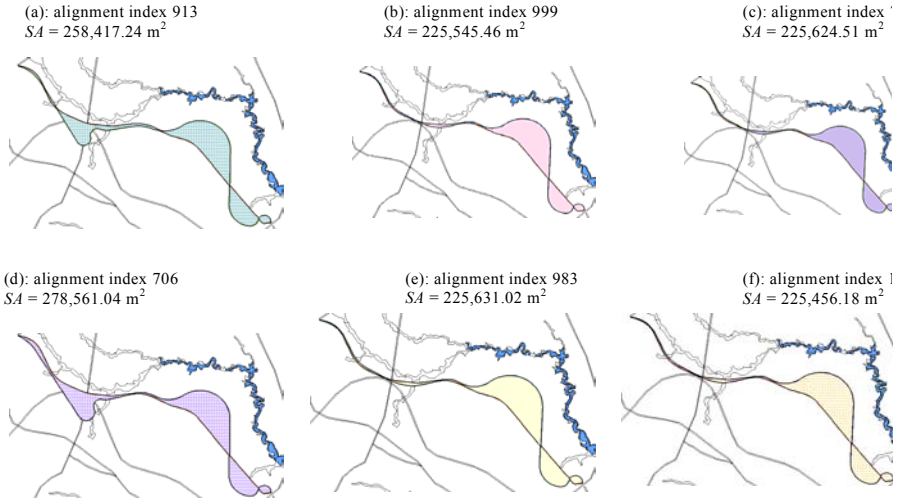
Figure 10.44: Intervening area of significantly different alignments.
