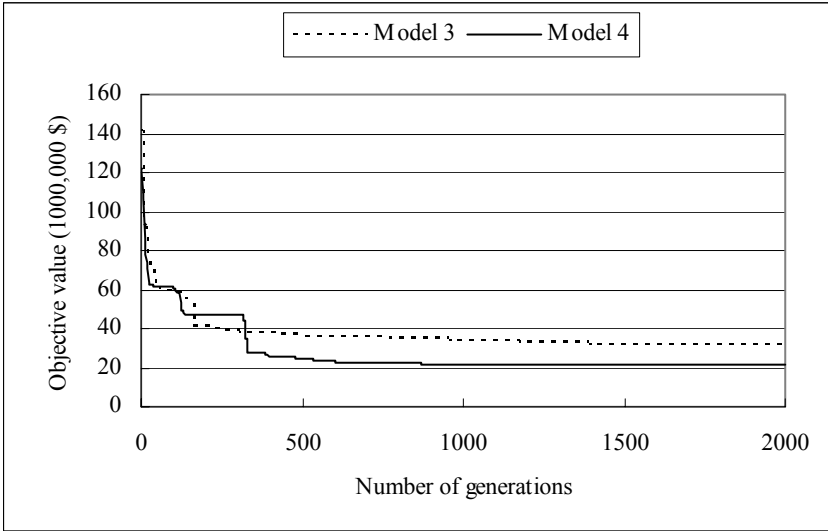
Figure 9.36: Objective value through successive generations for test example 3.
