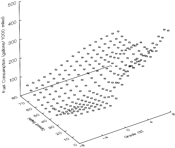
Figure 4.18: Fuel consumption data plots: 2A-SU truck.
