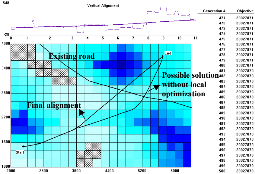
Figure 14.8: Solution in an artificial study area with 500 generations.
