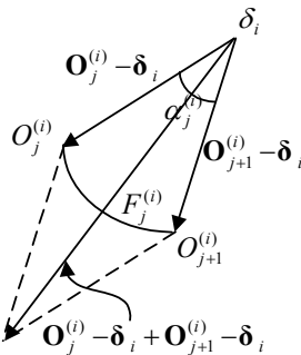
Figure 4.15: The vector presentation of eqns (4.25) and (4.29).
