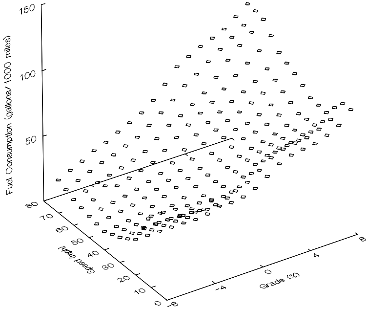
Figure 4.16: Fuel consumption data plots: medium car.
