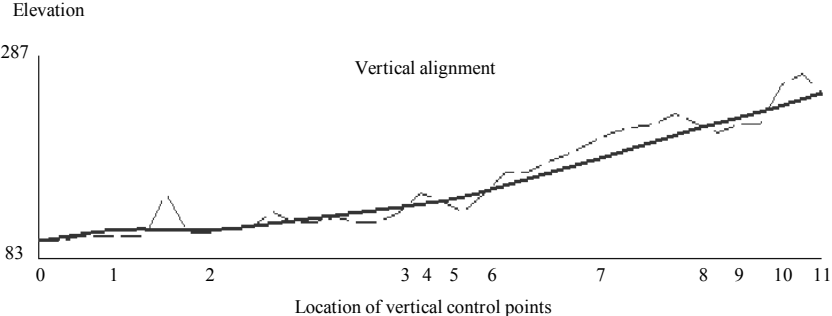
Figure 9.35: The optimized vertical alignment found by Model 4 for test example 3.
