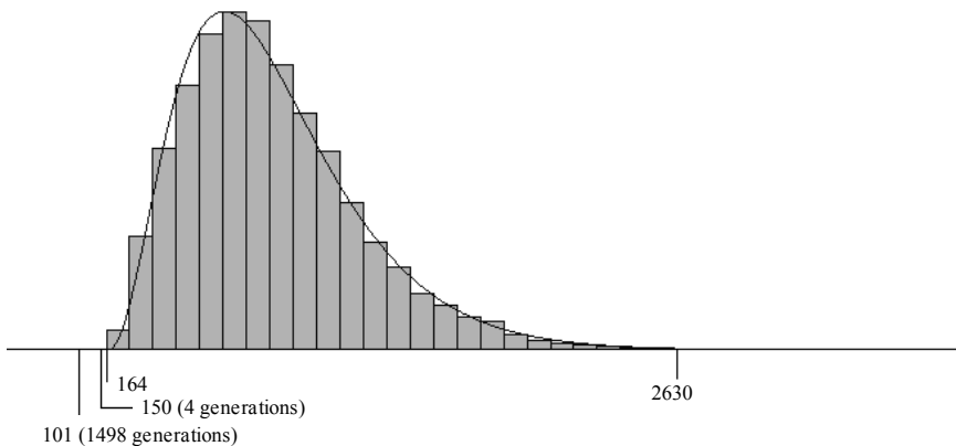
Figure 9.7: The fitted distribution of the objective value for test example 1.
