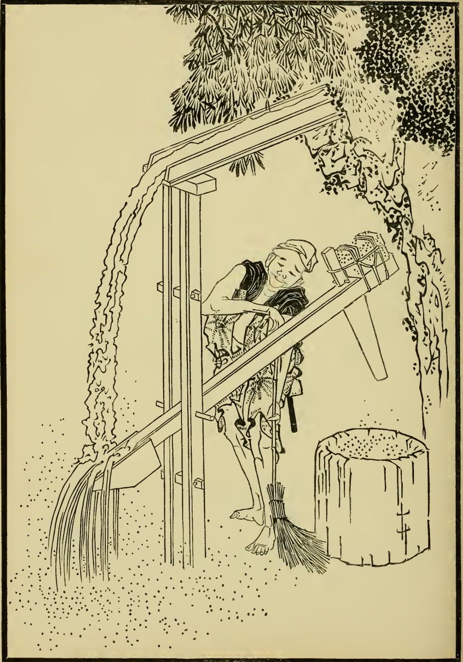
FIG. 202.—RICE MILL WORKED BY WATER POWER.
