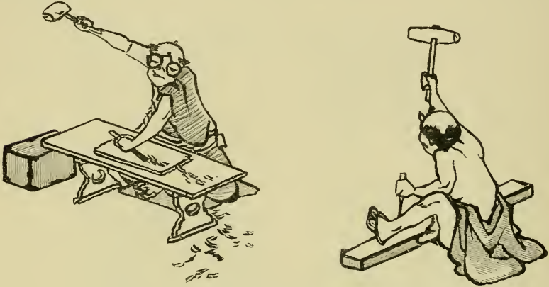
FIGS. 98, 99.—CARPENTERS AT WORK. After native drawings.
