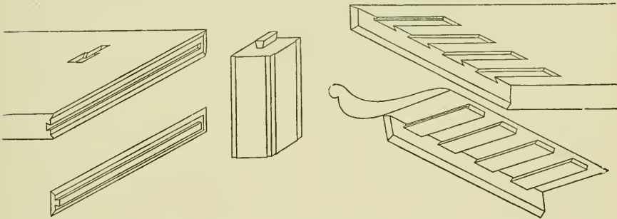
FIG. 107.—DETAILS. Showing the manner in which the parts are dovetailed together.
