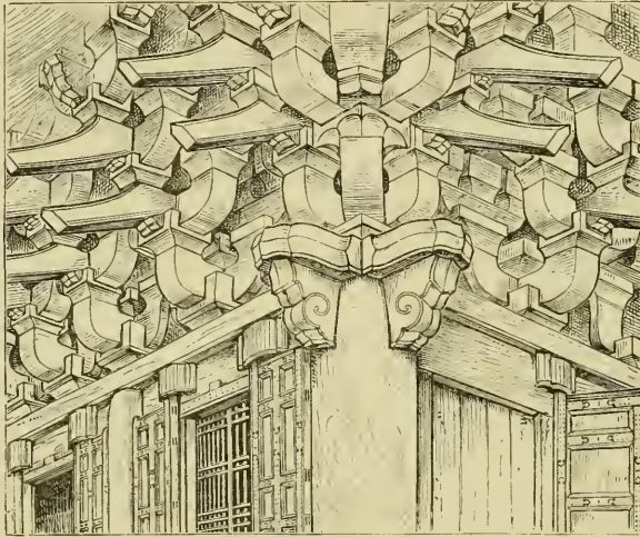
FIG. 74.—BRACKETING SUPPORTING ROOF OF TEMPLE-GATE, CHIONJIN, KIOTO.
