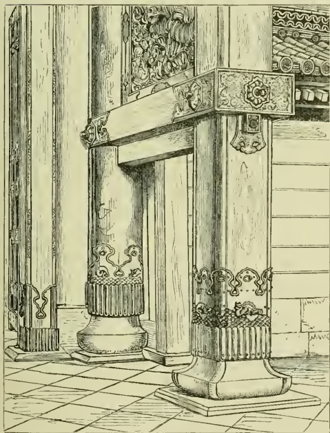
FIG. 44.—DETAILS OF EAST GATEWAY OF THE TEMPLE, NISHI-HONGWAN-JI, KIOTO.
