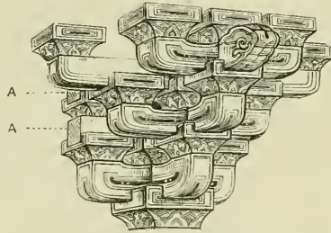
FIG. 72.—COMPOUND BRACKET.
