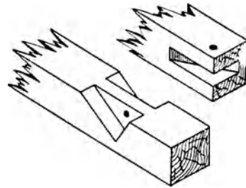
bridle joint, 1
