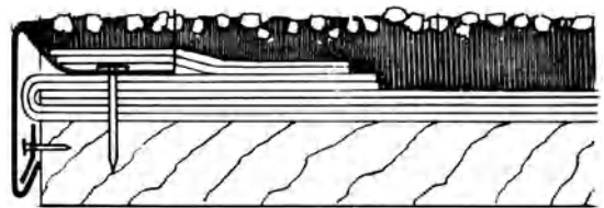
gravel stop
