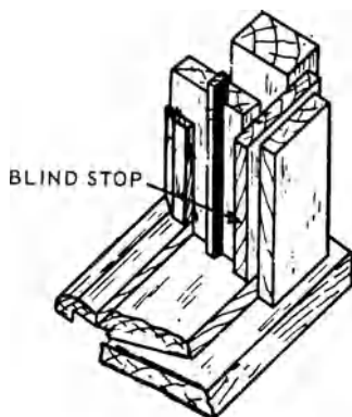
blind stop
