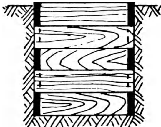
horizontal sheeting
