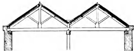
M-roof
