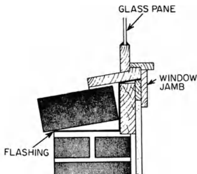
flashing
