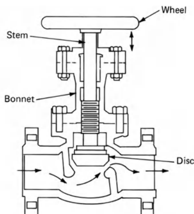
globe valve
