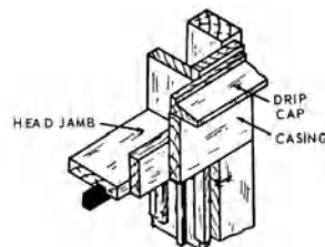
drip cap
