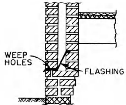
cavity flashing
