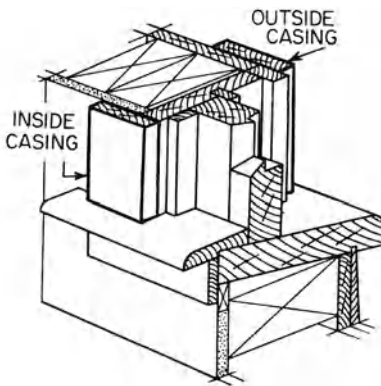
inside casing
