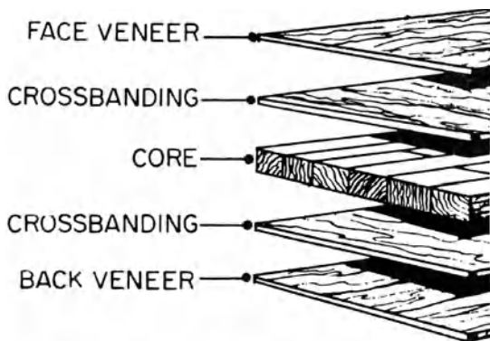
crossbanding, 1
