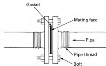
flanged joint
