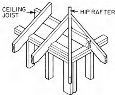
hip rafter
