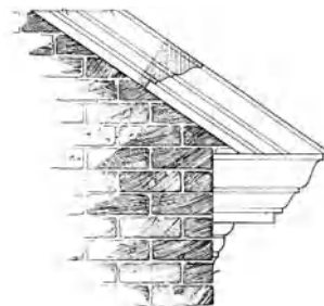
cornice return
