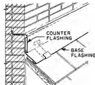
counterflashing
