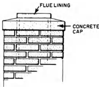
flue lining
