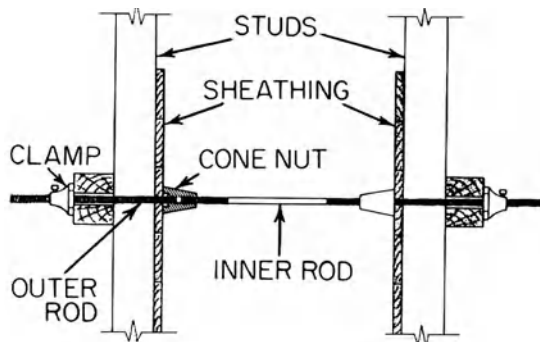
cone-nut tie
