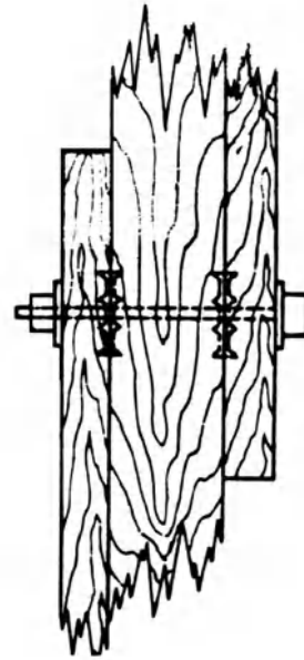
spike grid timber connector; joint employing two timber connectors is shown below
