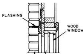
head flashing
