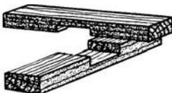
crosslap joint
