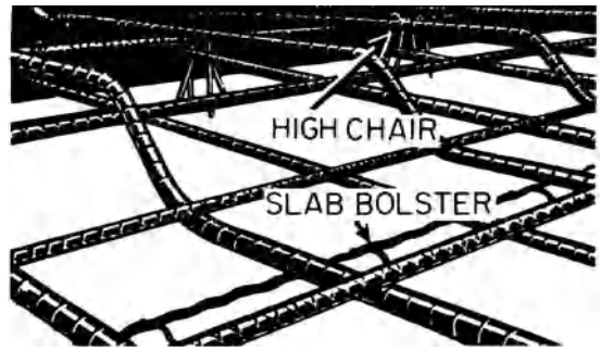
reinforcement, 1
