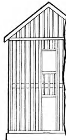
balloon framing
