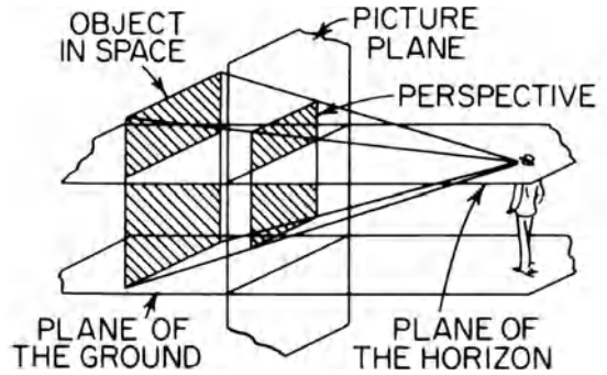
perspective drawing
