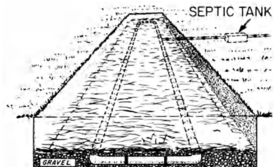
seepage bed
