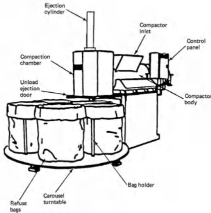
carousel packer
