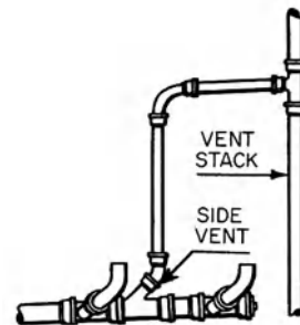
side vent
