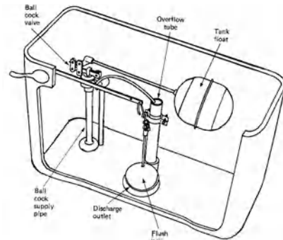
flush tank
