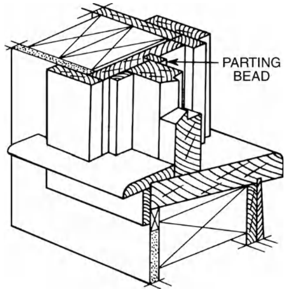
parting bead
