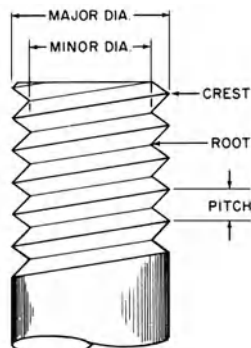
thread: terminology
