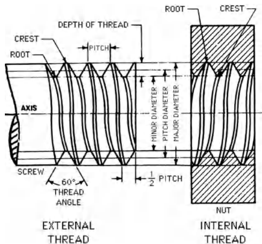
screw: nomenclature
