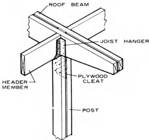
post-and-beam framing
