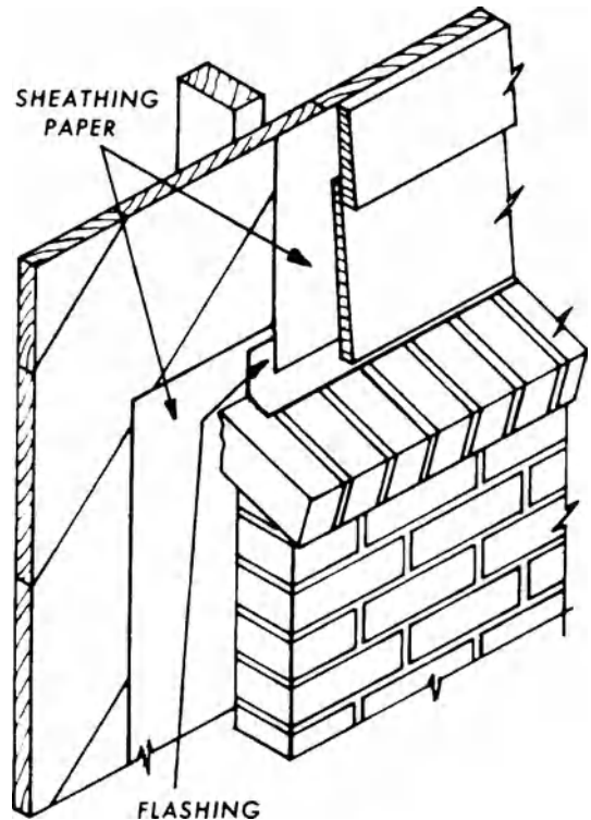
brick veneer
