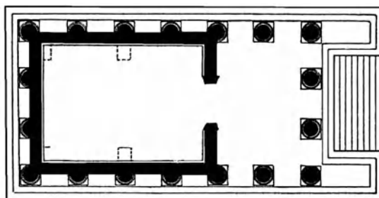
pseudoperipteral
