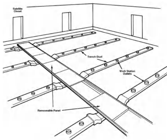
trench duct
