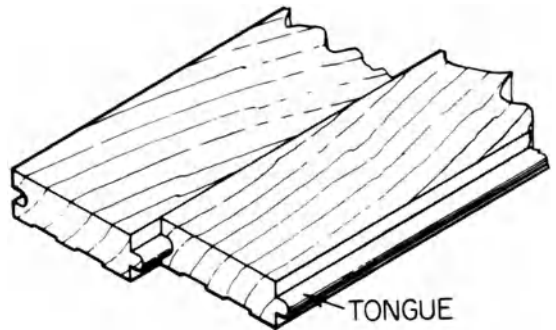
tongue-and-groove joint
