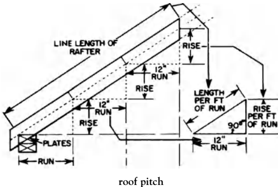
roof pitch
