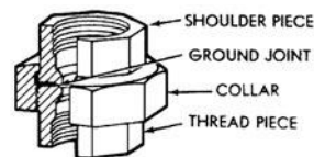
union
