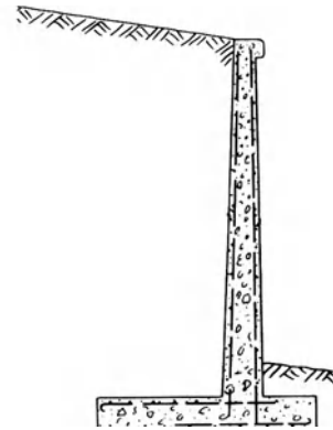
cantilever wall
