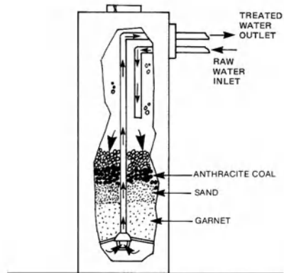
multimedia filter
