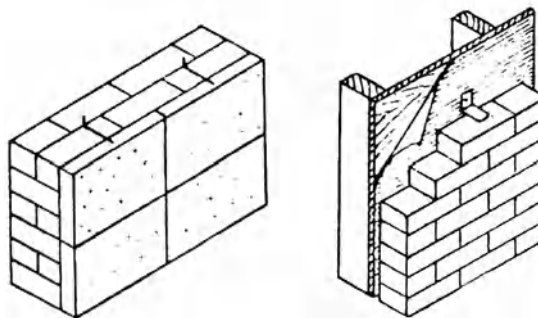
veneered construction (two types)
