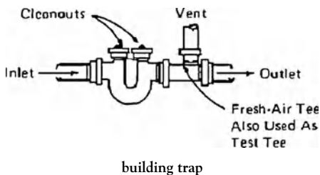
building trap
