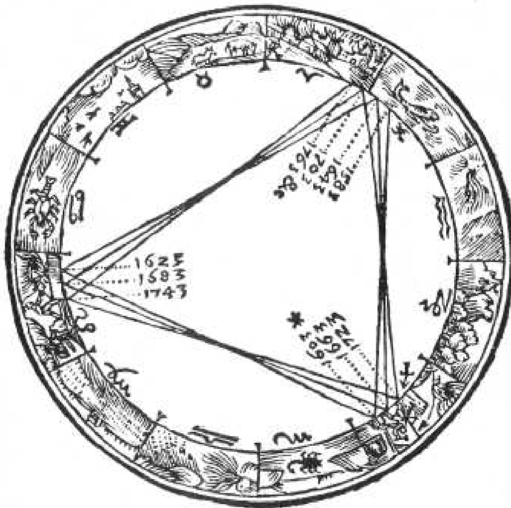
Figure 41. A detailed illustration of the motions of the Trigon of Great Conjunctions from 1583 to 1763
