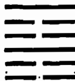
Yin
