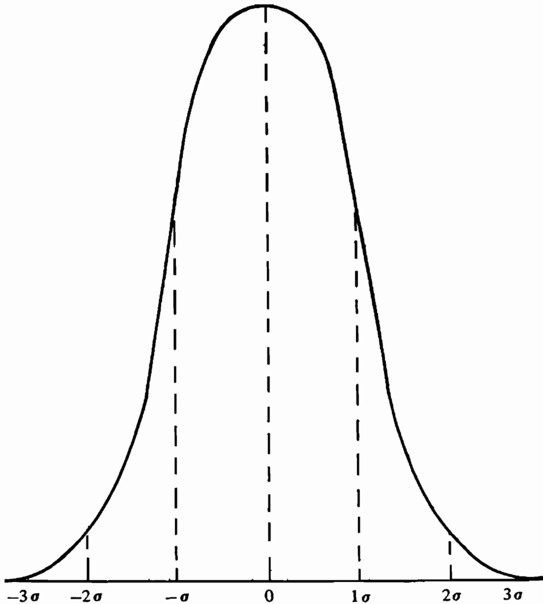
The normal curve
