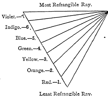
Fig. 33. PRISMATIC SPECTRUM.
