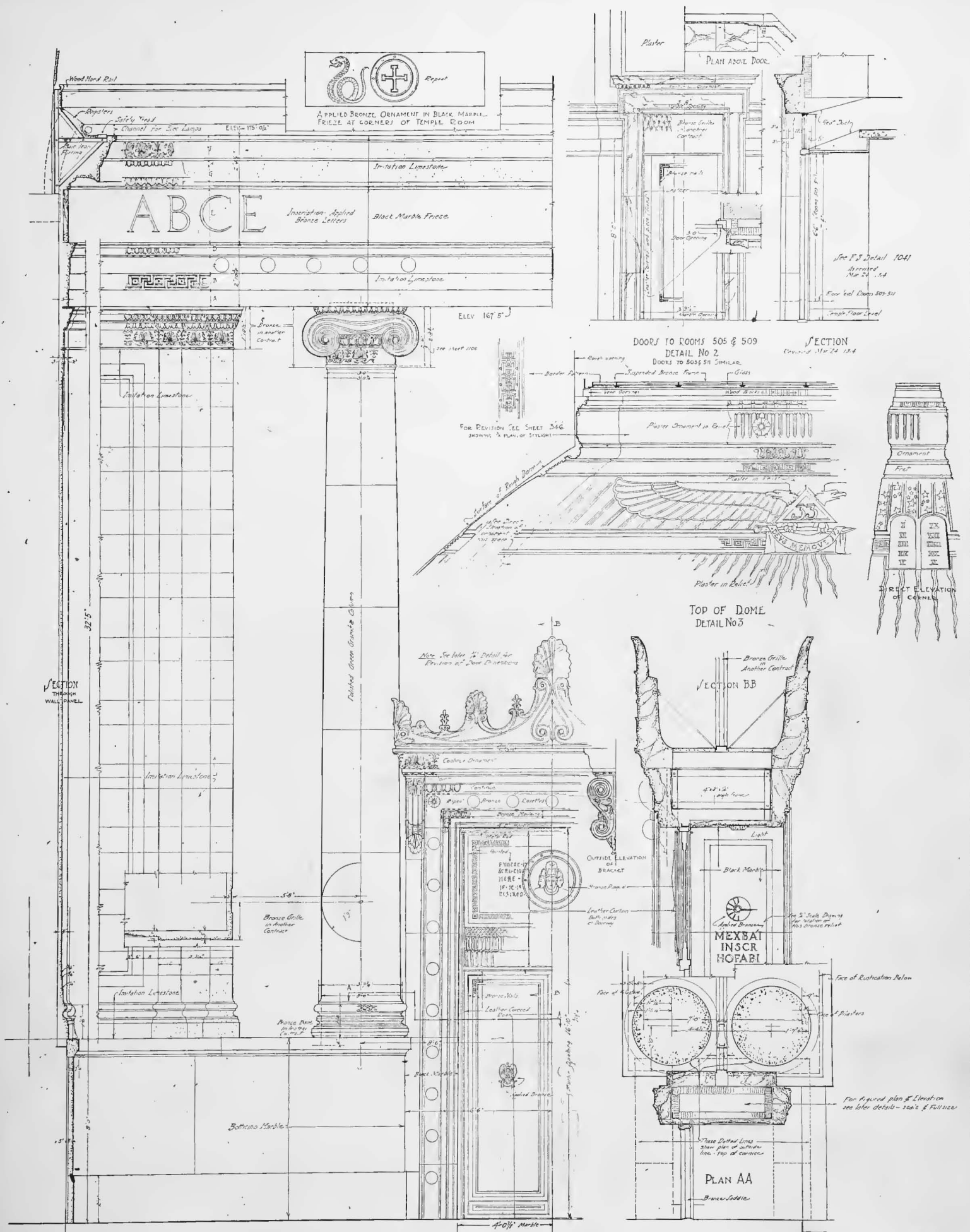
PARTIAL ELEVATION OF SIDE OF TEMPLE ROOM - SHOWING ENTRANCE DOOR - OTHER SIDES OF ROOM ARE SIMILAR. DETAIL No 1
