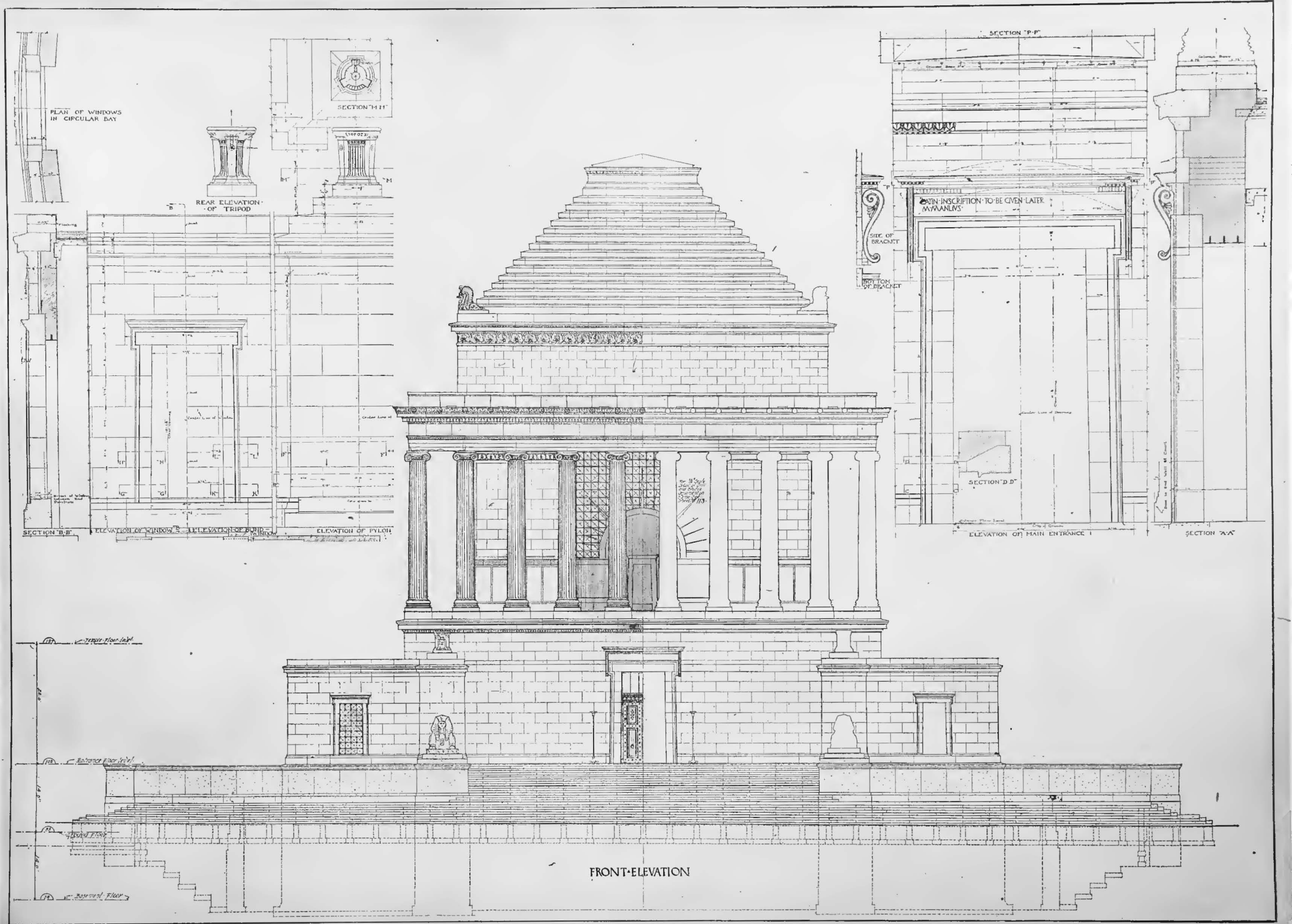
FRONT ELEVATION. ONE-TWENTY-FOURTH-INCH SCALE TEMPLE OF THE SCOTTISH RITE, WASHINGTON, D. C. JOHN RUSSELL POPE, ARCHITECT.
