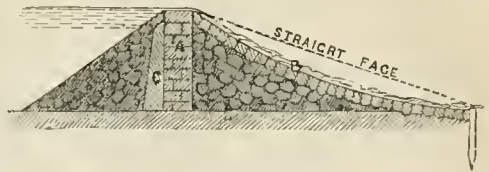
Fig. 4. A, masonry; B, pitching; C, clay puddle.
