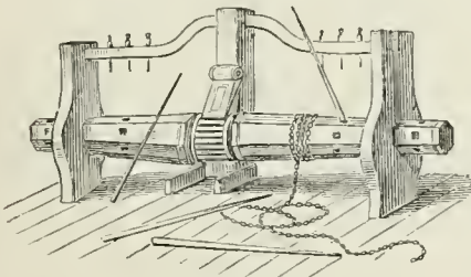
Fig. 1.—Ship's Windlass.
