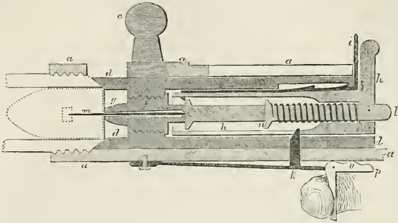
Fig. 9.—Prussian Needle-gun : Instant of firing.
