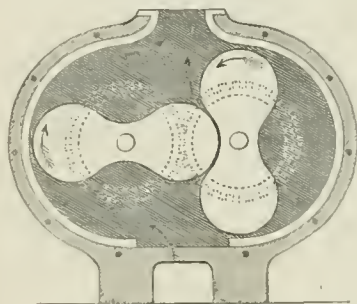
Fig. 9.—Roots' Blowing-machine.
