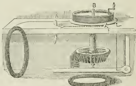
Wire-drawer's Bench.
