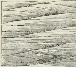
Section and External Appearance of Atlantic Cable of 1866.
