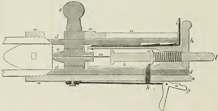
Fig. 8.—Prussian Needle-gun : Full-cock.
