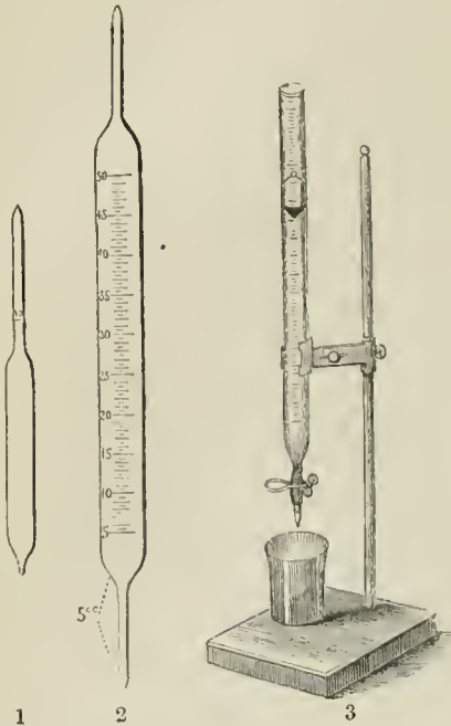
Fig. 1.—A Pipette, containing 10 c. c. Fig. 2.—A Pipette, containing 50 c. c., divided through its whole length in c. c.; being thus graduated for measuring the delivery of fluids. Fig. 3.— a , the india-rubber; b , the slips made of brass wire, by which the india-rubber tube can be closed at will.
