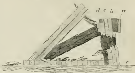
Fig. 3.—Section of do., showing the hole made by the 600-lb. shell, and displacement of the upper plate. a , armour plating, 4½ in. thick (displaced); b , teak backing, 18 in. thick; c , boiler-plate skin, ¾ in. thick; d , wrought-iron beams; e , platform.
