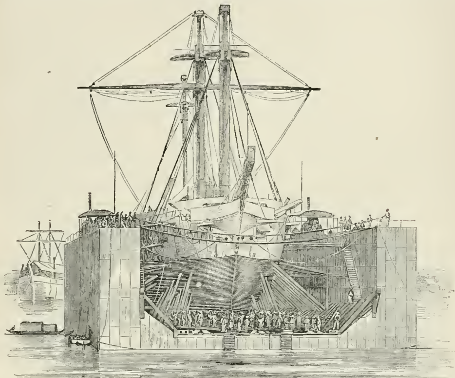
Fig. 3.—Floating-dock at Saigon, with the Persévérante of 70 guns. (From a Photograph.)
