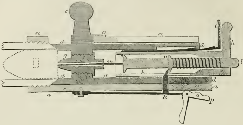
Fig. 7.—Prussian Needle-gun : Half-cock.
