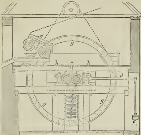
Fig. 1.—Ore Mill : End view of the crushing rollers, sieves, and bucket-wheel.
