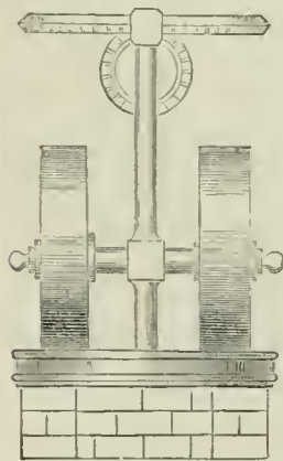
Fig. 4.—Edge-stone Mill.
