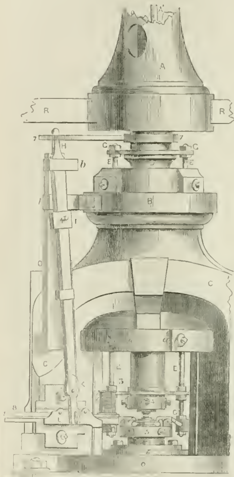
Coining-press.
