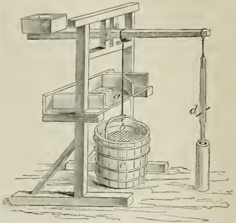
Fig. 3.—Jiggging Sieve.
