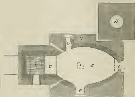
Fig. 2.—Plan of a Reverberatory Lead Furnace: a , hearth on which the ore is spread; b , fireplace or grate; c , the fire bridge; d , chimney; e , working doors; f , opening for supplying ore; g , tap-hole.
