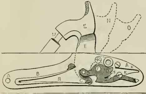
Percussion-lock.
