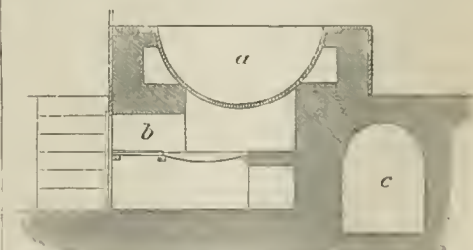
Fig. 3.—Desilverising Pot: a , pot; b , fireplace; c , main flue.
