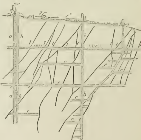
Fig. 2.—Cross-section of a Cornish Mine.
