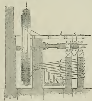
Fig. 2.—Ore Mill : Side view of the crushing rollers, sieves, and bucket-wheel.
