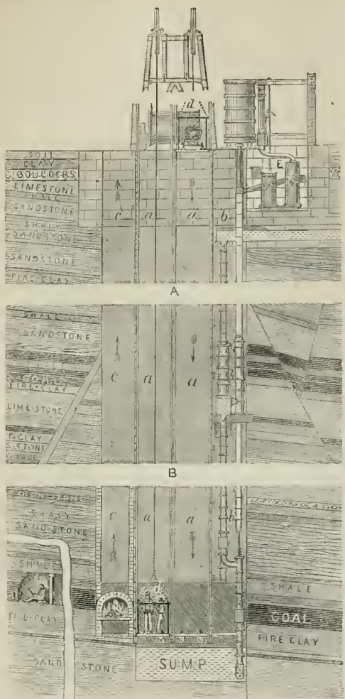
Fig. 9.—Vertical Section of the Shaft of a Coal-pit, with a Detached Portion, shewing a Miner at work on the Coal Seam.
