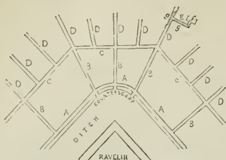
Fig. 3.—System of Countermines:
