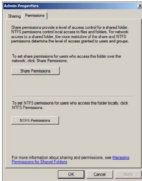
Figure 18-12: Setting permissions.
