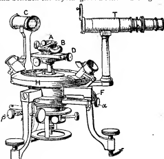
FIG. 3.—Horizontal-Circle Goniometer.
