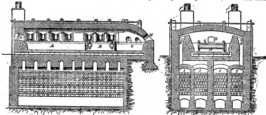
FIG. 15.—Siemens's Continuous Tank Furnace.
