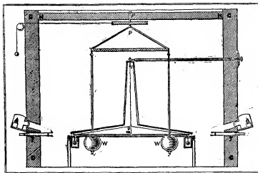
FIG. 2.—Cavendish's Apparatus.
