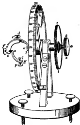
FIG. 2.—Vertical-Circle Goniometer.
