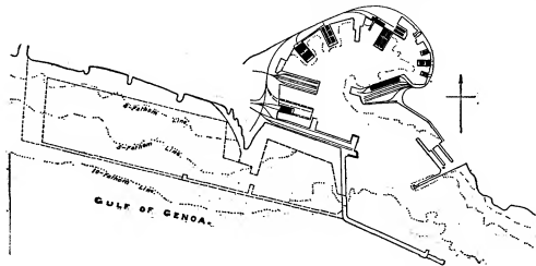
FIG. 3.—Genoa Harbour and Extensions.
