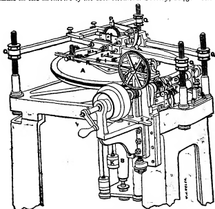
Dividing Engine.
