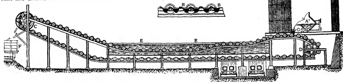
FIG. 13.—Diagram of Pig-Casting Machine.
