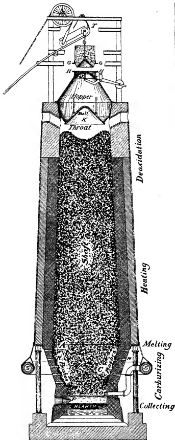
FIG. 7.—Section of Duquesne Blast Furnace.
