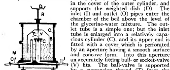
FIG. 21.—Moitessier's Gas Regulator.
