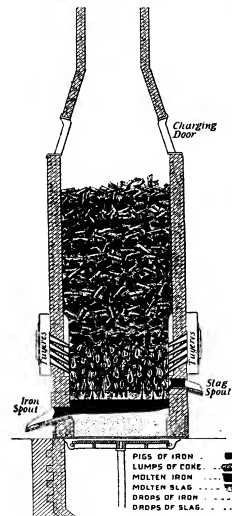
FIG. 26.—Cupola Furnace for Remelting Pig Iron.
