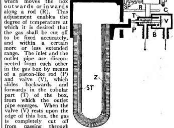
FIG. 19.—Dr Roux's Thermostat (U-shaped bar).
