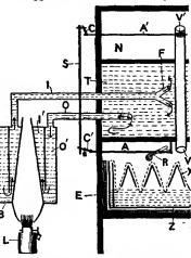
FIG. 2.—Halsted's Incubator.
