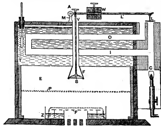
FIG. 4.—Hearson's Incubator.
