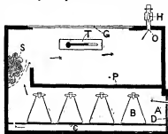
FIG. 13.—Tarnier's Incubator.
