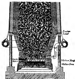
FIG. 8.—Lower Part of the Blast Furnace.
