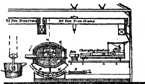
FIG. 21.—Section on CD through Body of Furnace.
