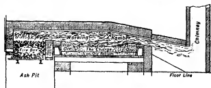
FIG. 14.—Puddling Furnace.
