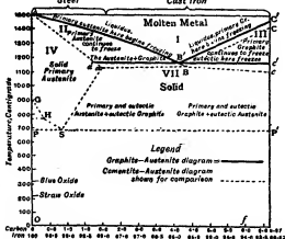
FIG. 5.—Graphite-austenite or stable carbon-iron, diagram.
