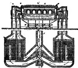
FIG. 20.—Plan through Regenerators, Flues and Reversing Valves.
