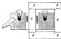
FIG. 24.—Kjellin Induction Electric Steel Melting Furnace.
