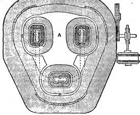
FIG. 25.—Plan of Roehling-Rodenhauser Induction Electric Furnace.
