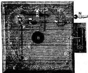
FIG. 12.—Hearson's Cool Biological Incubator.
