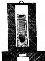
FIG. 31.—Section of Gjers Soaking Pit.
