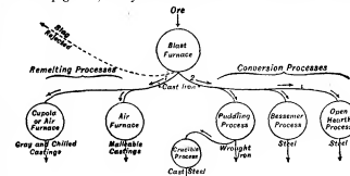
FIG. 6.—General Scheme of Iron Manufacture.
