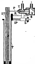
FIG. 18.—Dr Roux's Thermostat (straight bar).
