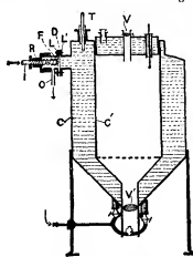
FIG. 8.—D'Arsonval Incubator.
