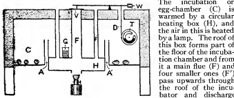
FIG. 7.—Hillier's Incubator.
