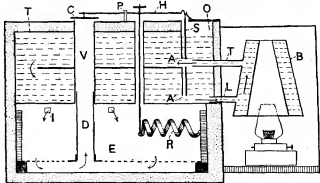
FIG. 1.—Christy's Improved Incubator.
