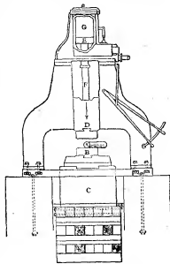
FIG. 37.—Steam Hammer.
