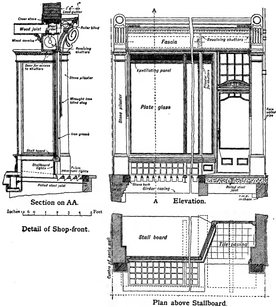
FIG. 10.—Shop-front.
