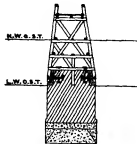
FIG. 2.—Dunkirk East Jetty.
