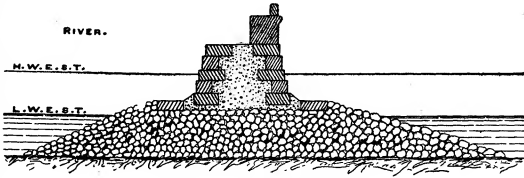
FIG. 6.—River Nervion Outlet, Western Jetty.
