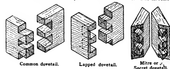
FIG. 3.—Dovetails.
