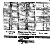
FIG. 4.—Prevention of Warping.
