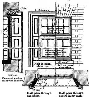
FIG. 8.—Casement window fitted with shutters.
