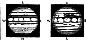
FIG. 2.—Jupiter, 1903, July 10, 2:50 a.m.
