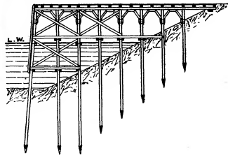
FIG. 1.—Timber Jetty across Dock Slope.
