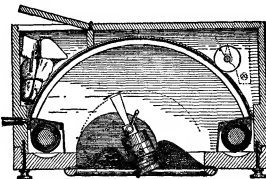
Fig. 11.—Section of "Al-Vista" Panoramic Camera.
