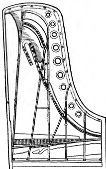
FIG. 33.—Steinway's Grand Piano, 1884. Metal framing in a single casting and overstrung.
