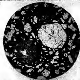
FIG. 3.—LEUCITE-BASANITE, VESUVIUS ( \times 8 ).
