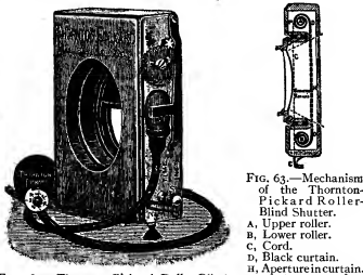
FIG. 62.—Thornton-Pickard Roller-Blind Shutter with automatic exposure roller-appliance.
