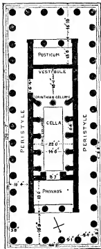
Plan of the Temple at Bassae.
