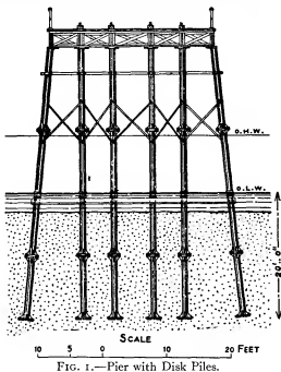
Fig. 1.—Pier with Disk Piles.
