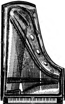
Fig. 34.—Broadwood Barless Grand.
