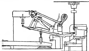
FIG. 26.—Erard's Double Escapement Action, 1884. The double escapement or repetition is effected by a spring in the balance pressing the hinged lever upwards, to allow the hopper which delivers the blow to return to its position under the nose of the hammer, before the key has risen again.
