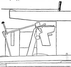
FIG. 23.—Grand Piano Action, 1776. The "English" action of Americus Backers.
