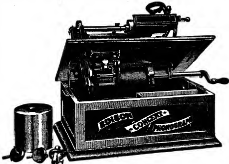
FIG. 1b.—Mechanism of Edison Phonograph.
