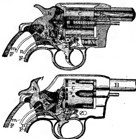
FIGS. 7 and 8.—Colt double-action revolver.
