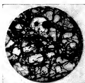
FIG. 5.—PERLITIC PITCHSTONE, MEIßSEN, GERMANY (×15).
