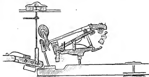
FIG. 27.—Steinway's Grand Piano Action, 1884. The double escapement as in Erard's, but with shortened balance and usual check.
