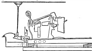
FIG. 24.—Broadwood's Grand Piano Action, 1884. English direct mechanism.
