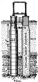
Fig. 2.—Cylindrical Piers for River Bridges.
