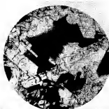
FIG. 6.—OPHITIC OLIVINE-DOLERITE, DUN FION, ARRAN, SCOTLAND.
