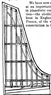
FIG. 30.—Allen's Compensating Grand Piano, 1820. The first complete metal framing system applied over the strings.
