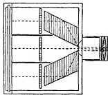
FIG. 13.—Diagram of Camera for Three-colour Photography.
