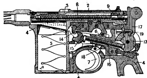
FIG. 9.—Mauser pistol ( Text-book of Small Arms , by permission of the Controller of H. M. Stationery Office).
