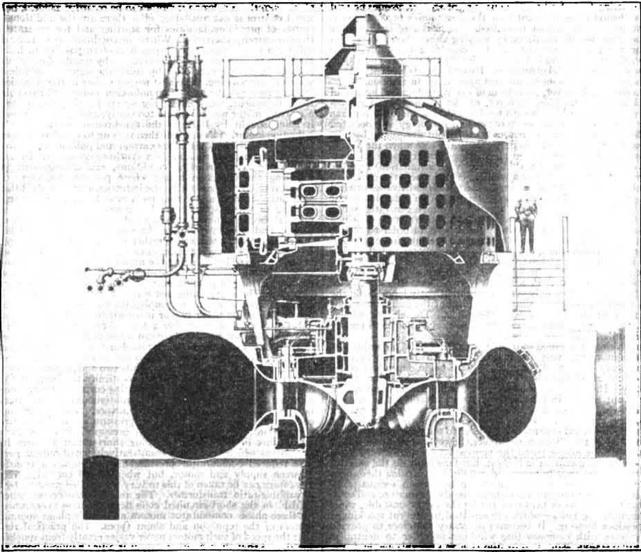
FIG. 3.—32,500-kva. Combined Water-Turbine and Alternator.
