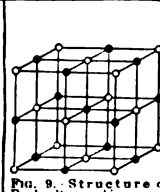
FIG. 9. Structure of Rocksalt (sodium and chlorine atoms in simple cubic space-lattice); or all of the same kind, or Zinc-blende when of two kinds.
