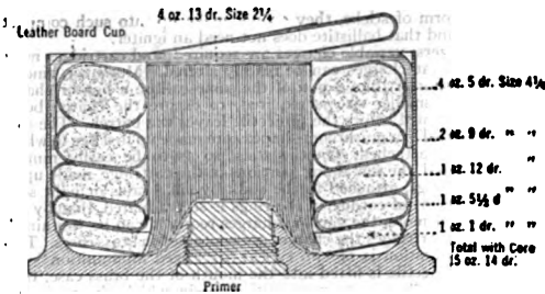
FIG. 1.—4-5 in. Q. F. Howitzer Cartridge.
