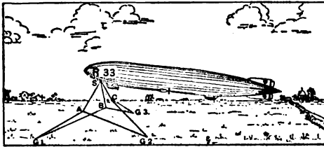
G. I. G. S. Denotes swivelling Pulley attached to Ground Bollards S. Denotes Mooring Point, A, B, C. Denotes Rings.
