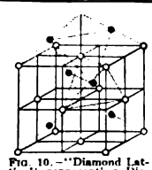
FIG. 10.—"Diamond Lattice" representing Diamond when the atoms are cubic space-lattice; or all of the same kind, or Zinc-blende when of two kinds.
