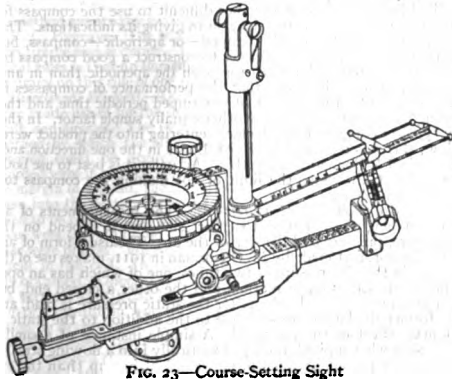
FIG. 23—Course-Setting Sight
