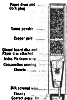
FIG. 2.—Tube, Vent Sealing, Electric W. P.
