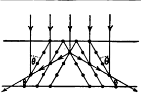
FIG. 7.—Reflection of X Rays by Planes of Particles: production of spots in the Laue photographs.
