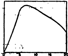
FIG. 6b.—Variation of the ratio of lift to Resistance for the wing alone as the Angle varies.
