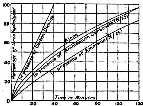
FIG. 4. Behaviour of Urease under Action of Enzyme.
