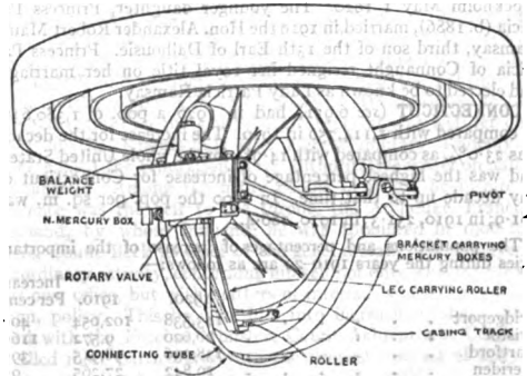
FIG. 4.—General view of mercury control.
