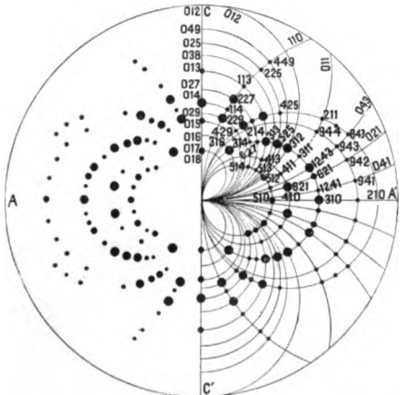
FIG. 8.—Stereogram of Laue Photograph of Anhydrite on the Face (100).
